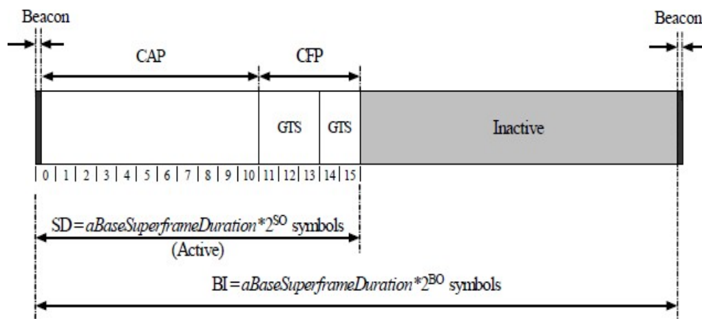
Fig: An example of the Super Frame structure
