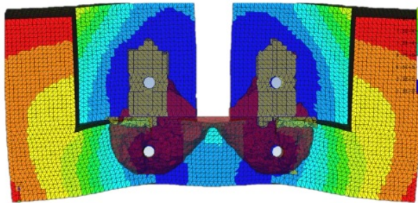
Figure 25 – Final optimised bracket projected onto the displacement study
