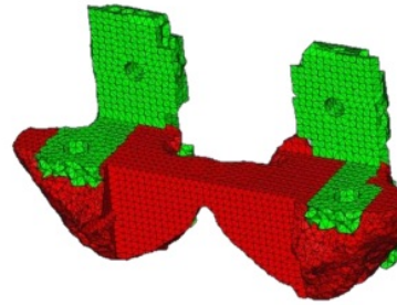
Figure 18 - Optimisation results with second element group (View 2)
