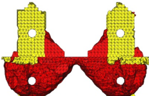
Figure 21 - Optimisation results with modified element group (View 1)
