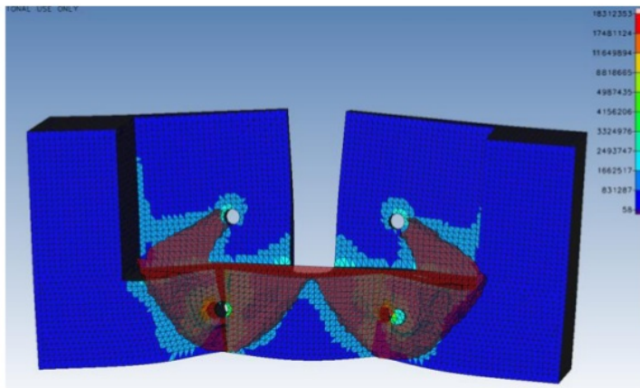
Figure 13 – Optimised bracket projected onto the stress study
