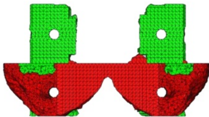
Figure 16 – Optimisation results with second element group (View 1)
