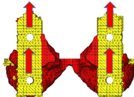
Figure 22 – Arrows indicating the force acting in the Z direction
