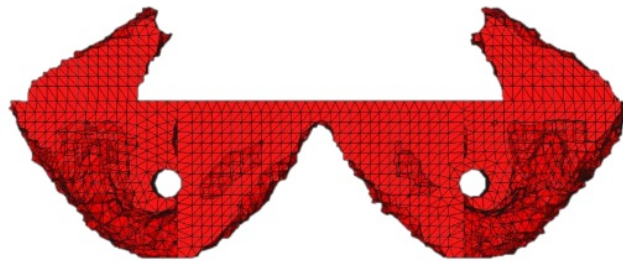
Figure 12 – First optimised bracket
