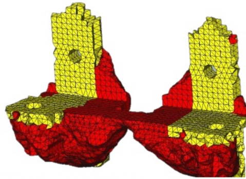
Figure 23 - Optimisation results with modified element group (View 2)
