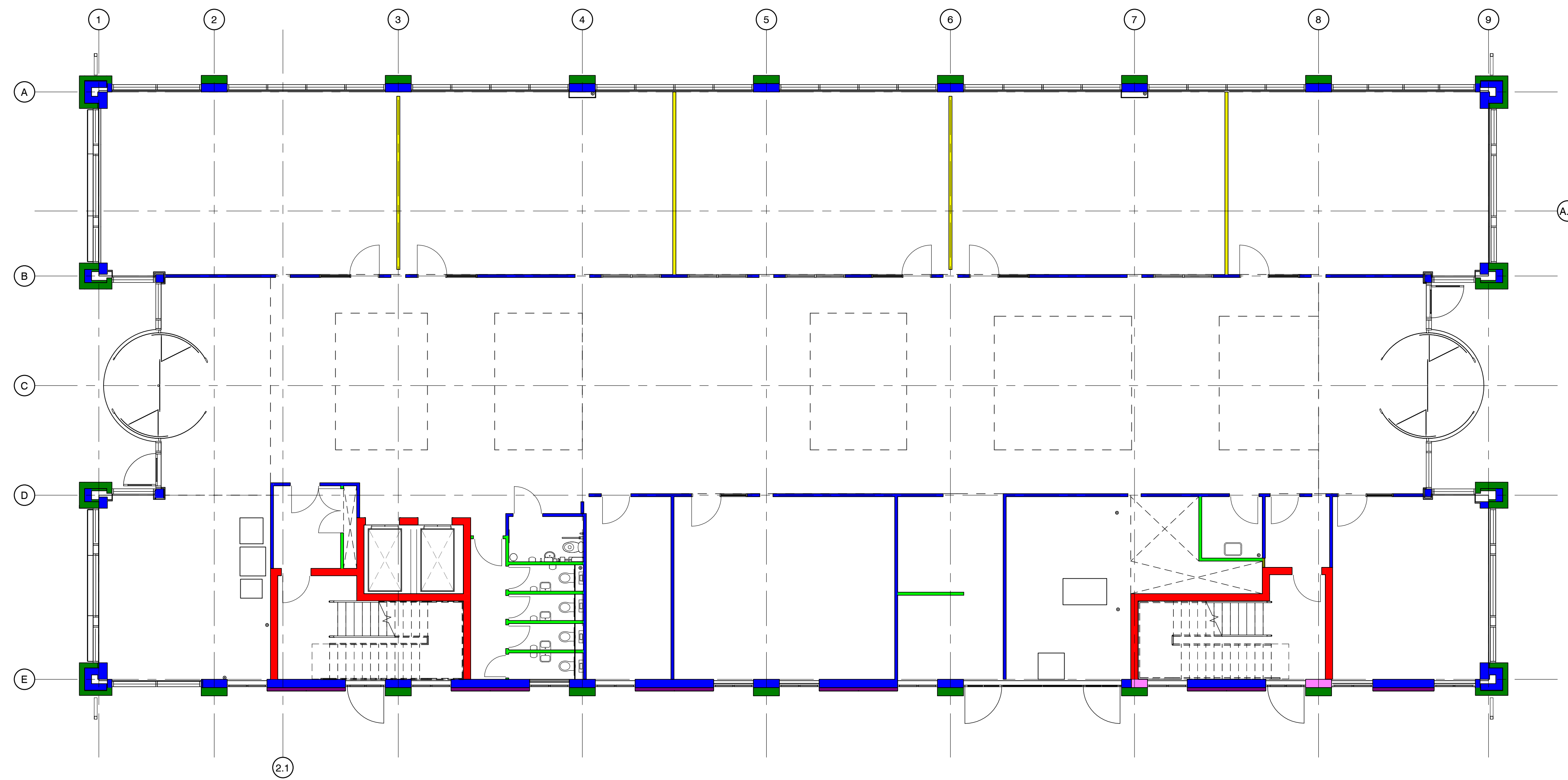
1 00 Ground Floor Level 1:100
