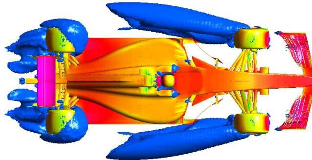
Figure 49 - Full Car Geometry Testing 2018 Spec Turbulent Kinetic Energy
