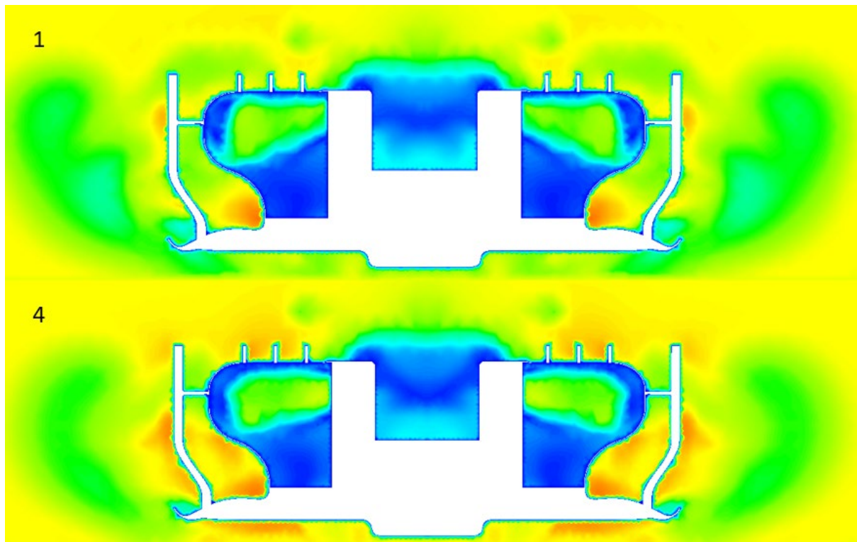
Figure 46 - Full Car Geometry Testing Velocity Cut Plane Designs 1 & 4
