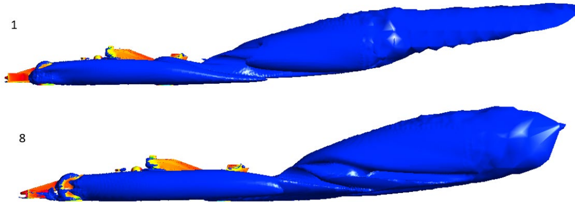
Figure 54 - Isosurface showing wake region designs 1 & 8 Side View
