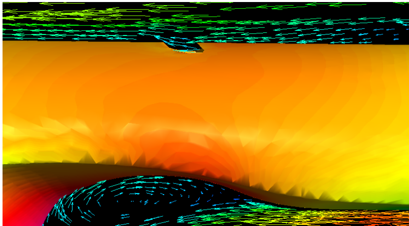
Figure 23 - Slot Gap Testing Flow Vectors Forward Opening
