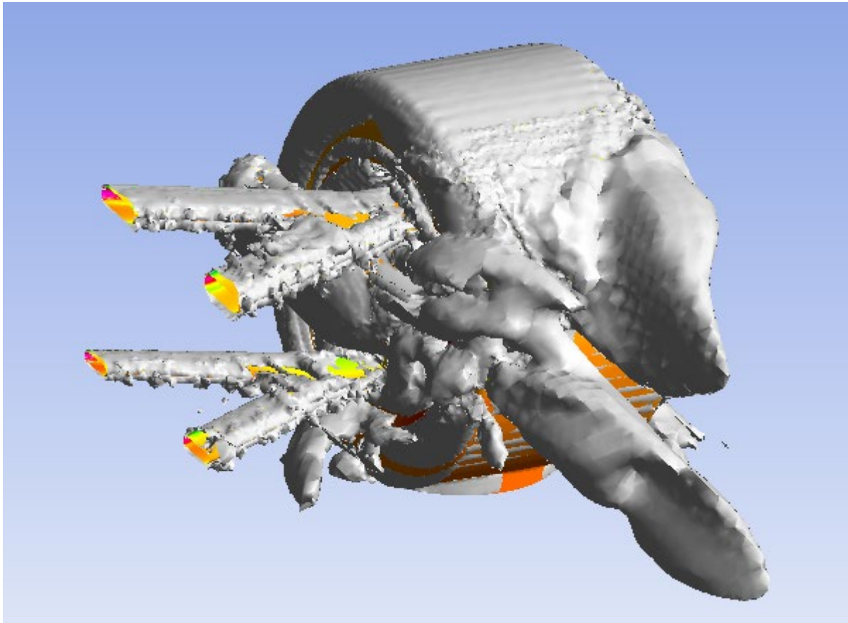
Figure 15 - Vorticity Regions Original Geometry
