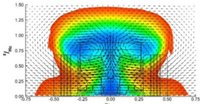
Figure 56 - F1 Car Wake Representation (Newbon, et al., 2017)
