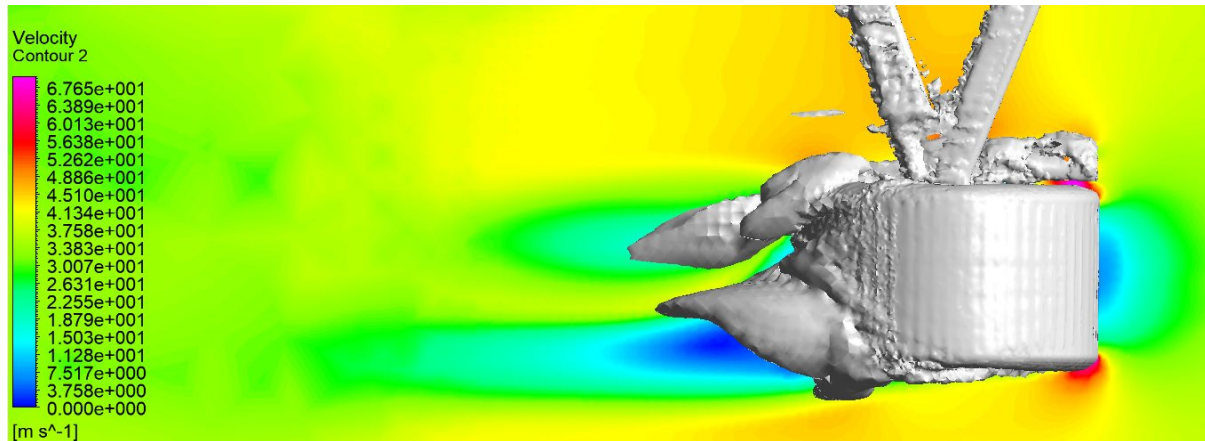
Figure 16 - Brake Duct Initial Run Velocity Profile
