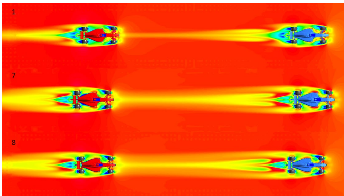
Figure 63 - Following Car Testing Velocity Contours
