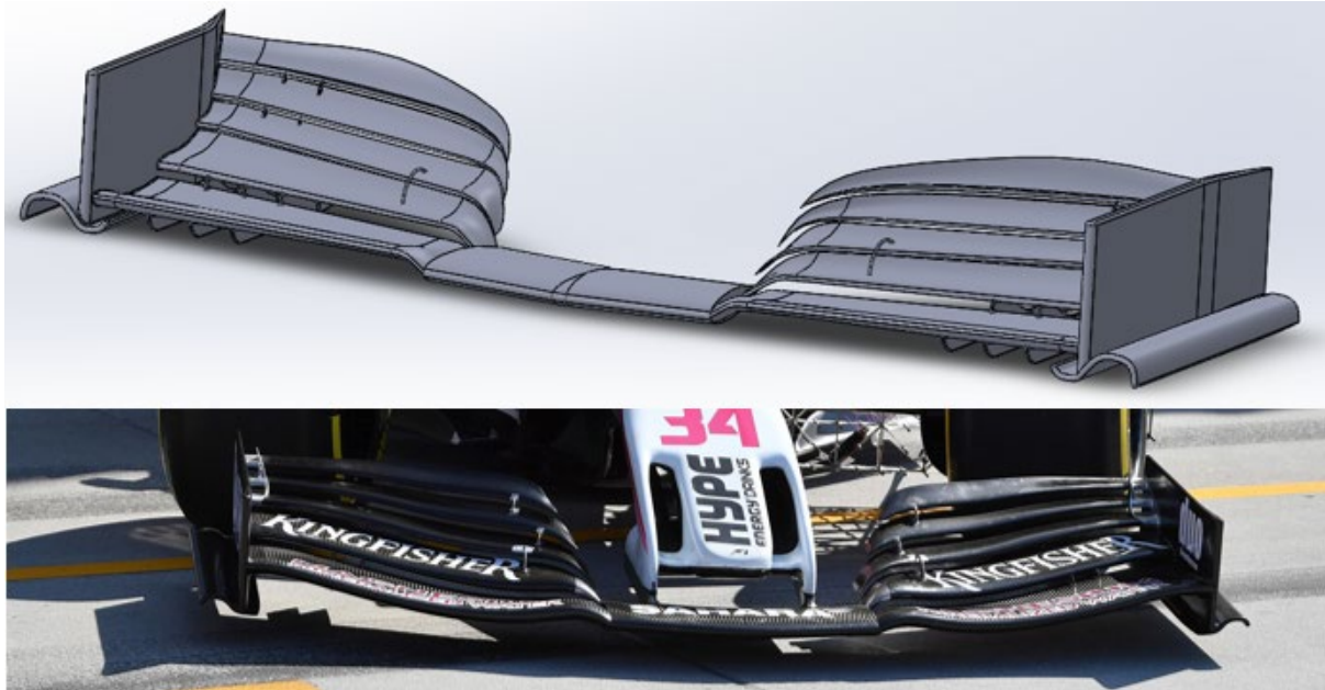
Figure 32 - 2019 Wing Geometry Comparison (FIA Formula 1, 2018)
