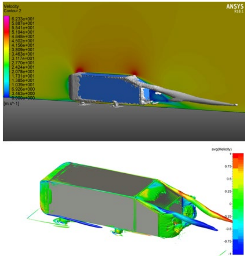
Figure 10 - Ahmed Body Vortex Comparison (Guilmineau, et al., 2017)
