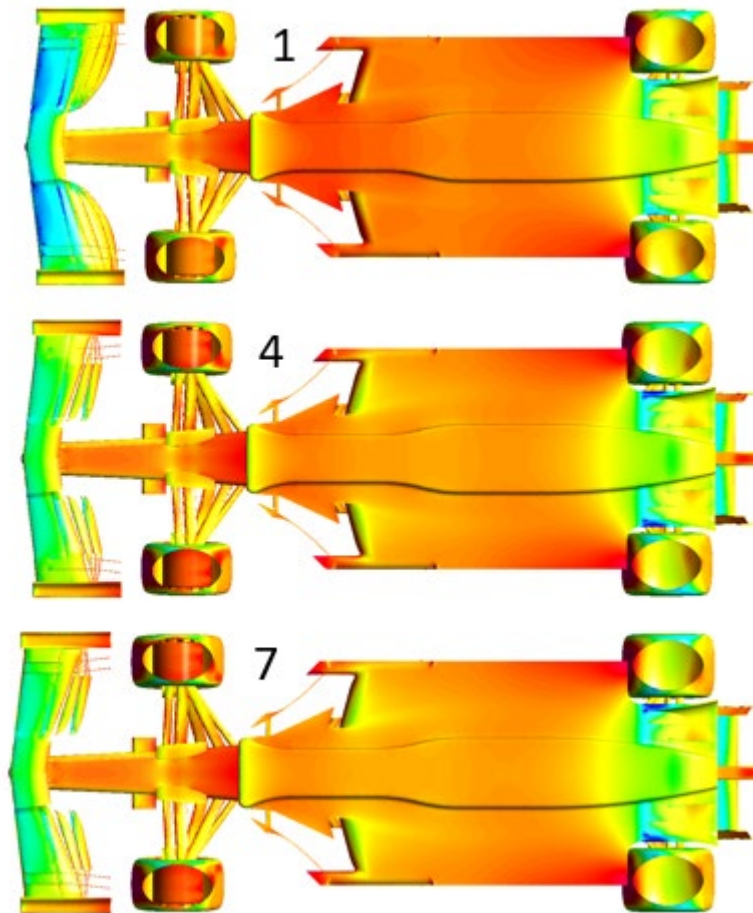
Figure 45 - Full Car Geometry Testing Designs 1,4 & 7 Underside Pressures
