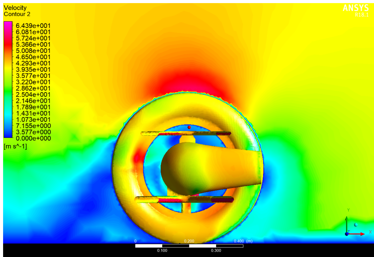
Figure 14 - Brake Duct Initial Run Velocity Contours
