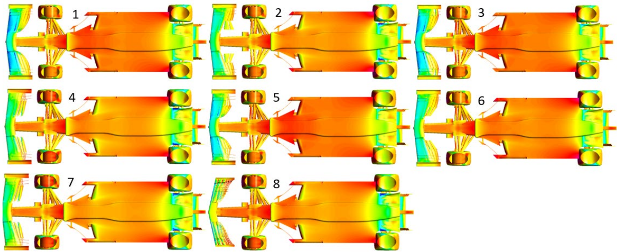
Figure 44 - Full Car Geometry Testing Underside Pressure Distributions
