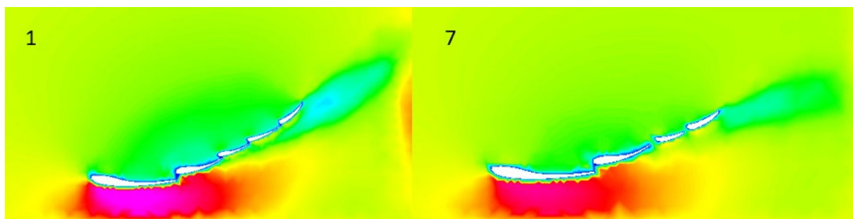
Figure 47 - Front Wing Upwash Characteristics
