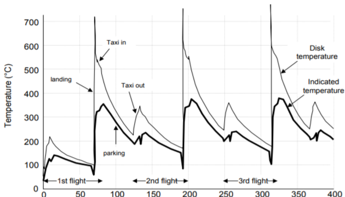
Figure 3 - Carbon Braking System Temperature Management (Airbus, 2014)
