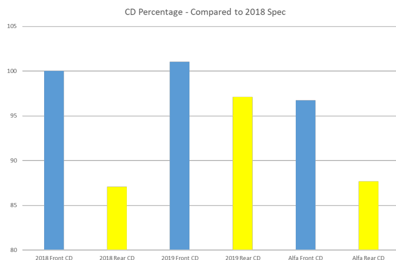
Figure 62 - Following Car Testing Cd Percentage Values
