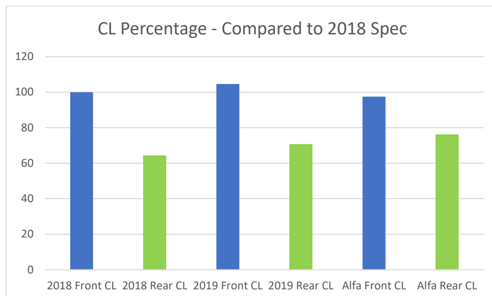
Figure 64 - Following Car Cl Results 0.35s Separation
