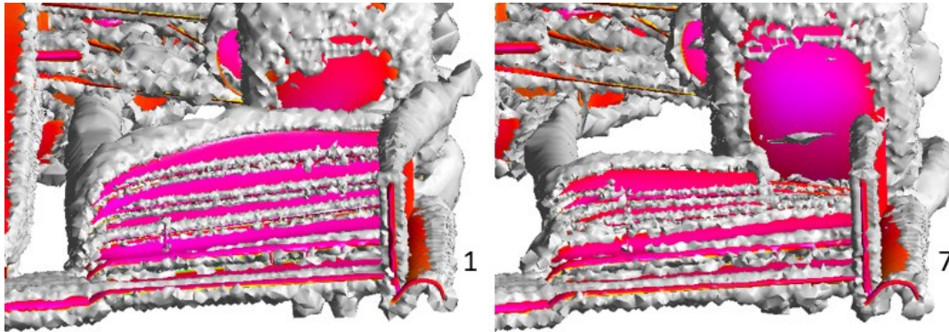
Figure 52 - Y250 Vortex Designs 1 and 7
