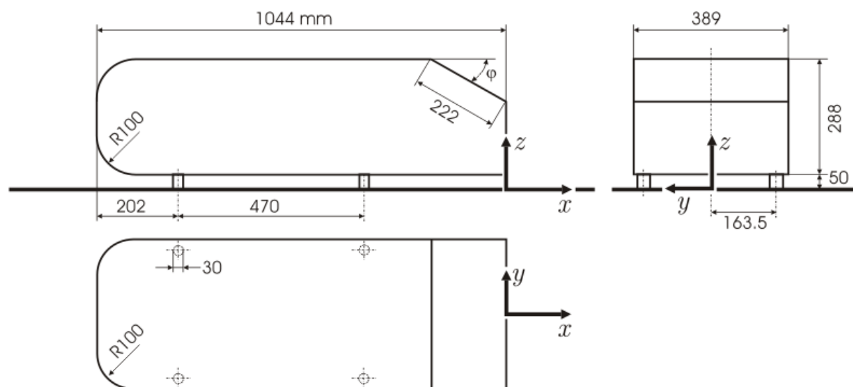
Figure 4 - Ahmed Body Dimensions (CFD Online, 2014)
