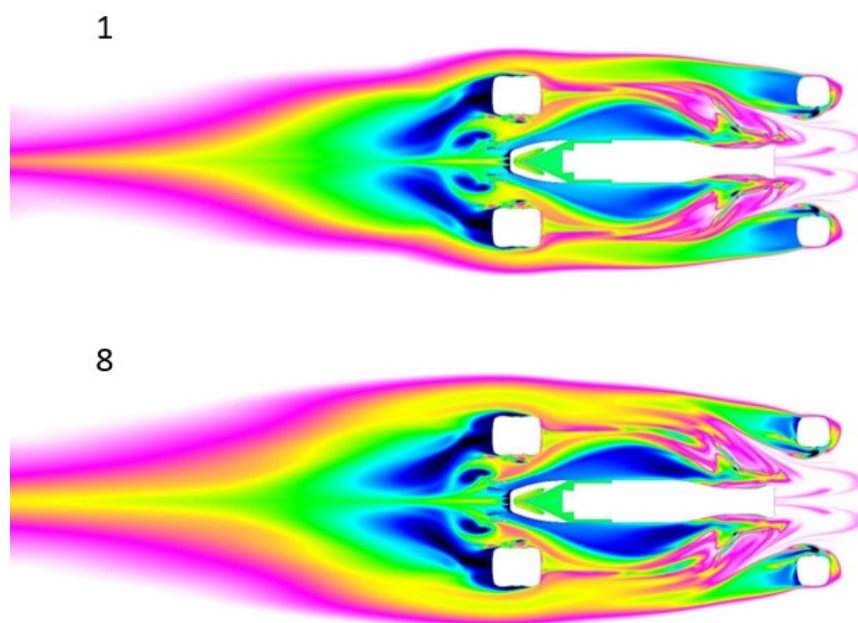
Figure 58 - F1 2018 2019 Wake Comparison (Iley Design, 2019)
