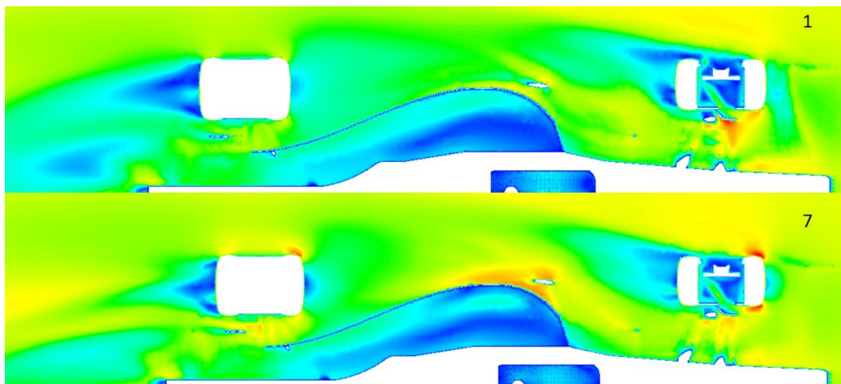
Figure 50 - Velocity Contours Section View 0.35m above Ground Plane
