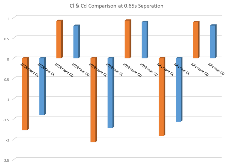
Figure 60 - Cl and Cd results from 5 Car Length Separation Testing
