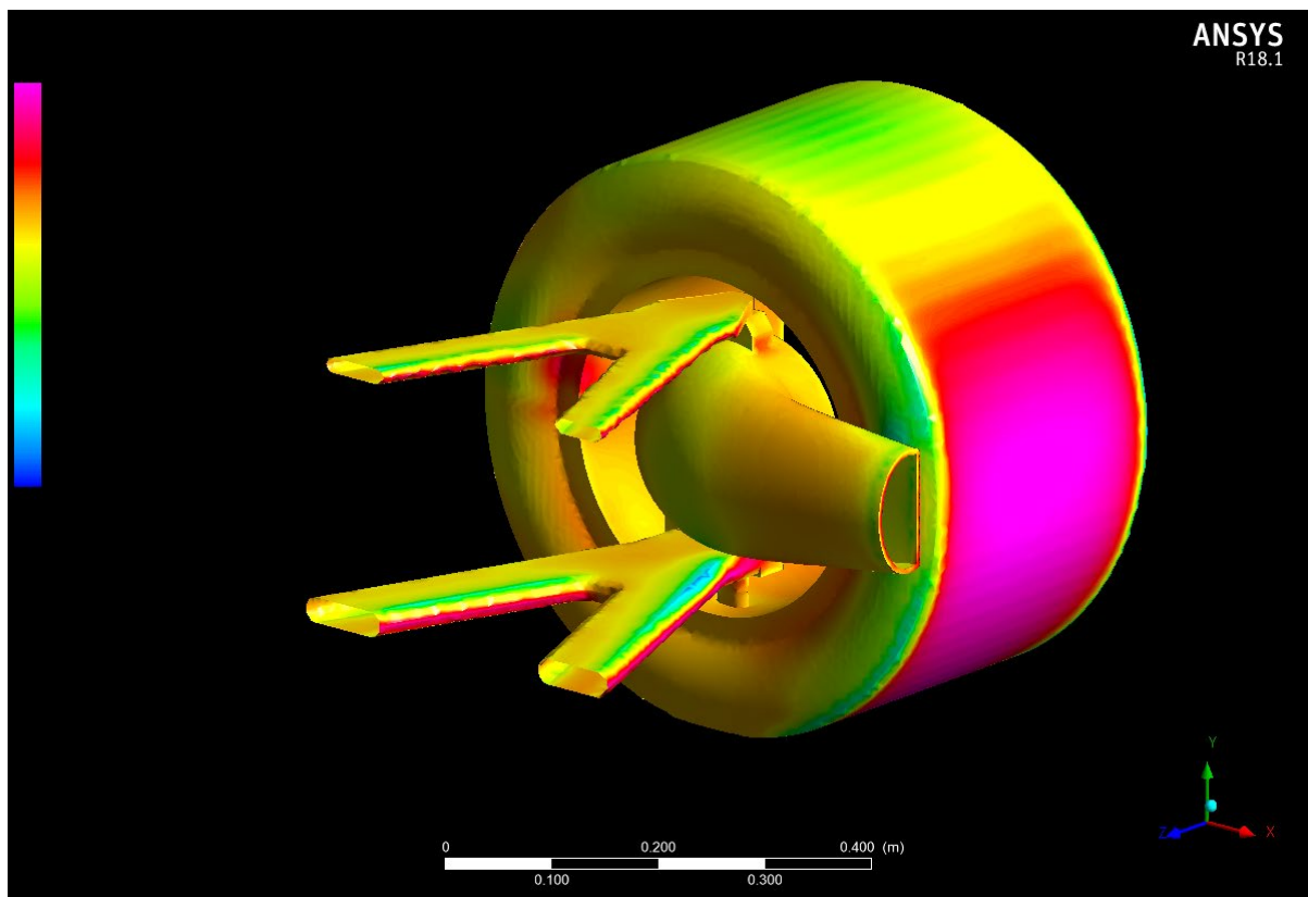
Figure 13 - Brake Duct Initial Run Pressure Distribution
