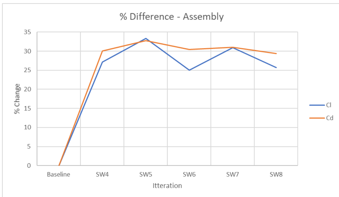
Figure 18 - Slot Gap Testing Assembly C_i C_d Results
