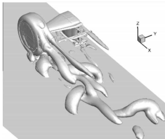
Figure 2 - Turbulent Wheel Wake (Croner, et al., 2013)
