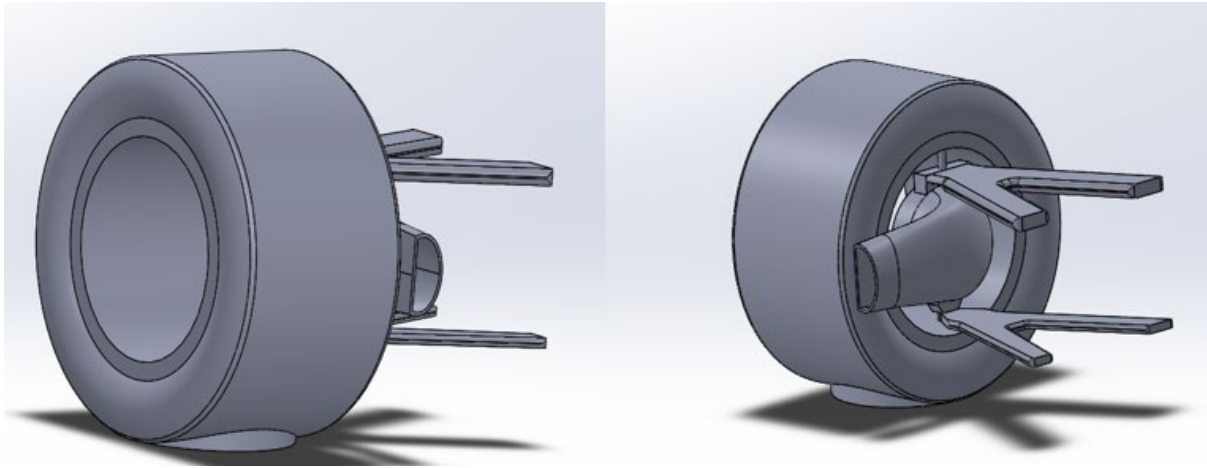
Figure 12 - Simplistic Brake Duct Testing Geometry
