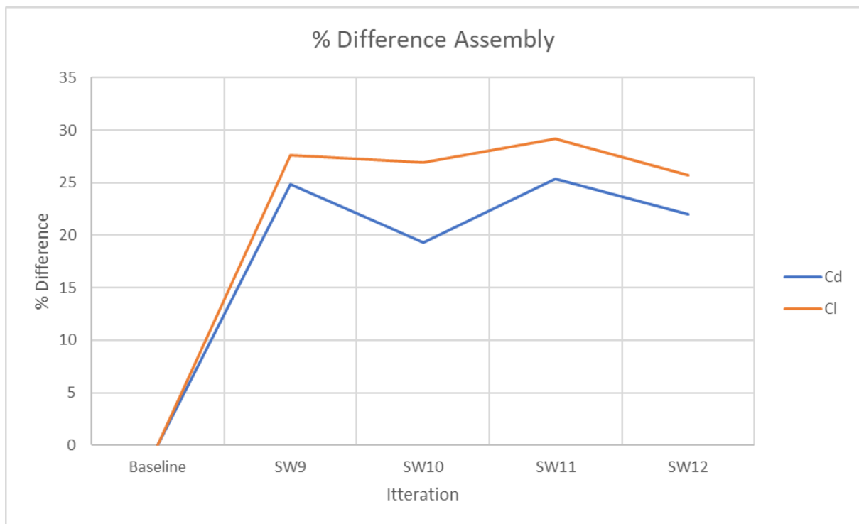
Figure 24 - Duct Opening Size Results on Assembly
