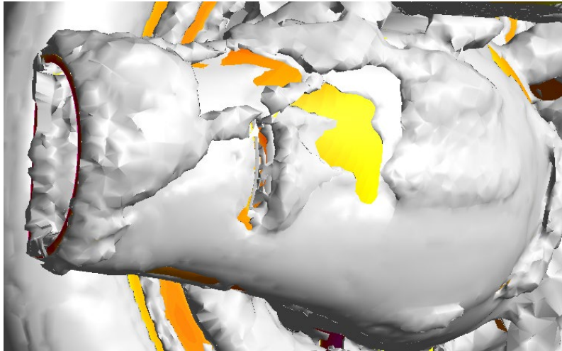
Figure 22 - Slot Gap Testing Turbulent Flow around Duct
