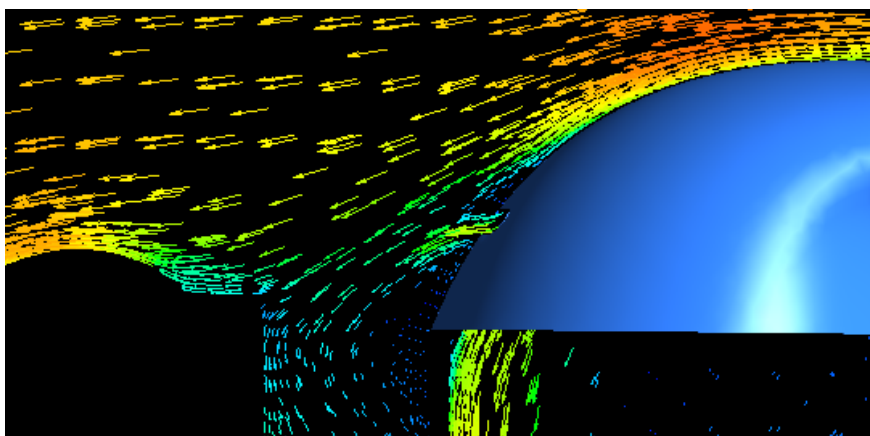
Figure 20 - Slot Gap Testing Flow Vectors
