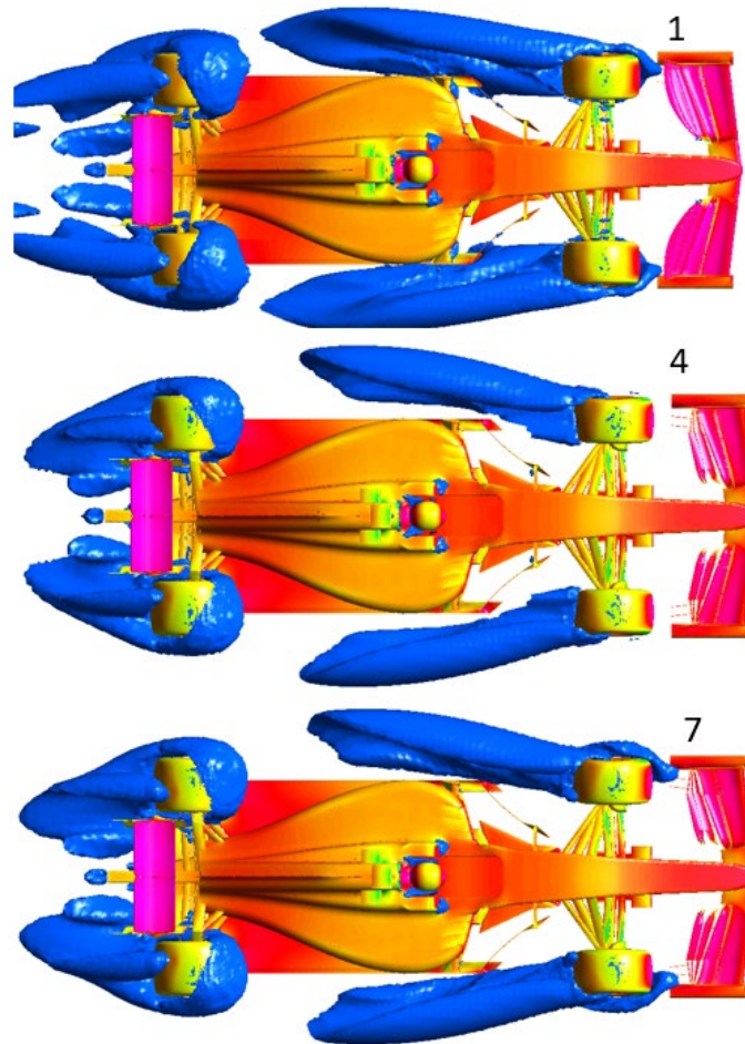
Figure 48 - Full Car Geometry Testing Turbulent Kinetic Energy Isosurface
