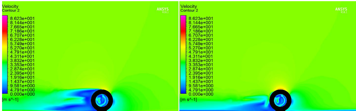
Figure 29 - Rotating Wheel Wake Comparison Velocity Contours
