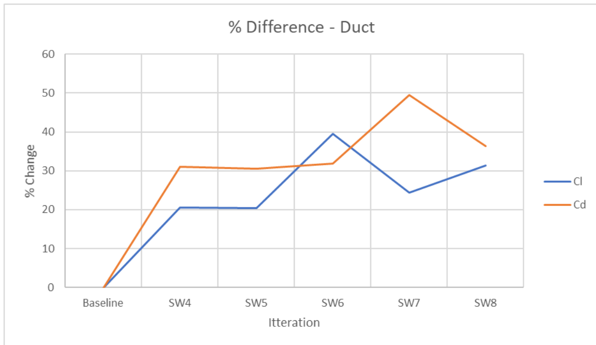
Figure 19 - Slot Gap Testing Duct Cl Cd Results
