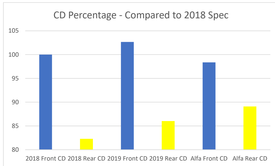
Figure 65 - Following Car Cd Results 0.35s Separation
