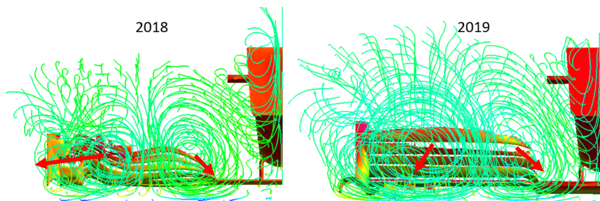
Figure 36 - Wing in Isolation Streamlines Rear View
