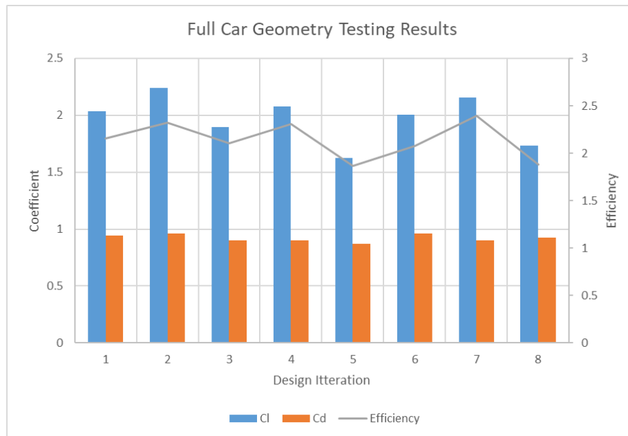
Figure 42 - Full Car Geometry Testing Results
