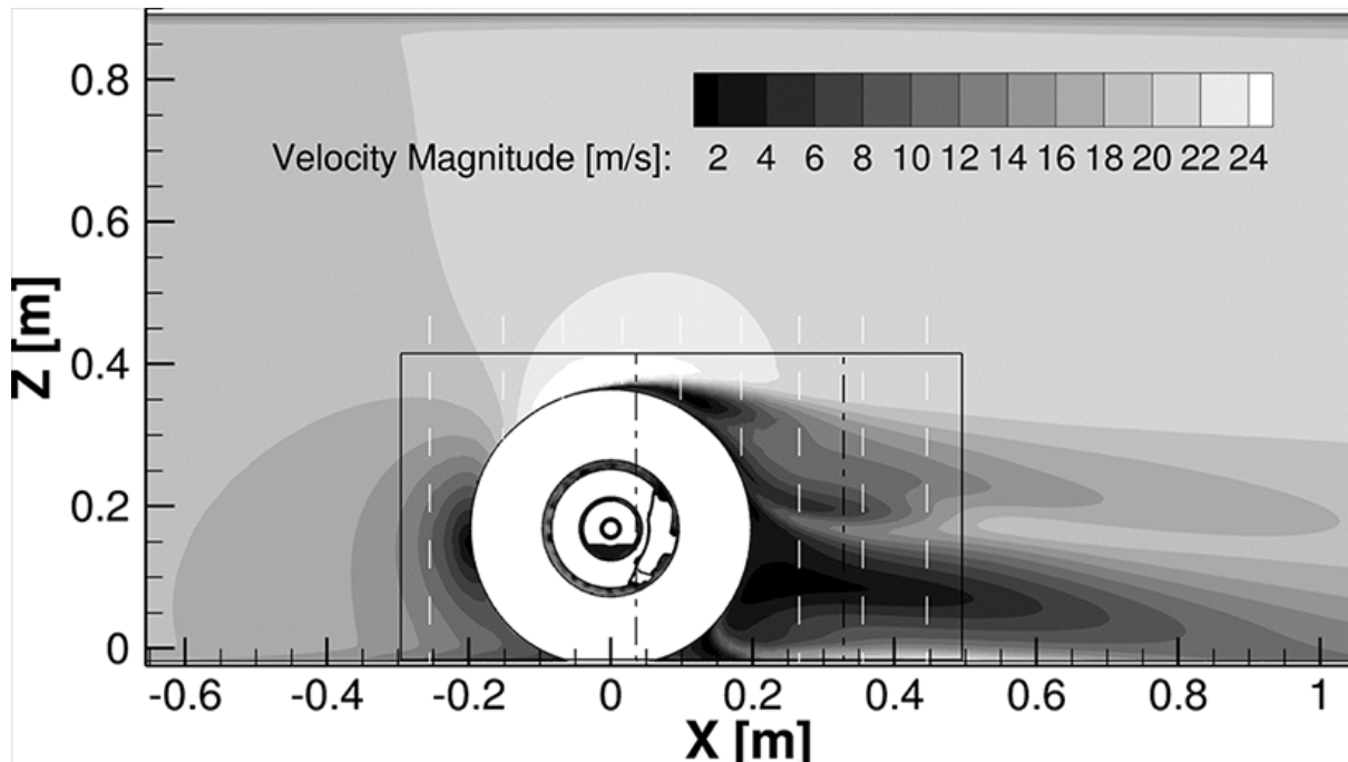
Figure 30 - Rotating F1 Wheel Wake Example (Axereo-Cilies & Iaccarino, 2012)
