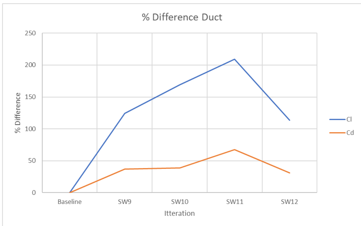
Figure 26 - Duct Opening Size Results on Duct
