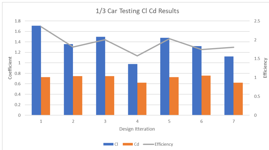
Figure 38 - 1/3 Car Testing Results
