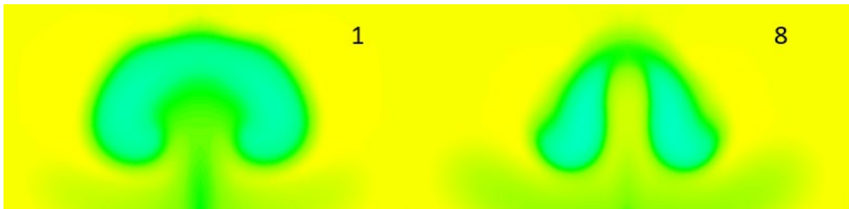
Figure 53 - Vehicle Wake 2.5m behind car designs 1 & 8
