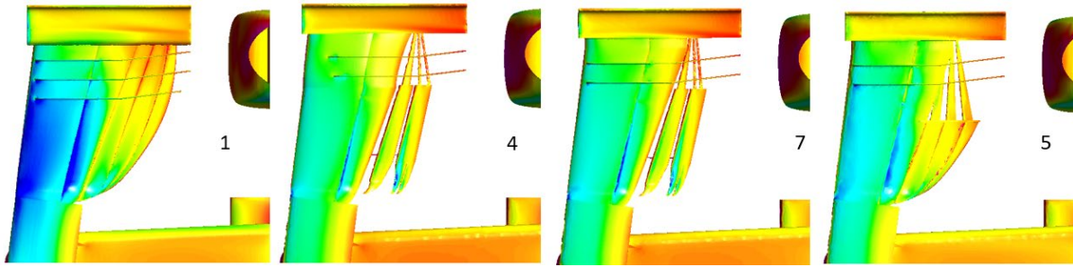
Figure 41 - Pressures on Wing Undersides Designs 1,4,5,7
