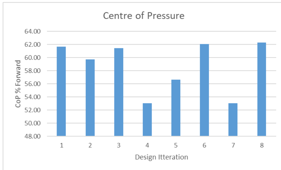
Figure 43 - Full Car Geometry Testing Centre of Pressure Results
