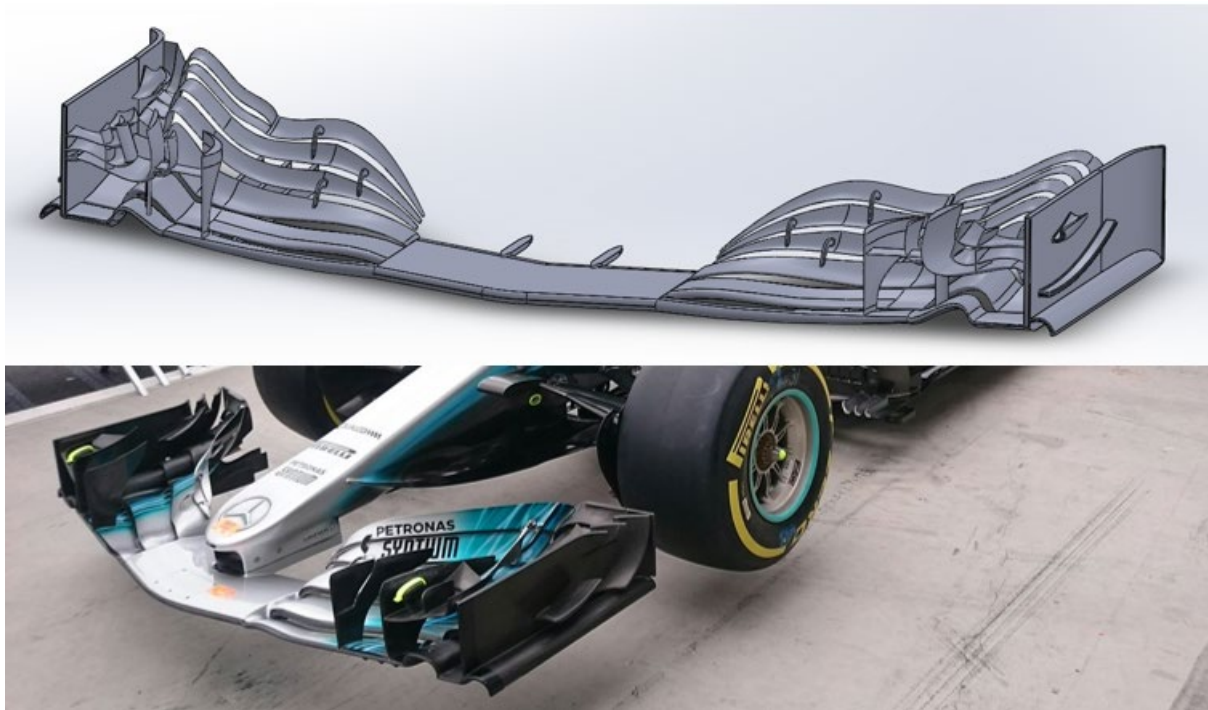
Figure 31 - F1 2018 Wing Geometry (F1Technical.net, 2018)
