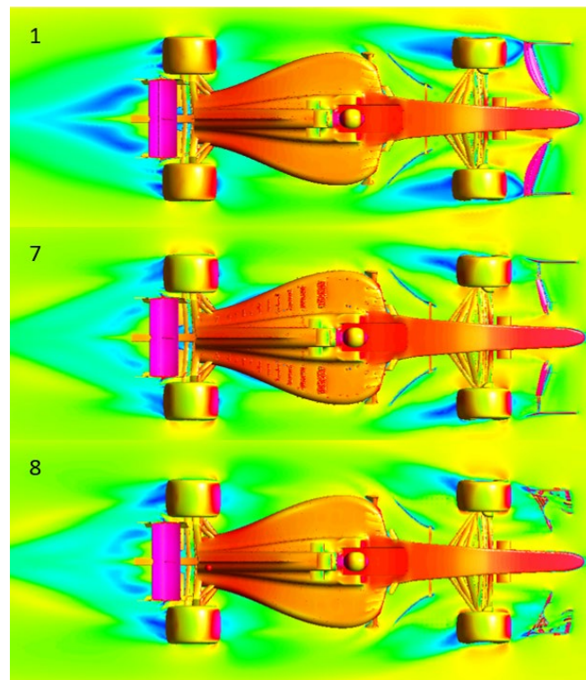
Figure 57 - Vehicle Wake Differences Plane 0.25m above ground
