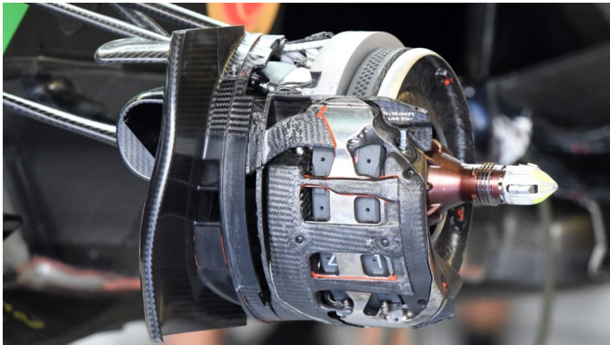
Figure 51 - Force India 2018 Front Brake Assembly (FIA Formula 1, 2018)
