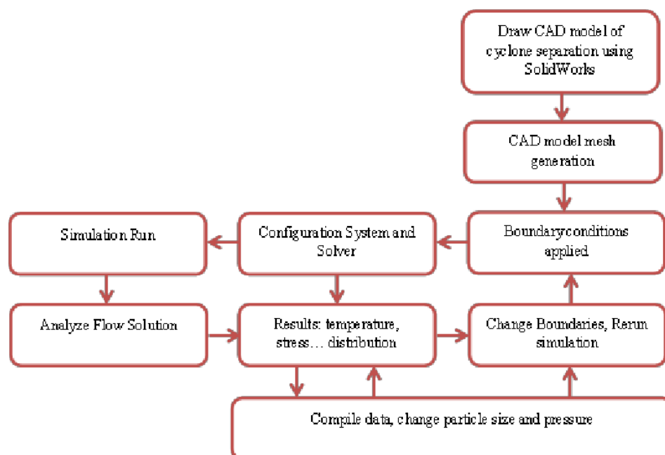
Figure 6 - CFD Workflow (Alahmer & Al-Dabbas, 2014)
