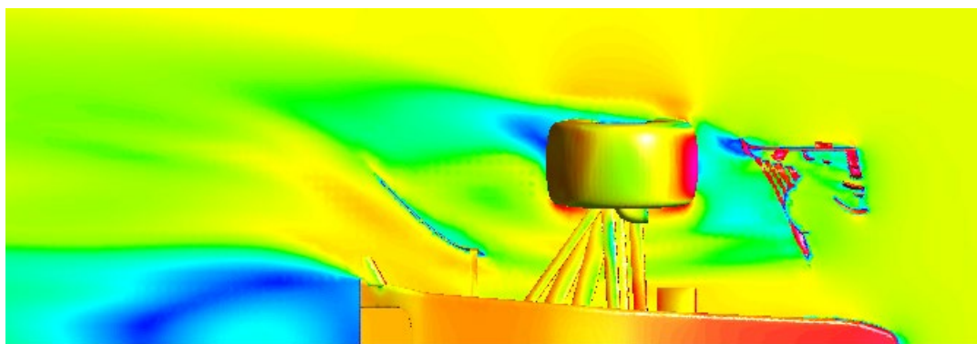
Figure 39 - 2018 Spec Velocity Cut Plane 0.2m from ground
