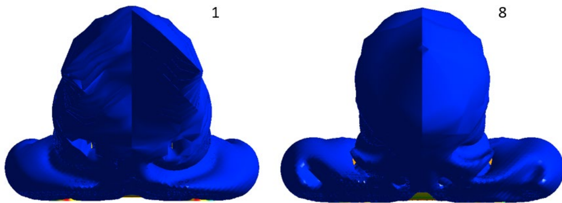
Figure 55 - Isosurface showing wake region designs 1 & 8 Rear view
