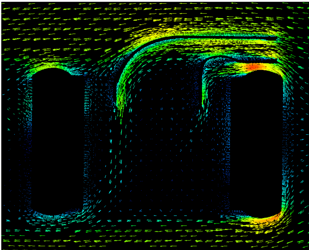
Figure 28 - Flow Vectors showing influence of duct flow
