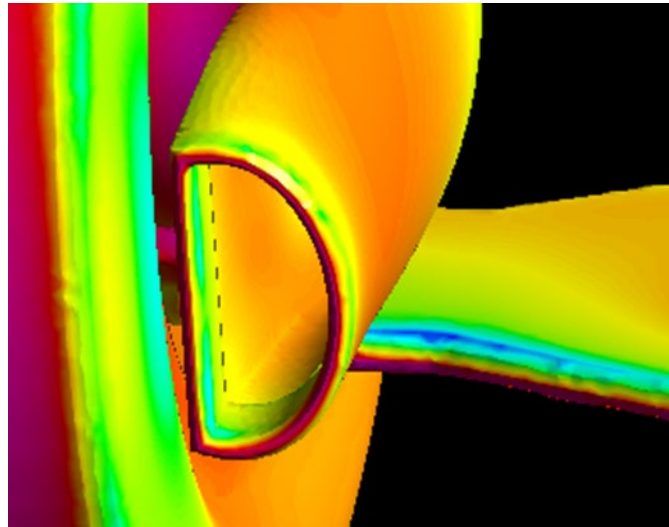
Figure 27 - Brake Duct Opening Tests Pressure Contours
