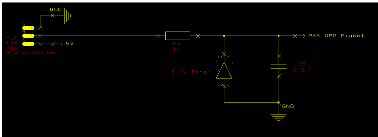
Figure 19 - Schematic of GPS Connection to Microcontroller
