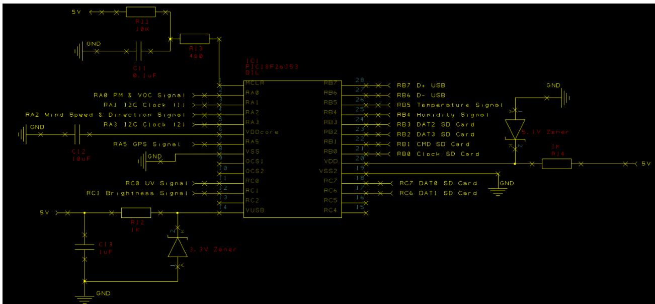
Figure 17 - Schematic of Microcontroller Connections
