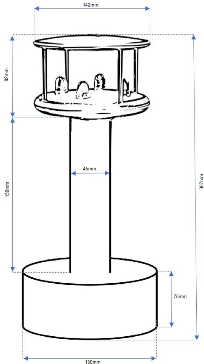
Figure 27 - Basic Design Concept
