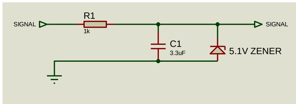
Figure 16 – 50Hz LPF with 5V Overvoltage Protection
