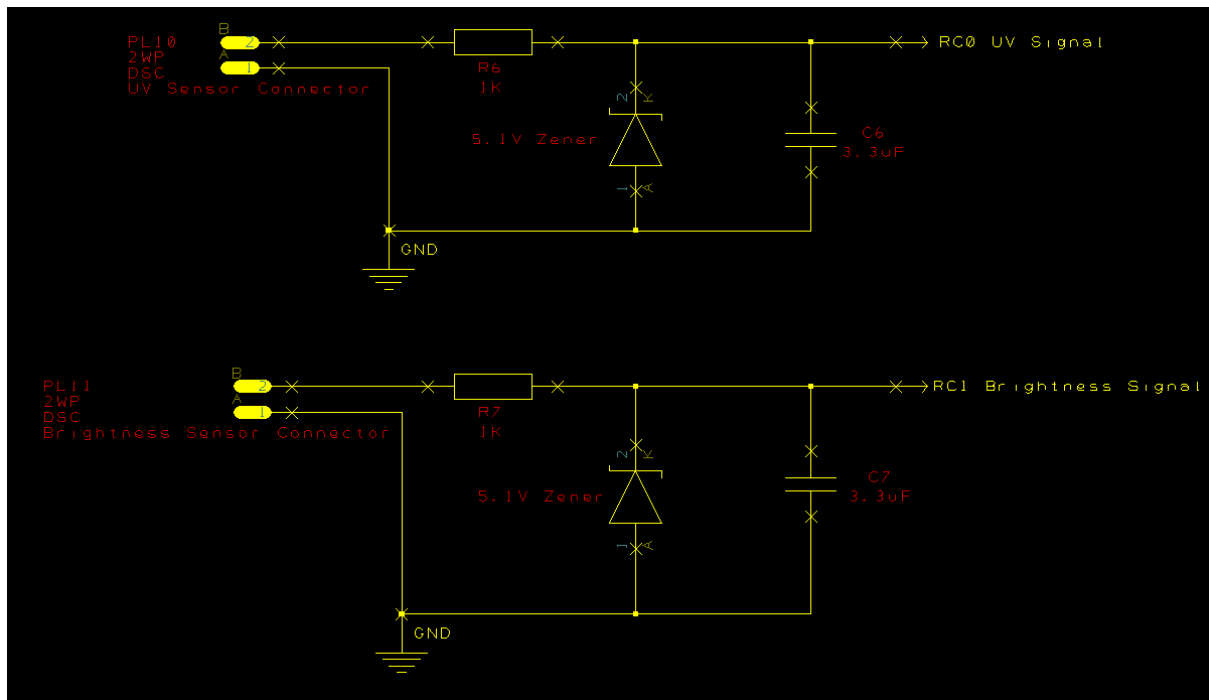
Figure 20 - Schematic of UC and Brightness Sensor Connections
