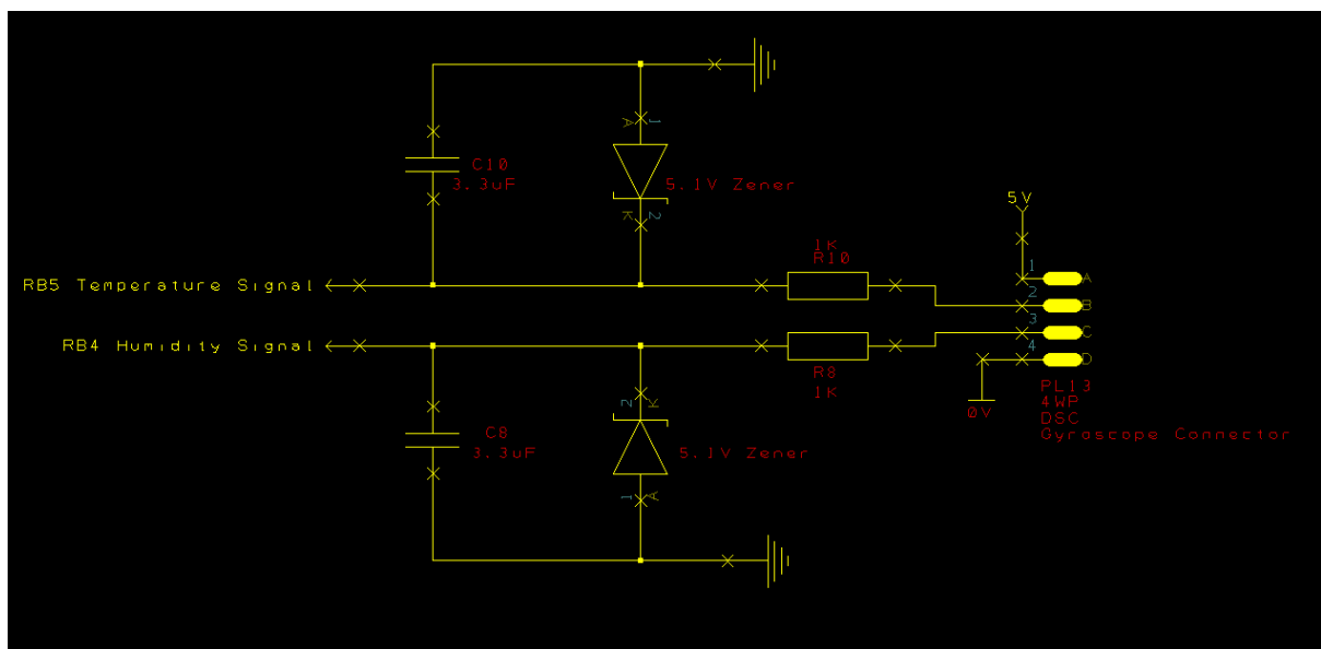
Figure 21 - Schematic of Temperature & Humidity Sensor Connections
