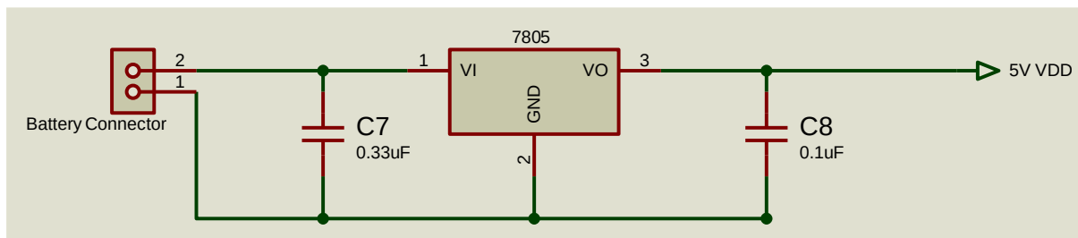
Figure 15 - 7805 Voltage Regulator Configuration
