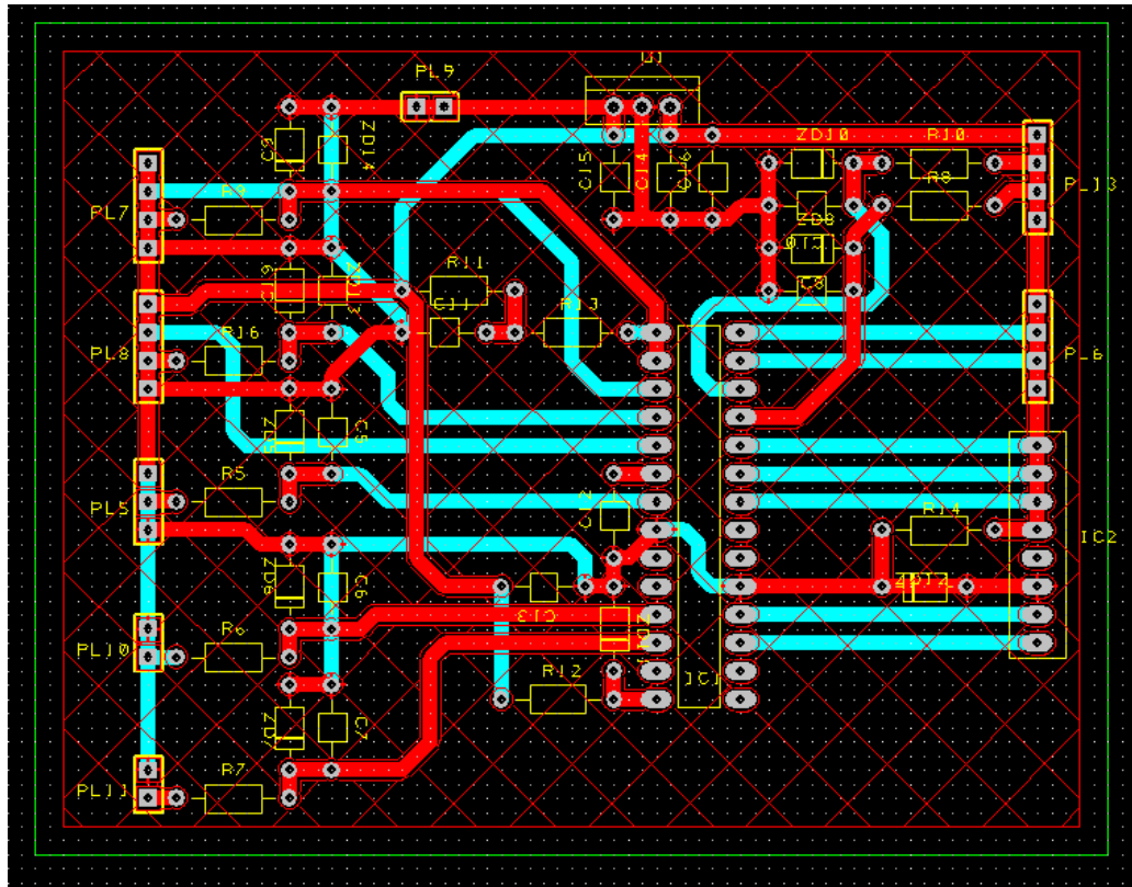
Figure 24 – Project PCB Design
