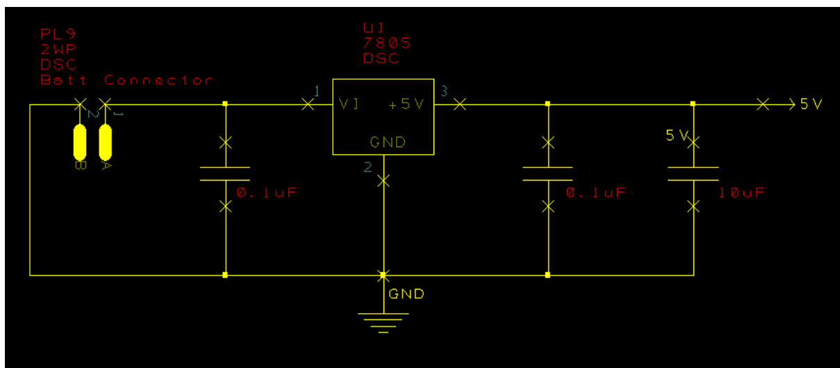
Figure 23 - Schematic of 7805 Voltage Regulator Connections
