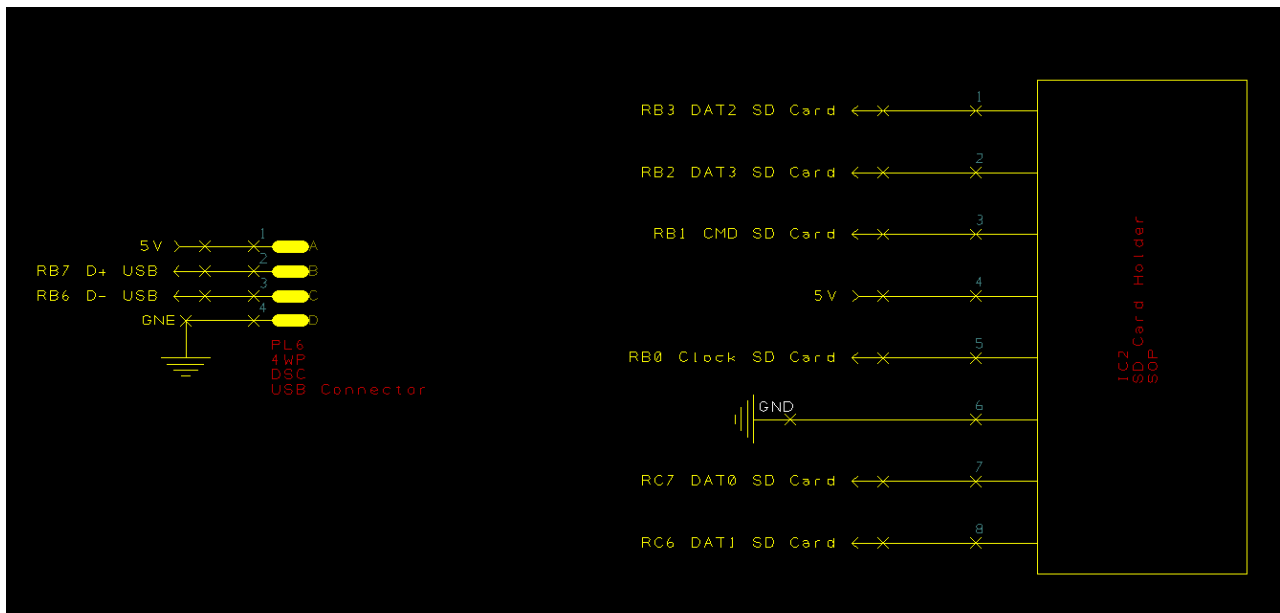
Figure 22 - Schematic of USB and SD Card Holder Connections
