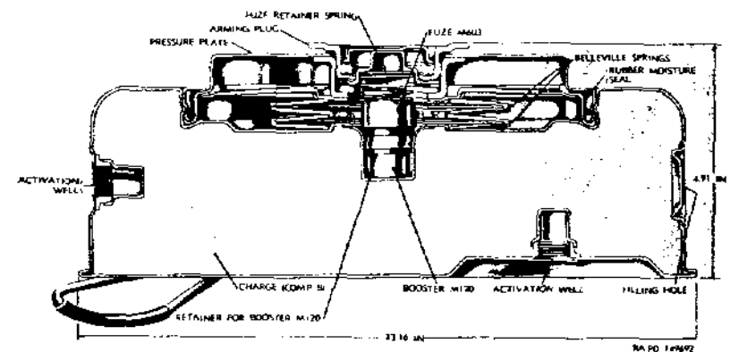
Figure 64. Antitank Mine (M15)
