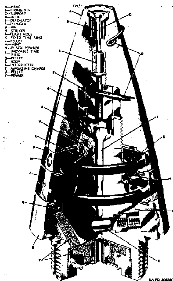
Figure 44. Fuze M54
