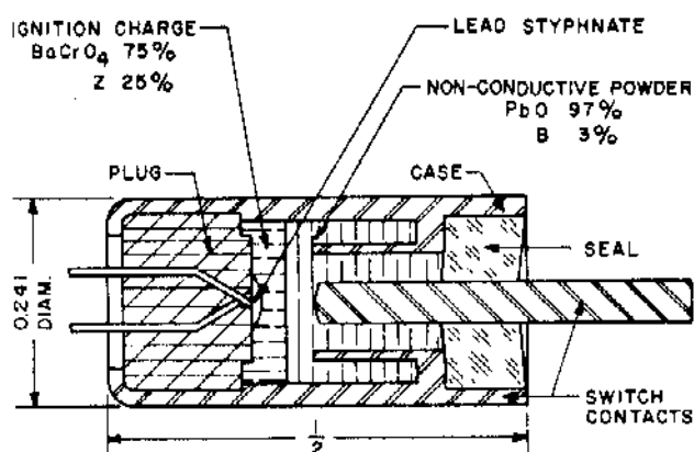
Figure 71. Pyroswitch
