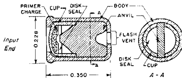
PERCUSSION PRIMER (M39A1)
