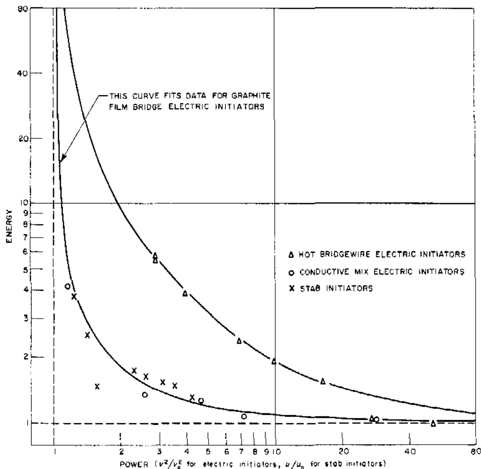
Figure 5. Energy-Power Relationship for Various Initiators
