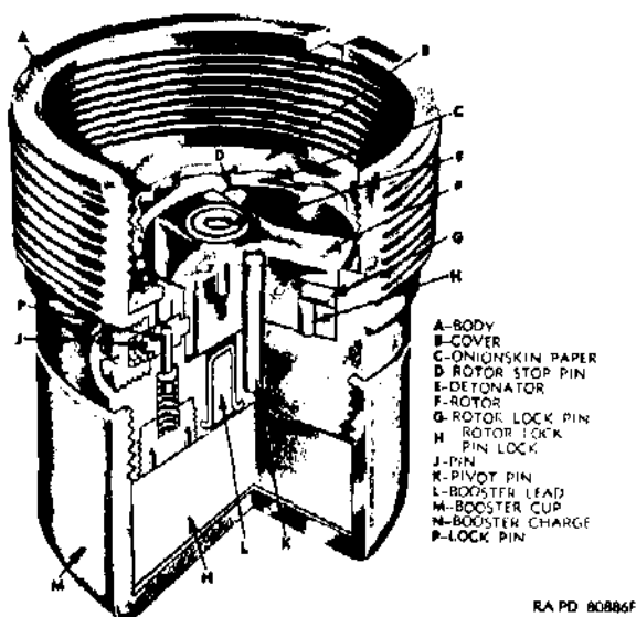
Figure 49. Booster (M21A4)
