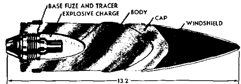
Figure 62. Armor Piercing Projectile
