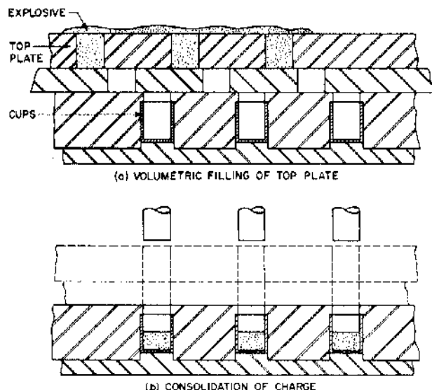
Figure 76. Charging Plate Loading
