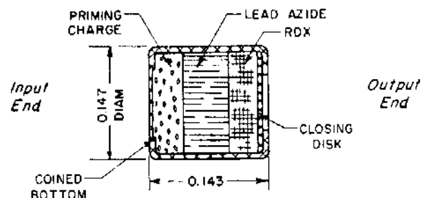
STAB DETONATOR (M55)
