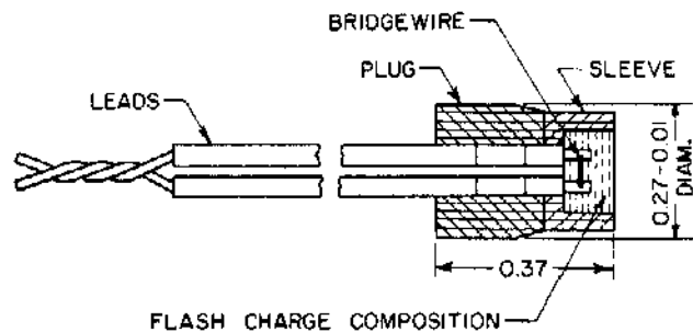
Figure 34. Electric Squib (M2)
