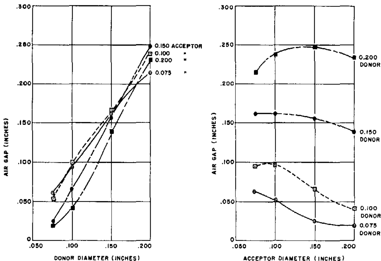
Figure 12. Critical Gap as a Function of Column Diameter
