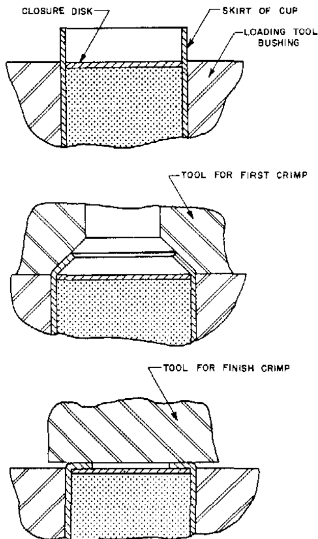
Figure 39. Initiator Cup Crimping
