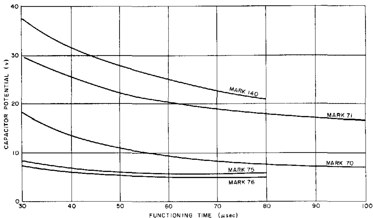
Figure 36. Functioning Times of Hot Wire Bridge Initiators
