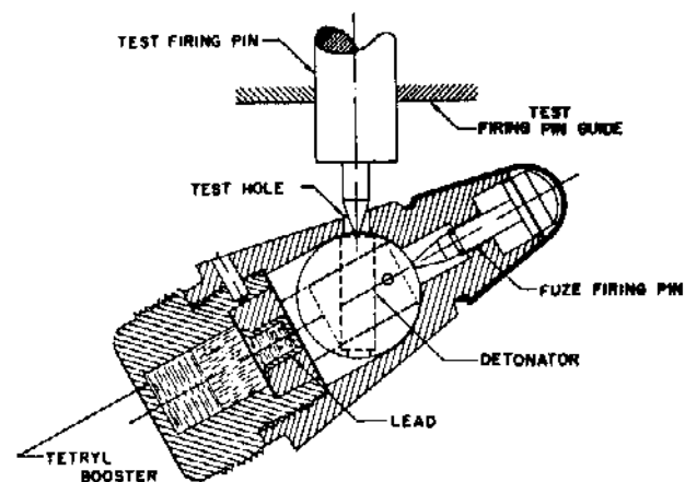
Figure 92. Arrangement for Detonator Safety Test
