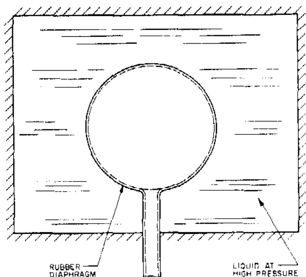
Figure 83. Isostatic Press Principle
