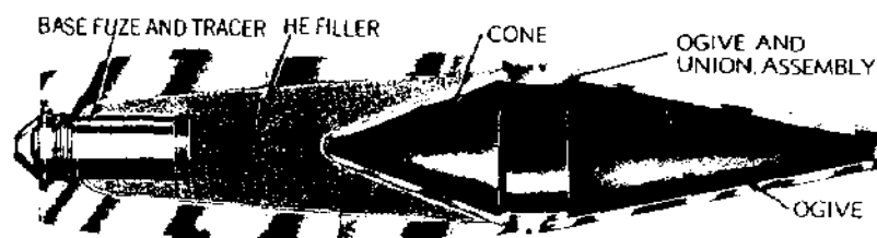
Figure 65. High Explosive Antitank Projectile
