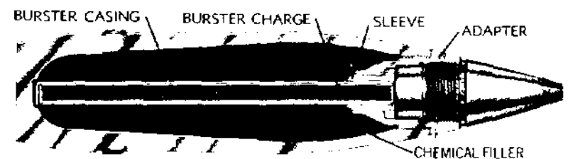
Figure 66. Burst Type Chemical Projectile
