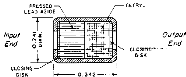
FLASH DETONATOR (M17)
