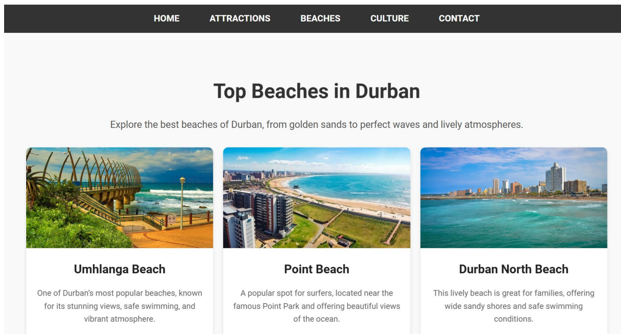
Figure 3: Beach Page
