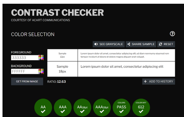
Figure 9:Contract Checker
