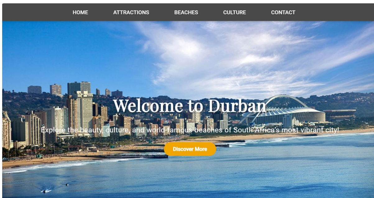
Figure 1 : Home Page
