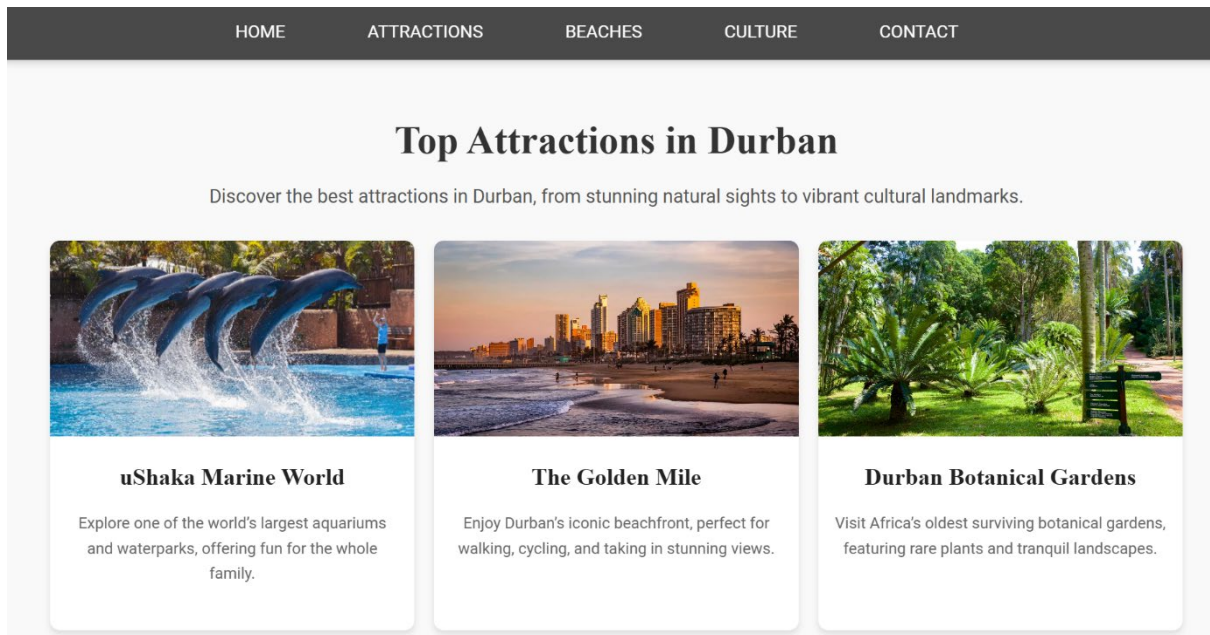
Figure 2 : Attractions Page
