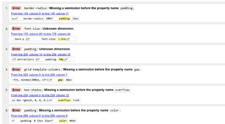
Figure 7: CSS Validation
