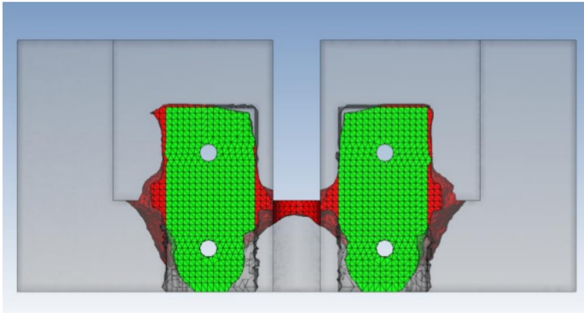
Figure 33: Optimised bracket inside original bracket, back view, (Genesis. Roberts, 2020).
