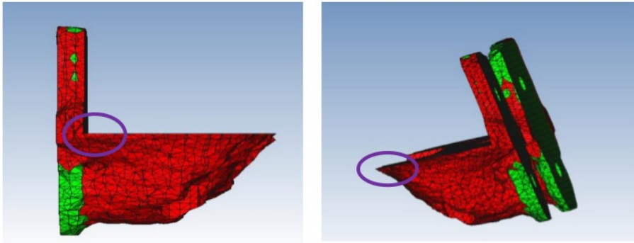
Figure 30: Side views of optimised bracket, (Genesis . Roberts, 2020).
