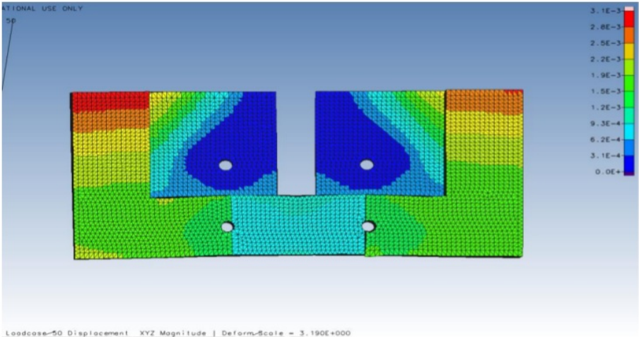
Figure 21: Bracket displacement at cycle 12, front view, (Genesis. Roberts, 2020).
