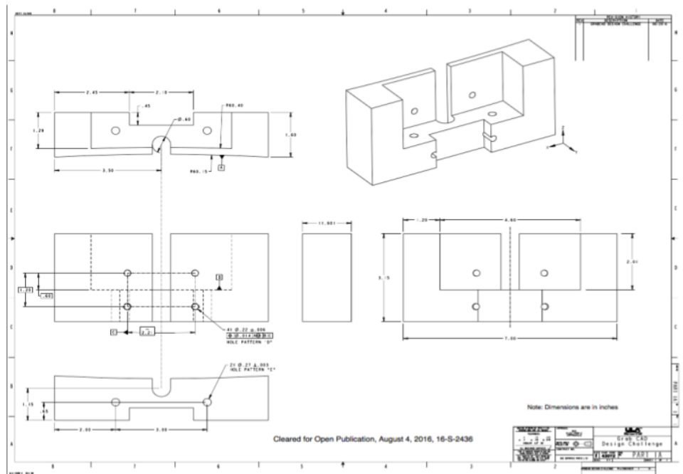
Figure 1: ULA Drawing of Boat Tail Bracket. (Alliance, 2016)
