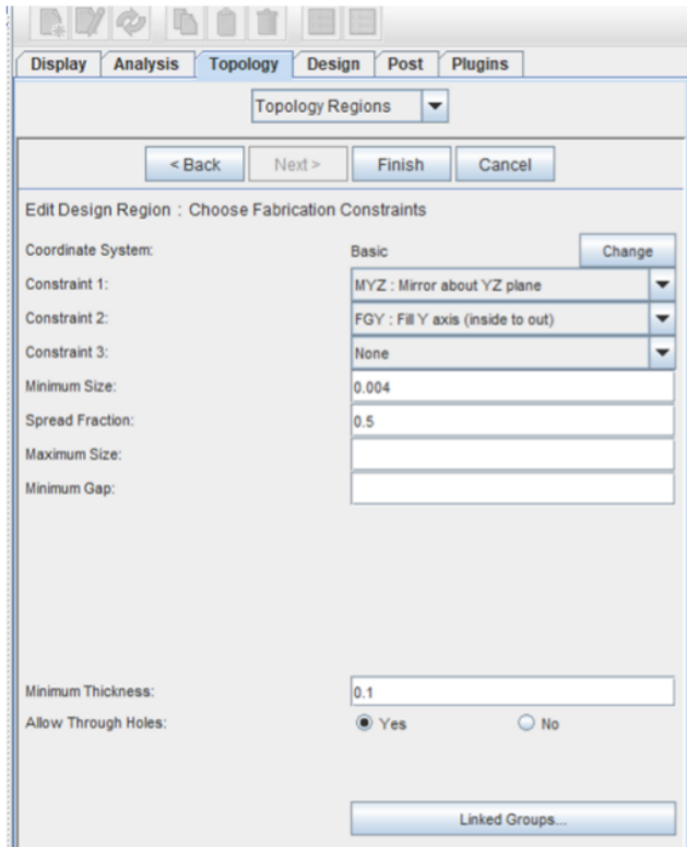
Figure 13: Setting up fabrication constraints on genesis, (Roberts, 2020).
