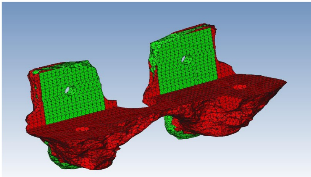
Figure 29: Angular view of optimised bracket, (Genesis. Roberts, 2020)
