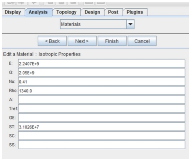
Figure 5: Converted material values inputted into genesis (Roberts, 2020).
