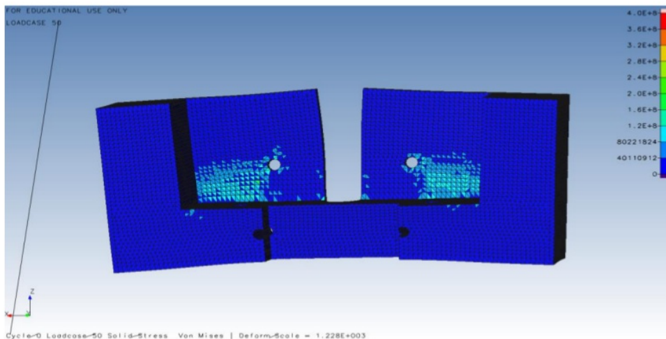
Figure 16: Bracket Stresses at cycle 0, front view, (Genesis. Roberts, 2020).
