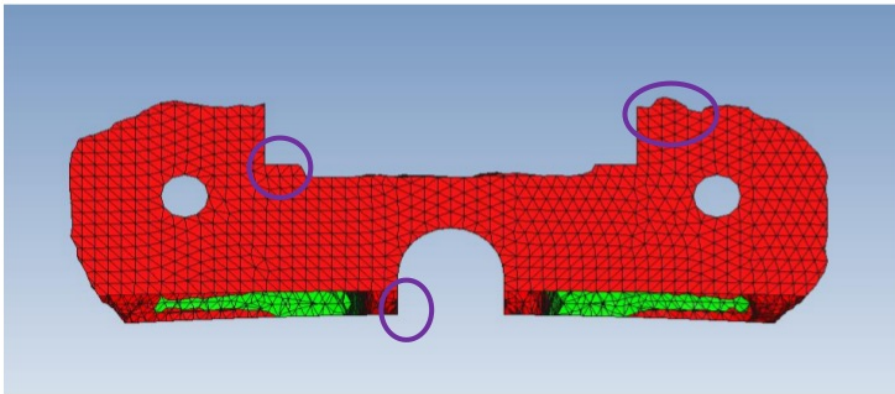
Figure 31: Top view of optimised bracket, (Genesis . Roberts, 2020) .
