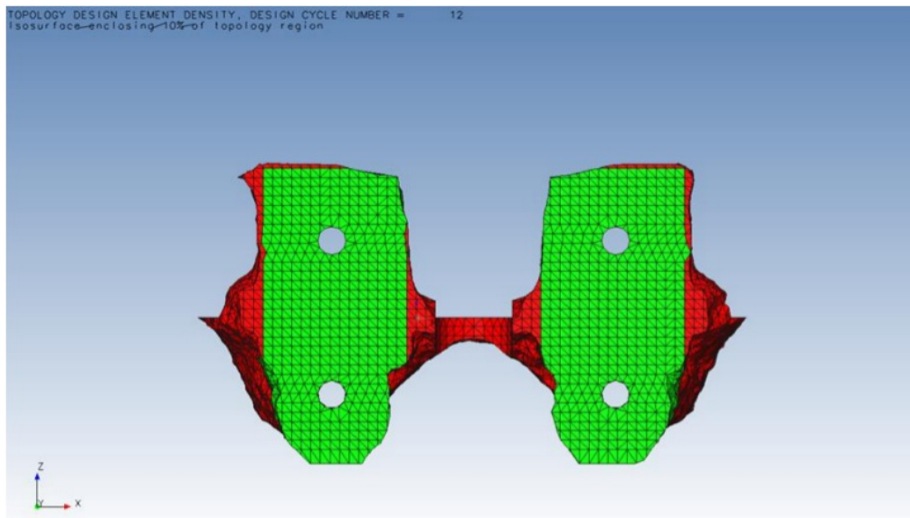
Figure 28: Back view of optimised bracket, (Genesis. Roberts, 2020).
