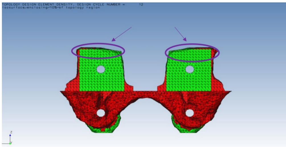
Figure 27: Front view of optimised bracket, (Genesis. Roberts, 2020).
