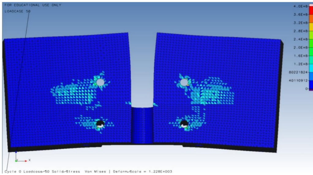
Figure 17: Bracket stresses at cycle 0, back view, (Genesis.Roberts, 2020).
