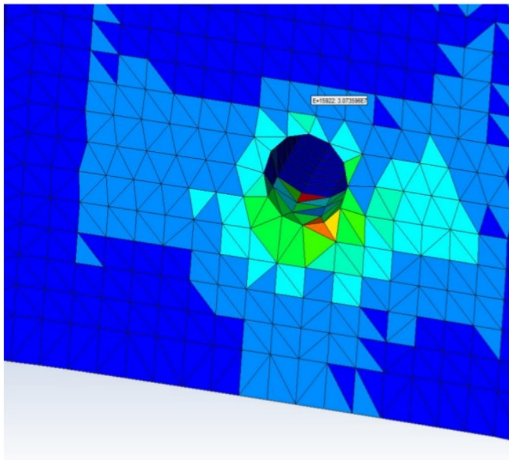
Figure 18: Stressed Elements in bolt holes, (Genesis.Roberts, 2020)
