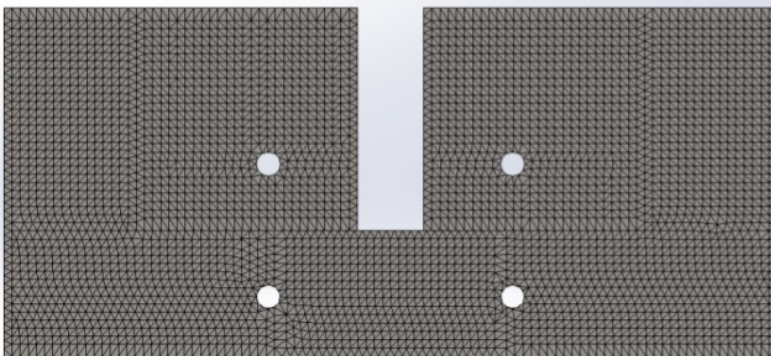
Figure 4: The boat tail bracket which was modelled and meshed in solid works, (Roberts, 2019).
