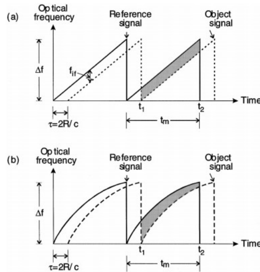
Figure 21 - Instantaneous optical frequencies vs time of object & reference mirror signal (a) linear optical frequency ramp (b) nonlinear optical frequency ramp (11)
