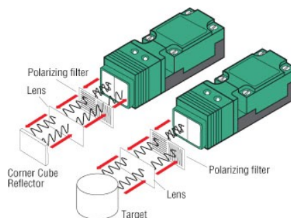
Figure 13 - operation of a retroreflective photocell (9)
