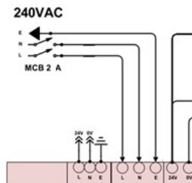
Figure 52 - Supply voltage circuit design
