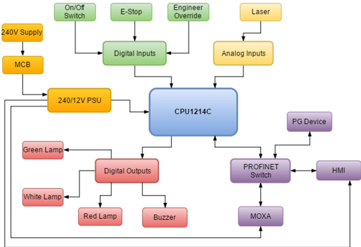
Figure 54 - Block circuit diagram
