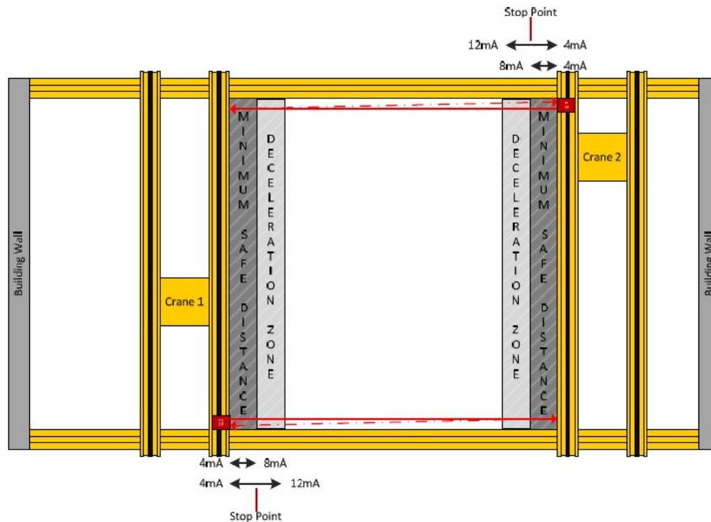
Figure 103 - Crane Speed Control (27)
