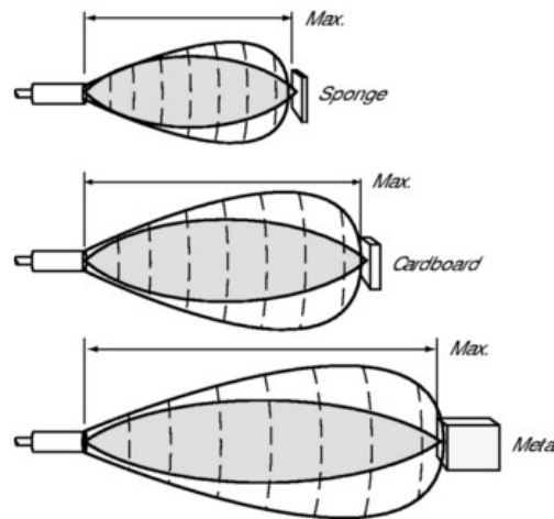
Figure 8- Sensing range with maximum sensitivity (8)
