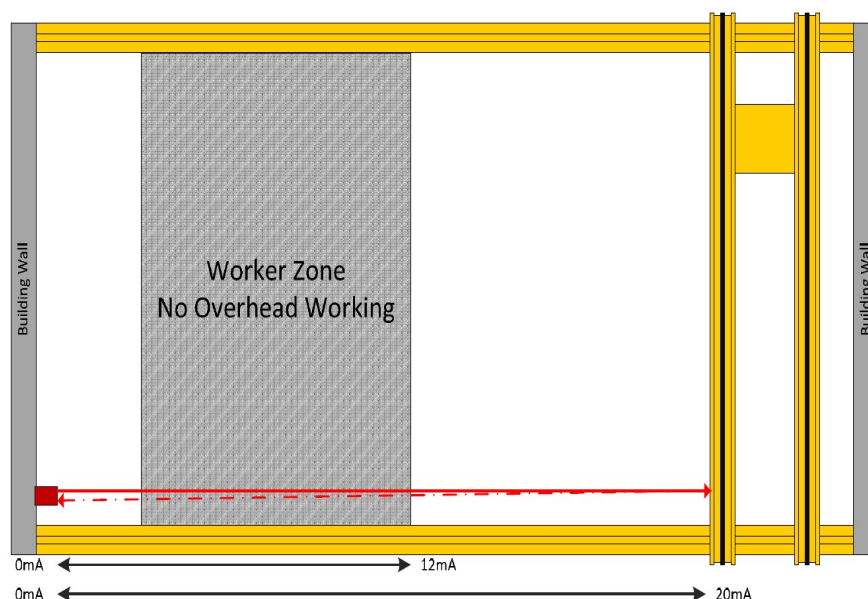
Figure 31 - example of laser utilised for crane to wall sensing (26)
