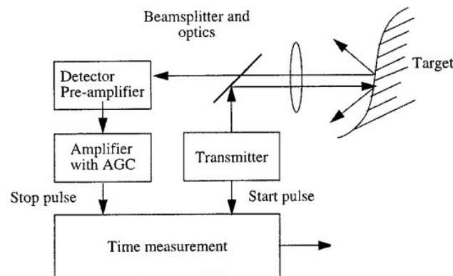
Figure 14 - Block diagram of TOF laser rangefinder
