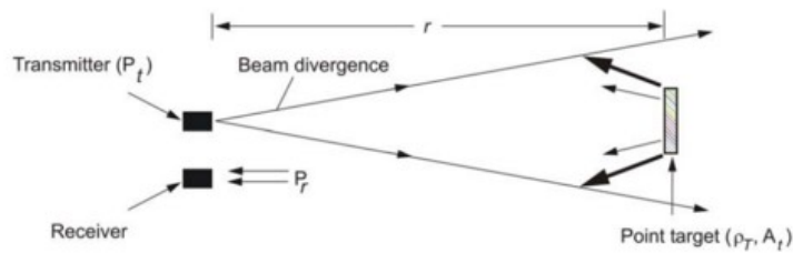
Figure 23 - Schematic of the detection of point target (20)
