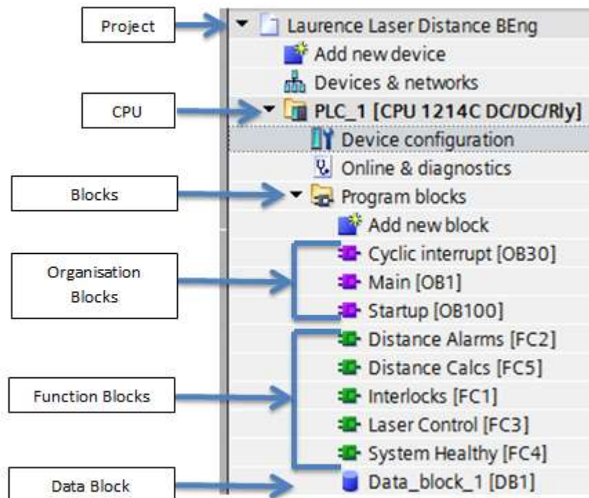
Figure 59 - Project Structure
