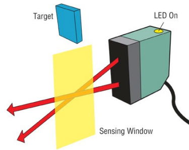
Figure 12 - Diffused convergent beam sensing window (9)
