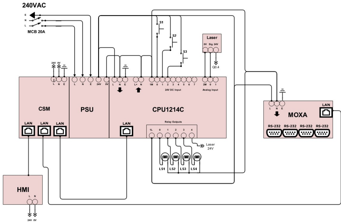
Figure 48 - Circuit Design
