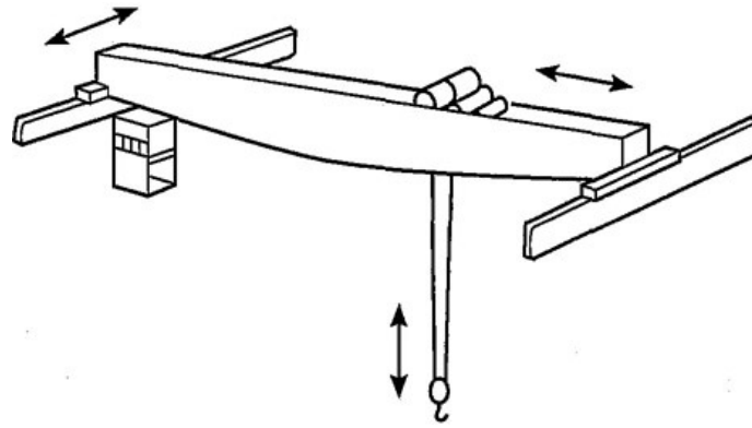
Figure 3 - Directional motions of an overhead bridge crane
