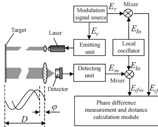
Figure 18 - Block diagram of phase shift laser range finder (14)
