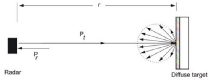
Figure 26 - Reflectivity of a diffuse target (large scattering reflection) (20)
