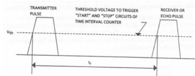
Figure 16 - Leading edge detection using threshold trigger (13)
