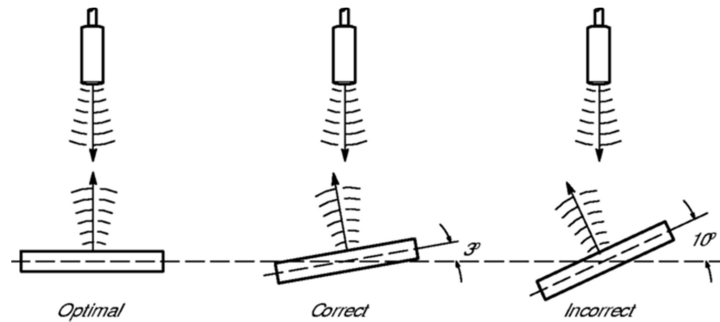
Figure 9 - Alignment of flat target (8)
