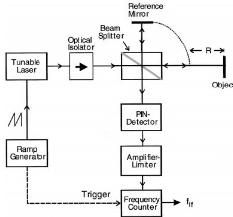
Figure 20 - Set up of FMCW optical radar system using tuneable laser diode as light source (11)
