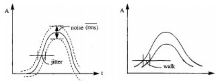
Figure 17 - Timing walk and jitter
