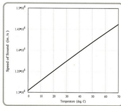
Figure 6 - Speed of sound as a function of temperature (3)
