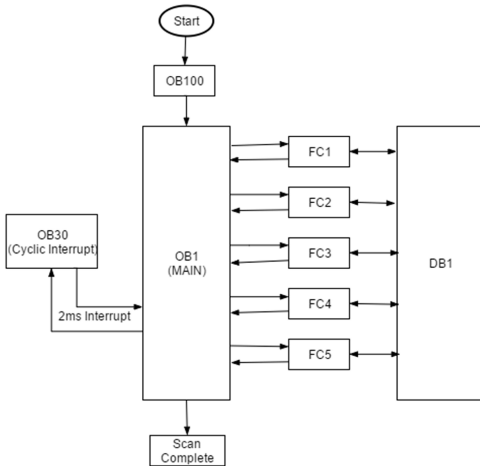
Figure 79 - Final Program Structure Diagram
