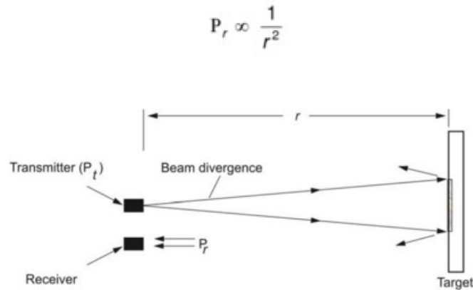
Figure 24 - Schematic of extended target detection (20)
