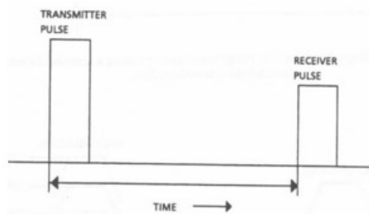
Figure 15 - Pulse range measurement by leading edge detection (13)
