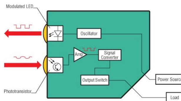
Figure 11 - operation of a photoelectric sensor (9)
