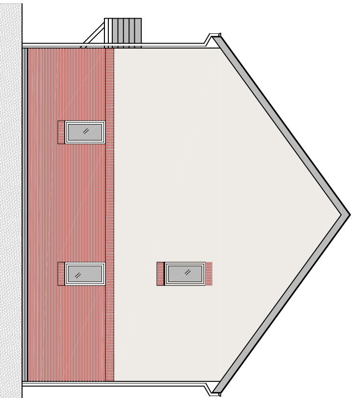
Edrychiad Ochr Arfaethedig 1:100 Proposed Side Elevation 1:100
