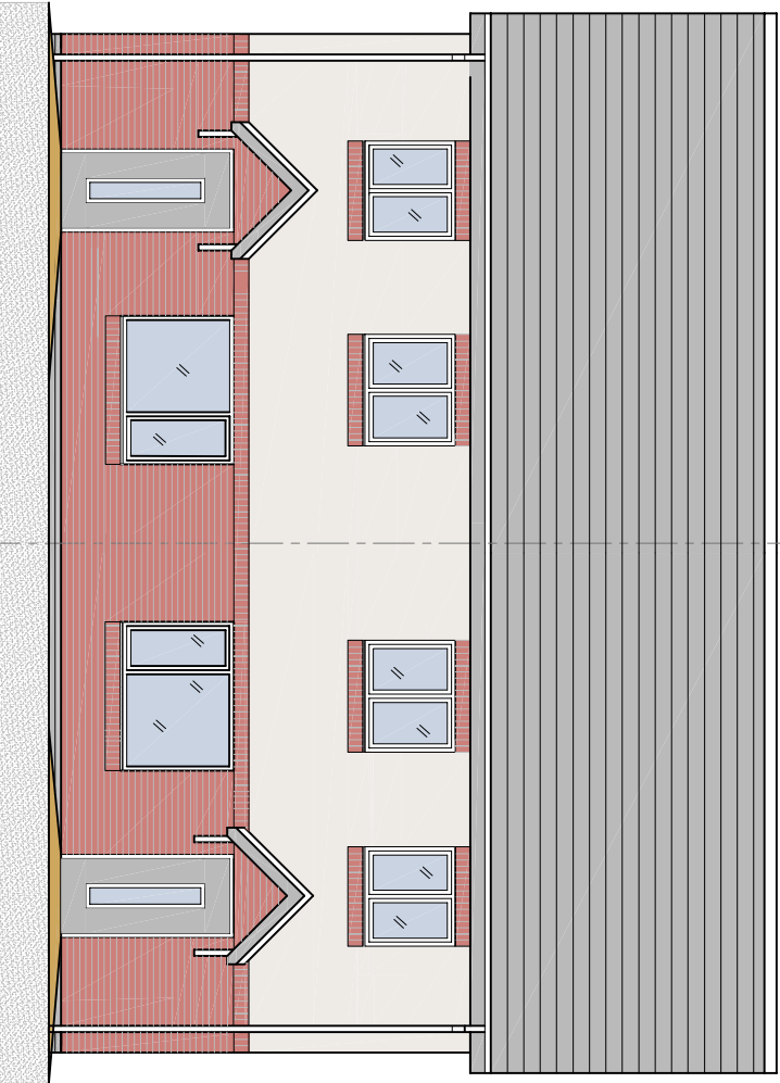
Edrychiad Blaen Arfaethedig 1:100 Proposed Front Elevation 1:100
