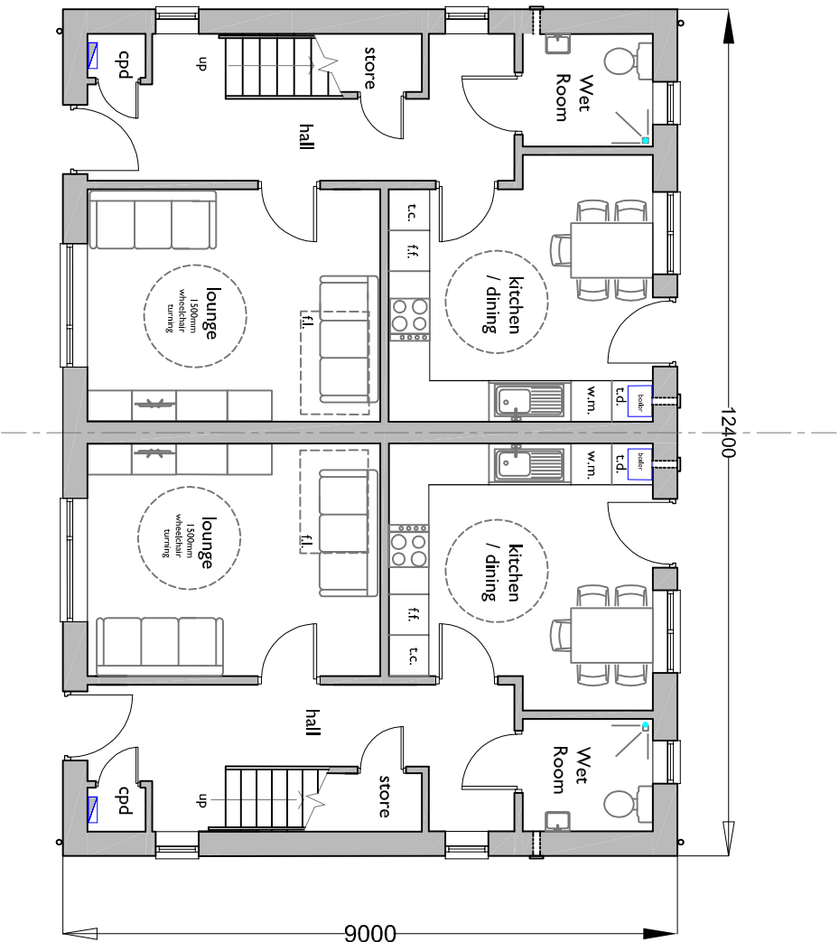
Cynllun Llwr Gwaelod Arfaethedig 1:100 Proposed Ground Floor Plan 1:100
