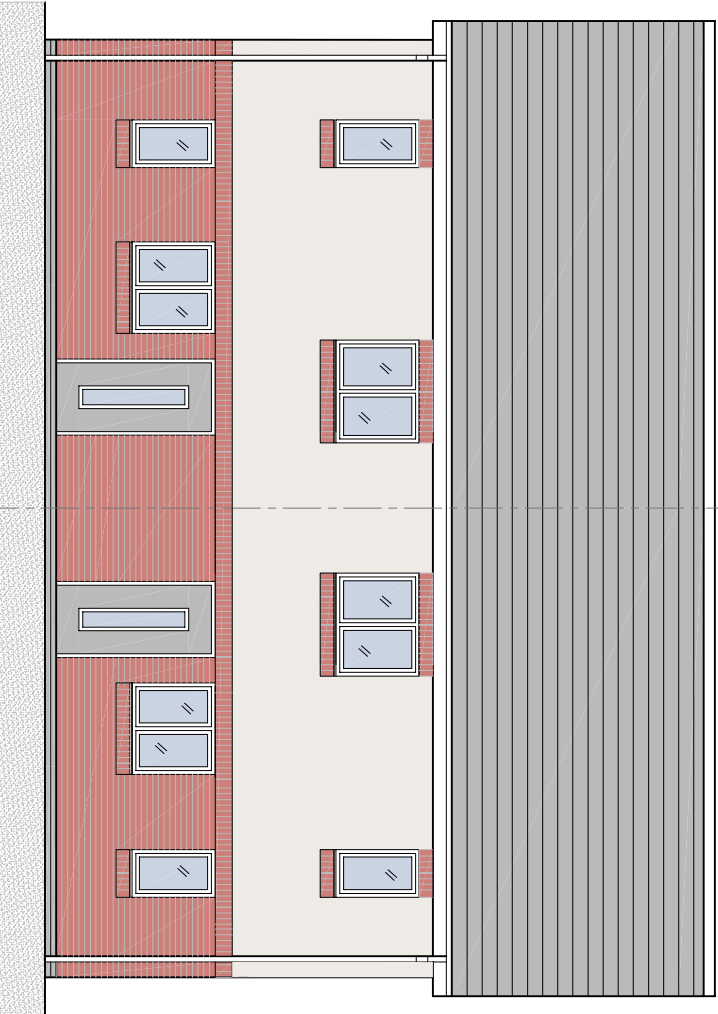
Edrychiad Cefn Arfaethedig 1:100 Proposed Rear Elevation 1:100
