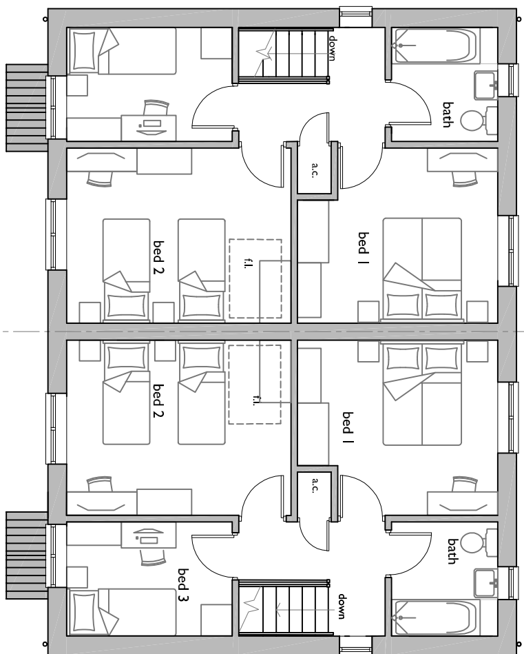
Cynllun Llwr Cyniaf Arfaethedig 1:100 Proposed First Floor Plan 1:100
