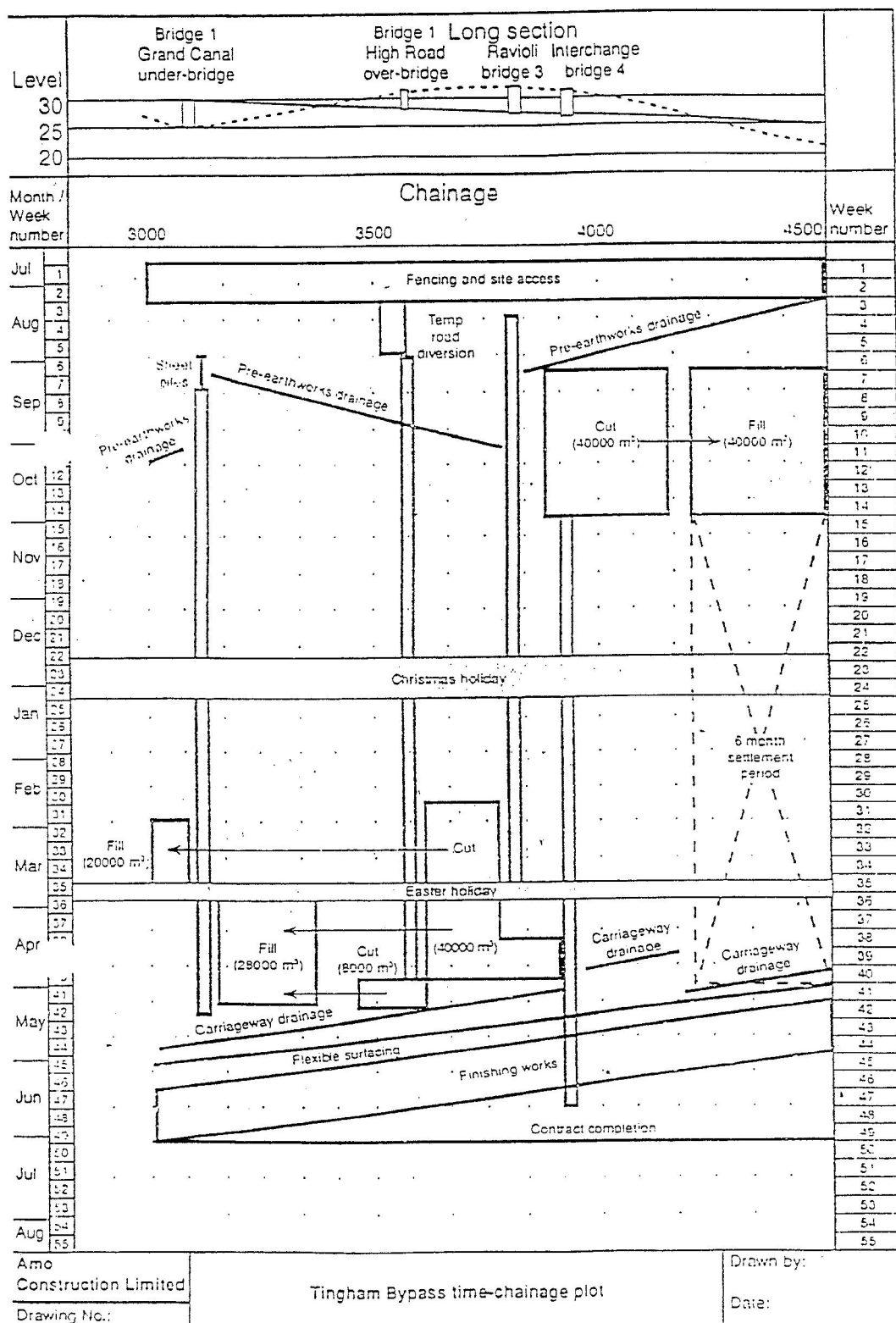
Time-chainage chart for a road project.
