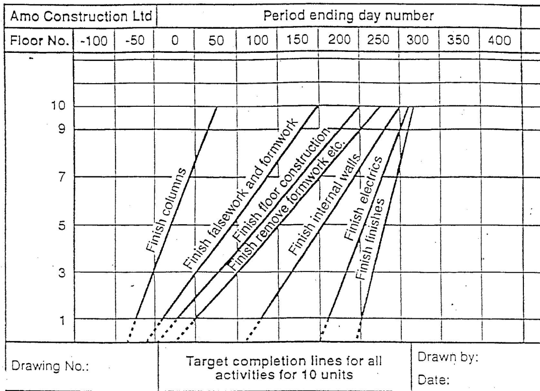
Resource-based target- completion-time graph.
