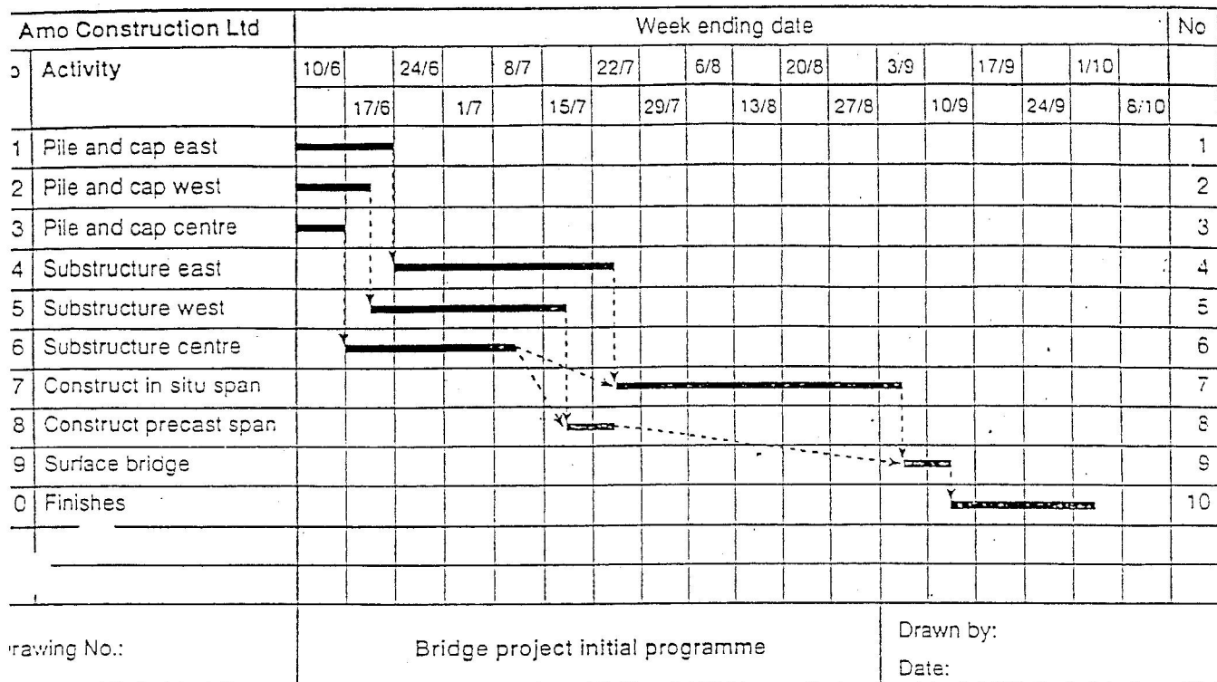
A linked bar chart.
