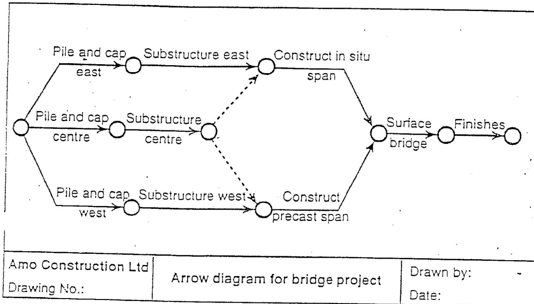
An activity-on-arrow network (arrow diagram).
