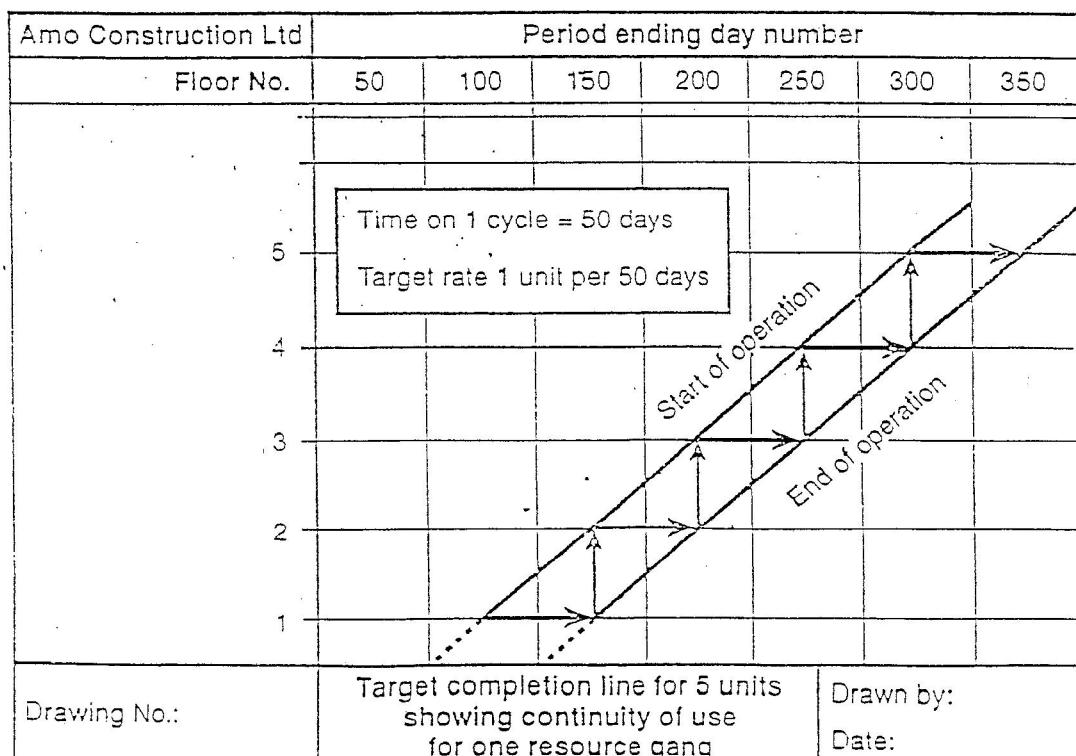
Progress line showing continuity of working for a single resource gang.
