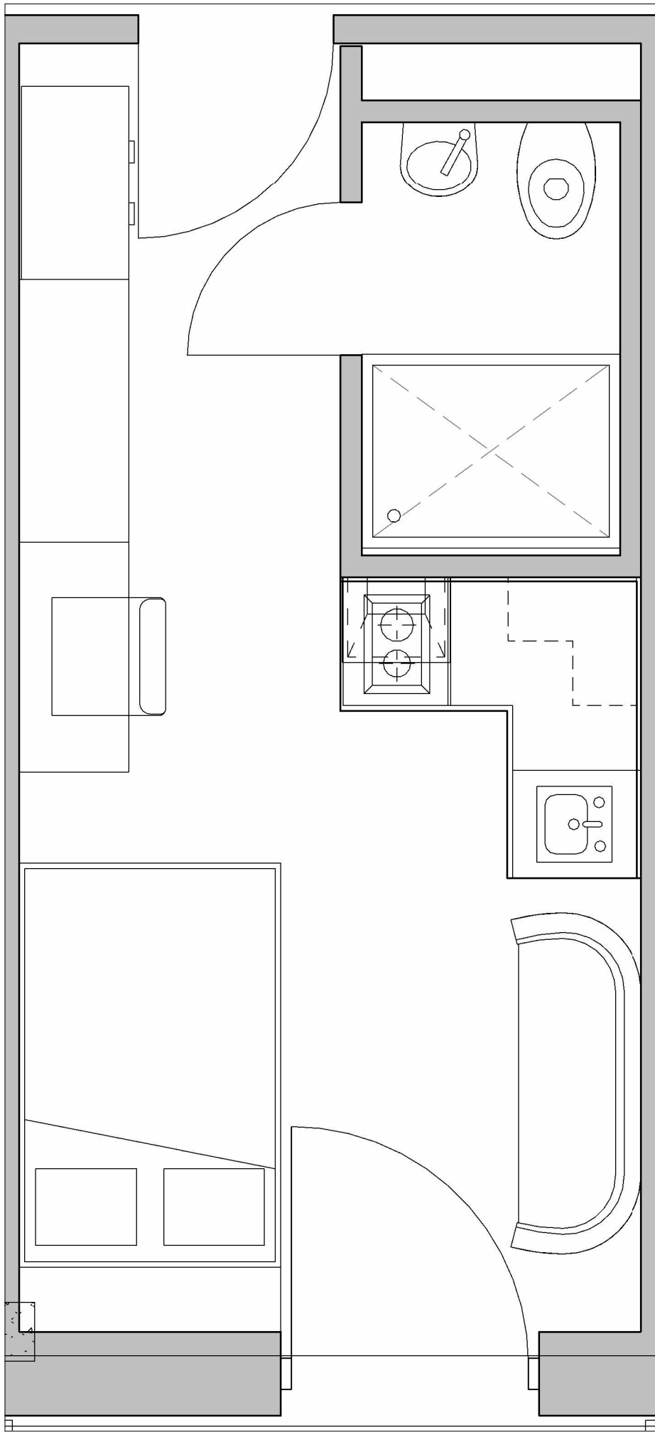
Social Studio Plan 1 : 25
