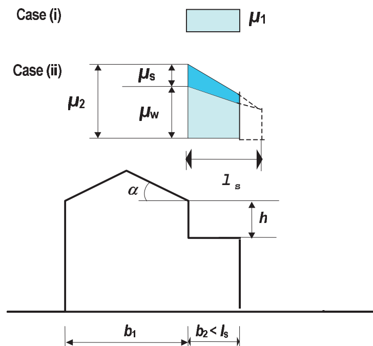
Figure 5.6 \langle A_1 \rangle : Snow load shape coefficients for roofs abutting to taller construction works
