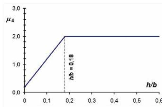
Figure 5.4 — Recommended snow load shape coefficient for cylindrical roofs of differing rise to span ratios (for \beta \leq 60^\circ ) \langle A_1 \rangle
