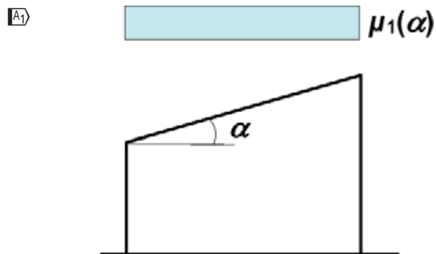
Figure 5.1 — Snow load shape coefficient - monopitch roof \langle A_1 \rangle
