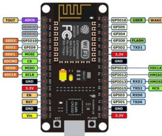
Figure 3: NodeMCU V2 and pin diagram
