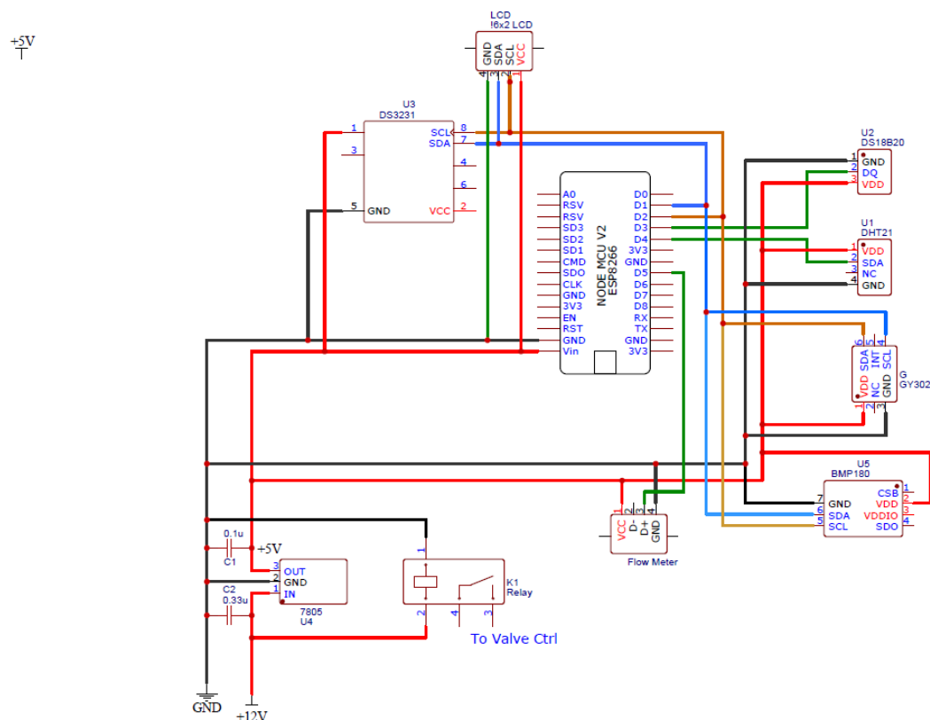
Figure 2: Schematic diagram of the proposed Smart farming system
