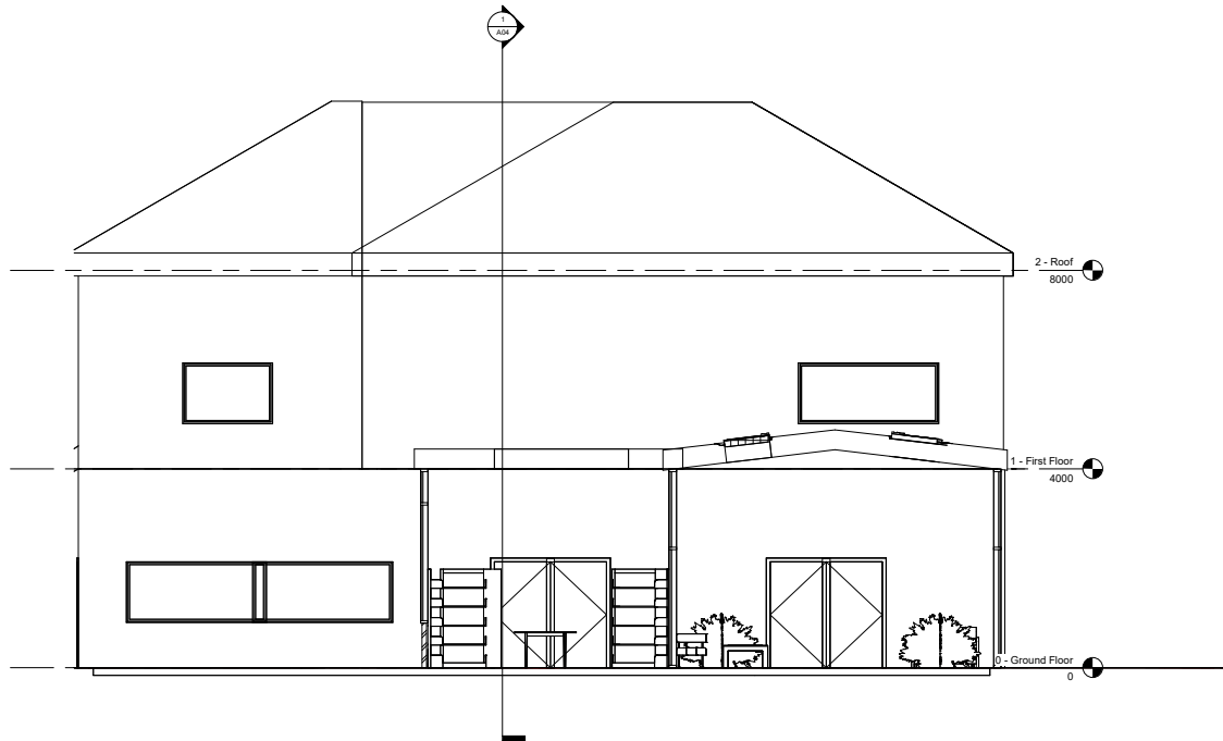
1 Section B-B (Short Section) 1 : 50
