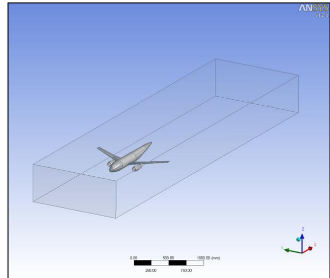
Enclosure created for an airplane
