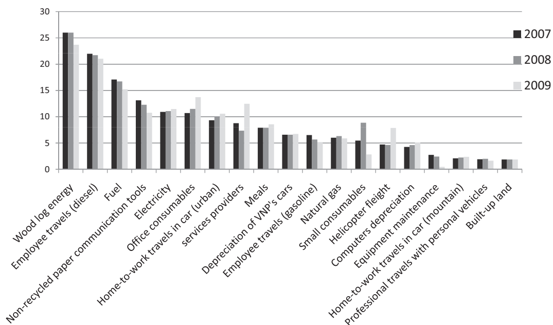
Fig. 3. Evolution of the 20 main ecological footprint contributors, 2007–2009 (gha).
