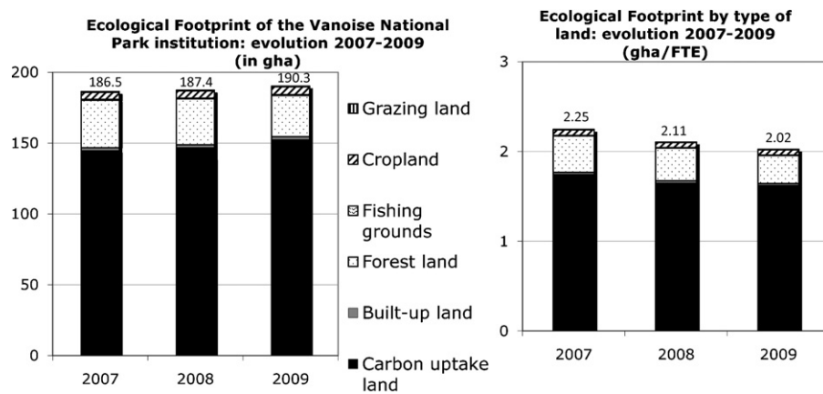
Fig. 1. Evolution of the Vanoise National Park Ecological footprint (2007–2009).
