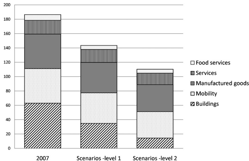
Fig. 4. 2007 Ecological footprint and scenarios more (scenario 2) or less (scenario 1) ambitious (expressed in gha).
