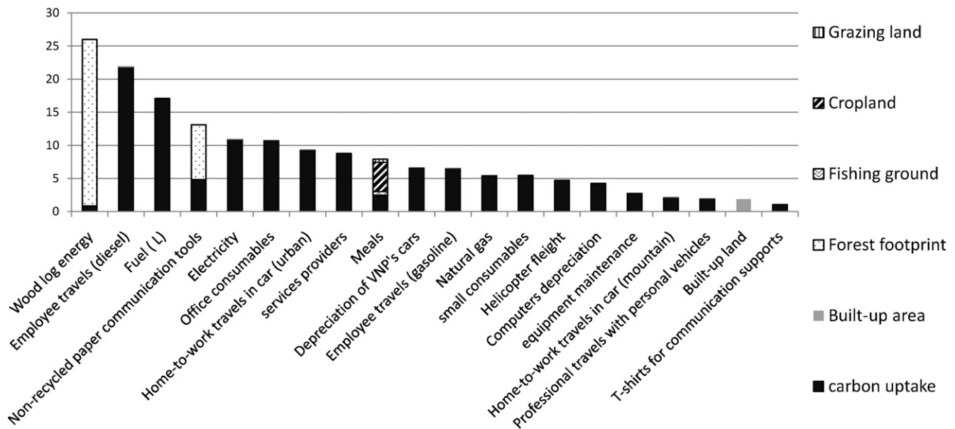
Fig. 2. 20 main components of the 2007 Vanoise National Park's ecological footprint (gha) by type of land.
