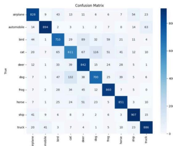
Figure 4.3: Confusion Matrix
