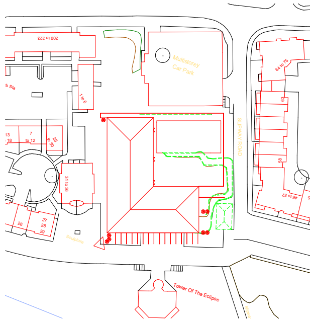
② Location Plan 1 : 500
