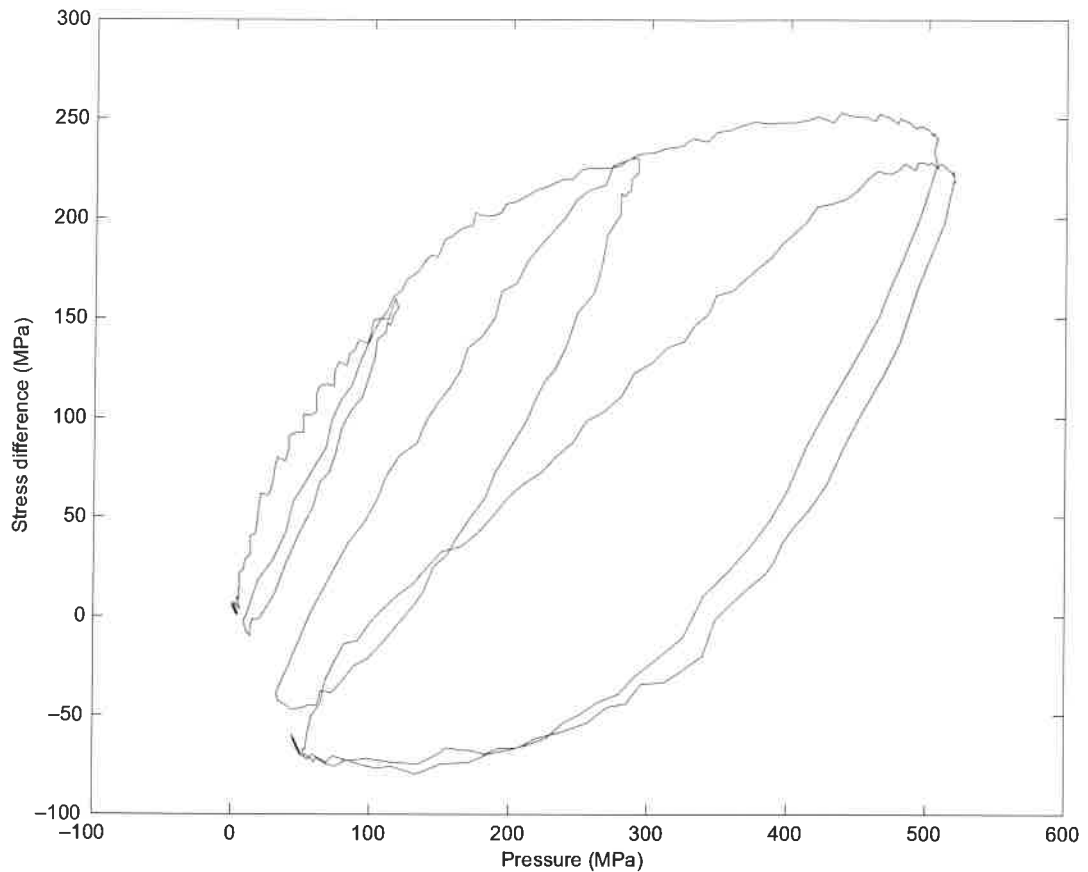
Figure 4.2: GREAC cell stress difference data from a real test.
