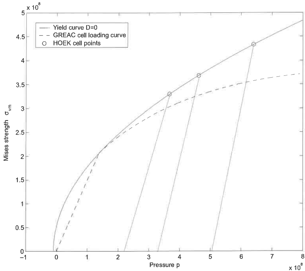
Figure 4.5: By performing various Hoek Cell tests we can obtain different points on the D=0 yield curve.
