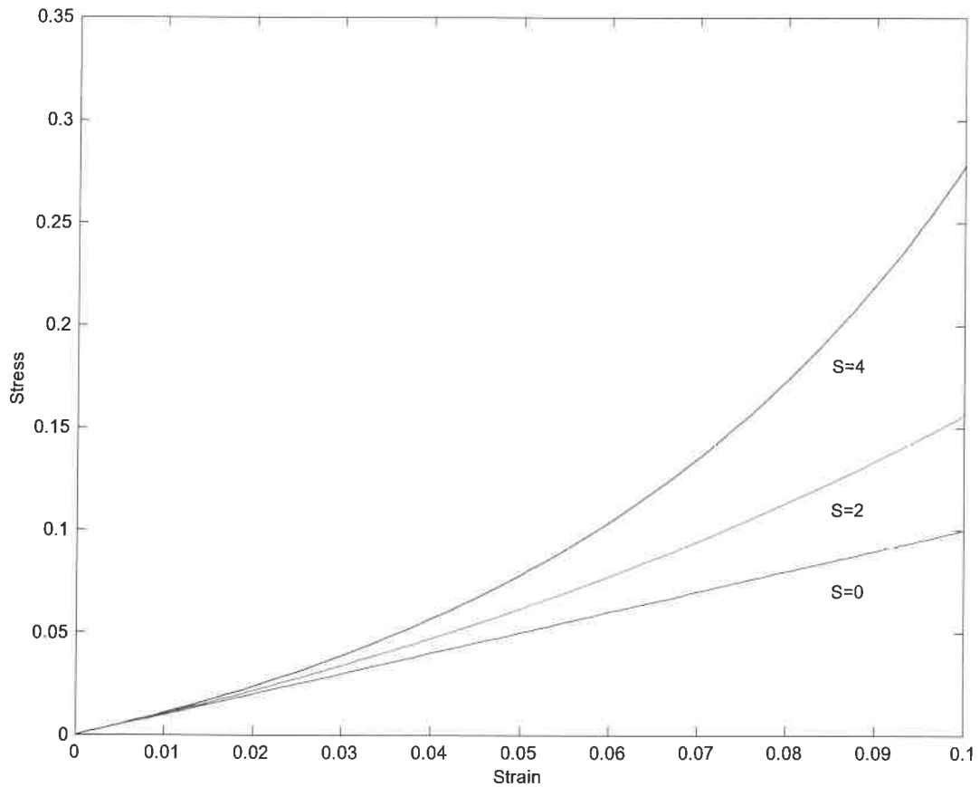
Figure 8.1: Stress-strain relationship for different values of the parameter S in the (linear) EOS Equation (8.4). Note that the stress is divided by \rho_0 c^2 and that actually the negative of stress/strain has been plotted (thus, positive values in the figure corresponds to compression).
