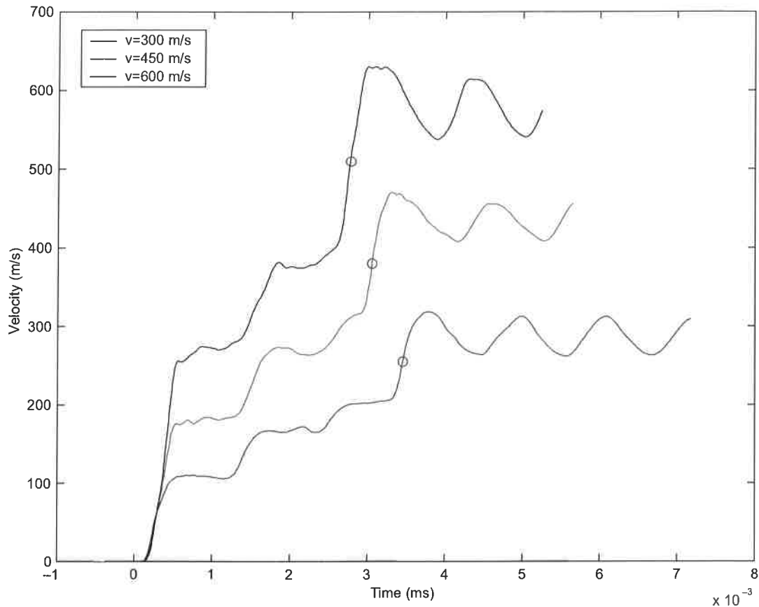
Figure 8.4: Velocity at the back face of the target plate for a material with a linear shock EOS.
