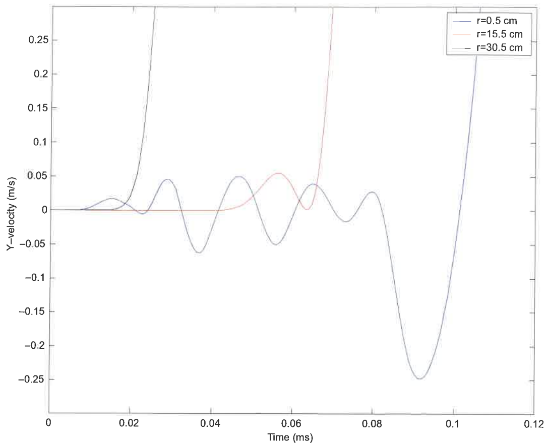
Figure 5.4: Radial velocity for the same three target points.
