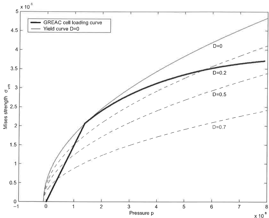
Figure 4.4: During a GREAC cell test the damage may not be constant and thus the yield curve obtained is not for constant D=0 . (This is a theoretical plot not based on any experimental data).
