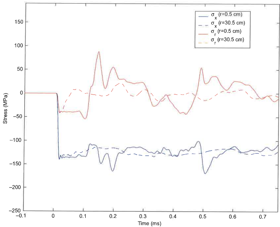
Figure 5.2: Axial and radial stress as a function of time at two points inside the target.
