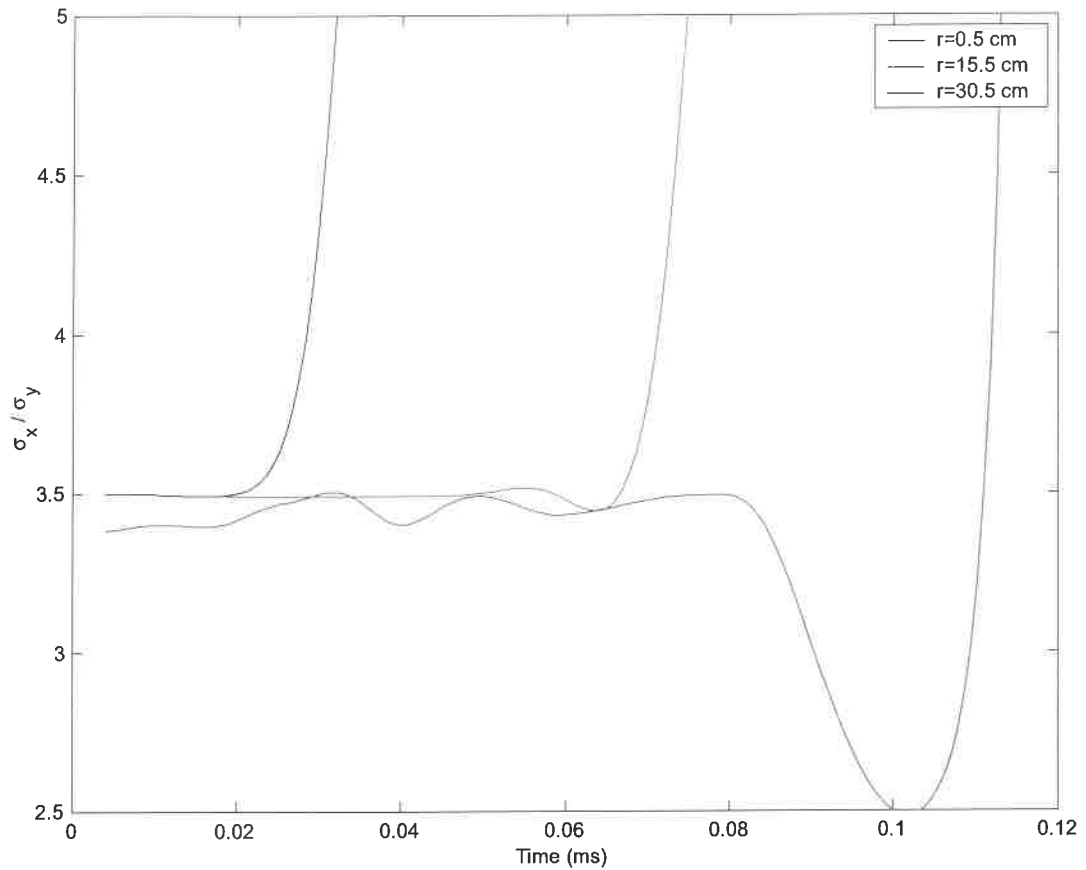
Figure 5.3: Ratio of axial and radial stress for several targets points located at different distance from the symmetry axis.
