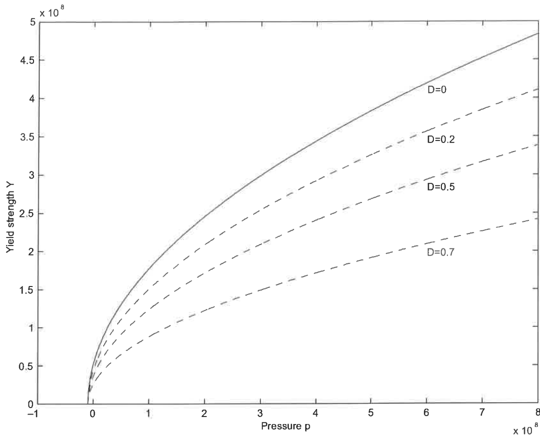
Figure 4.3: Possible yield curves for various values of the damage parameter.
