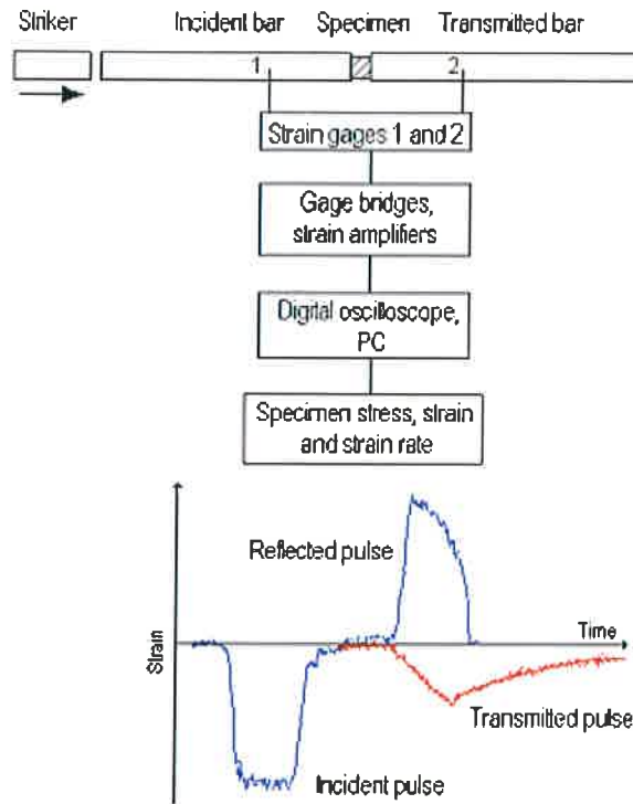
Figure 7.1: Illustration of a Split Hopkinson Bar. (Figure created by University of Tampere, Finland).
