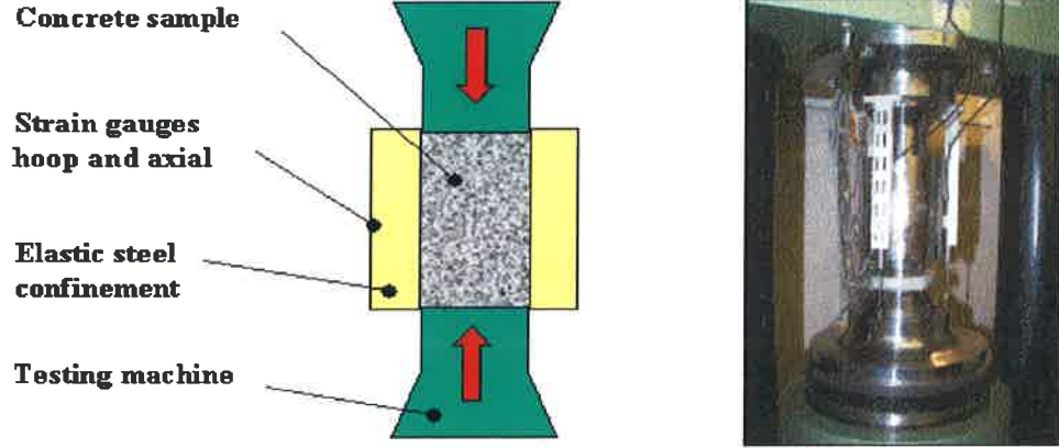
Figure 4.1: GREAC cell
