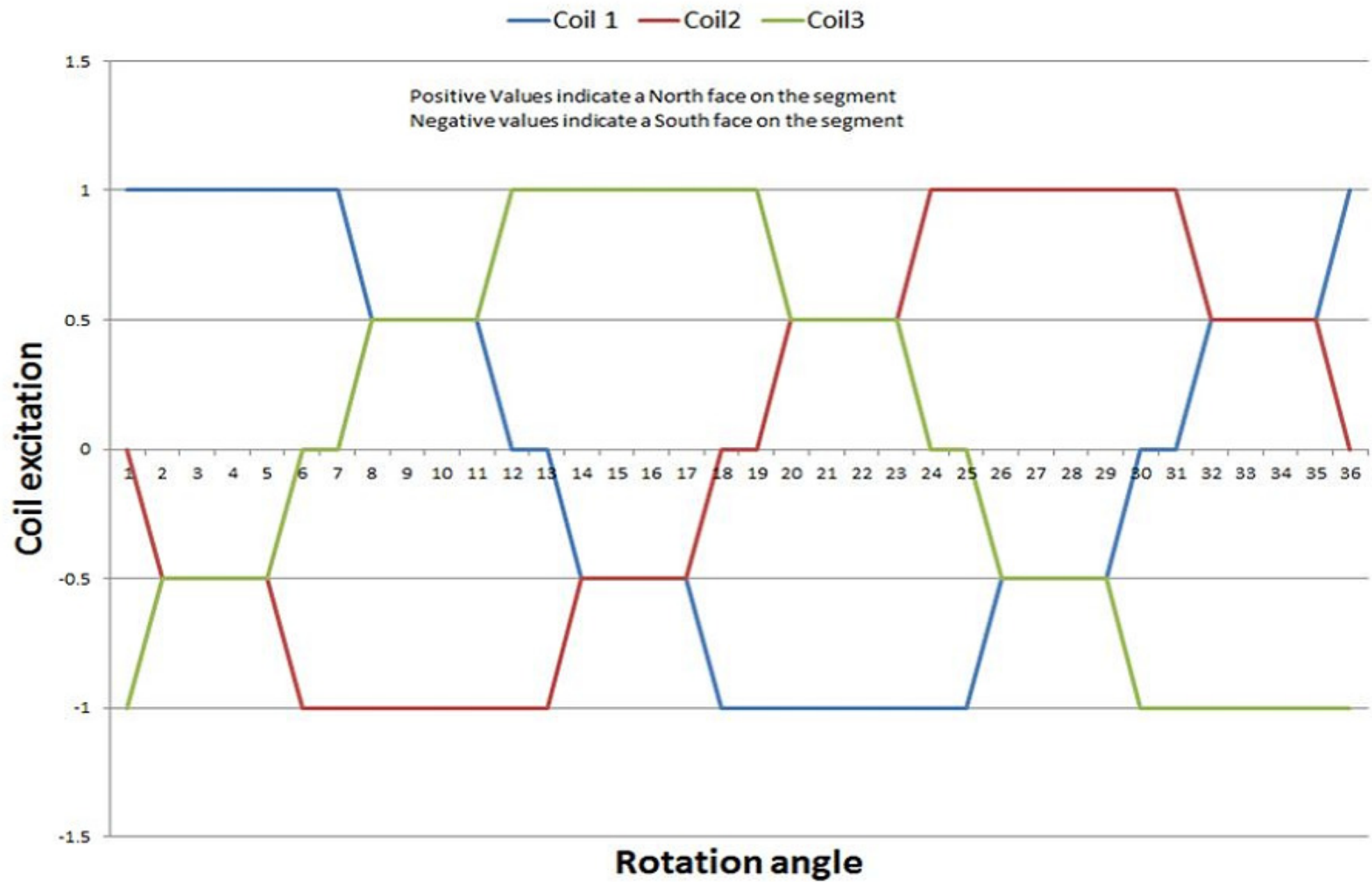
Coil Excitation timing diagram
