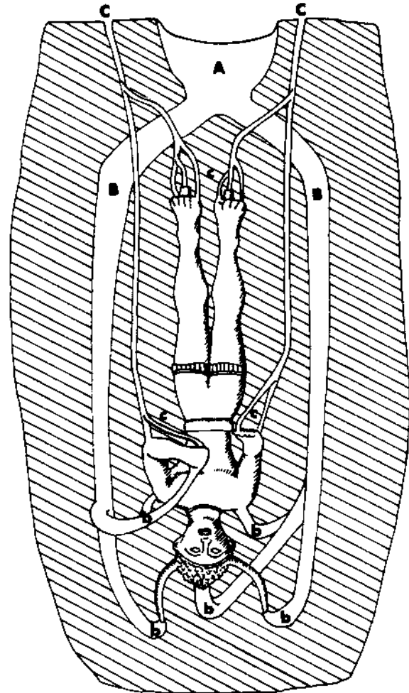
FIG. 129. Hypothetical mold for casting Horned God from Enkomi, by Susan Womer. A. Funnel-shaped opening. B. Metal runners. C. Air vents.
