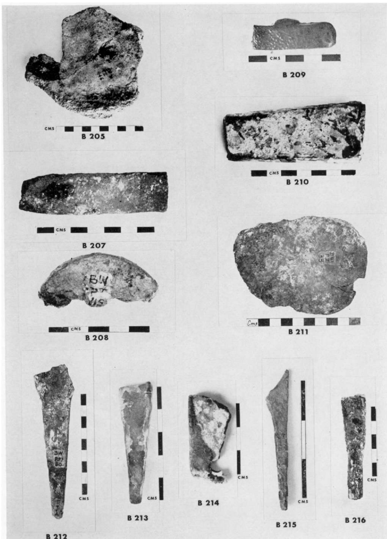
FIG. 123. Bronze attaching devices and unidentified objects.
