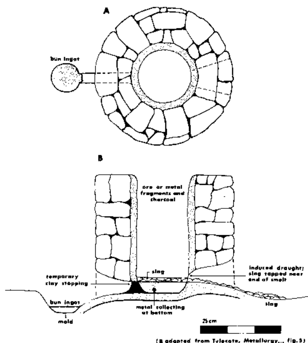
CONCEPTION OF FURNACE WHICH COULD HAVE MADE COPPER OR BRONZE BUN INGOTS
