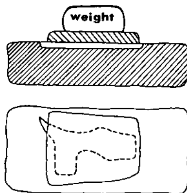
FIG. 125. Stone cover on open mold prevents oxidation on surface of bronze.
