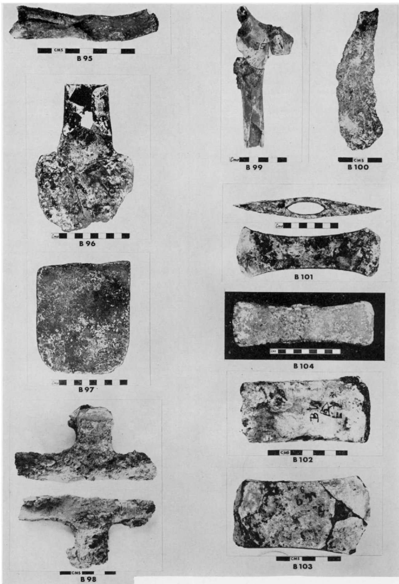
FIG. 108. Socketed tool, shovel, mattock, pruning hooks, sickle, and double axes.
