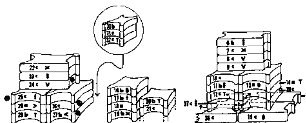
FIG. 91. Restored order of stacking of ingots in ship. Ingots from area P (bow) at right, from area G (stern) at left. Exact orientation of In 15 and In 39 uncertain.
