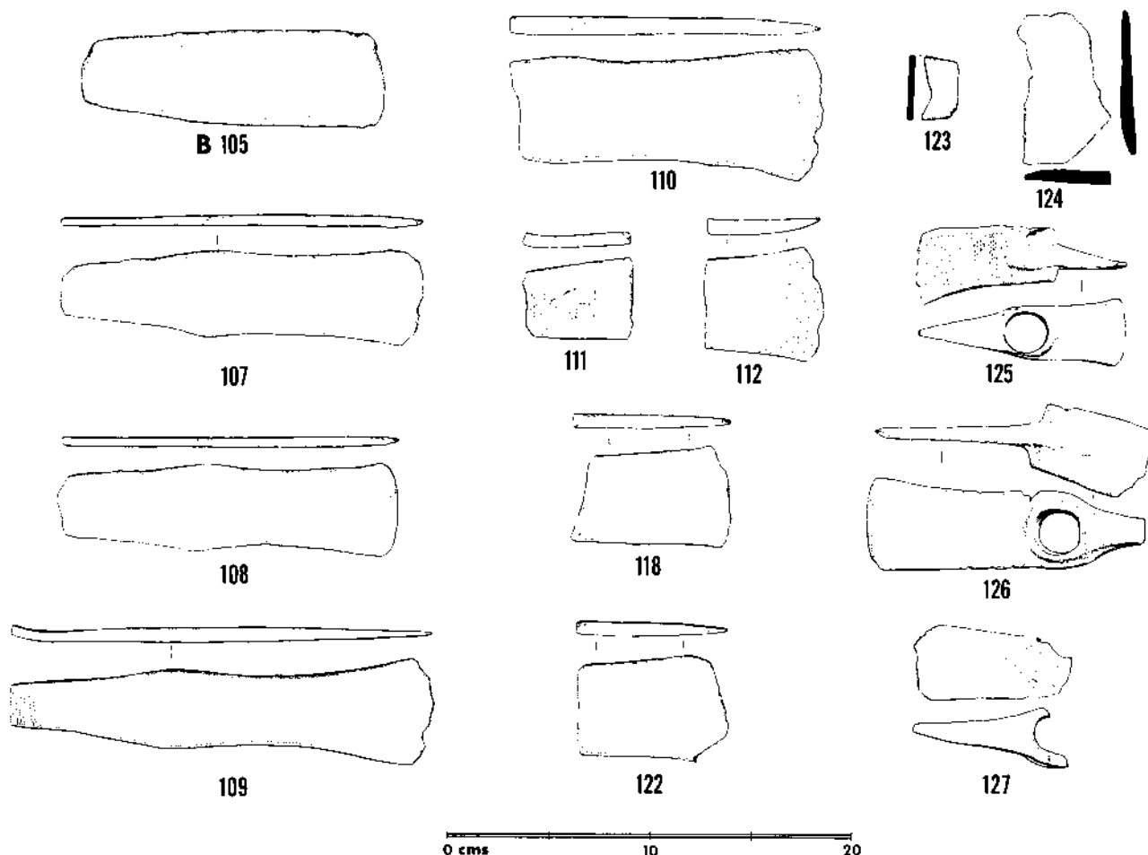
FIG. 109. Bronze adzes and axe-adzes: B 105 to B 127.
