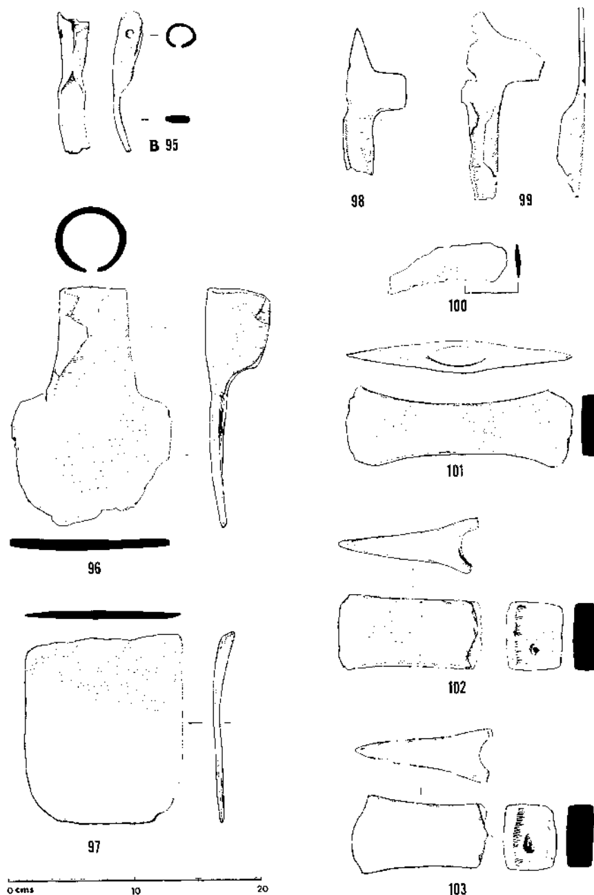
FIG. 107. Bronze tools: B 95 to B 103.
