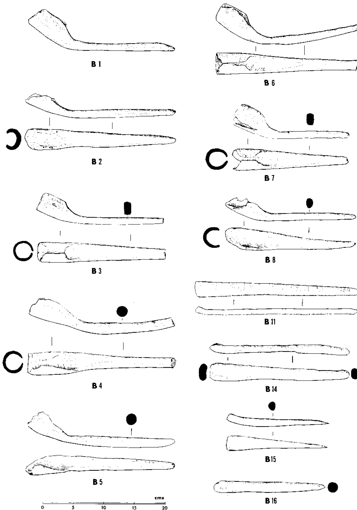
FIG. 99. Bronze picks: B1 to B16.
