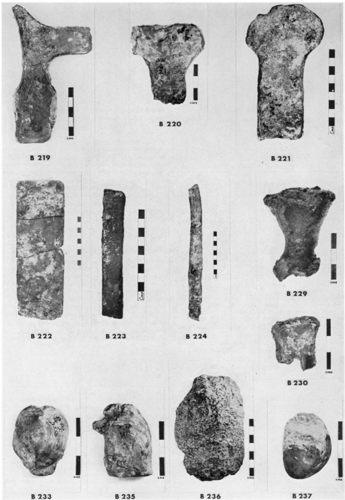
FIG. 127. Blanks for unfinished bronze tools, and casting waste.
