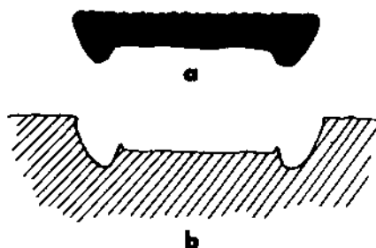
FIG. 89a. Usual draft of Cape Gelidonya ingots.
