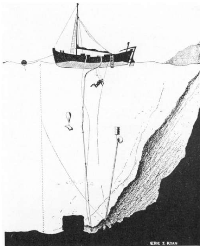
FIG. 21. Both air lifts positioned on wreck with Lutfi Gehl above.
