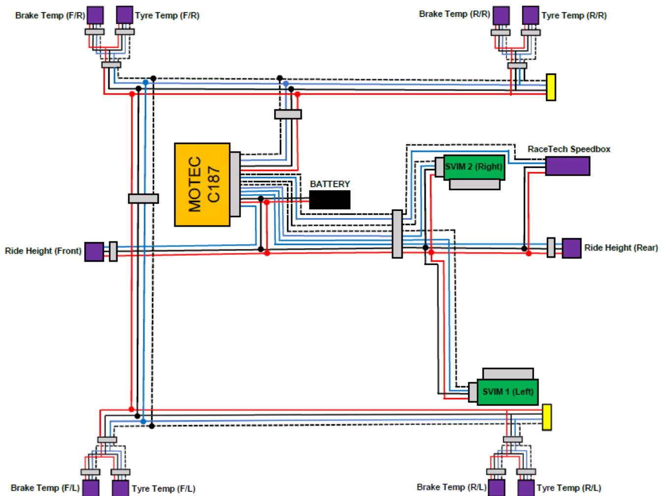
Figure 19: MOTEC C187 & CAN Schematic
