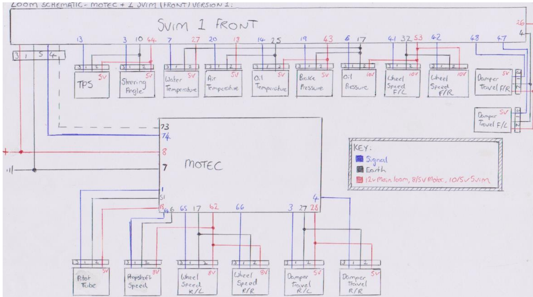
Figure 50: DAS Version 1: Motec and 1 SVIM Schematic (Bartram, 2018)
