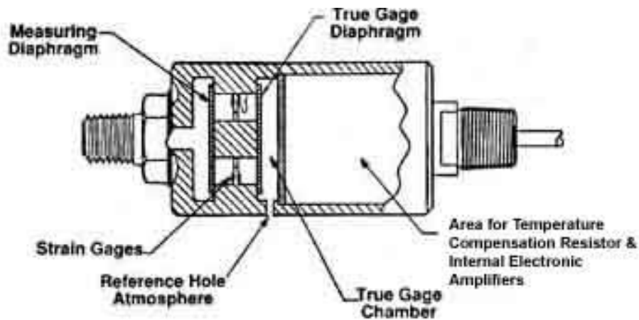
Figure 11: Pressure Transducer (Industrial Electronics, 2018)
