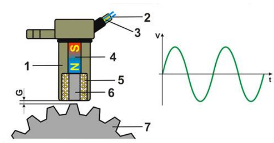
Figure 8: Inductive Sensor (Mucevski, 2015)
