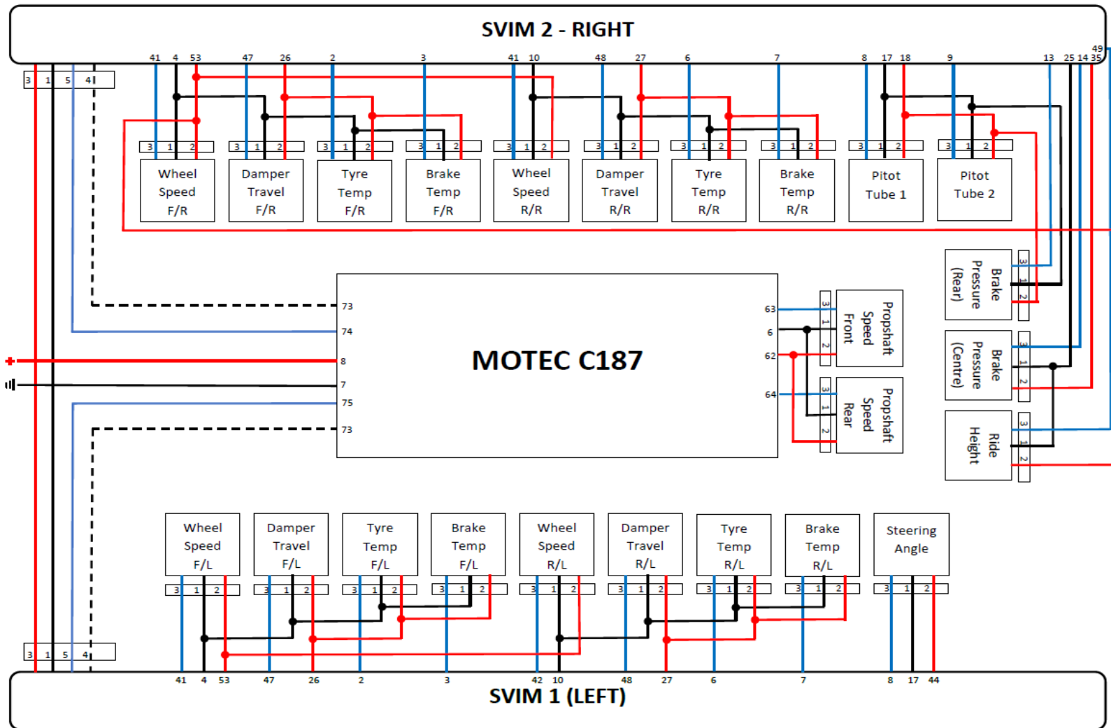
Figure 52: DAS Version 2: Motec and SVIM Schematic (Bartram, 2018)
