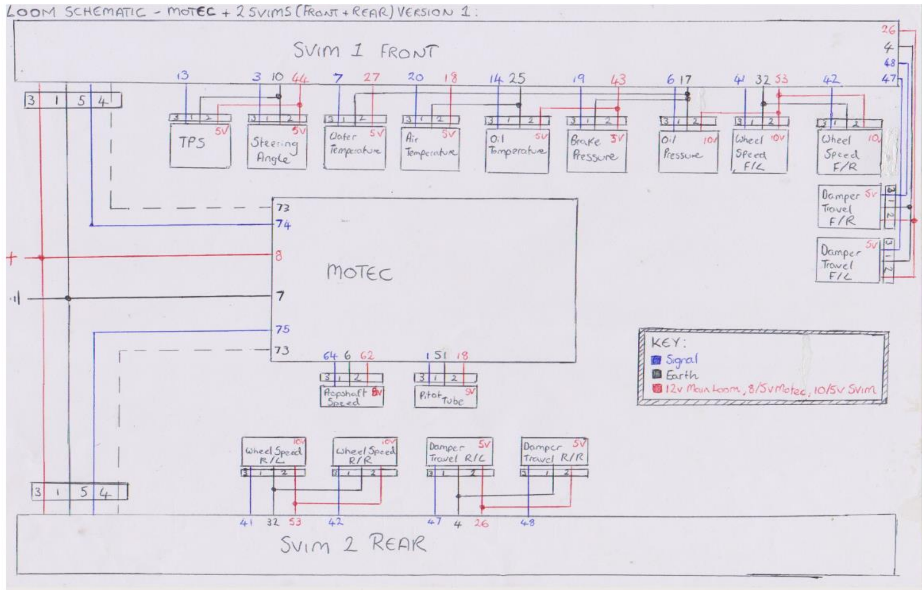
Figure 51: DAS Version 1: Motec and 2 SVIMs Schematic (Bartram, 2018)
