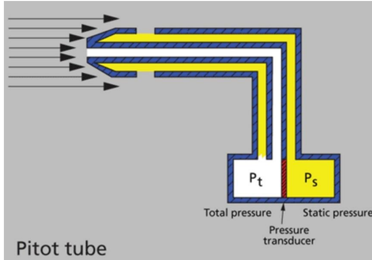
Figure 12: Pitot Tube (Denizen, 2017)
