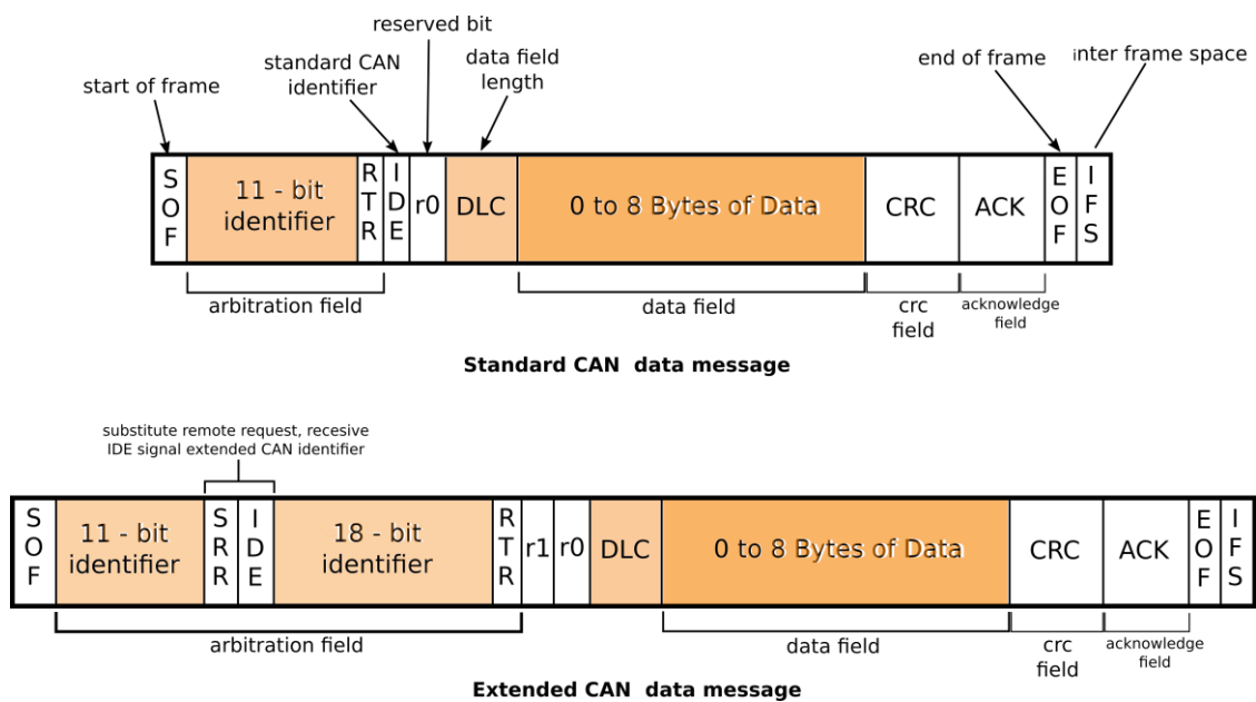
Figure 4: Architecture of a Data Frame (Dewesoft, 2019)
