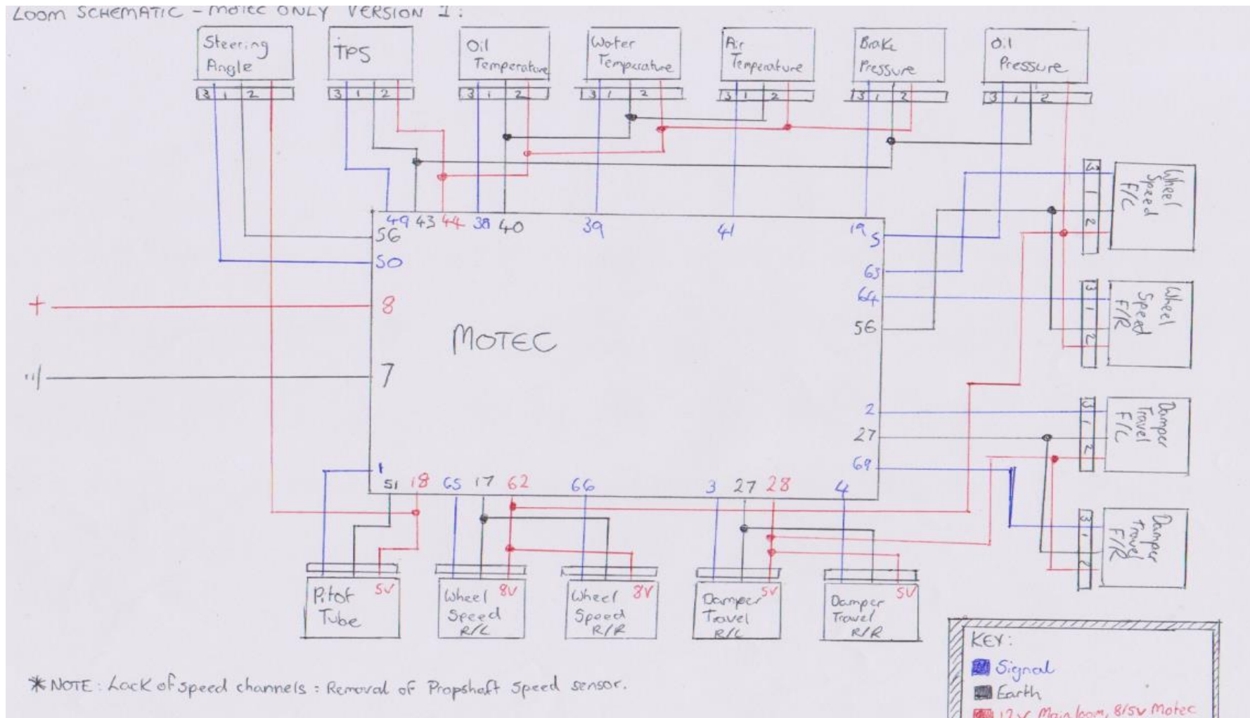
Figure 49: DAS Version 1: Motec Only Schematic (Bartram, 2018)
