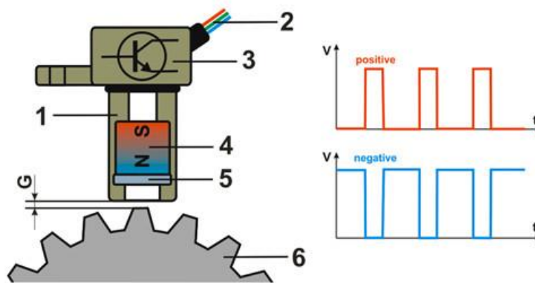
Figure 7: Hall Effect Sensor (Mucevski, 2015)
