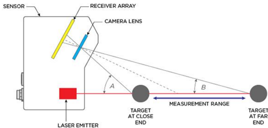
Figure 13: Laser Transducer (Pastorius, 2014)
