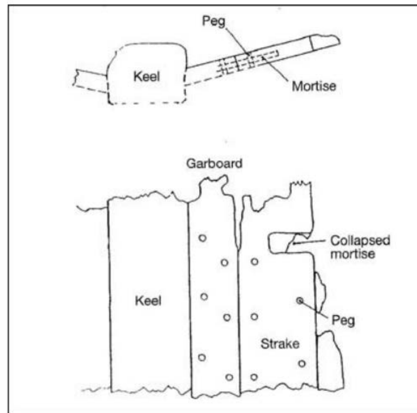
Plate Uluburun wreck remains (after McGrail, 2001, Fig. 4.22)
