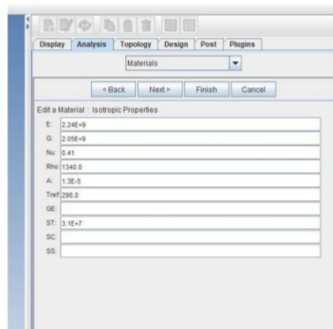
Figure 2 - Ultem 9085 Material Properties
