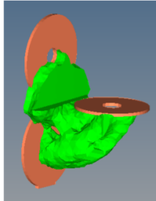
Figure 16 - Topology Optimisation from Winning Contestant
