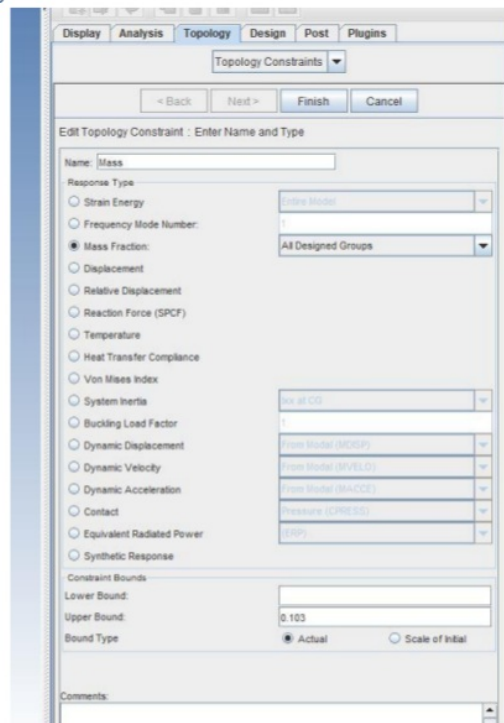
Figure 10 - Topology Constraints
