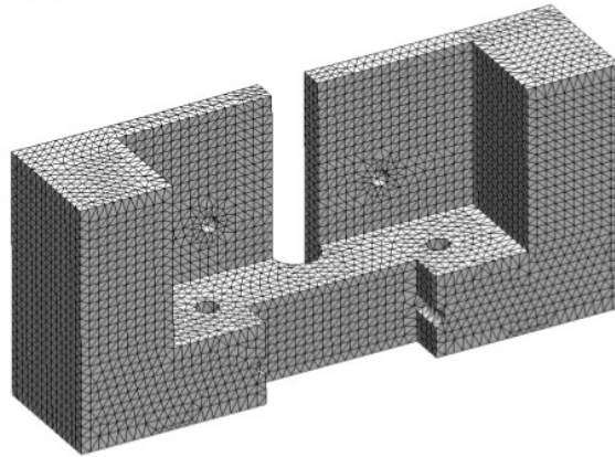
Figure 1 - CAD Model Mesh
