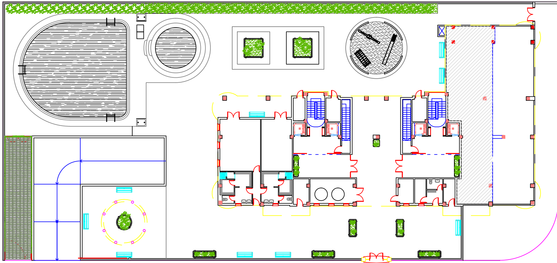
GROUND FLOOR SCALE 1/300
