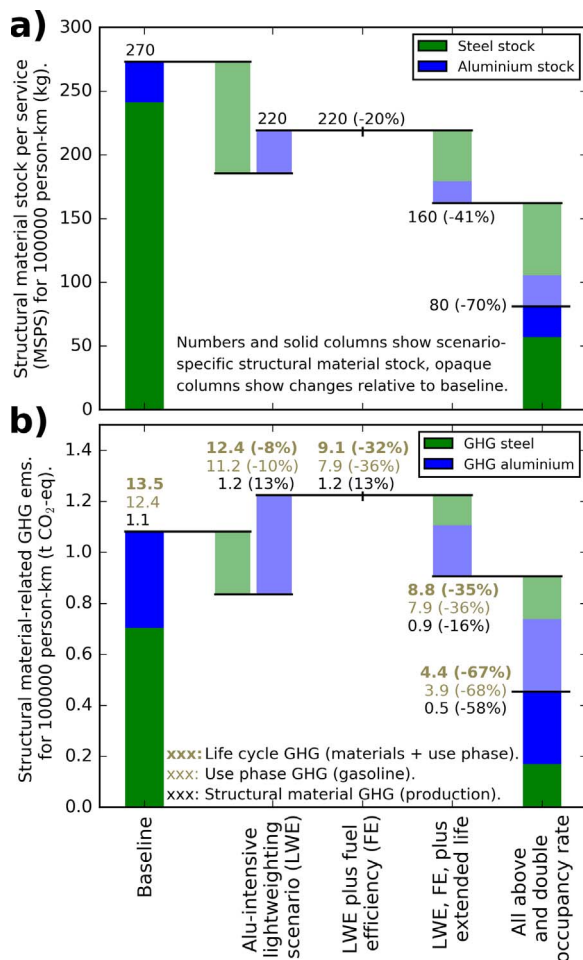
Fig. 3. Material stock per service (MSPS) (a) and greenhouse gas (GHG) emissions for the production of steel and aluminum (b) for the reference flow of 100,000 person-km provided by a gasoline-driven passenger car under different light-weighting and efficiency scenarios. The life cycle carbon footprint decreases from left to right. Data and scenario assumptions were extracted from Modaresi et al. (2014) and are described in the SI, the doubling of the occupancy rate in the rightmost scenario is an assumption.
