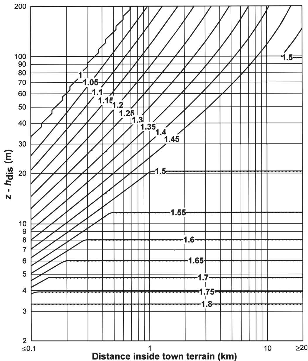
Figure NA.6 Values of turbulence correction factor k_{1,T} for sites in Town terrain
