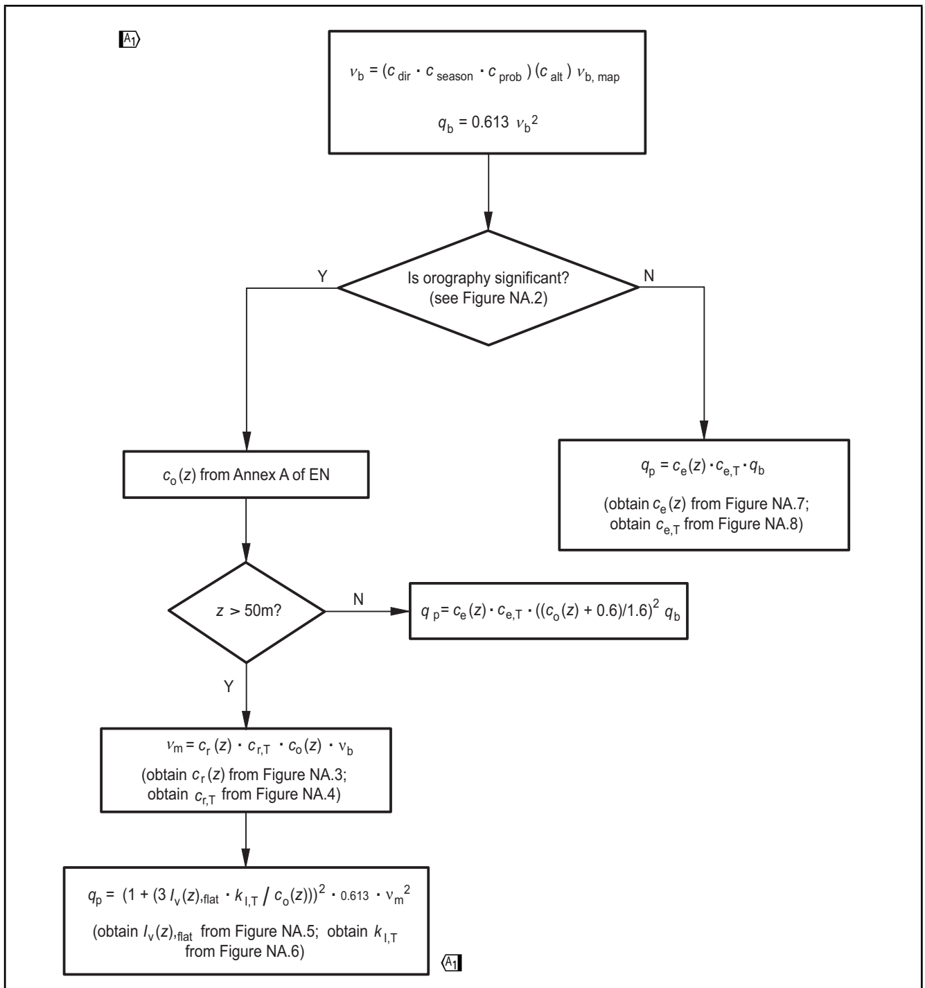
Figure A.NA.2 Flowchart for obtaining q_p for sites in town
