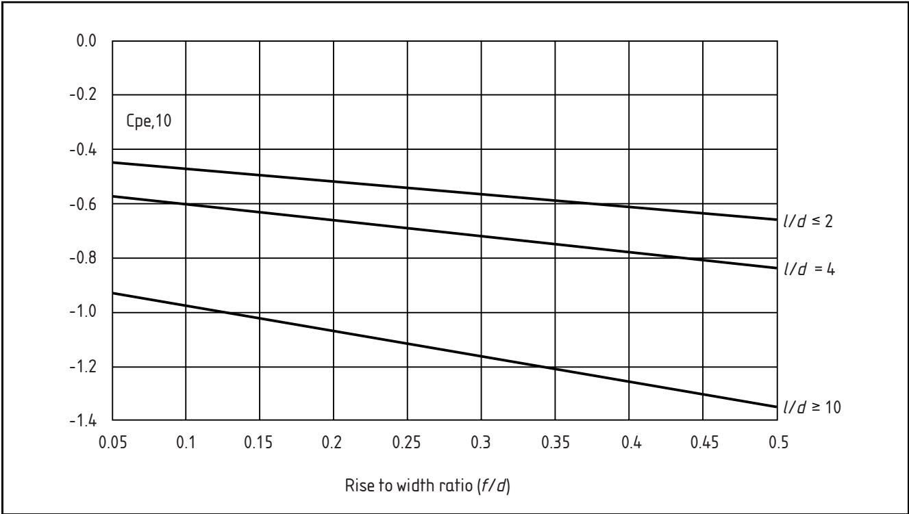
Figure NA.12 External pressure coefficients c_{pe,10} for zone B of vaulted roofs
