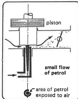
Principle of the constant-depression carburetter
