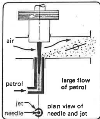
Principle of the constant-depression carburetter
