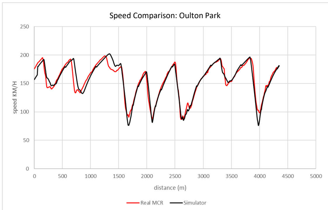
Graph 25 Oulton Park Speed Comparison Updated Braking Force
