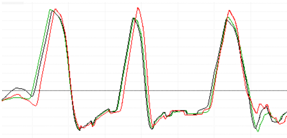
Figure 41 Oulton Park Longitudinal G Force Comparison
