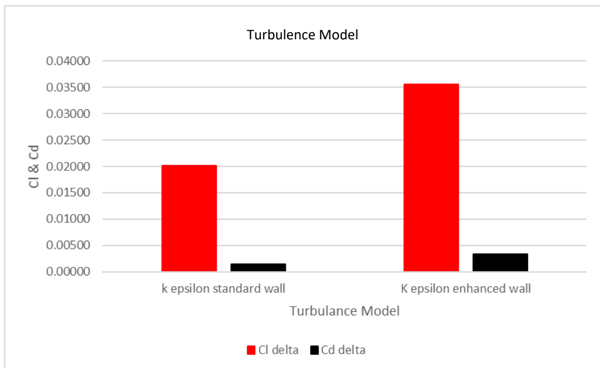
Graph 11 CFD Validation - Turbulence Model
