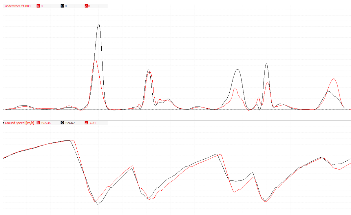
Figure 54 Understeer Comparison Both Drivers
