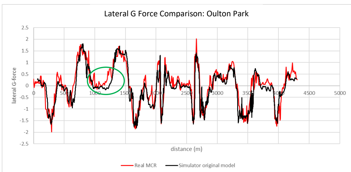
Graph 6 Oulton Park Lateral G Force Comparison
