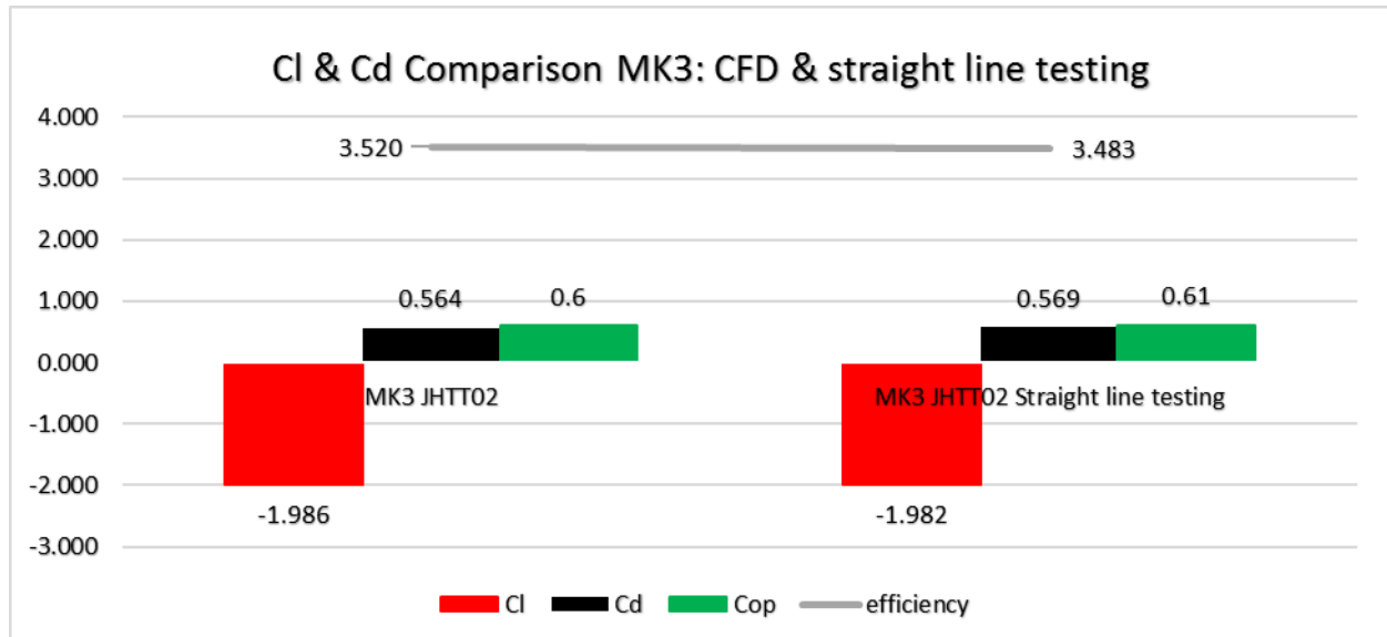
Graph 31 Aerodynamic Validation MK3
