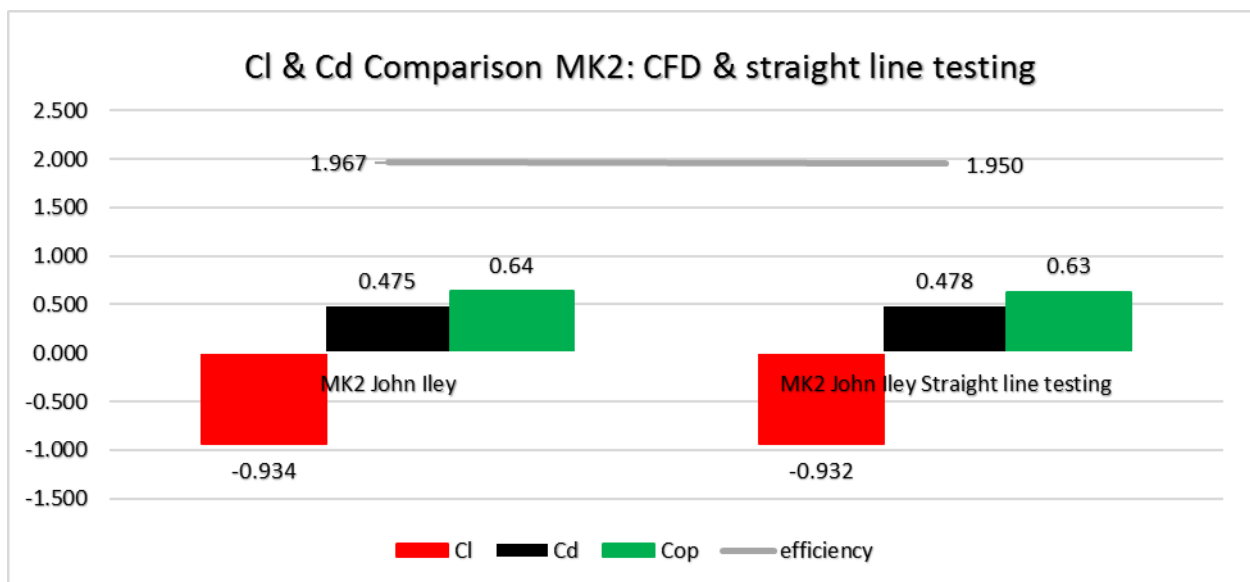
Graph 29 MK2 Aerodynamic Validation Comparison
