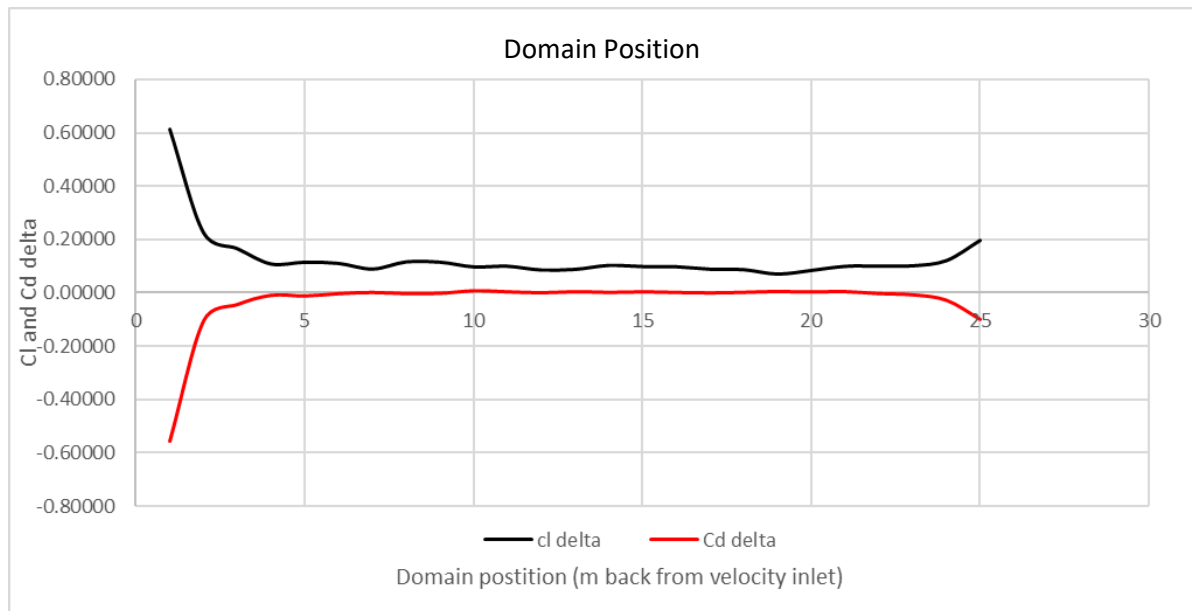
Graph 9 CFD Validation - Domain Position
