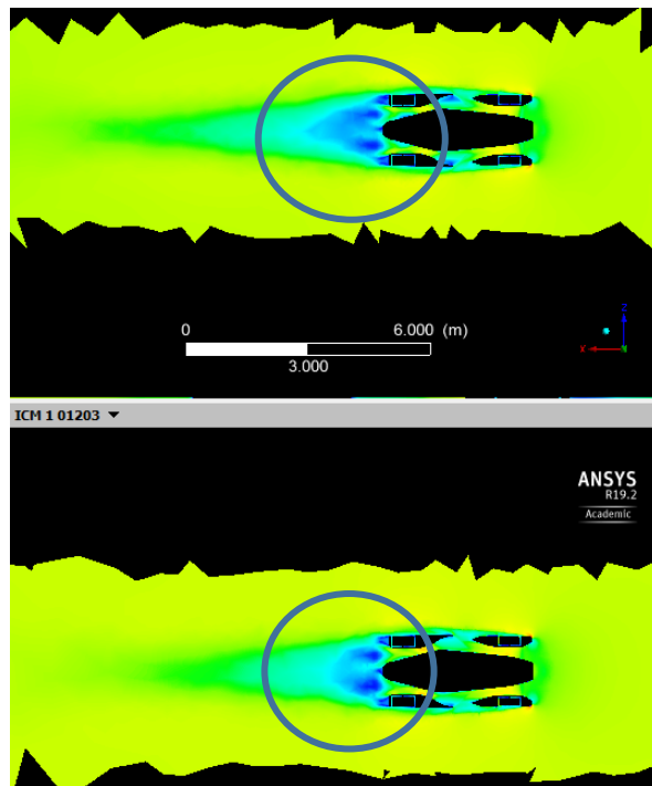
Figure 57 Moving Road and Rotating Wheels comparison MK4
