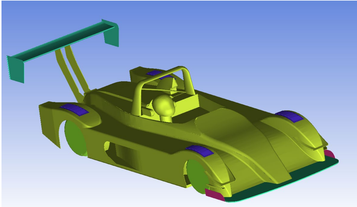
Figure 15 Separated MK1 Model
