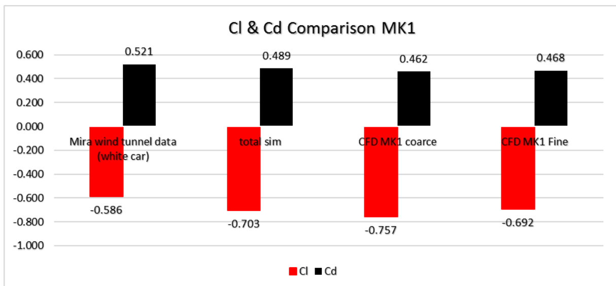
Graph 12 Cl & Cd Comparison MK1
