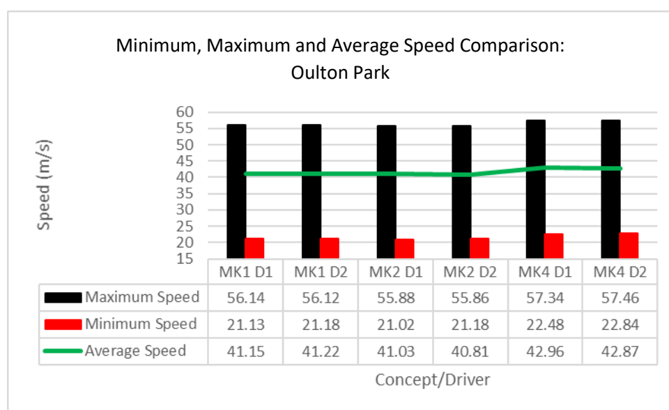
Graph 38 Oulton Park Speed Comparison
