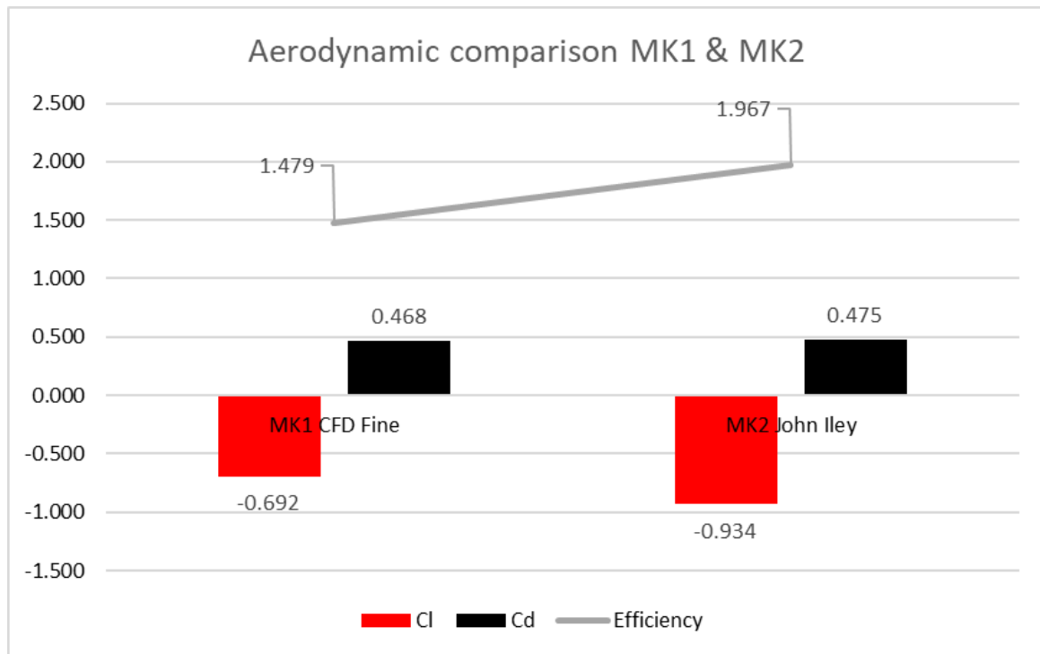
Graph 28 Aerodynamic Comparison MK1 and MK2
