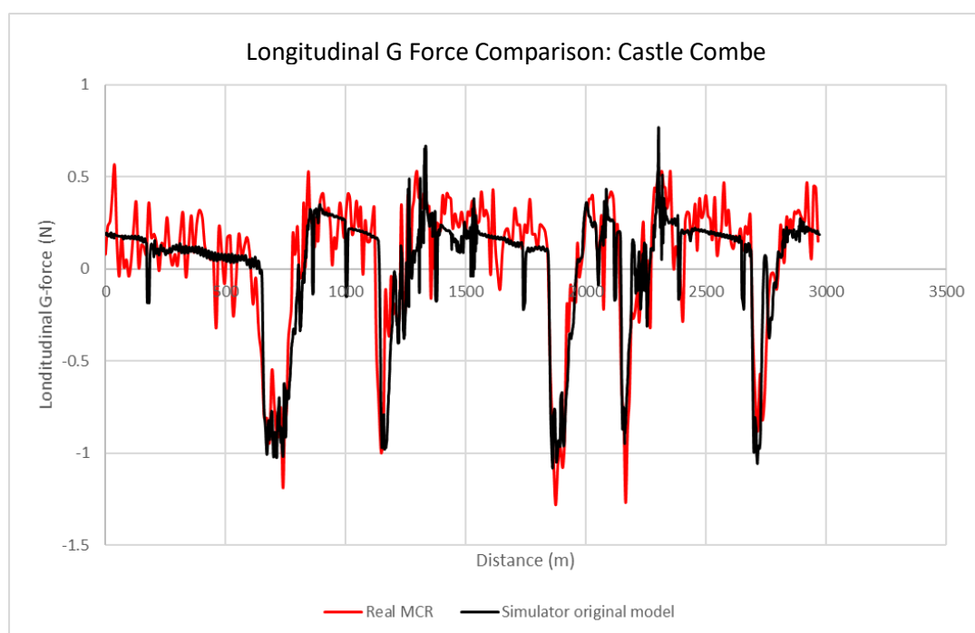
Graph 7 Castle Combe Longitudinal G Force Comparison
