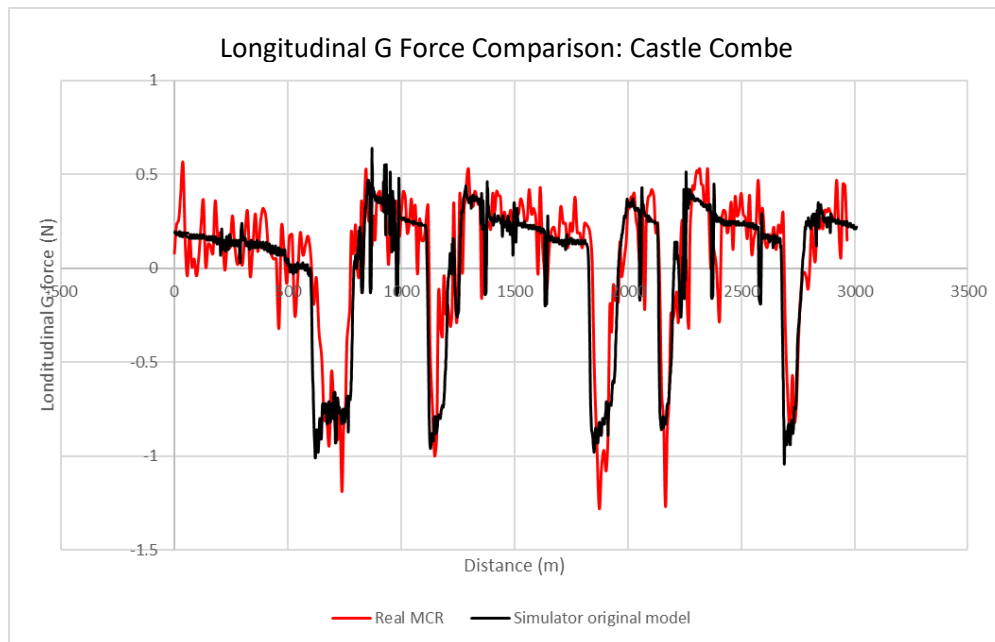
Graph 20 Castle Combe Longitudinal G Force Comparison Updated Mass and Engine
