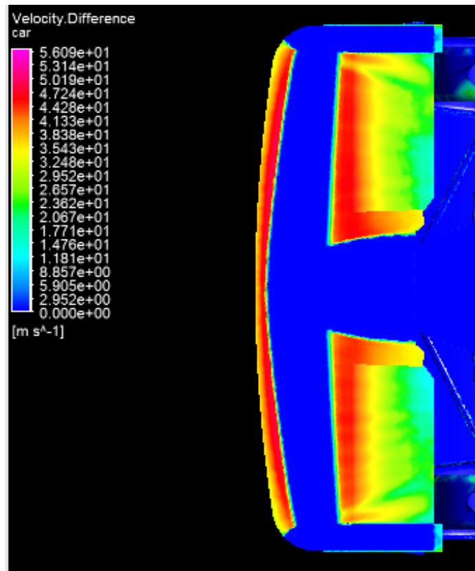
Figure 24 Velocity Contour Case Comparison MK1 and MK2
