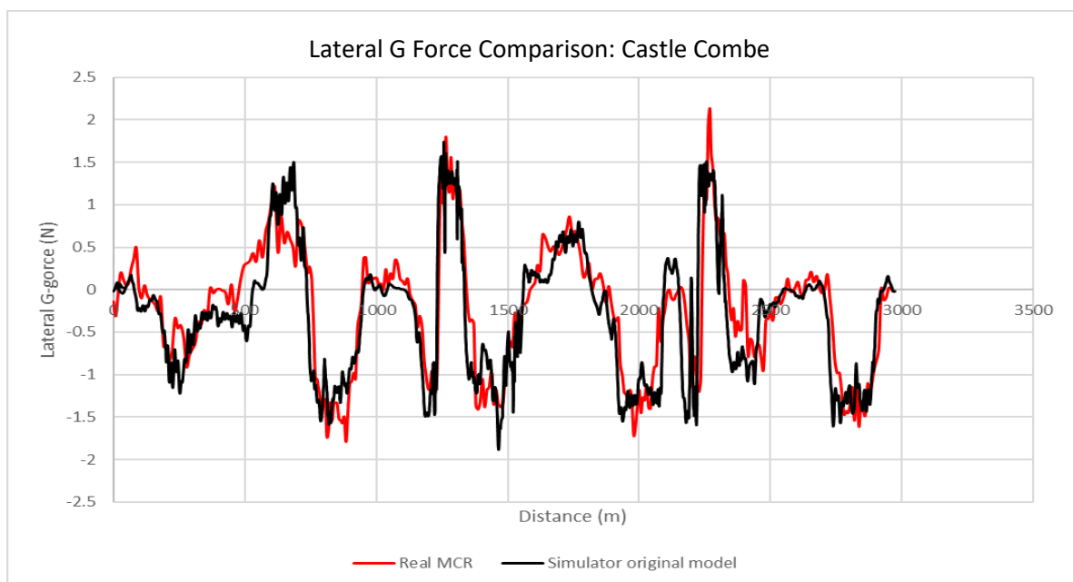
Graph 5 Castle Combe Lateral G Force Comparison
