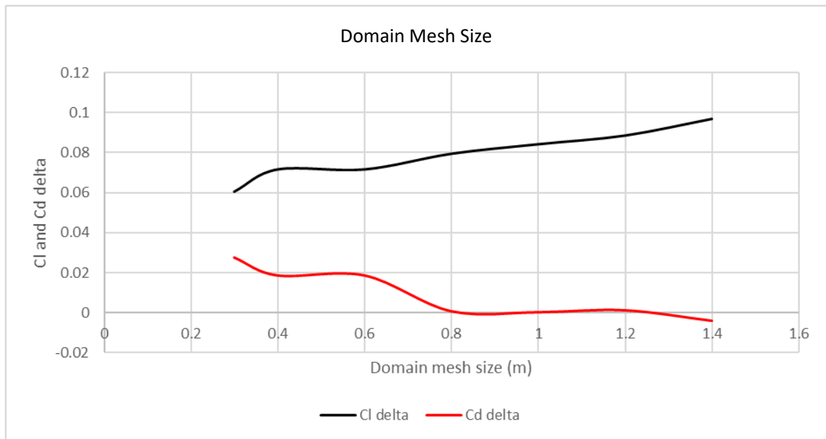
Graph 10 CFD Validation - Domain Mesh Size
