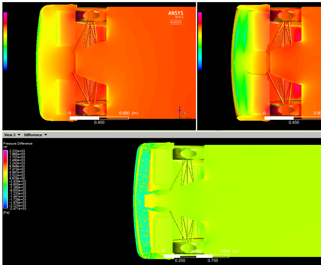
Figure 25 Pressure Contour Lower Surface Case Comparison MK1 and MK2
