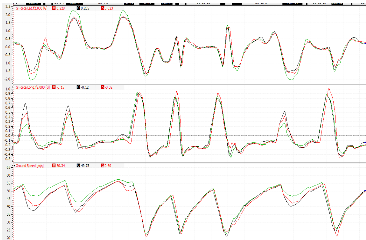
Figure 38 Oulton Park G Force Comparison
