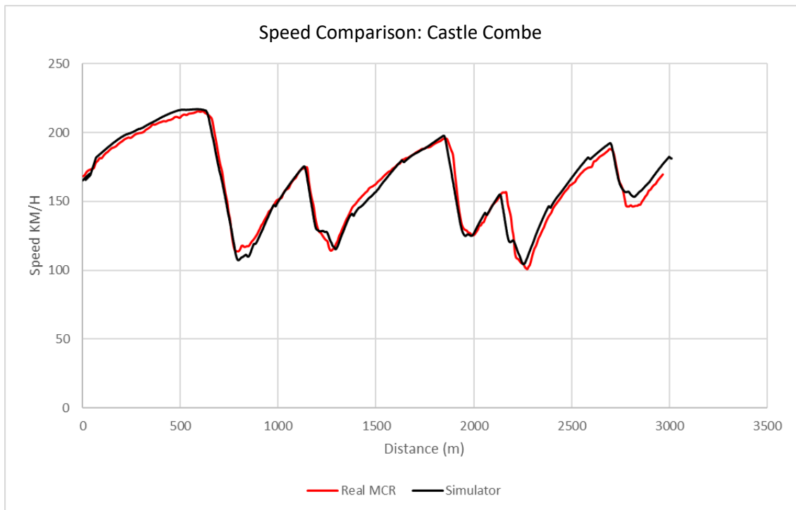
Graph 24 Castle Combe Speed Comparison Updated Braking Force
