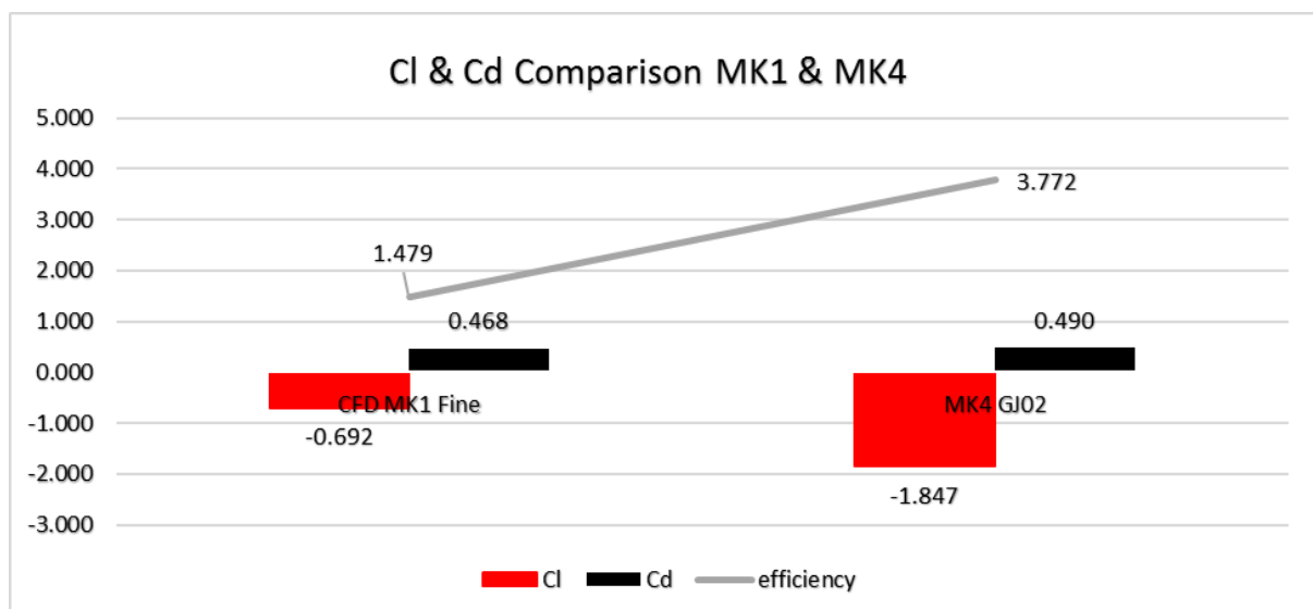
Graph 32 Aerodynamic Comparison MK1 and MK4
