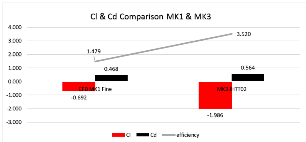
Graph 30 Aerodynamic Comparison Mk1 and MK3
