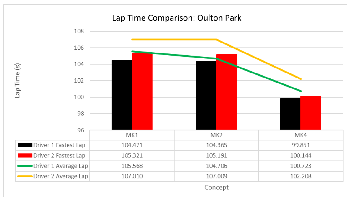
Graph 36 Oulton Park Lap Time Comparison
