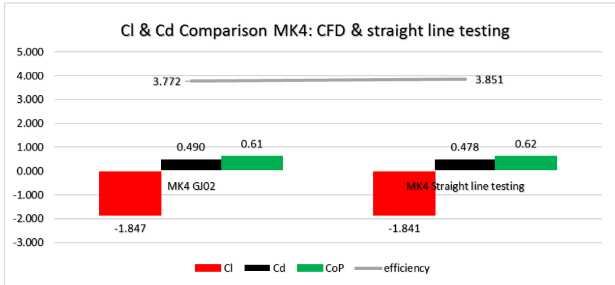
Graph 33 MK4 Aerodynamic Validation
