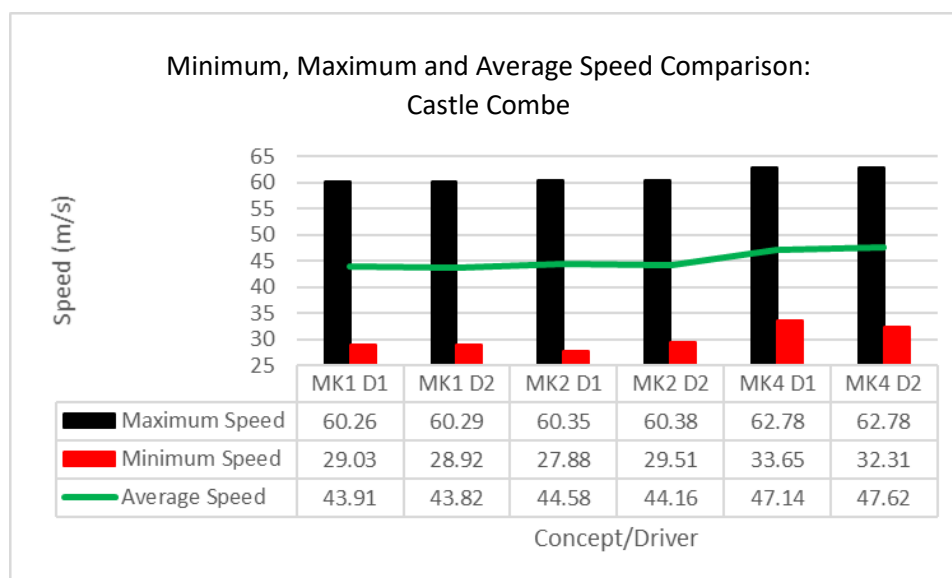
Graph 37 Castle Combe Speed Comparison
