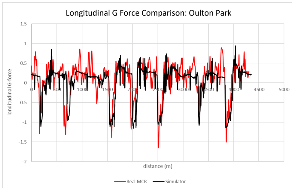
Graph 23 Oulton Park Longitudinal G Force Comparison Increased Braking Force
