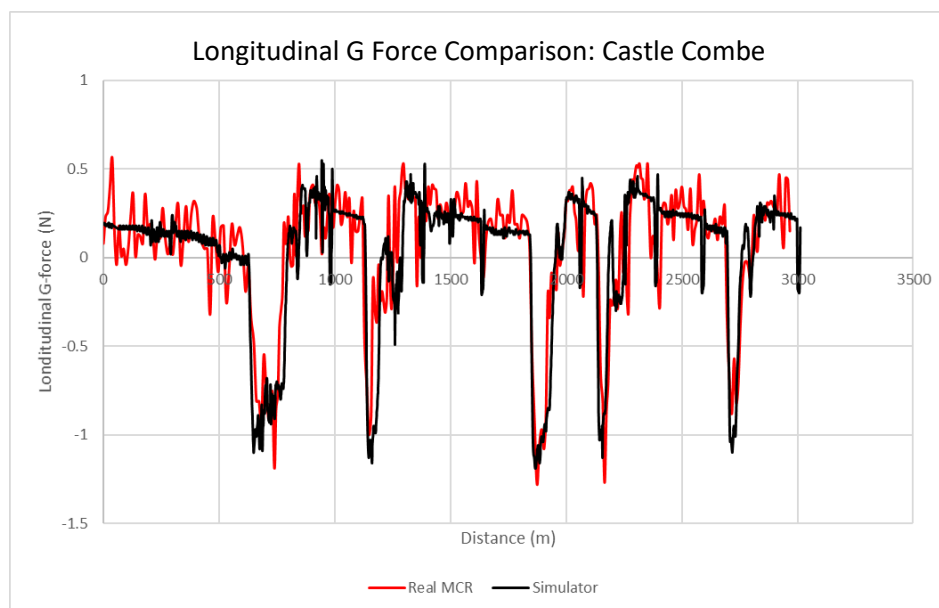
Graph 22 Castle Combe Longitudinal G Force Comparison Increased Braking Force
