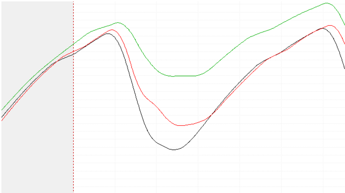
Figure 32 Oulton Park Speed Comparison - Turn One
