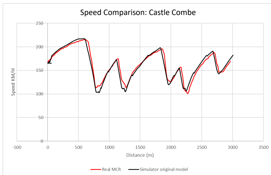
Graph 18 Castle Combe Speed Comparison Updated Mass and Engine
