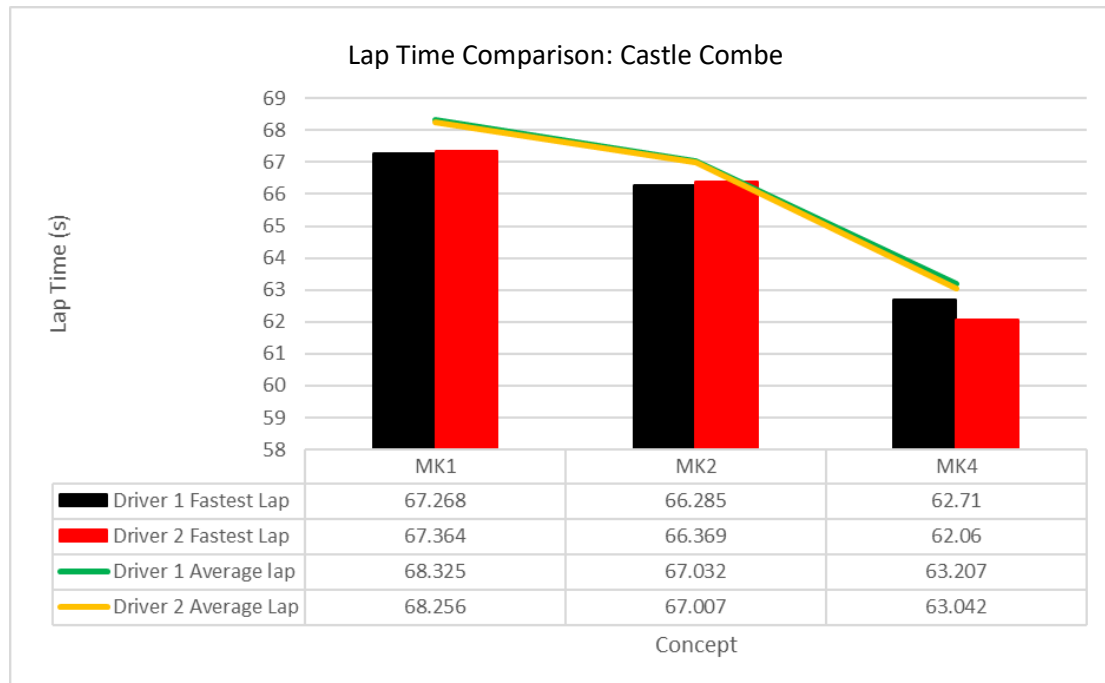
Graph 35 Castle Combe Lap Time Comparison
