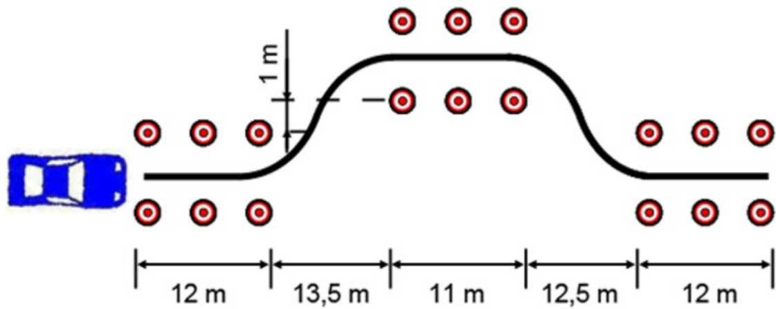
Figure 55 Lane Change Manoeuvre Layout
