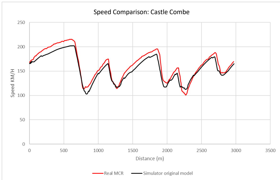
Graph 3 Castle Combe Original Simulation Model Speed Comparison
