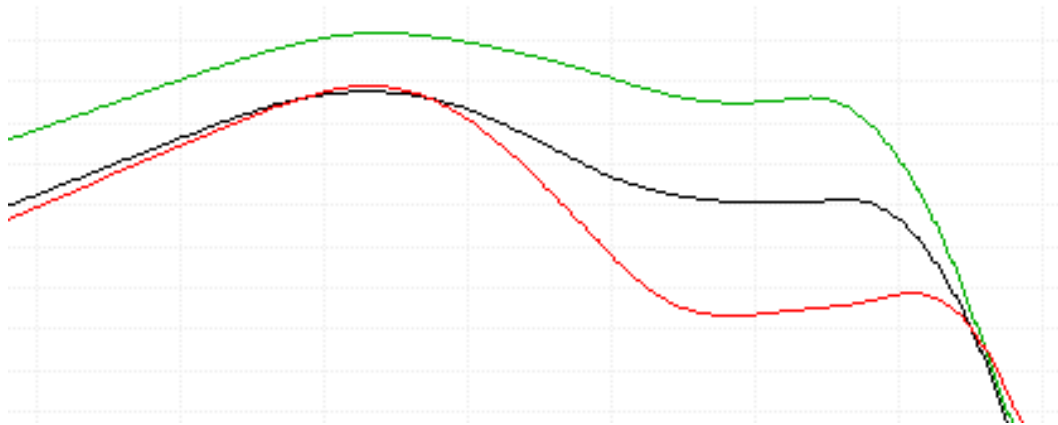
Figure 34 Oulton Park Speed Comparison - Turn Four
