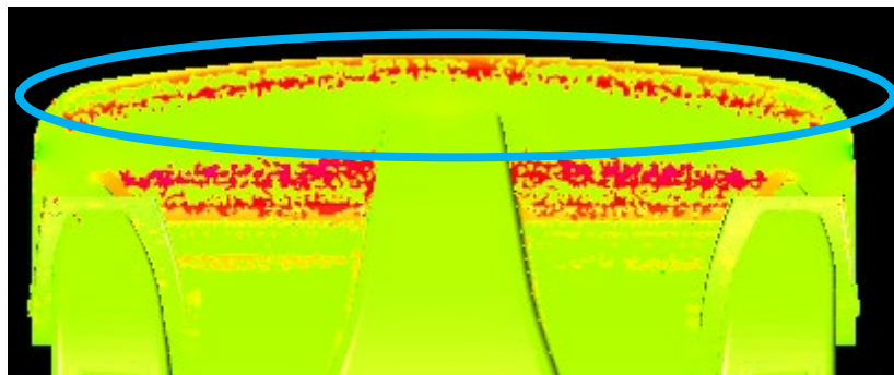
Figure 26 Pressure Contour Upper Surface Case Comparison MK1 and MK2
