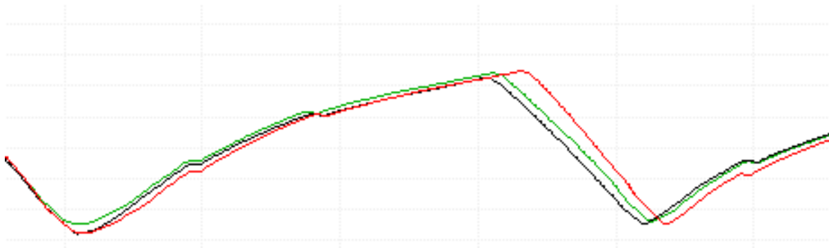
Figure 43 Oulton Park Later Braking Example
