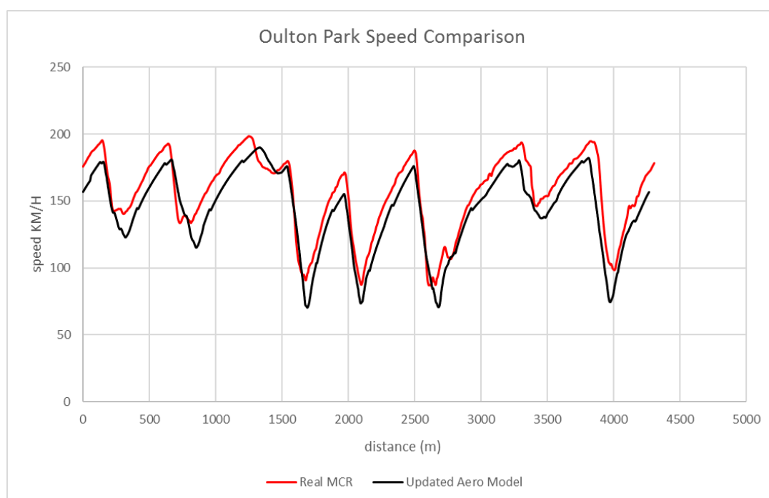
Graph 14 Oulton Park Updated Aerodynamism Speed Comparison
