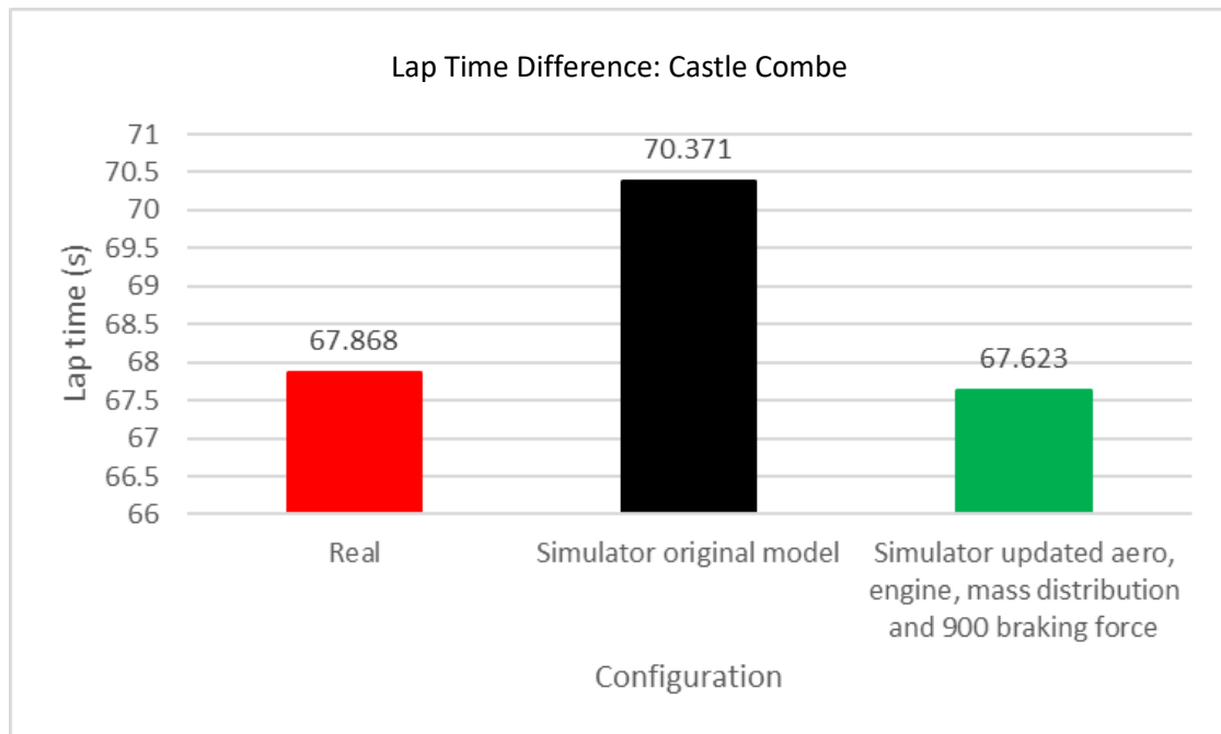
Graph 26 Castle Combe Lap Time Comparison Updated Braking Force
