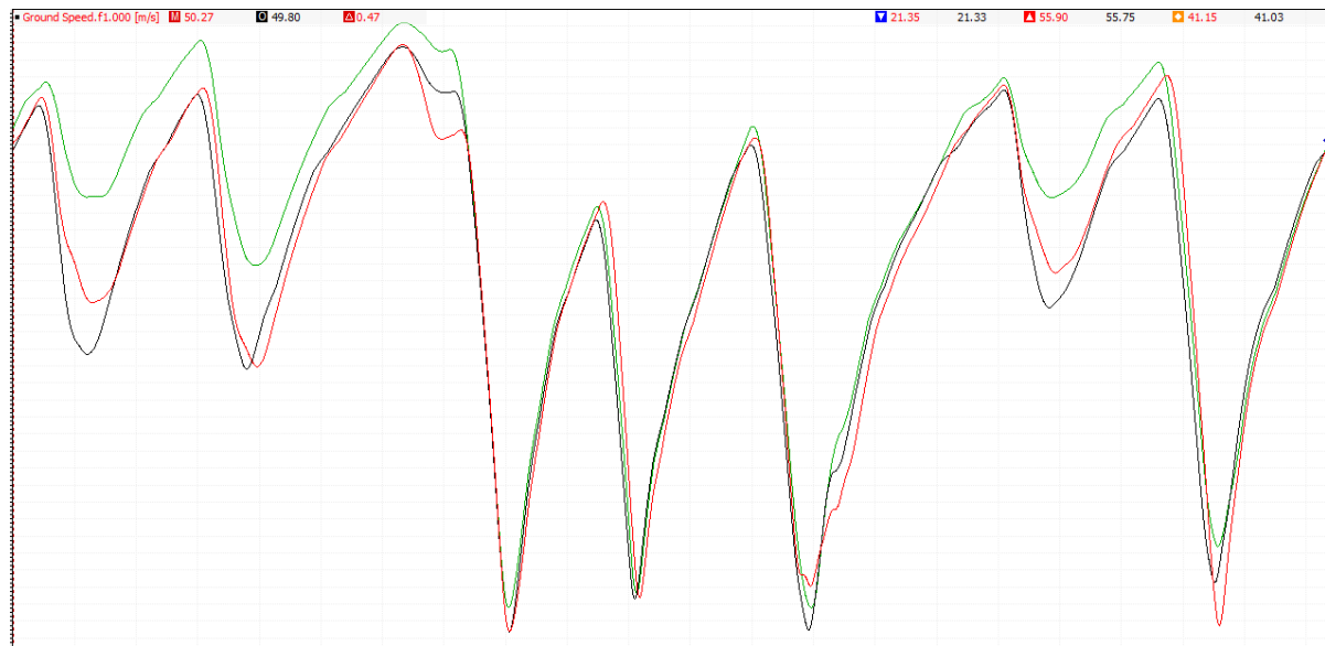
Graph 39 Oulton Park Speed Comparison
