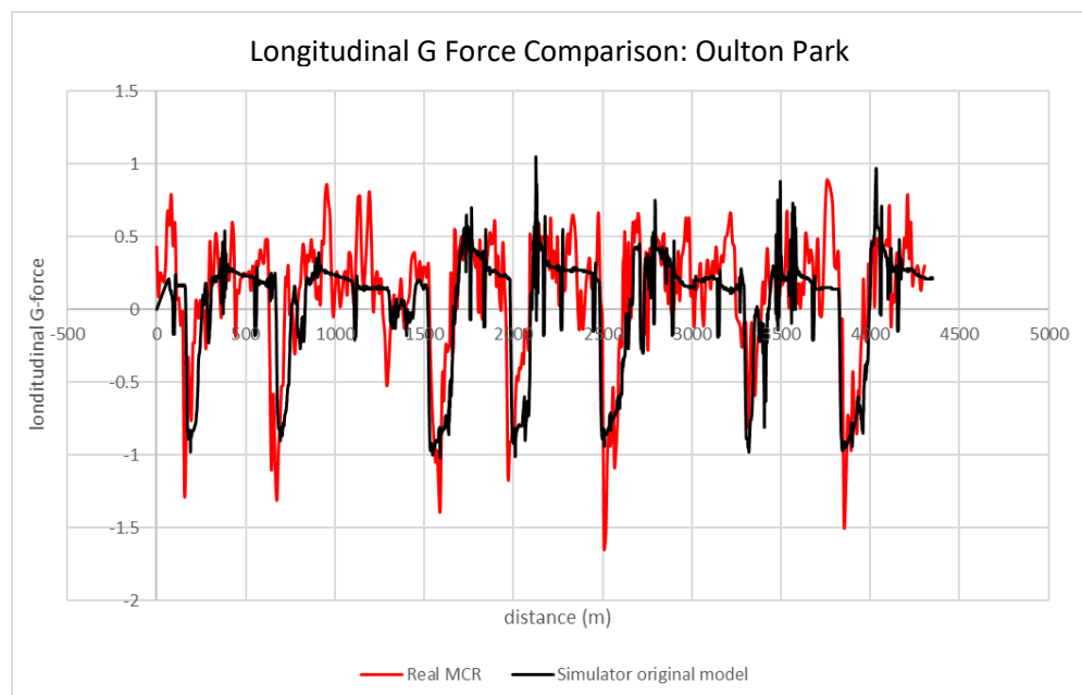
Graph 21 Oulton Park Longitudinal G Force Comparison Updated Mass and Engine
