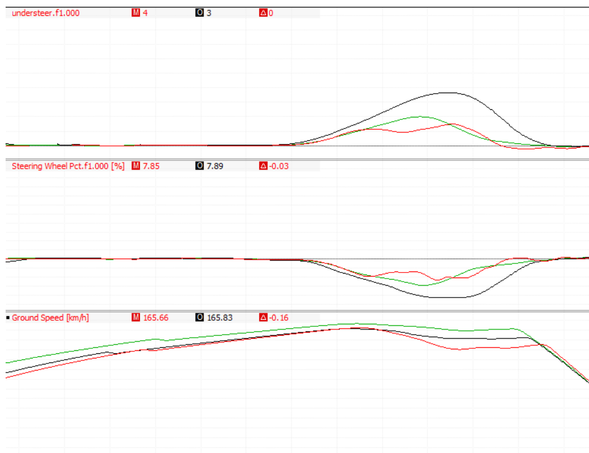
Figure 52 Oulton Park Understeer Comparison - Turn Four
