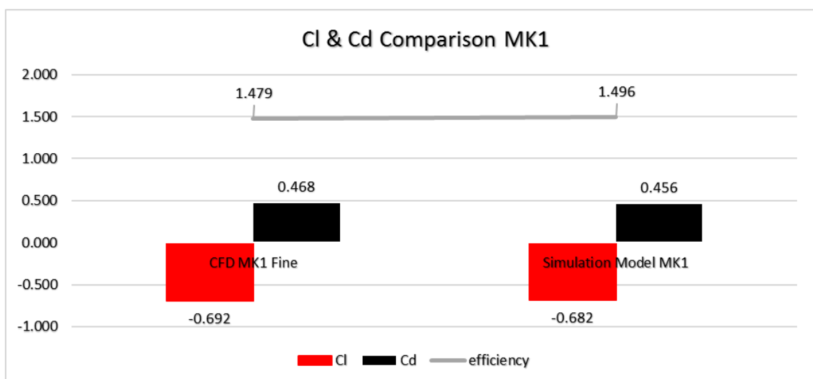
Graph 13 Simulation Aerodynamic Validation MK1
