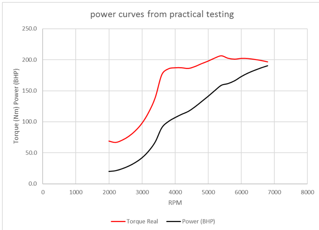
Graph 16 Power Curves from Practical Testing
