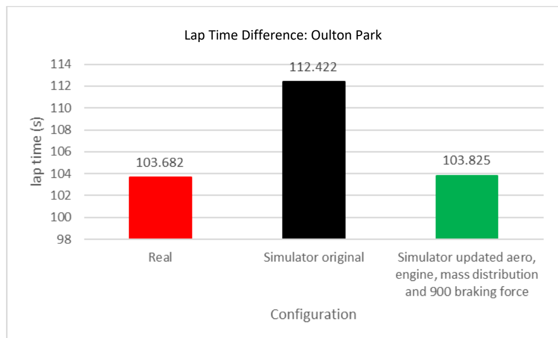
Graph 27 Oulton Park Lap Time Comparison Updated Braking Force
