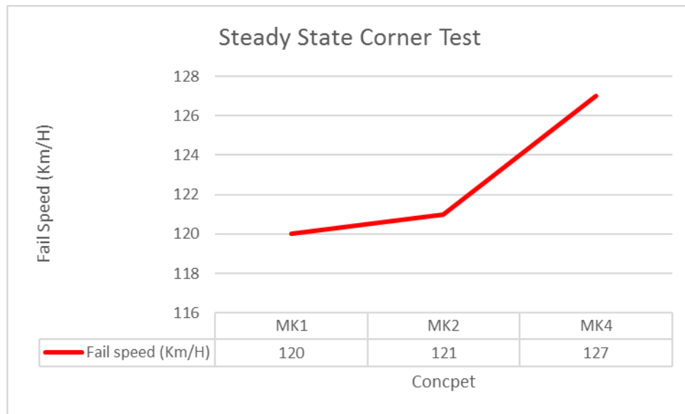
Graph 41 Steady State Corner Results
