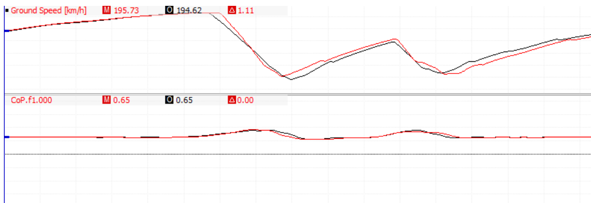
Figure 47 Slight Variation of CoP with Speed
