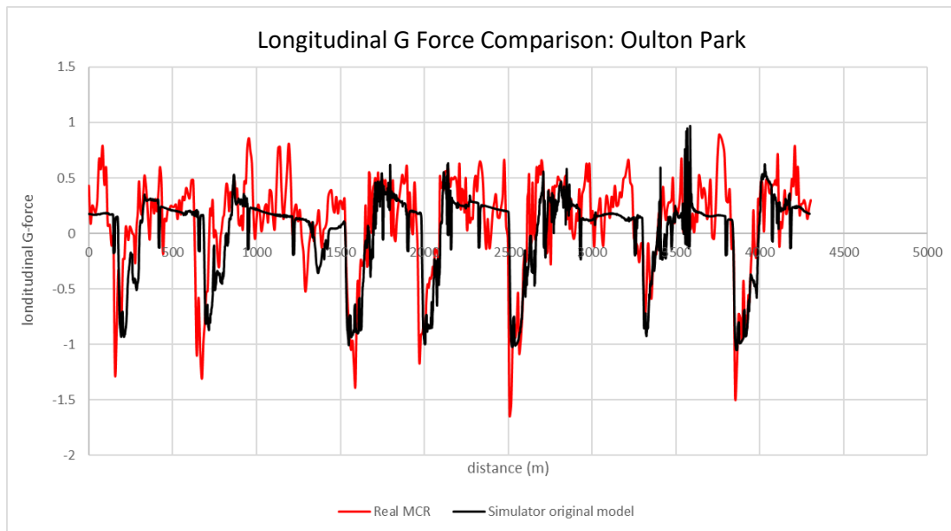
Graph 8 Oulton Park Longitudinal G Force Comparison
