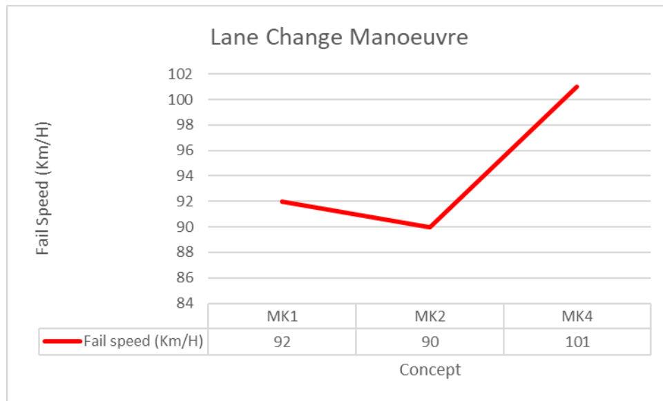
Graph 40 Lane Change Manoeuvre Results
