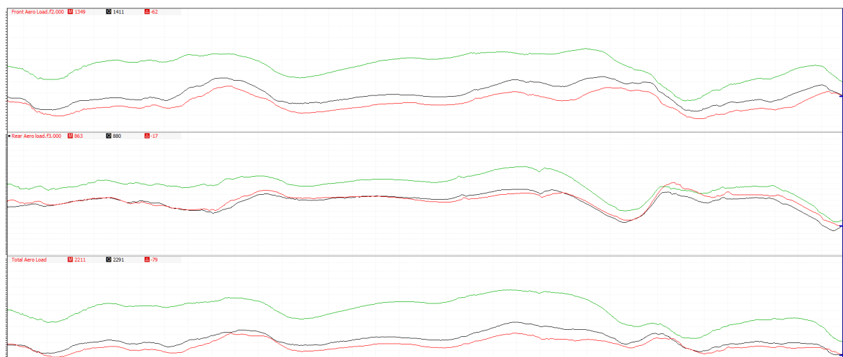
Figure 45 Oulton Park Aerodynamic Load Comparison
