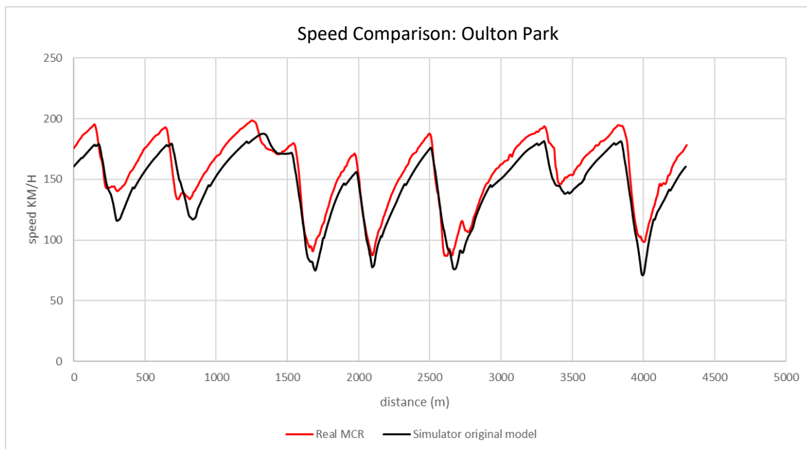
Graph 4 Oulton Park Original Simulation Model Speed Comparison
