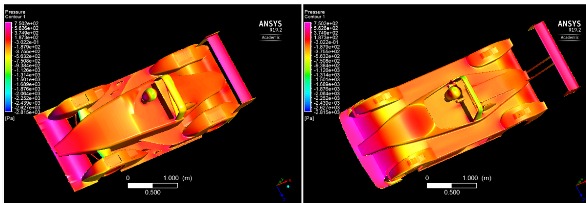
Figure 28 Pressure Contour Comparison Upper Surface MK1 and MK3
