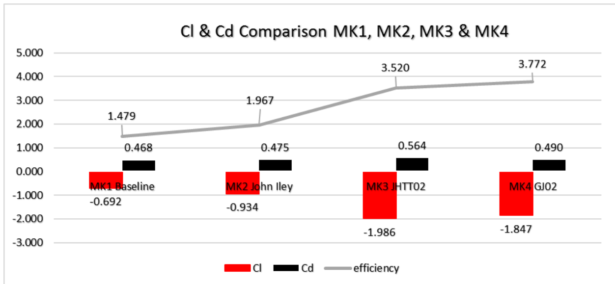
Graph 34 Aerodynamic Comparison MK1, MK2, MK3 and MK4
