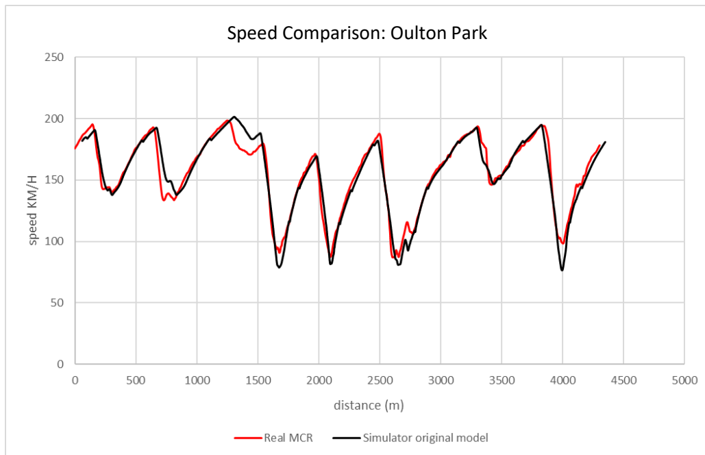
Graph 19 Oulton Park Speed Comparison Updated Mass and Engine
