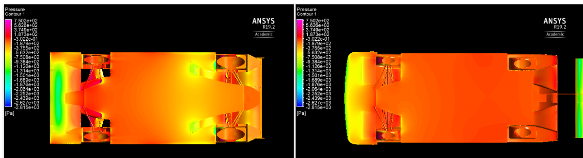
Figure 29 Pressure Contour Comparison Lower Surface MK1 and MK3
