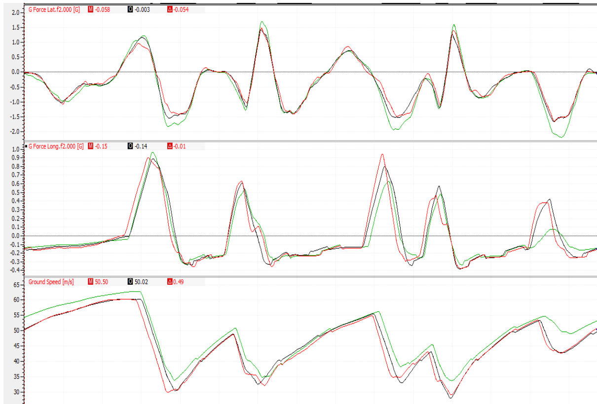
Figure 37 Castle Combe G Force Comparison
