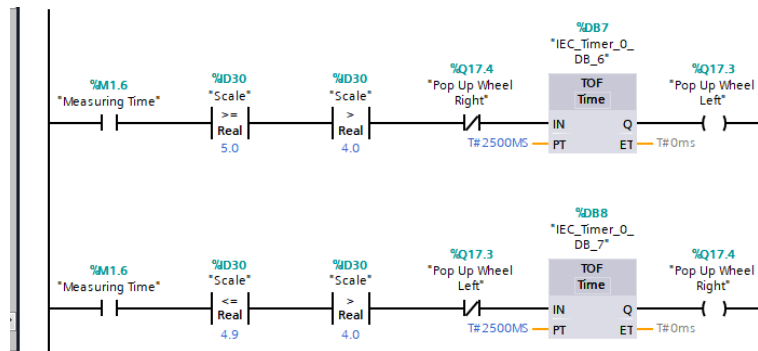
Figure 23 - Network 7B
