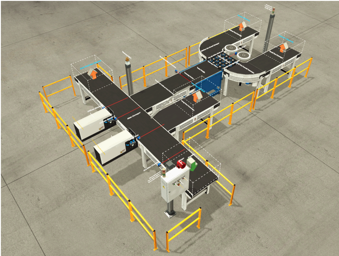
Figure 38 - Entire System
