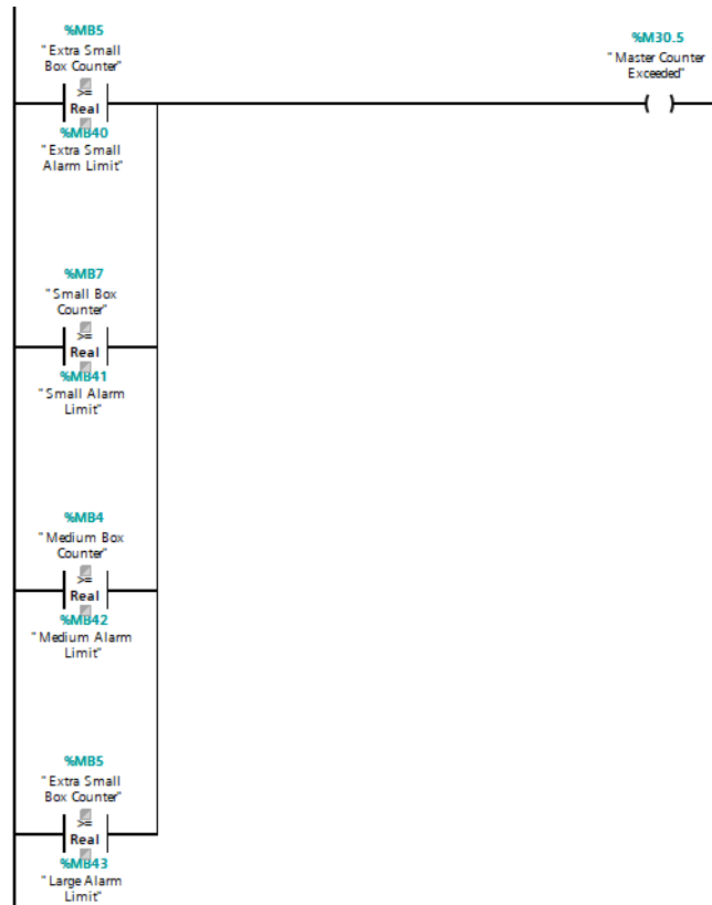
Figure 27 - Network 9B
