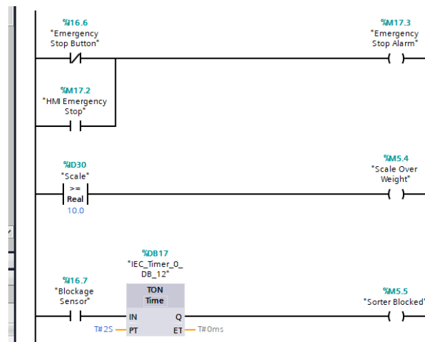
Figure 26 - Network 9A
