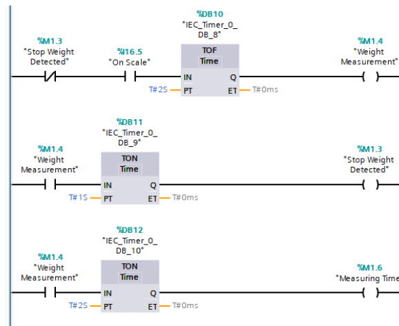
Figure 22 - Network 7A
