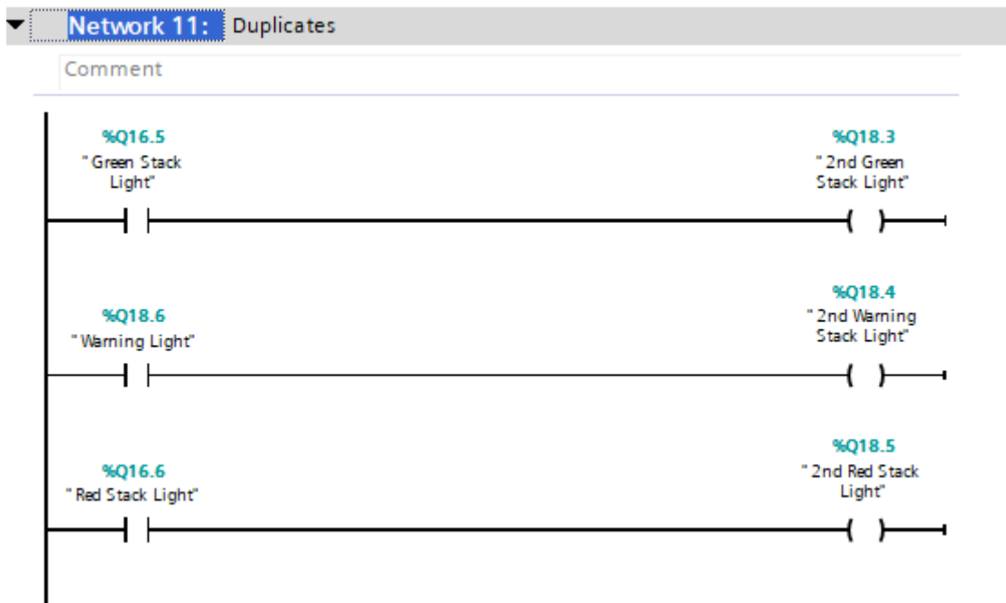
Figure 30 - Network 11
