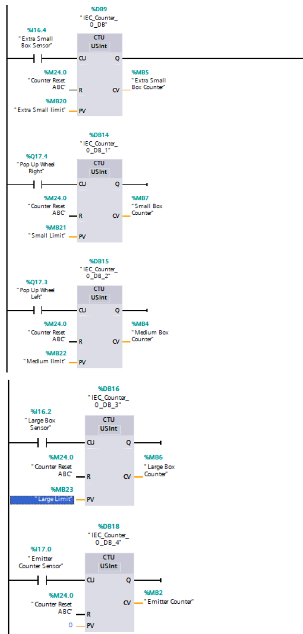
Figure 24 - Network 8A
