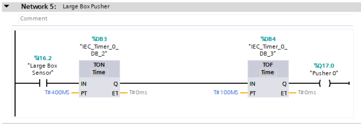
Figure 20 - Network 5
