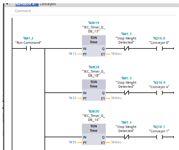
Figure 19 - Network 4
