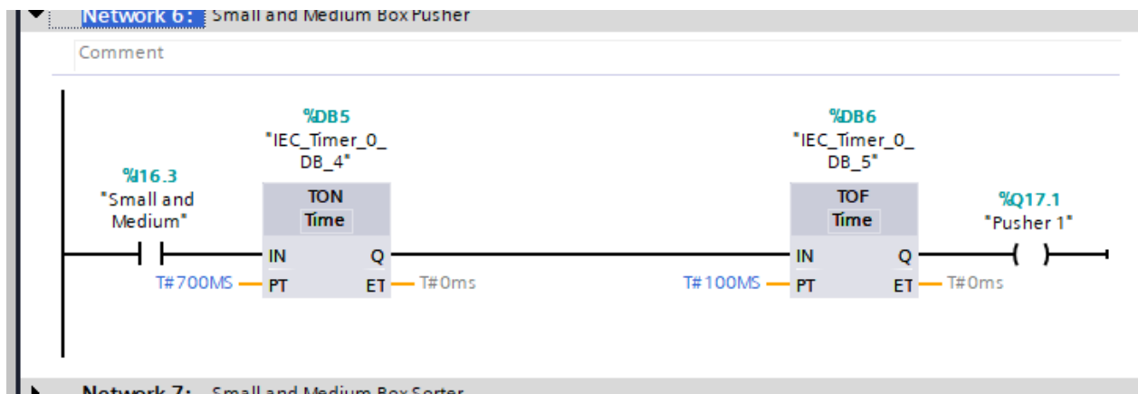
Figure 21 - Network 6
