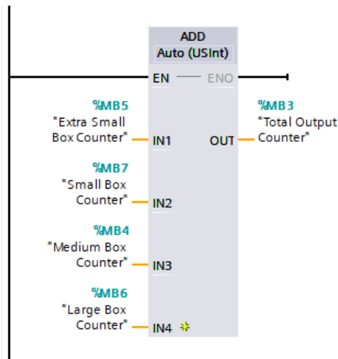
Figure 25 - Network 8B
