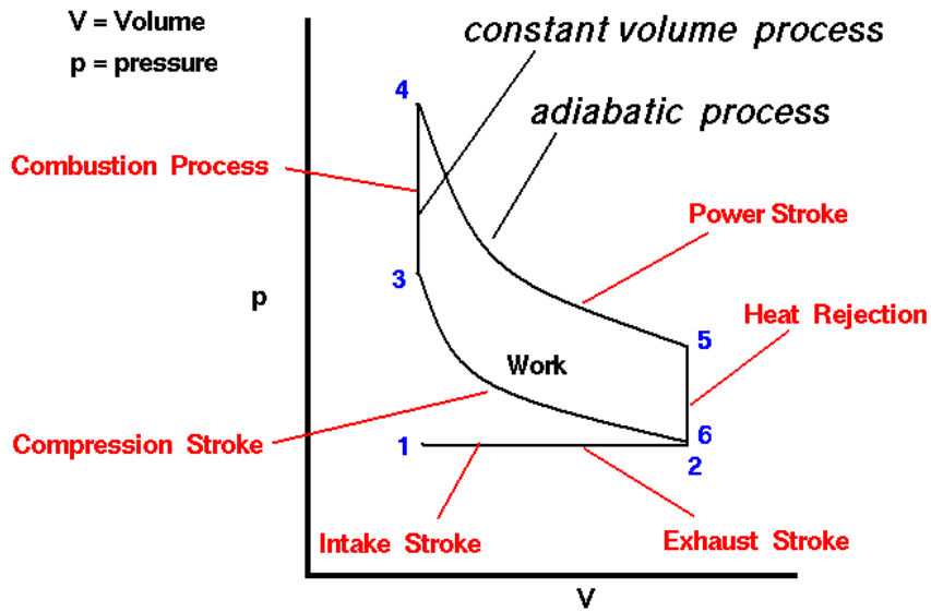
Figure 16 - Ideal Otto Cycle pV diagram from Nasa [21].
