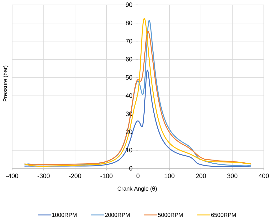
Figure 10 - Pressure vs Crank Angle across the rev range for Ford Fox engine.
