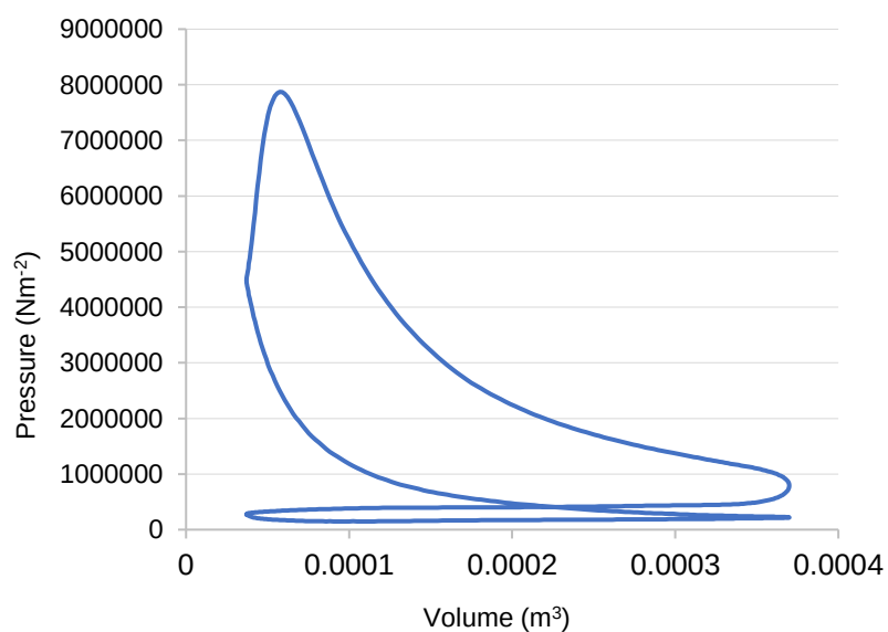
Figure 12 - Pressure vs Volume Graph for Ford Fox engine at 6000rpm.
