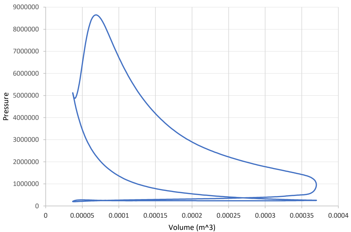
Figure 17 - Real pV diagram from Ford Fox engine at 3500rpm.
