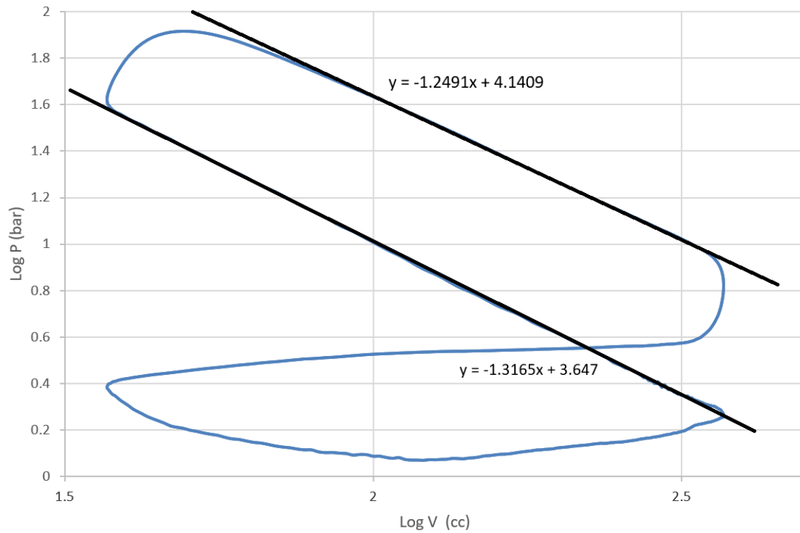
Figure 18 - Log P vs Log V graph for 6500rpm for Ford Fox engine.
