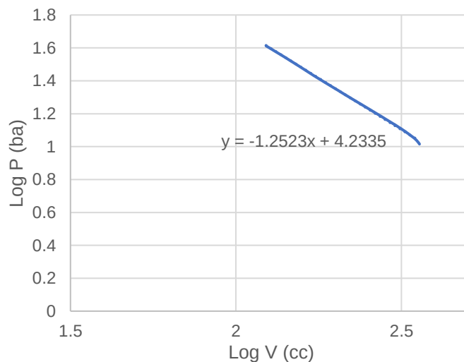
Figure 28 - Expansion stroke Log P/Log V diagram for Ford Fox engine at 6000rpm.
