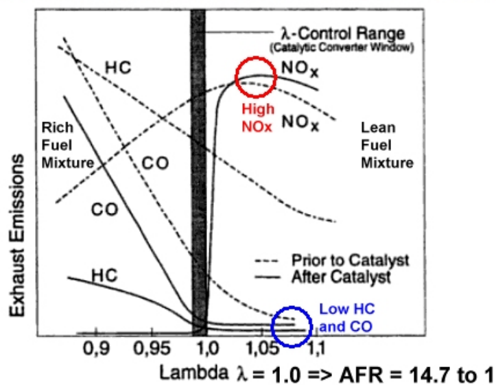
Figure 3 - Emission Curve against \lambda
