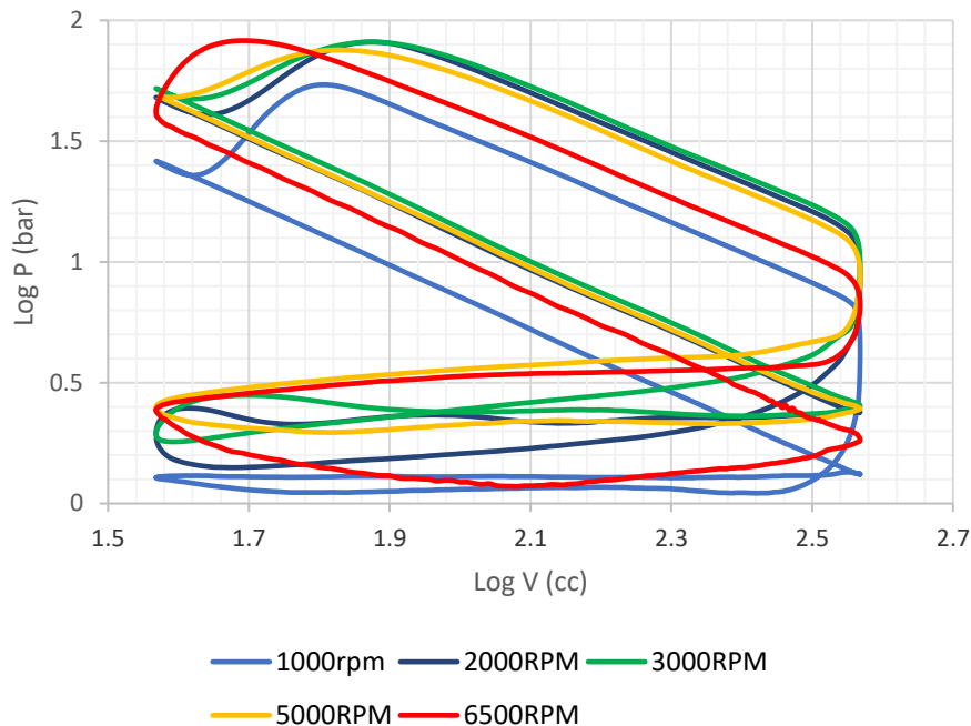
Figure 22 - Log P/LogV diagrams across the rev range for the Ford Fox engine.
