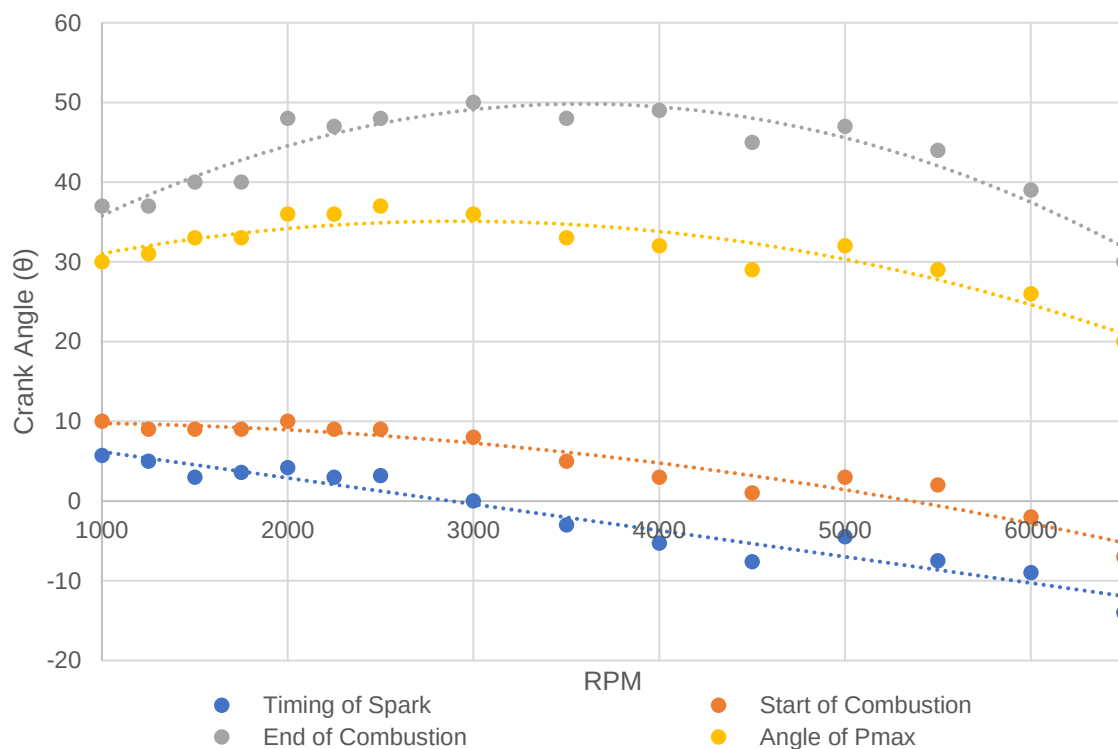
Figure 29 - Combustion timings for the Ford Fox engine.
