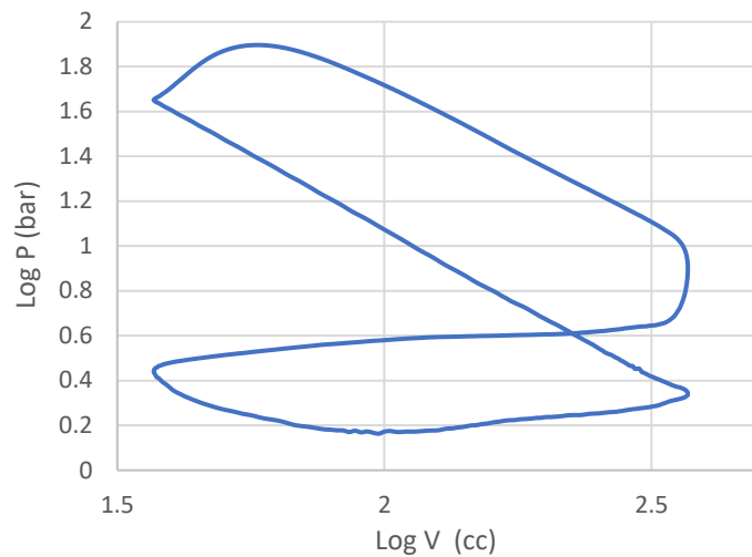
Figure 27 - Figure 6 Log P/Log V diagram for Ford Fox engine at 6000rpm.
