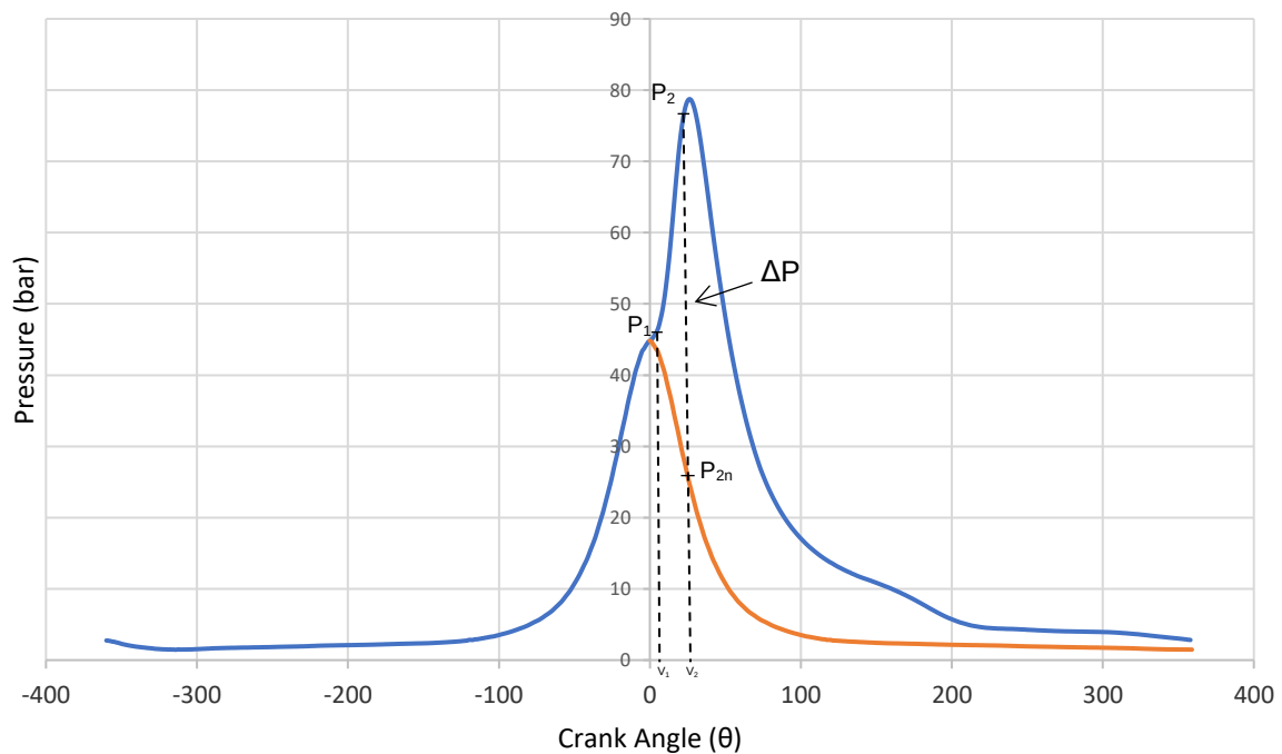
Figure 30 - Graph depicting change in pressure due to combustion for Ford Fox engine at 6000rpm.
