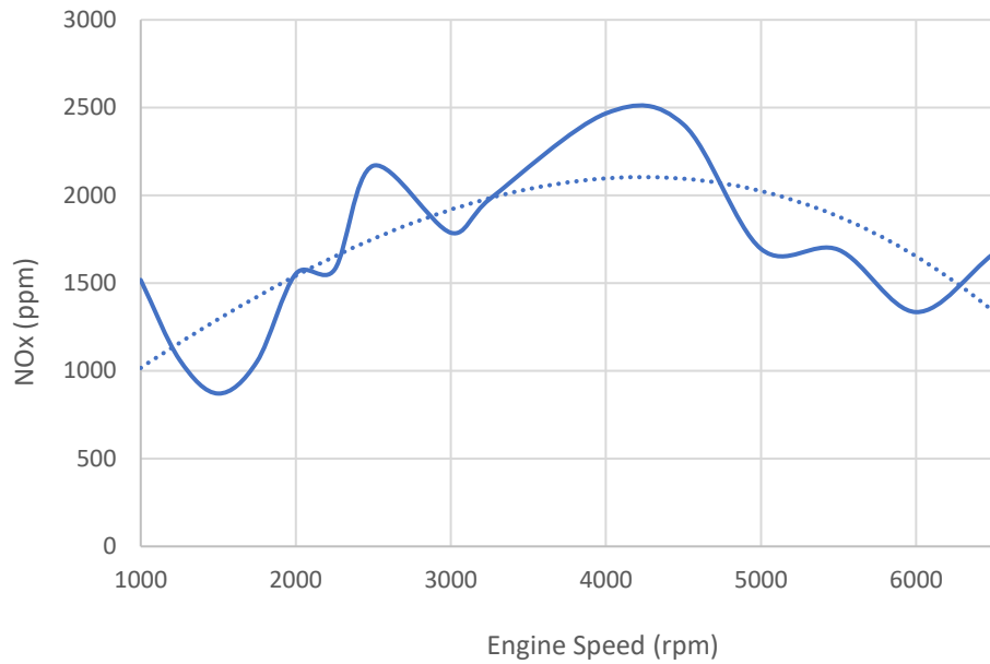
Figure 2 - NOx output at full load, throughout the rev range from engine test data on Ford Fox engine.
