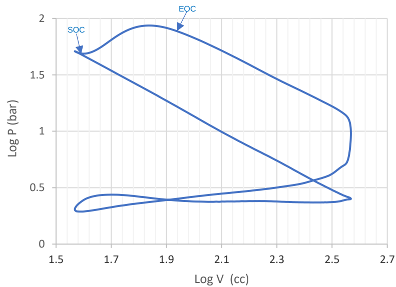
Figure 20 - Log P/Log V graphs from Ford Fox engine at 3500rpm.
