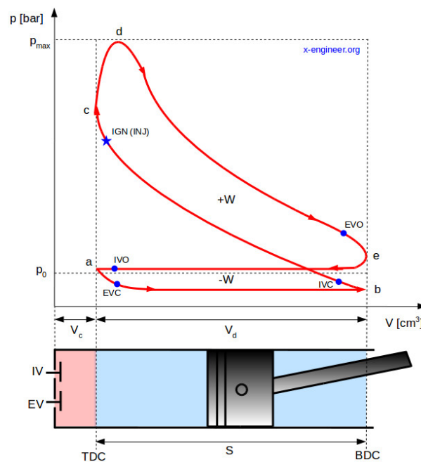
Figure 11 - x-engineer pV Diagram.
