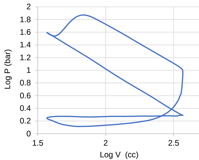
Figure 24 - Log P/Log V diagram for Ford Fox engine at 1500rpm.
