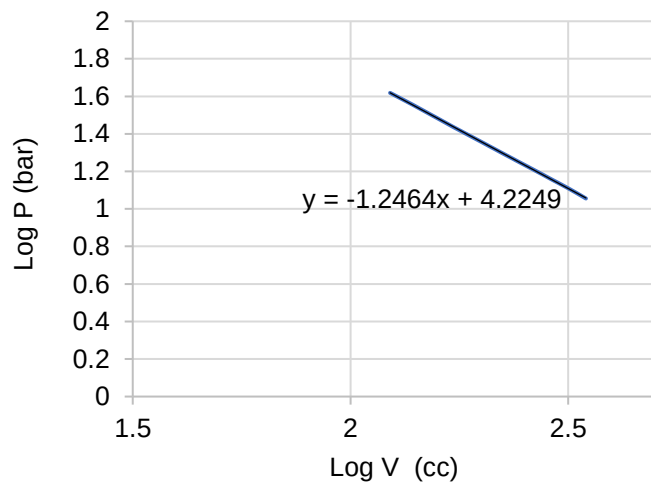
Figure 25 - Expansion stroke Log P/Log V diagram for Ford Fox engine at 1500rpm.
