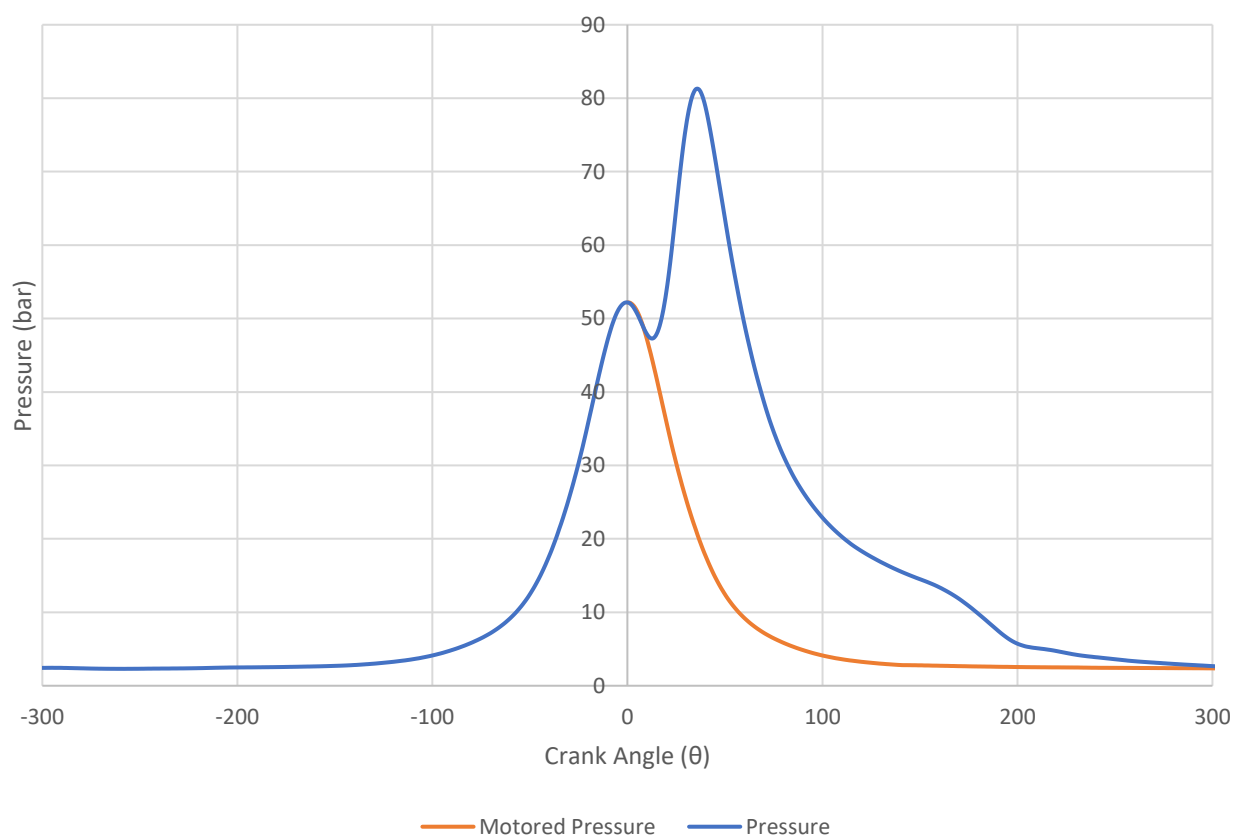
Figure 19 - Pressure/Crank Angle graph for 3000rpm from the Ford Fox data.
