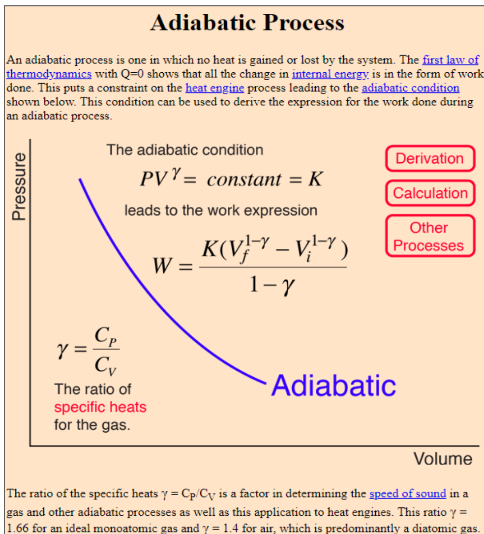
Figure 37 - Adiabatic Process from [#]
