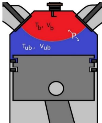
Figure 32 - Two-Zone Model.
