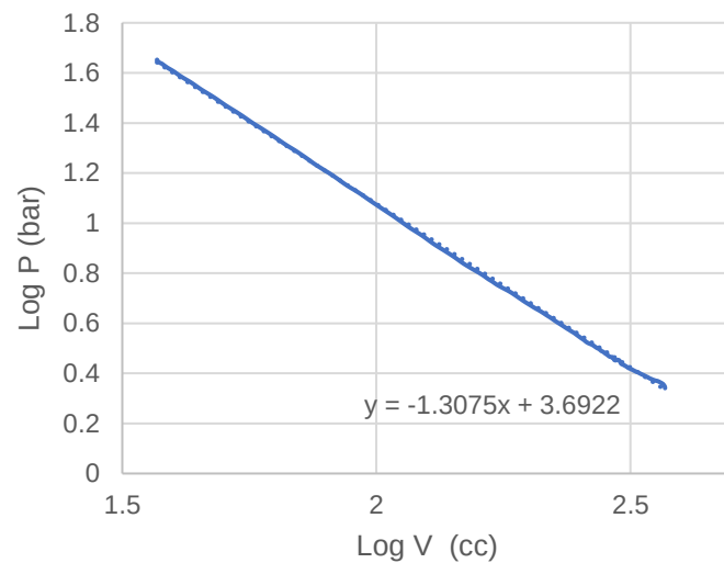
Figure 26 - Compression part of Log P/Log V diagram for Ford Fox engine at 6000rpm.
