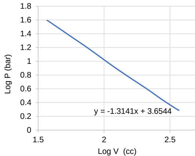
Figure 23 - Compression part of Log P/Log V diagram for Ford Fox engine at 1500rpm.
