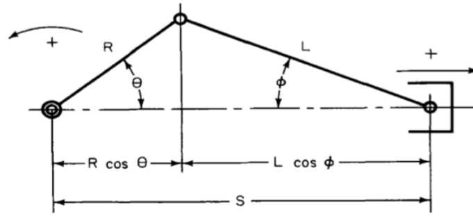
Figure 6 - Piston, Rod and Crank schematics from C F Taylor.
