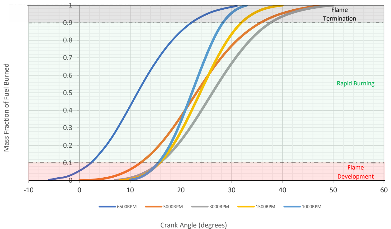
Figure 31 - Mass Fraction Burned vs Crank Angle across the rev range for the Ford Fox engine.
