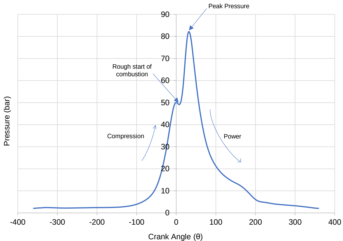
Figure 9 - Pressure vs Crank Angle graph from Ford Fox engine at 3500rpm.
