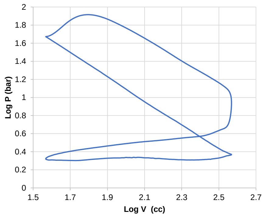
Figure 15 - Log pV diagram from Ford Fox engine at 4500rpm.
