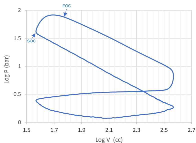
Figure 21 - Log P/Log V graphs from Ford Fox engine at 6500rpm.
