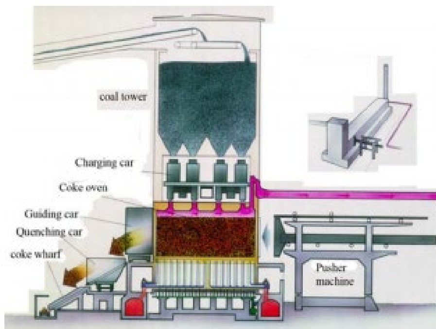
Figure 13 - Diagram of a typical by-product furnace (Hilding, 2005)
