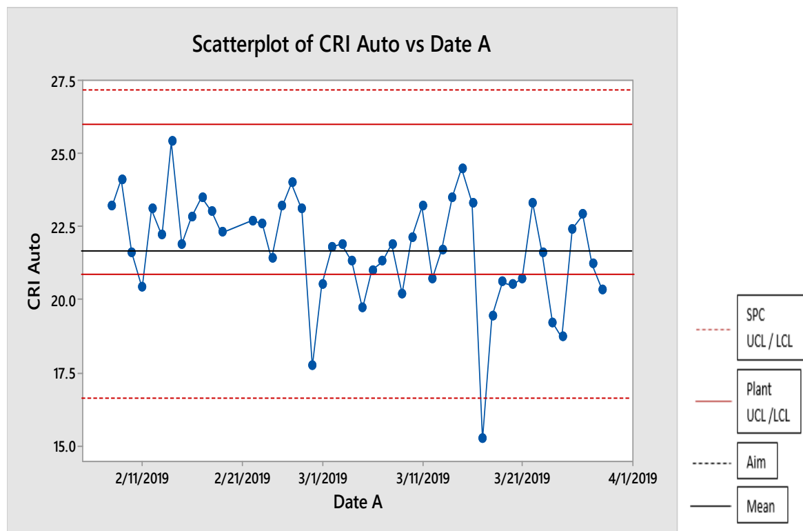
Figure 60 – SPC control chart of the CSR results from coke sampled from the autosampler
