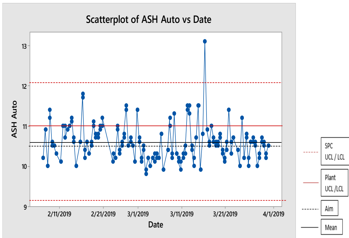
Figure 66 – SPC control chart of the ash results from coke sampled from the autosampler
