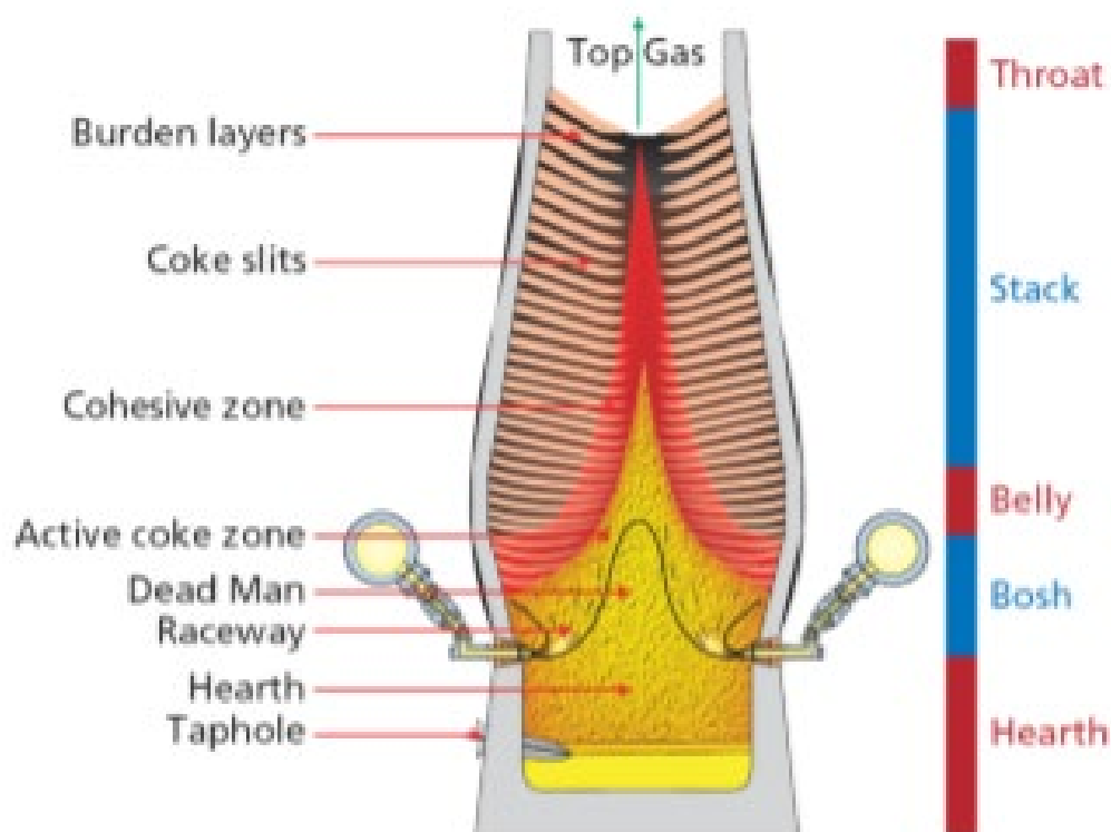
Figure 3 - The blast furnace (Geerdes, et al., 2009)
