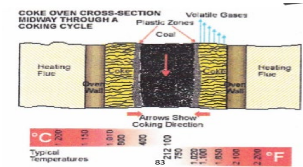
Figure 14 - Cross section through a coke oven during a coking cycle (METaL, 2016)
