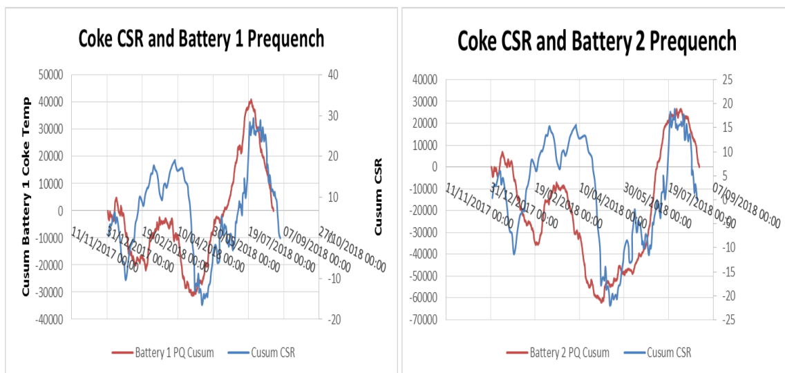
Figure 26 - CuSum graph showing correlation between coke temperatures and CSR (Dickinson, 2018)
