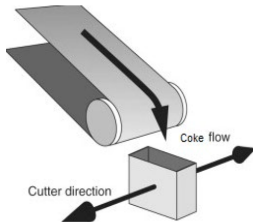
Figure 16 - Diagrammatic representation of falling stream sampling (Membrey, 2013)
