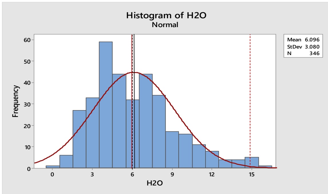
Figure 46 – Histogram and normal distribution of the moisture results between October 2018 and January 2019
