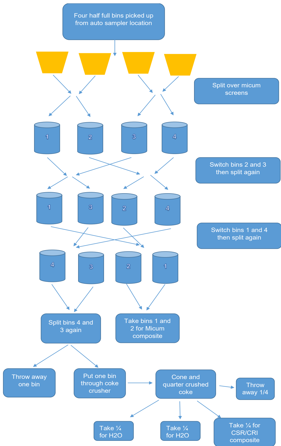
Figure 38 - The coke mixing process implemented for use after the autosampler installation (Waters, 2018)
