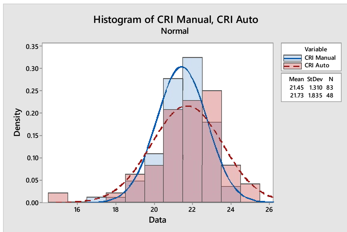
Figure 61 – Histogram and normal distribution comparison of CRI results sampled manually and with the autosampler
