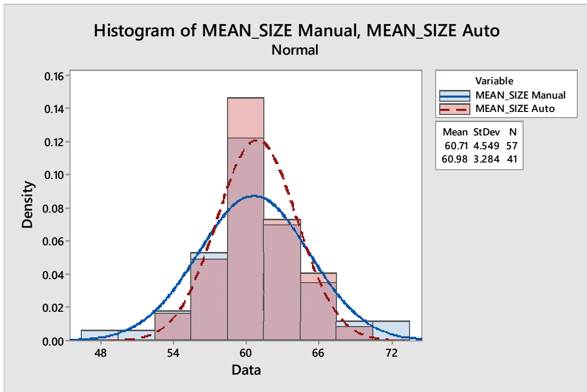
Figure 70 – Histogram and normal distribution comparison of mean size results sampled manually and with the autosampler
