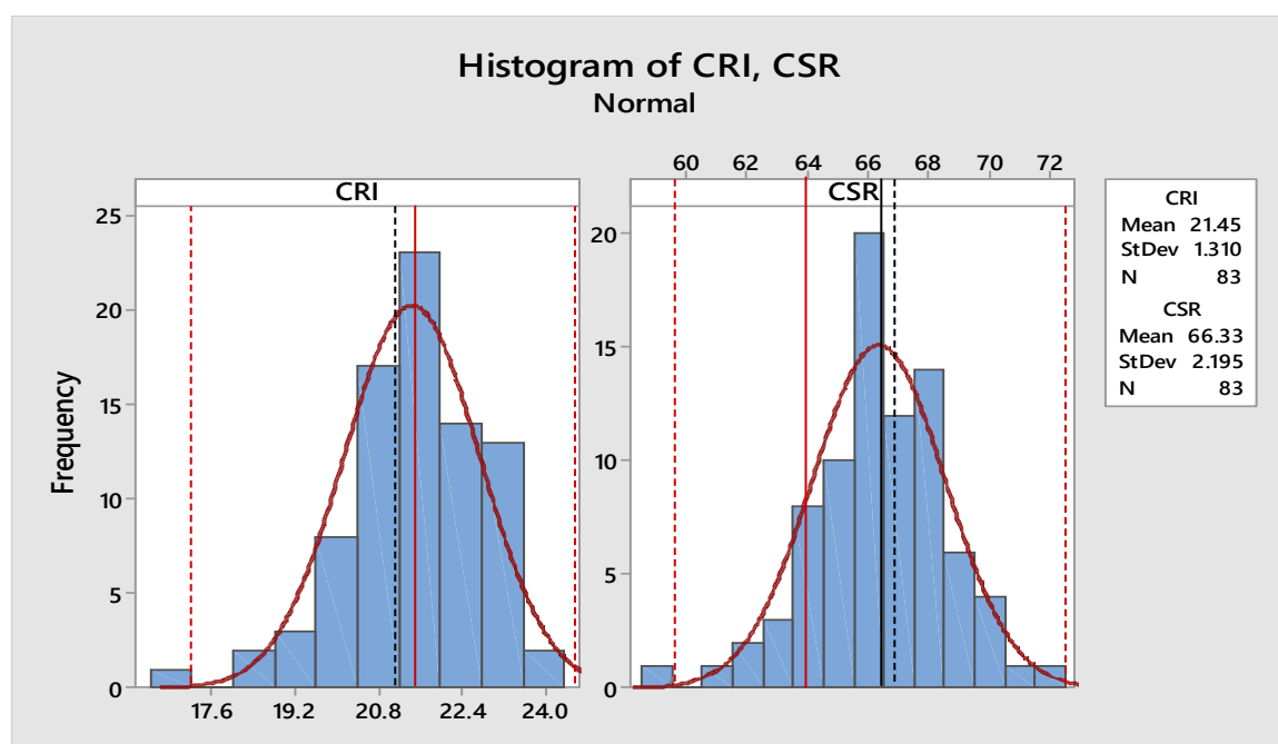
Figure 43 – Histogram and normal distribution of CSR and CRI results between October 2018 and January 2019
