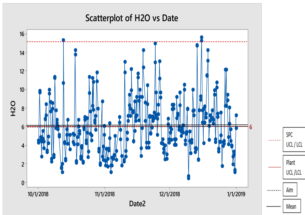
Figure 45 – SPC control chart of the moisture results between October 2018 and January 2019
