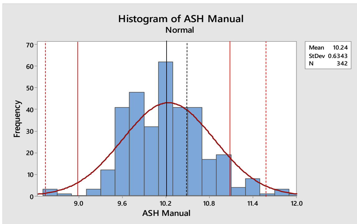
Figure 49 – Histogram and normal distribution of the ash results between October 2018 and January 2019
