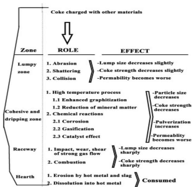
Figure 5 - The degradation process of coke in a blast furnace (Li, et al., 2014)
