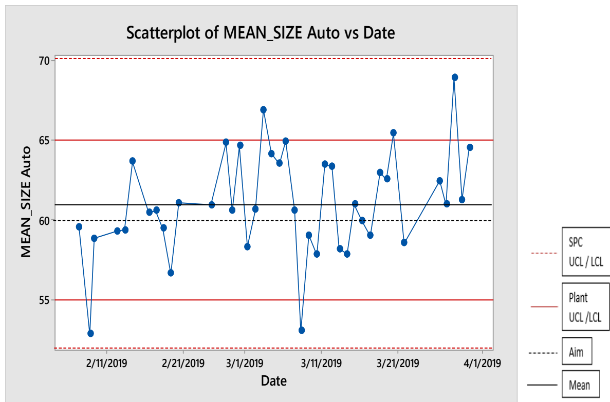
Figure 69 – SPC control chart of the mean size results from coke sampled from the autosampler
