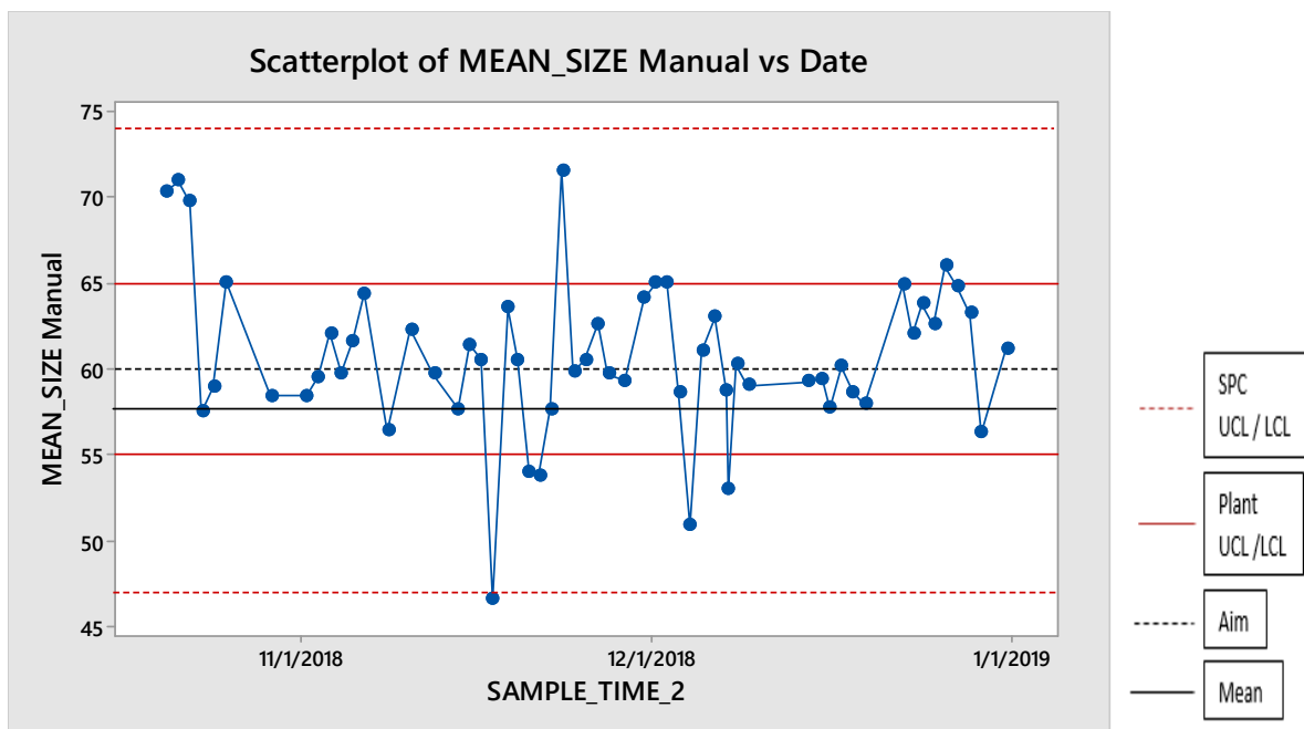
Figure 51 – SPC control chart of the mean size results between October 2018 and January 2019
