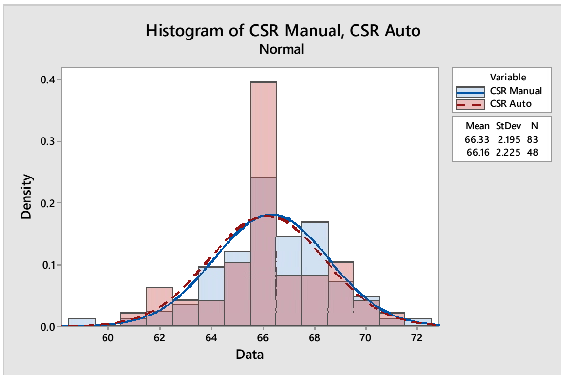
Figure 58 – Histogram and normal distribution comparison of CSR results sampled manually and with the autosampler
