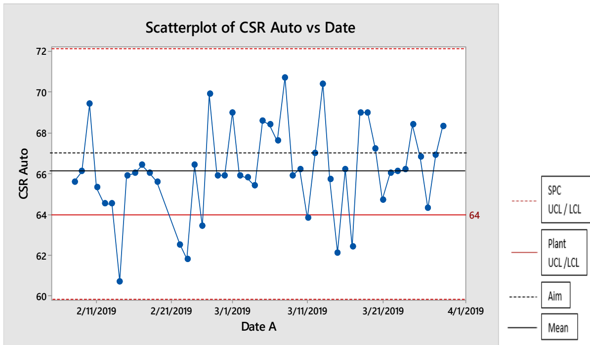
Figure 57 – SPC control chart of the CSR results from coke sampled from the autosampler
