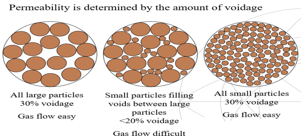
Figure 6 - Diagram explaining the importance of particle size in gas flow (Danieli Corus BV, 2009)
