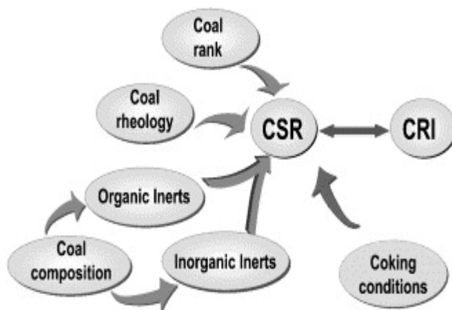
Figure 22 - Diagram showing the factors affecting CSR (Díez, et al., 2002)
