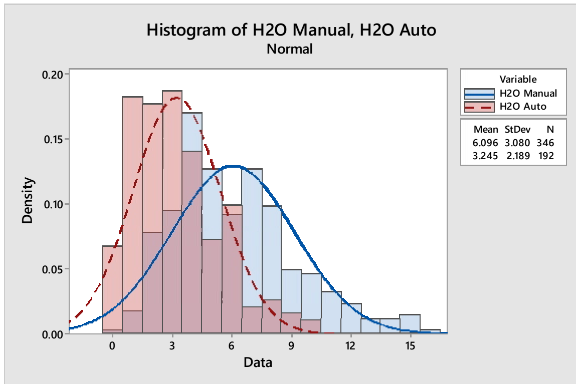
Figure 64 – Histogram and normal distribution comparison of moisture results sampled manually and with the autosampler
