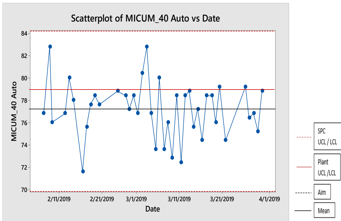
Figure 72 – SPC control chart of the M40 results from coke sampled from the autosampler
