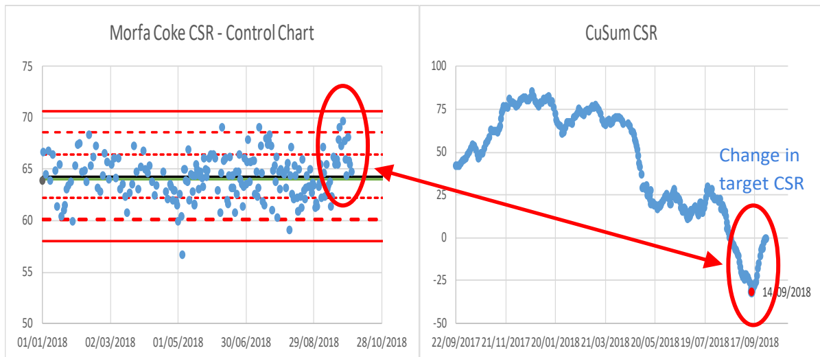
Figure 21 – Scatterplot and CuSum charts showing the drop in quality that triggered the change in CSR specification (Tatasteel, 2018)
