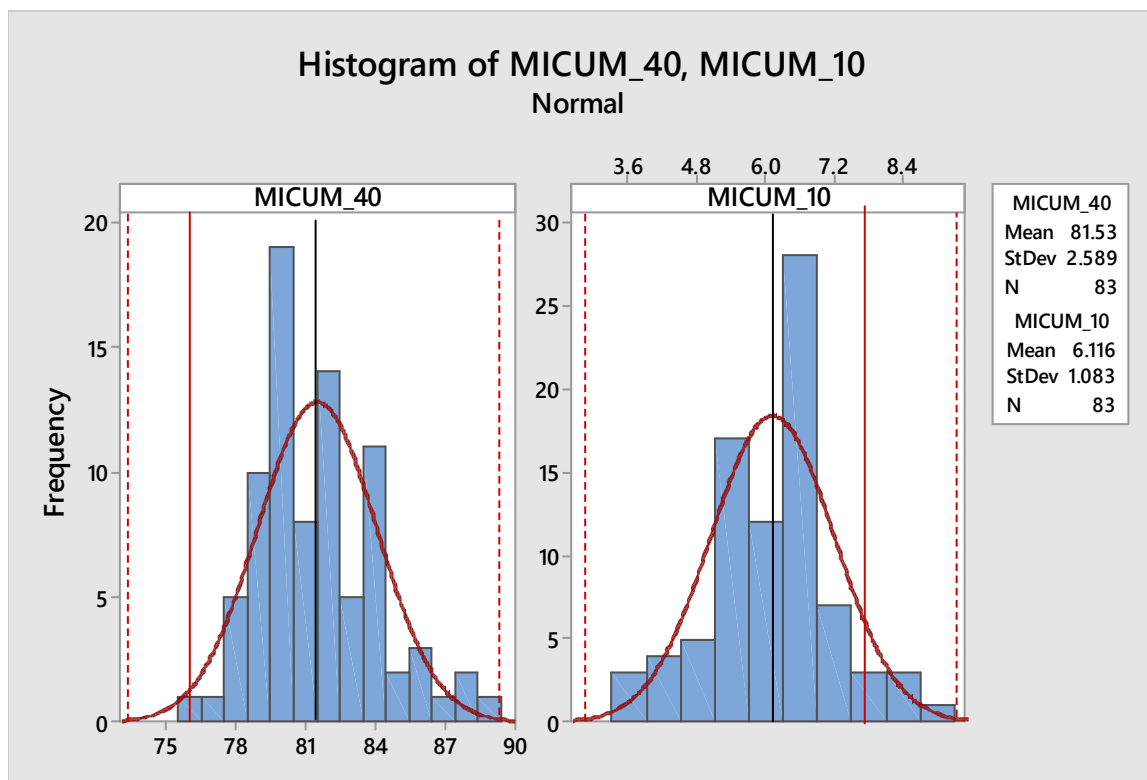
Figure 55 – Histogram and normal distribution of the M40 and M10 results between October 2018 and January 2019
