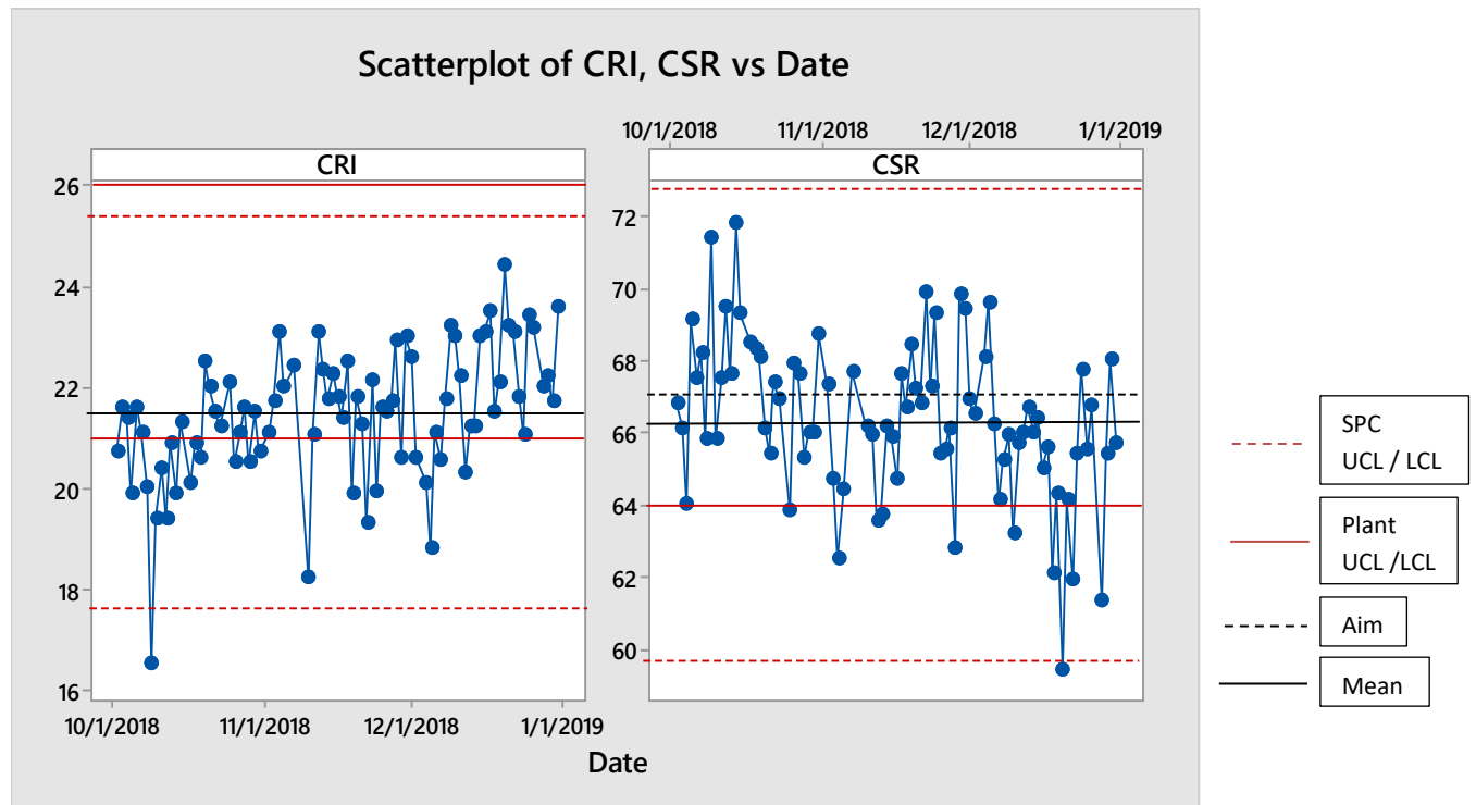
Figure 42 – SPC control charts for CSR and CRI between October 2018 and January 2019
