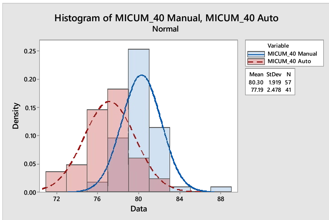
Figure 73 – Histogram and normal distribution comparison of M40 results sampled manually and with the autosampler
