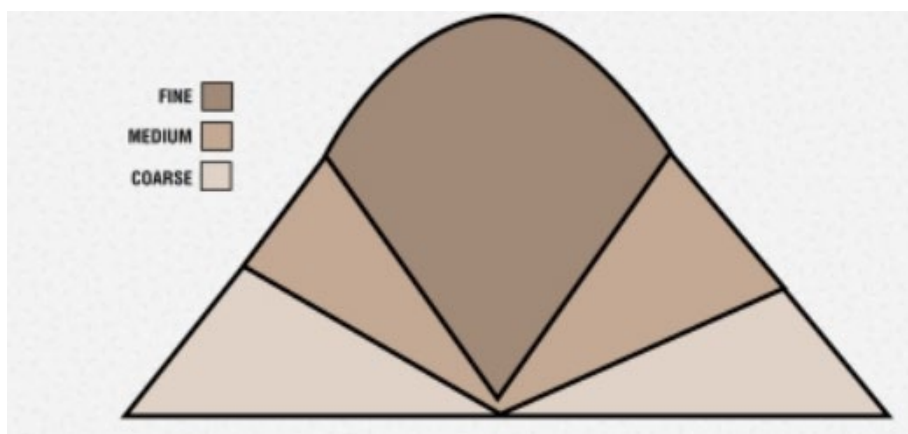
Figure 32 – Material segregation in a stockpile (Nohl & Domnick, 2000)
