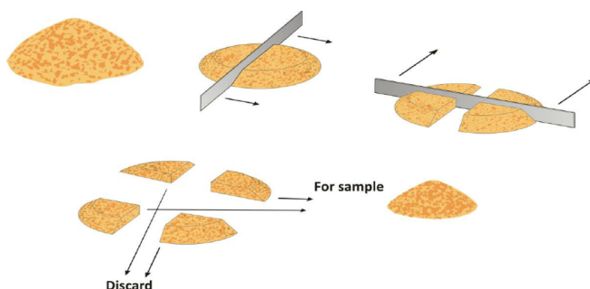
Figure 30 - The cone and quarter method (Alakangas, 2015)
