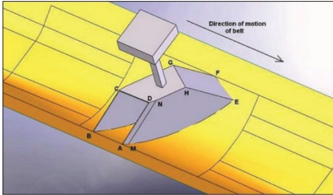
Figure 18 - The cutter on a 'hammer' cross belt autosampler (Robinson, et al., 2010)
