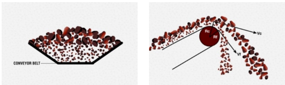
Figure 31 – Material segregation on a conveyor and conveyor discharge (Nohl & Domnick, 2000)
