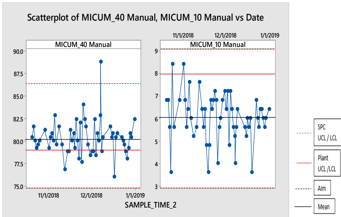
Figure 54 – SPC control chart of the M40 and M10 results between October 2018 and January 2019
