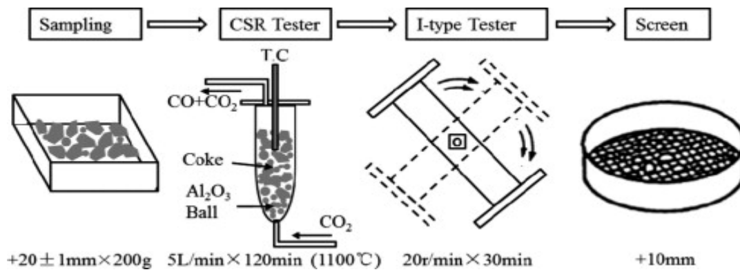
Figure 10 - Diagram of the CSR/CRI test (Li, et al., 2014)
