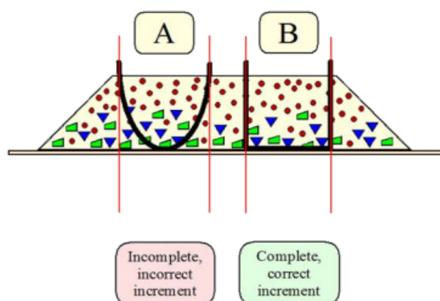
Figure 17 - The correct increment to take from a conveyor (Mortenson, 2015)
