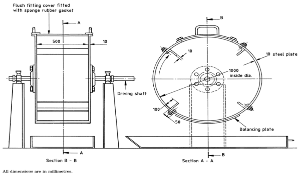
Figure 8 – Diagram of a Micum drum (British Standards Institute, 1992)
