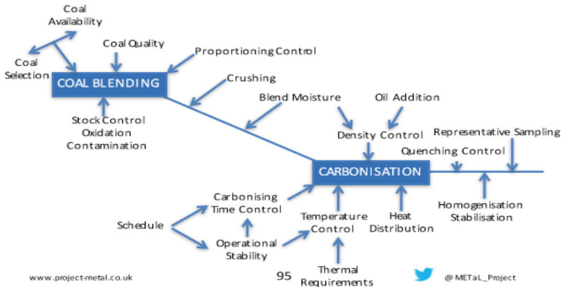
Figure 23 - Factors affecting coke quality (METaL, 2016)
