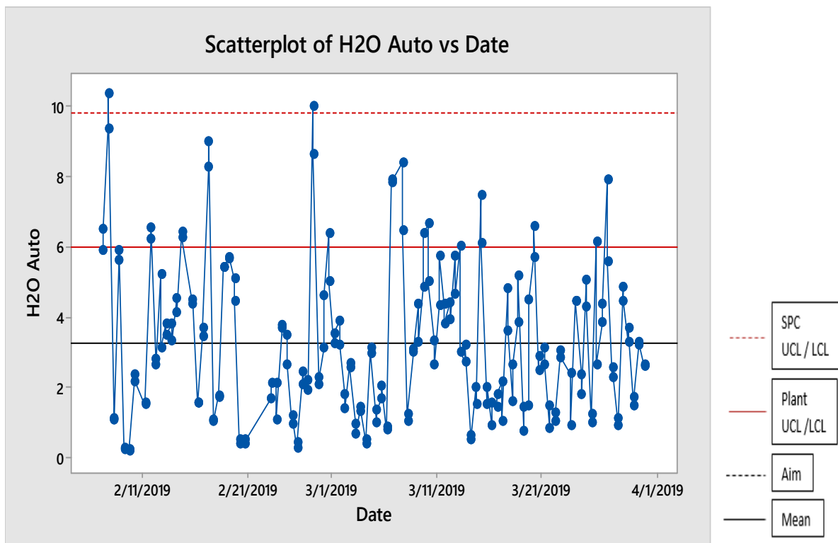
Figure 63 – SPC control chart of the moisture results from coke sampled from the autosampler
