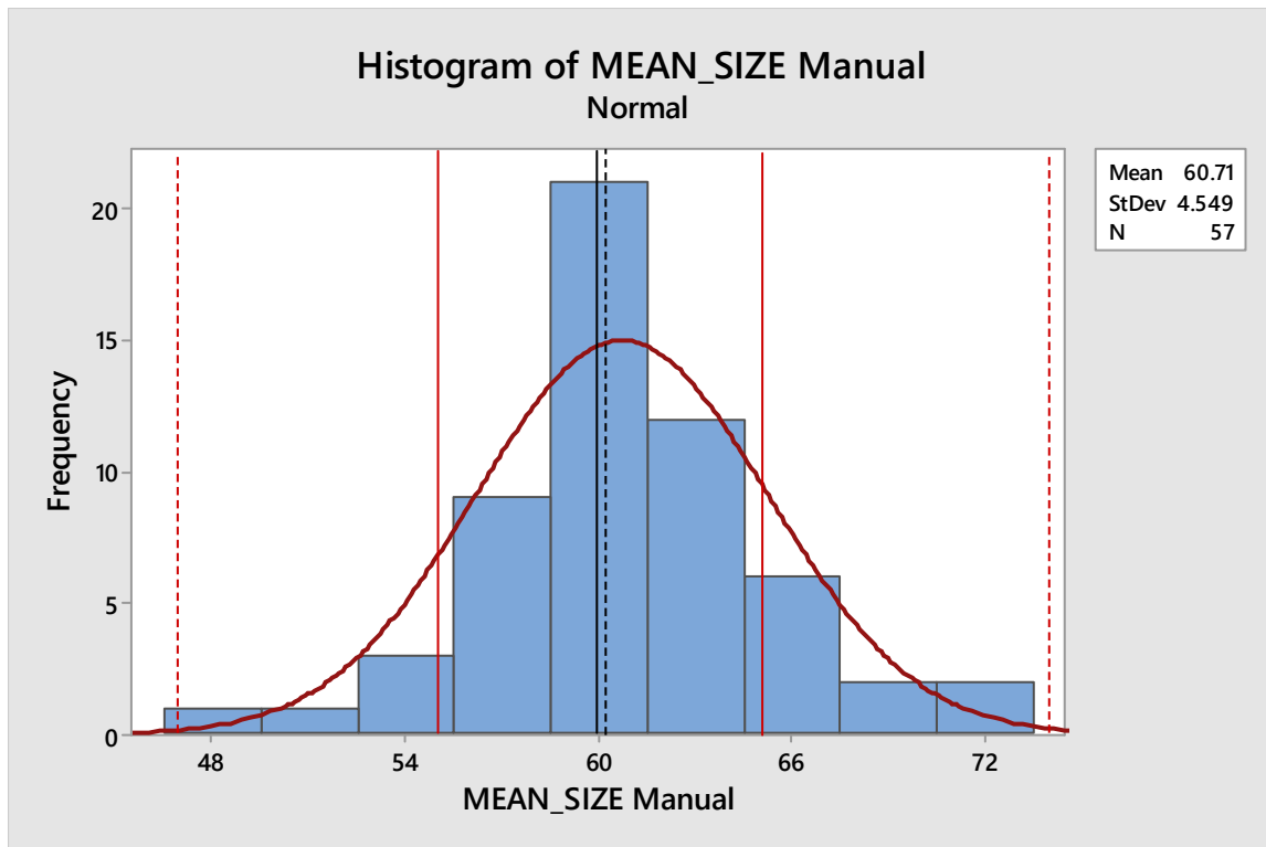
Figure 52 – Histogram and normal distribution of the mean size results between October 2018 and January 2019
