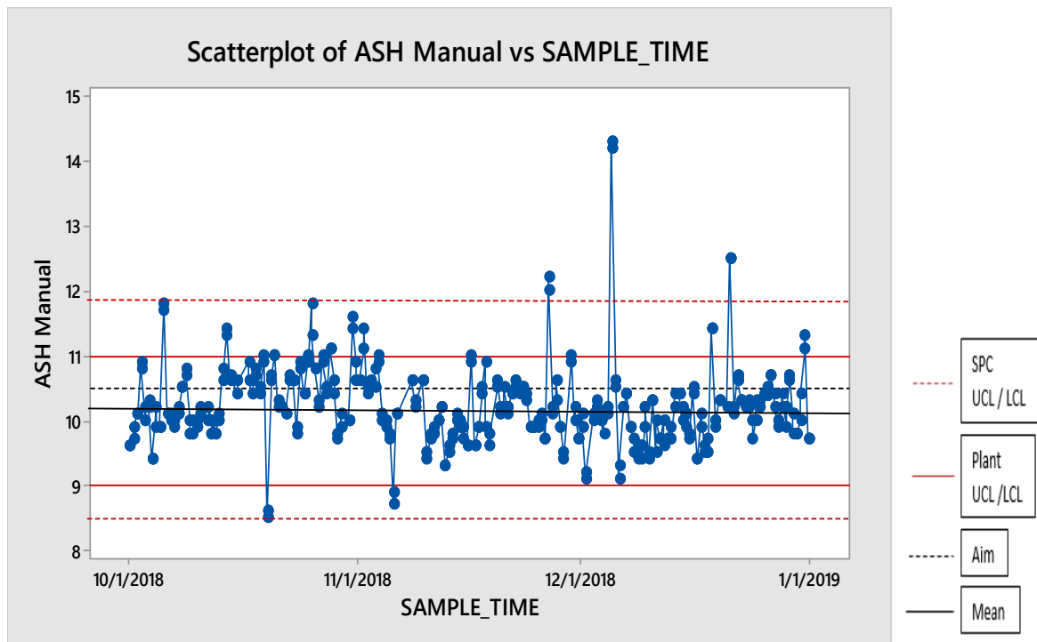
Figure 48 – SPC control chart of the ash results between October 2018 and January 2019
