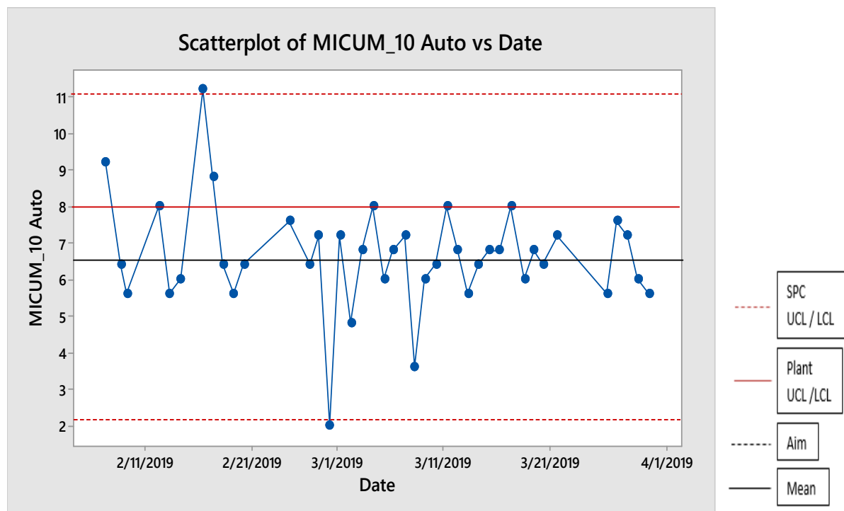
Figure 75 – SPC control chart of the M10 results from coke sampled from the autosampler
