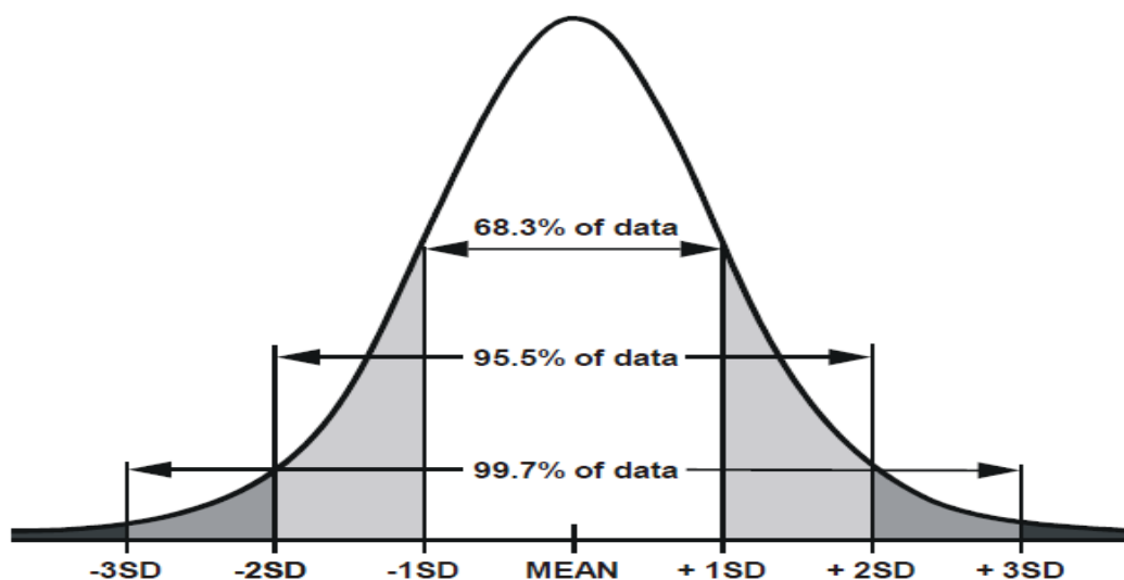
Figure 40 – Standard variation in a normal distribution curve (Jin, 2018)
