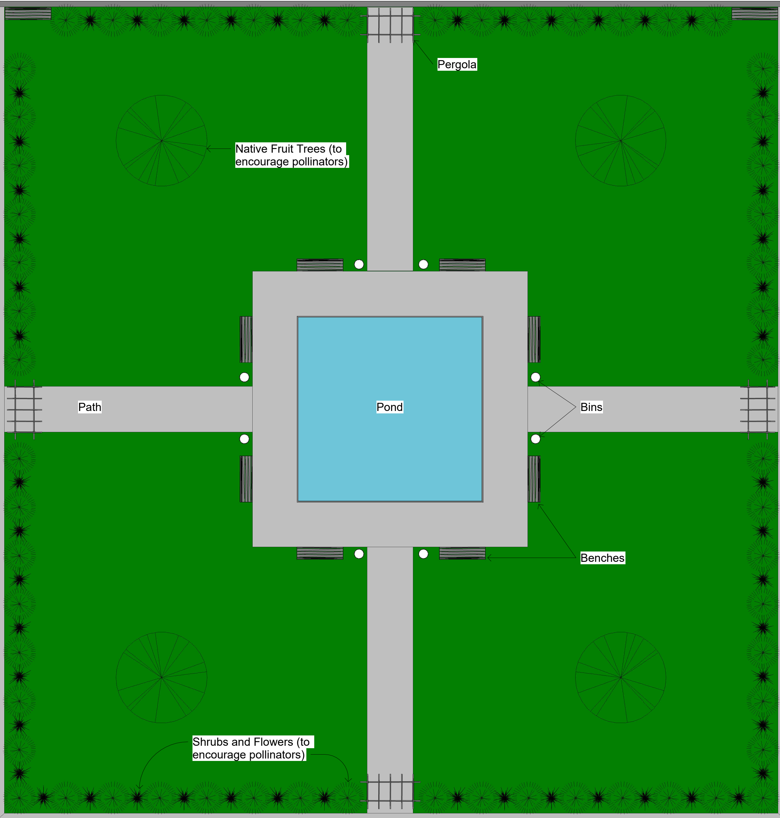
Communal Garden Landscape Plan 1 : 100
