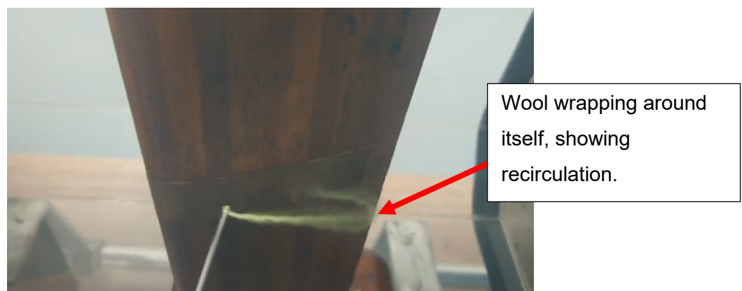
Figure 27 - Naca 0012 15° Recirculation
