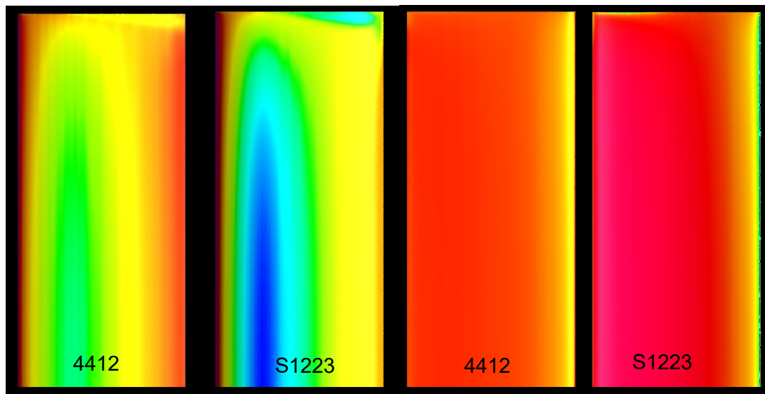
Figure 43 - Naca 4412 & S1223 Surface Pressure Contours
