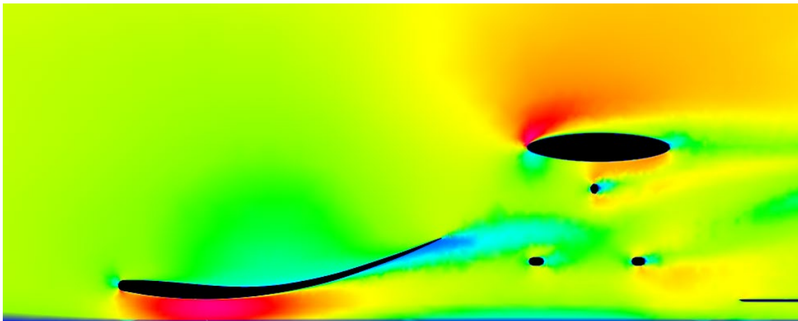
Figure 37 - JHTT02 Splitter Velocity Contours
