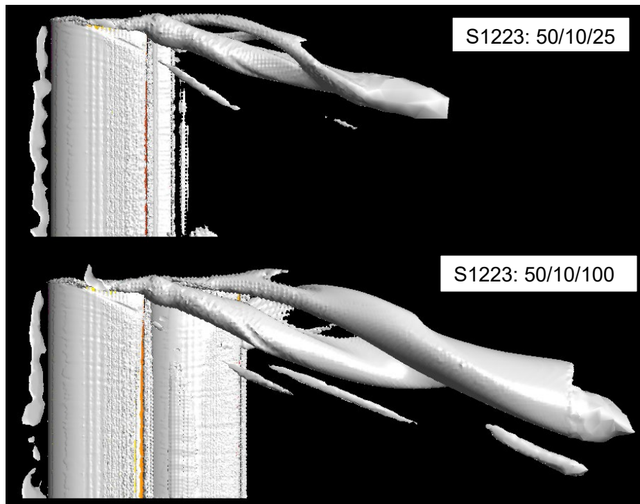
Figure 59 - Chord Length Study Vortex Generation
