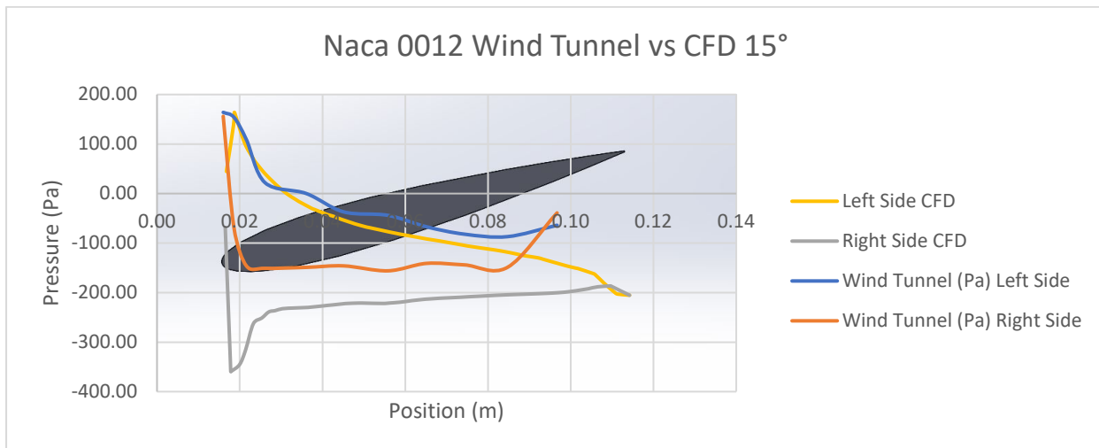
Graph 3 - Naca 0012 Wind Tunnel vs CFD (15°)
