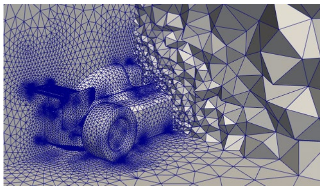
Figure 22 - Surface & Volume Mesh (Using a Symmetry Plane) (symscape, 2013)
