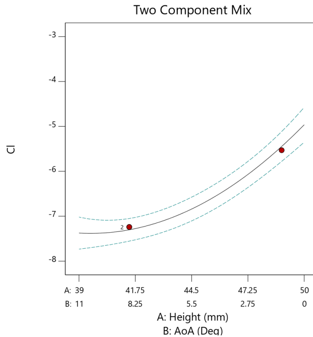
Graph 27 - Naca 4412 Overhang Influence ( C_l ) (0mm Overhang)
