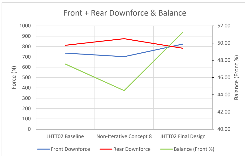
Graph 69 - Front + Rear Downforce & Balance
