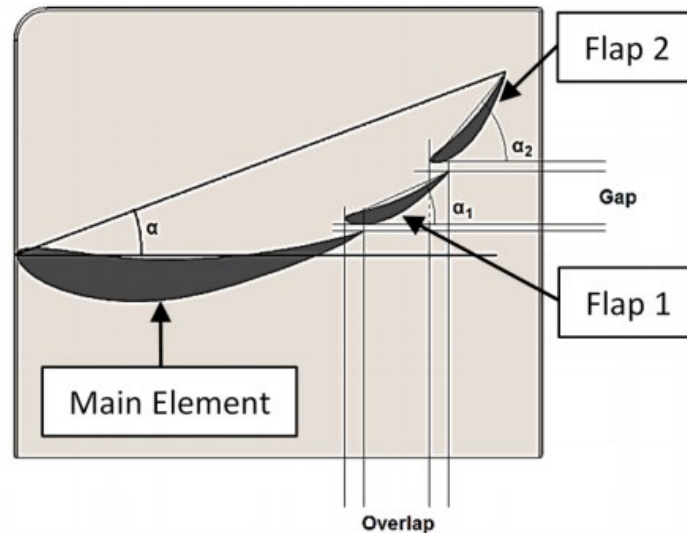
Figure 16 - Multi - Element Aerofoil (Jackson, 2018)
