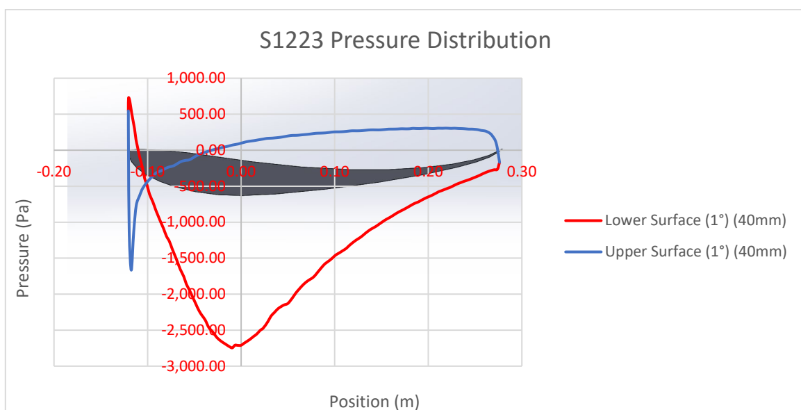
Graph 9 – S1223 Pressure Distribution
