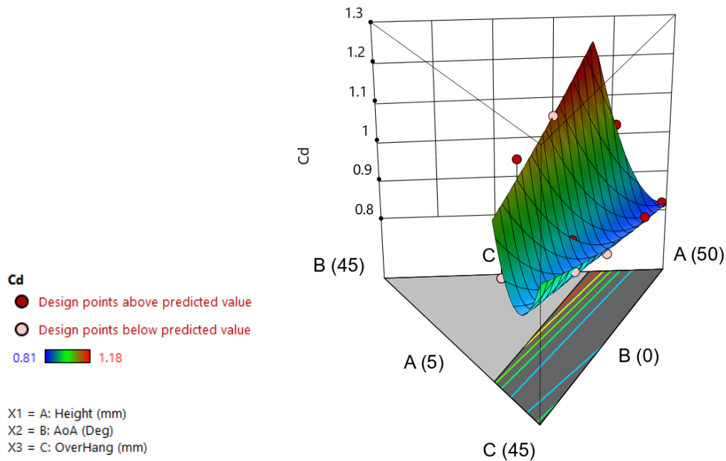
Graph 32 - S1223 Secondary Element DOE Study ( C_d )
