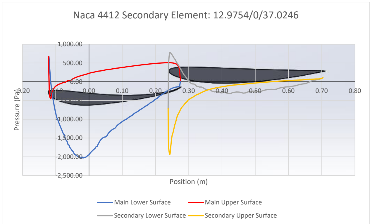
Graph 34 - Naca 4412 Secondary Element Pressure Distribution (12.9754mm/0°/37.0246mm)
