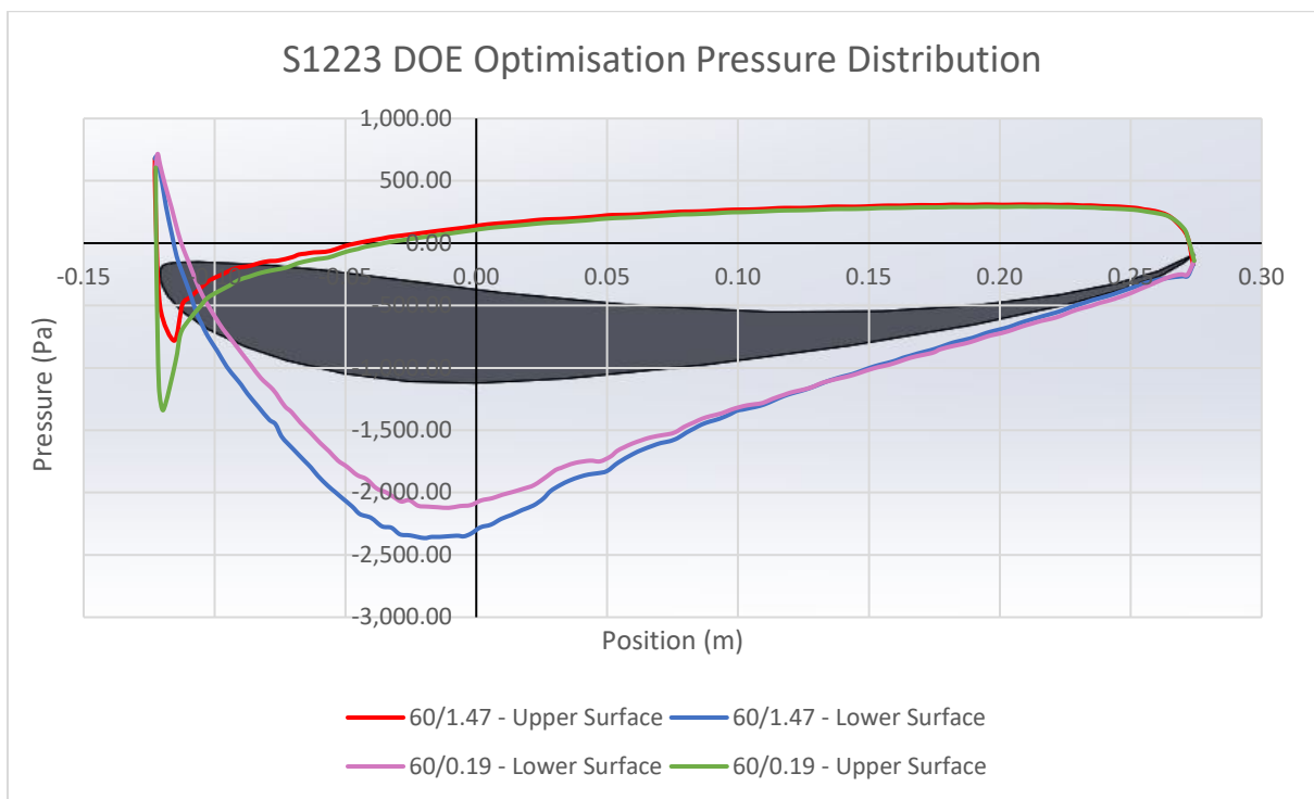
Graph 25 - S1223 DOE Optimisation Pressure Distribution
