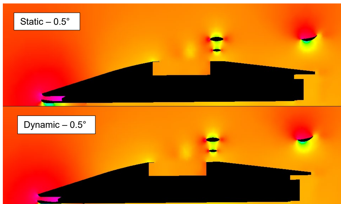
Figure 82 - Symmetry Plane Pressure Contours
