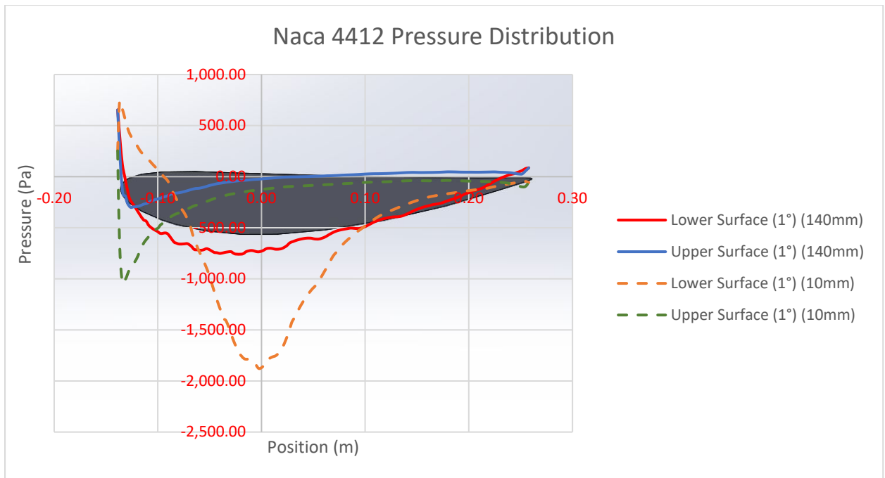
Graph 12 - Naca 4412 Pressure Distribution (10mm & 140mm)
