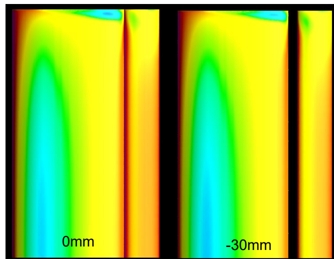
Figure 63 - Secondary Element Overhang (0mm - 30mm) (Lower Surface Pressure Contours)
