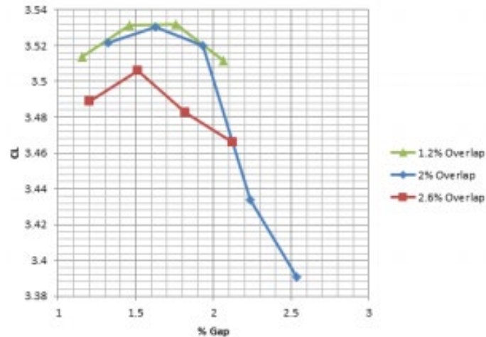
Figure 18 - Gap Size & Overlap Sensitivity Study (Craig & Passmore, 2014)
