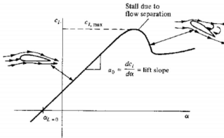
Figure 15 - C_l vs AoA (Seljak, 2008)
