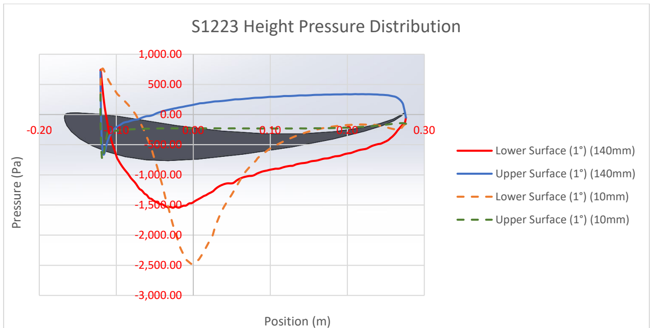
Graph 13 - S1223 Pressure Distribution (10mm & 140mm)
