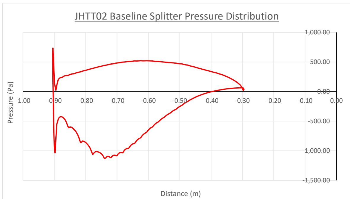
Graph 4 - JHTT02 Baseline Surface Pressure Distribution
