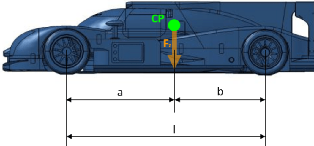
Figure 21 - Downforce Distribution (CP) (Quintarelli, 2018)
