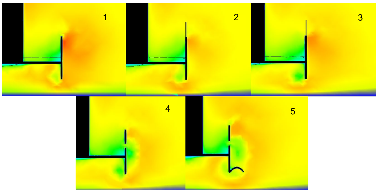
Figure 77 - End Plate Development Velocity Contours
