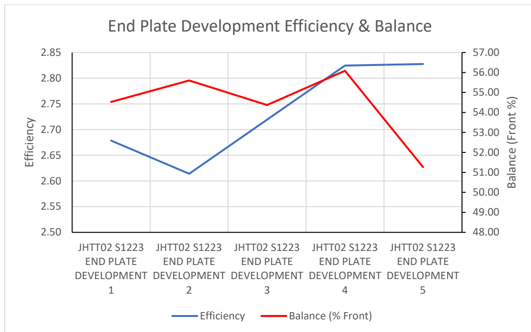
Graph 58 - End Plate Development Efficiency & Balance
