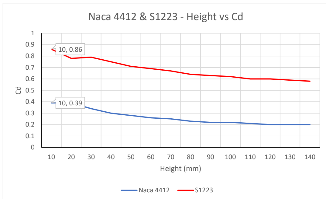
Graph 11 - Naca 4412 & S1223 - Height vs C_d
