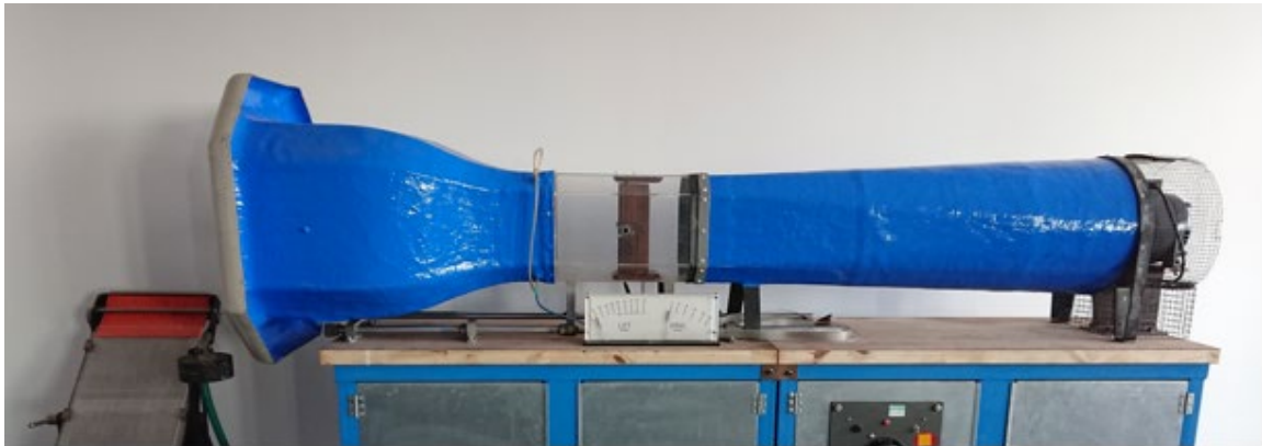
Figure 24 - C2 Open Loop Wind Tunnel
