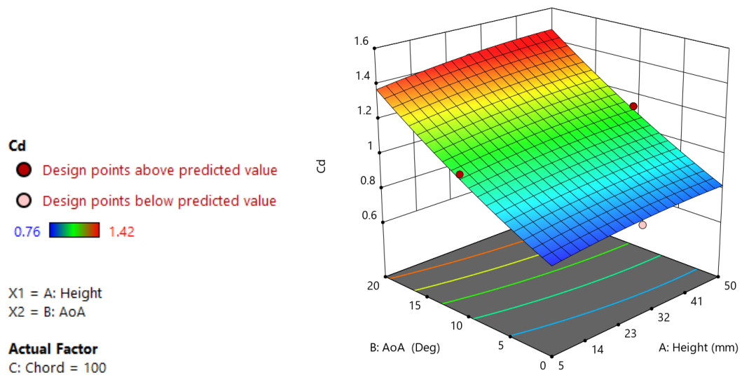
Graph 43 - S1223 Secondary Element DOE Study 2 (Cl) (100% Chord)
