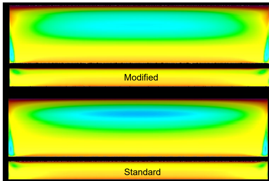
Figure 69 – Modified & Standard Main Plane Lower Surface Pressure Contours
