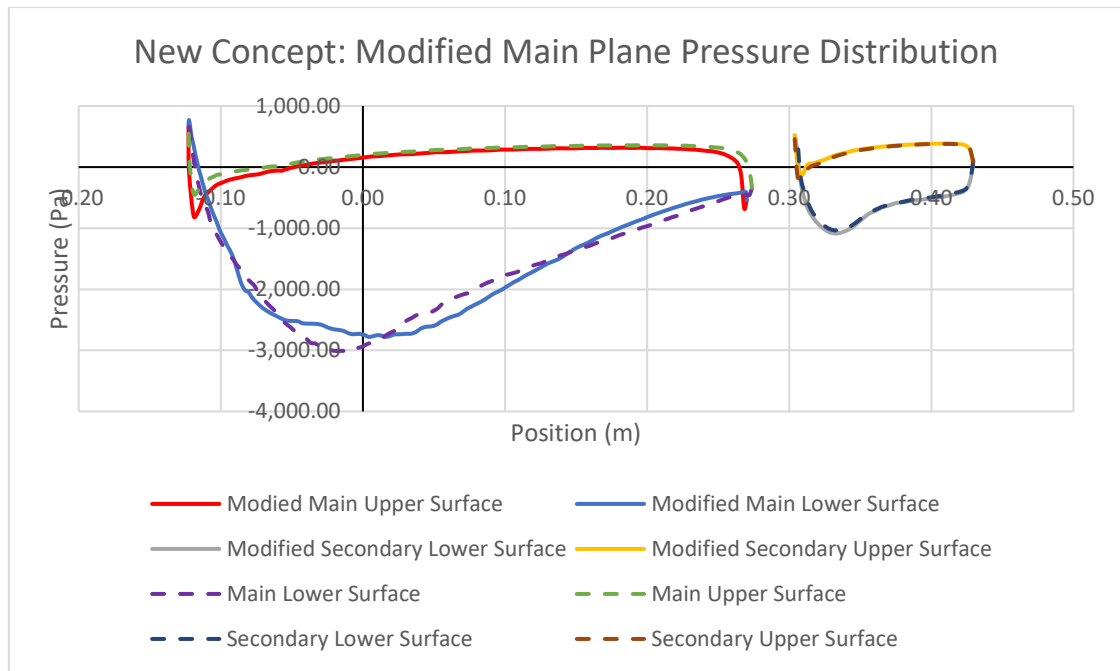
Graph 55 - New Concept: Modified Main Plane Pressure Distribution
