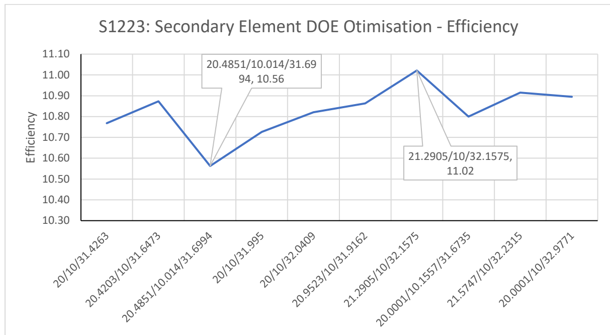
Graph 46 – S1223: Secondary Element DOE Optimisation (Efficiency)
