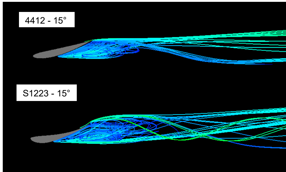
Figure 54 - Naca 4412 & S1223 Velocity Streamlines (15°)
