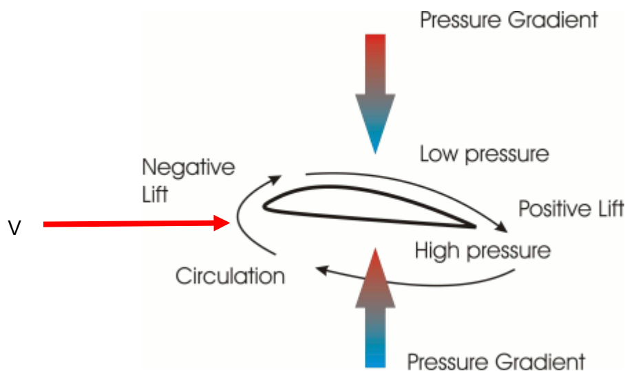
Figure 11 - Wing Recirculation (Glownia, 2007)
