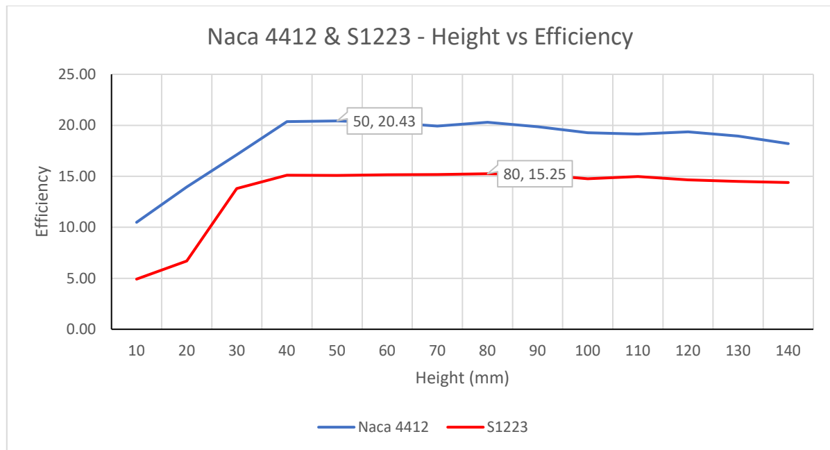
Graph 14 - Naca 4412 & S1223 - Height vs Efficiency
