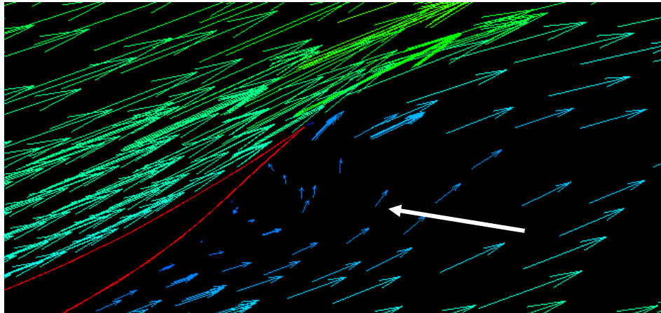
Figure 45 - S1223 Trailing Edge Velocity Vectors (Vortex)
