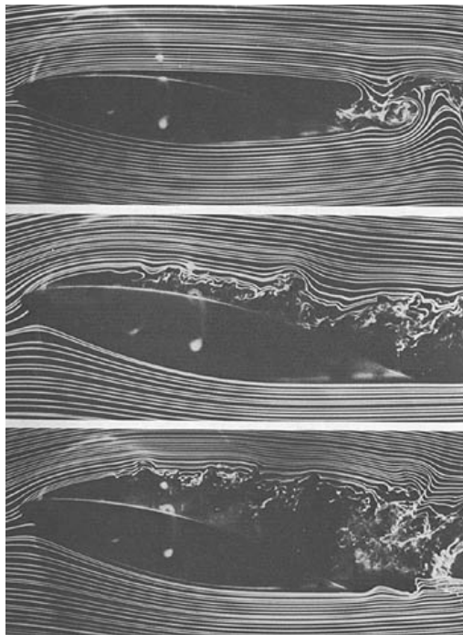
Figure 13 - Flow Separation (history.nasa.gov, 2010)
