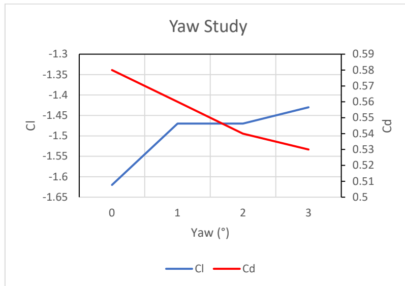
Graph 65 - Yaw Study C_l & C_d
