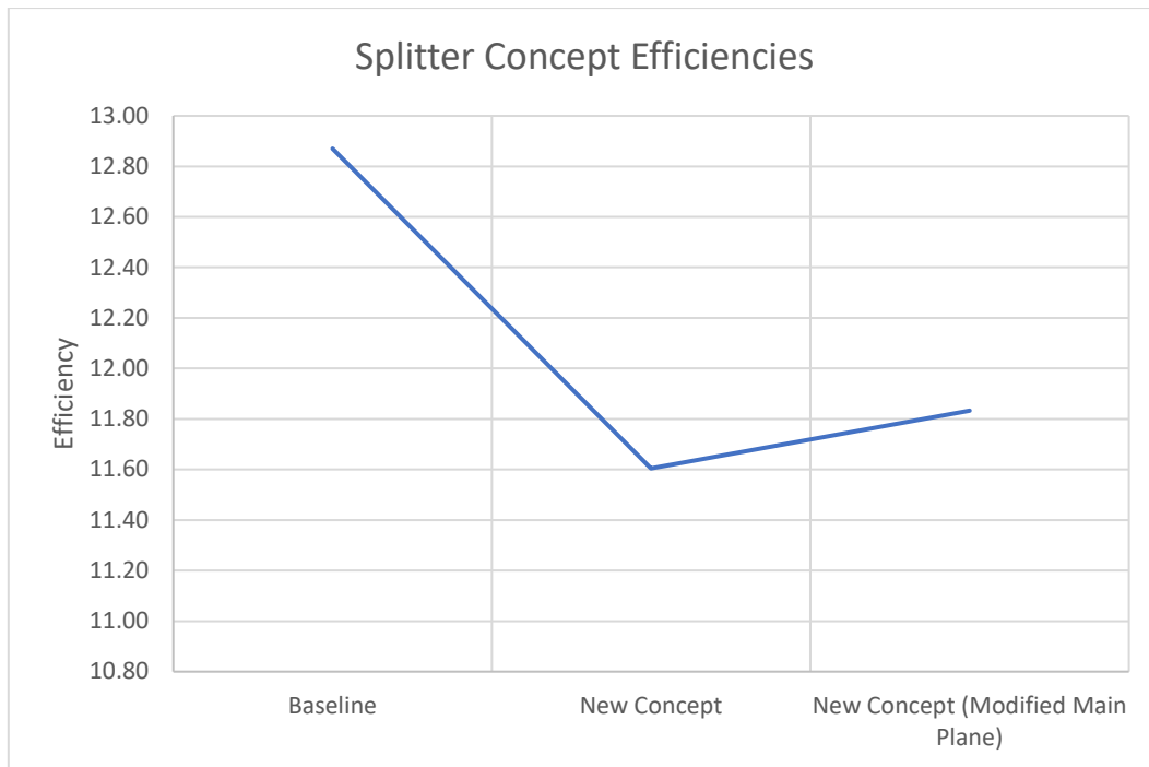
Graph 53 - Splitter Concepts Efficiency
