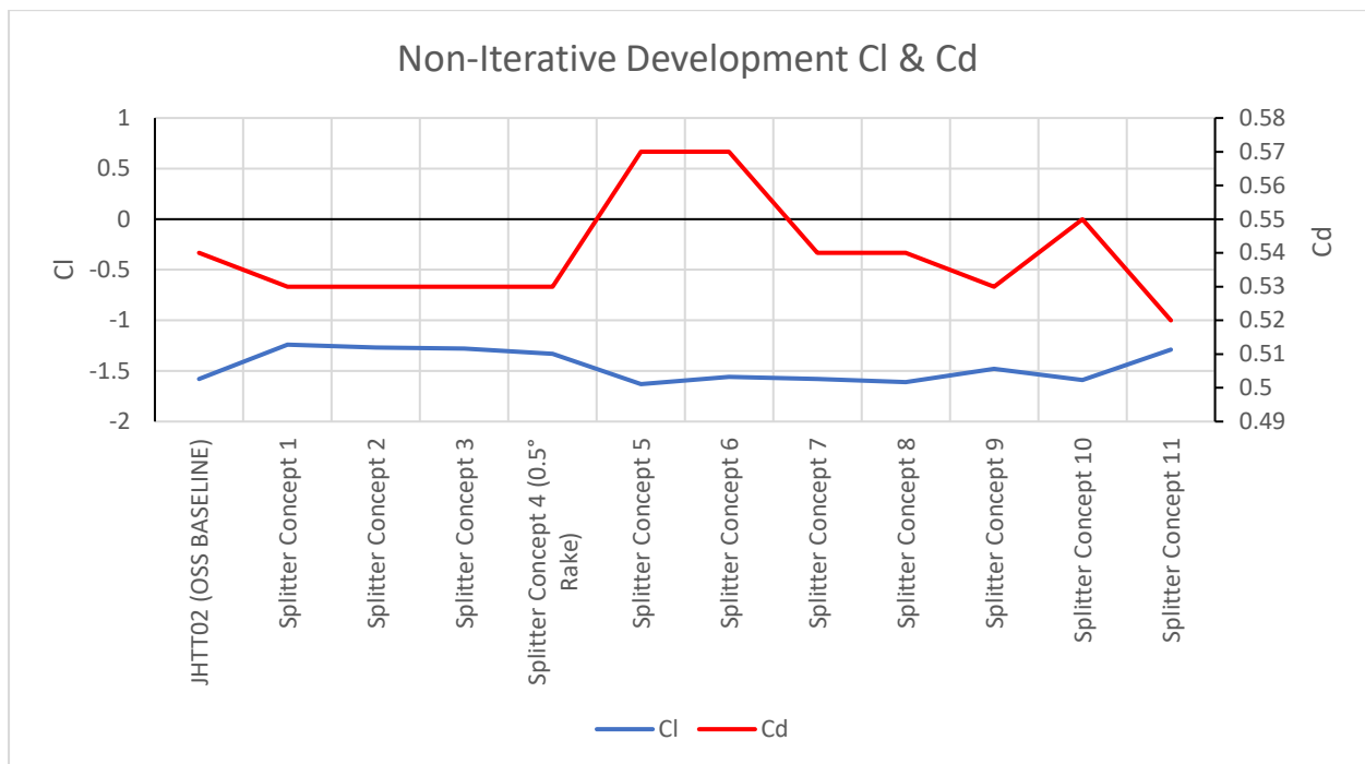
Graph 5 - Non-Iterative Development CI & Cd
