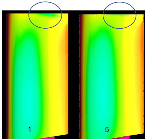
Figure 79 - End Plate Development Pressure Bleed
