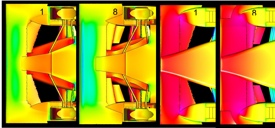
Figure 40 - Concept 1 & 8 Pressure Contours
