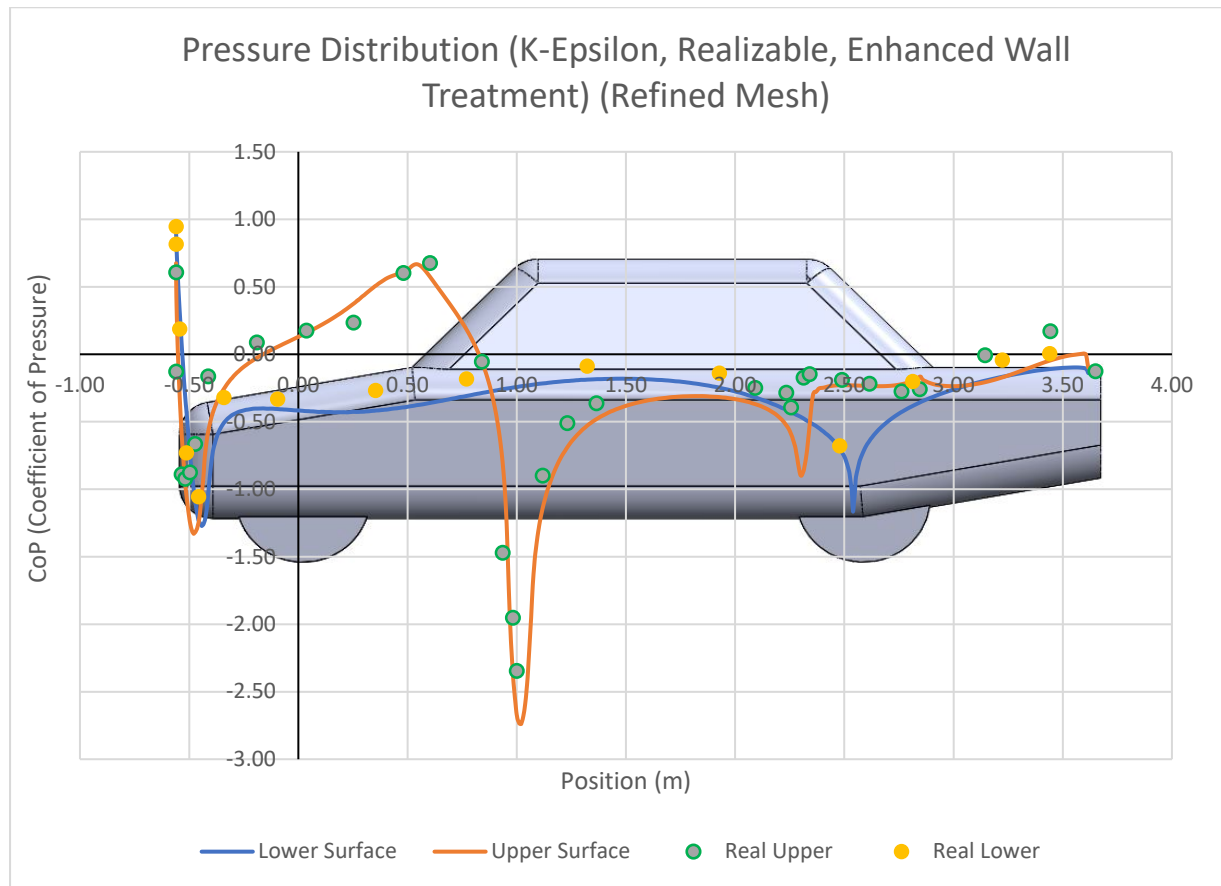
Graph 1 - MIRA Car Pressure Distribution (CFD Validation) (Hughes, 2018)
