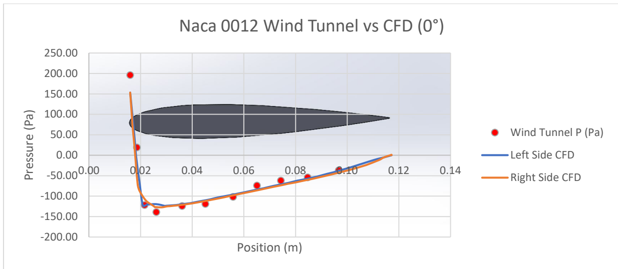
Graph 2 - Naca 0012 Wind Tunnel vs CFD (0°)
