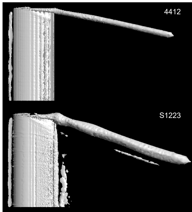
Figure 46 - Naca 4412 & S1223 Lower Surface Vortices
