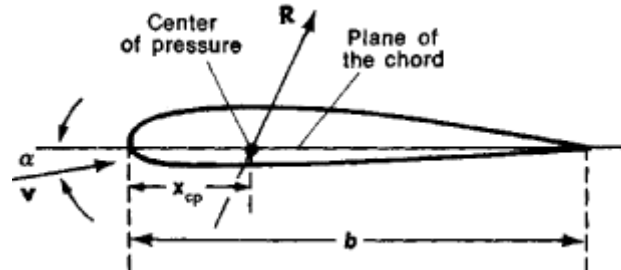
Figure 4 - Centre of Pressure on a Wing (The Great Soviet Encyclopedia, 1979)
