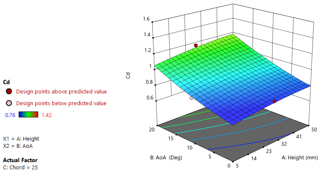
Graph 42 - S1223 Secondary Element DOE Study 2 (Cd) (25% Chord)
