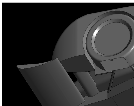
Figure 73 - Front Pontoon Geometry Change
