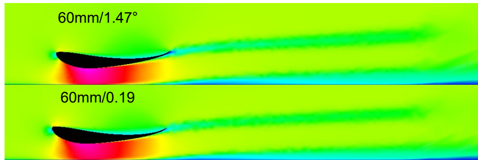
Figure 55 - S1223 Main Plane DOE Optimisation Velocity Contours
