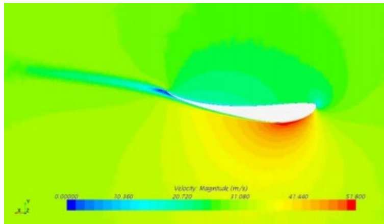
Figure 20 - Aerofoil in Freestream (S1223) (Mokhtar & Durrer, 2016)
