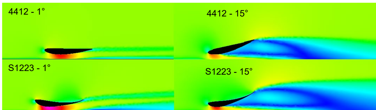
Figure 53 - Naca 4412 & S1223 Velocity Contours (1° - 15°)
