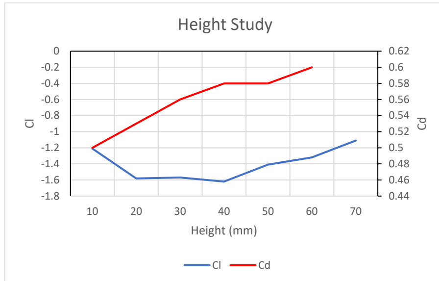
Graph 59 - Height C_l & C_d
