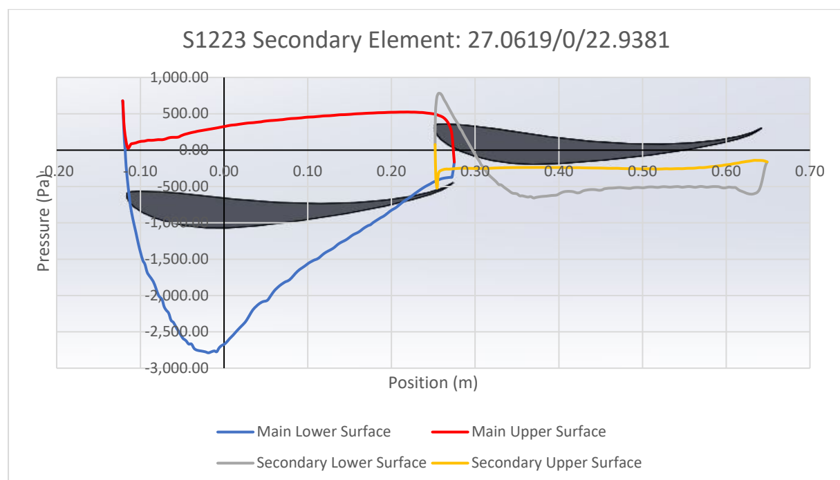
Graph 37 – S1223 Secondary Element Pressure Distribution (27.0619mm/0°/22.9381mm)
