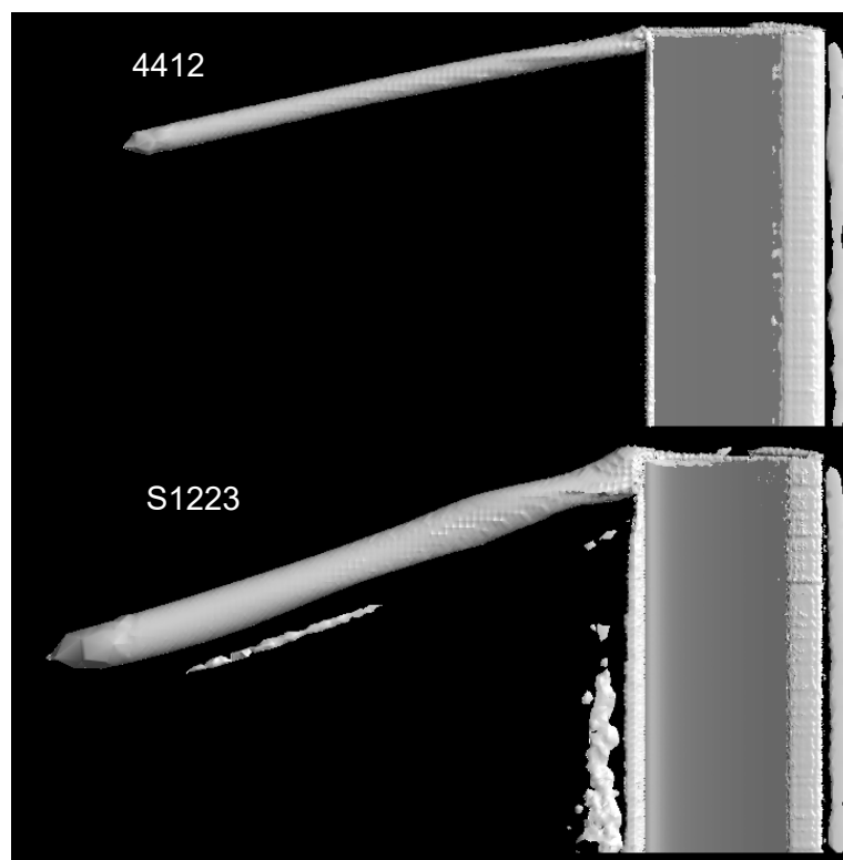
Figure 44 - Naca 4412 & S1223 Upper Surface Vortices
