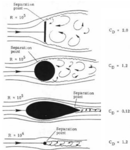
Figure 2 - Flow Around a Cylinder (Machin , 2015)
