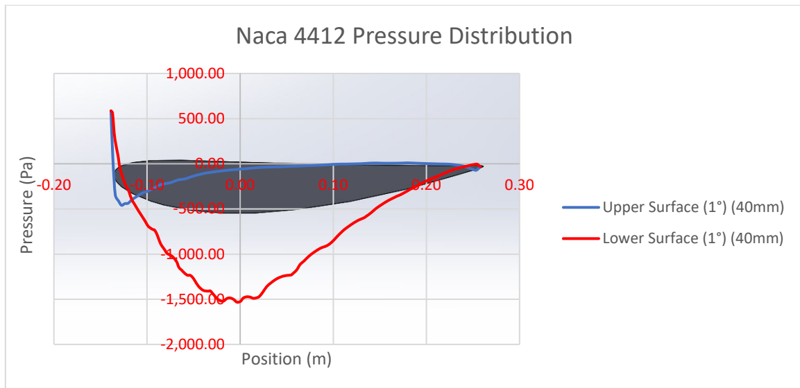
Graph 8 - Naca 4412 Pressure Distribution
