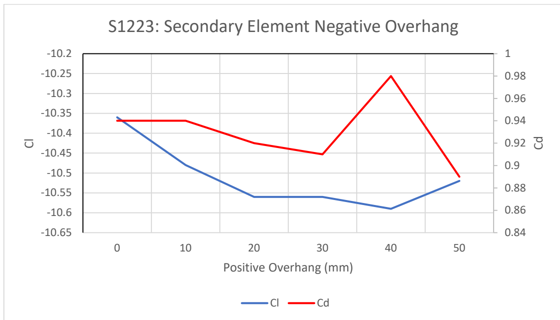
Graph 48 - S1223: Secondary Element Negative Overhang ( C_l & C_d )
