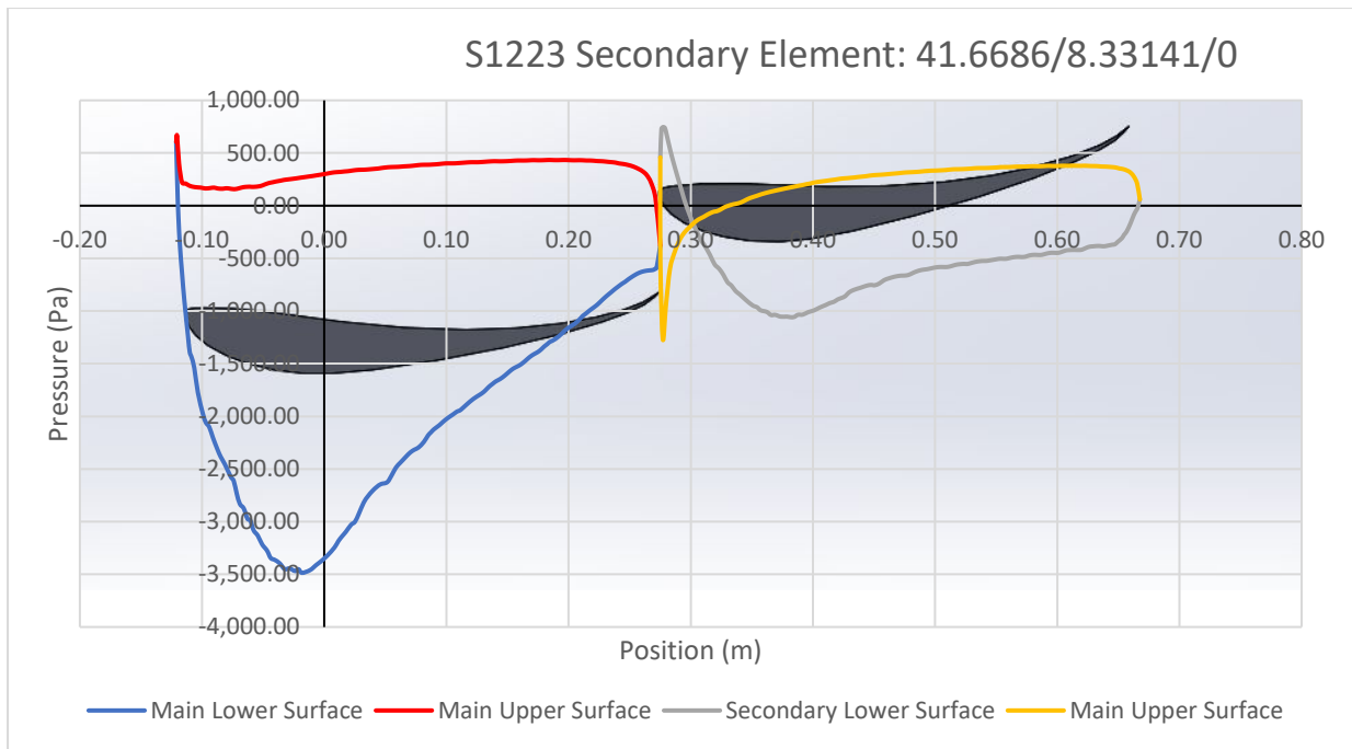
Graph 38 – S1223 Secondary Element Pressure Distribution (41.6686mm/8.33141°/0mm)
