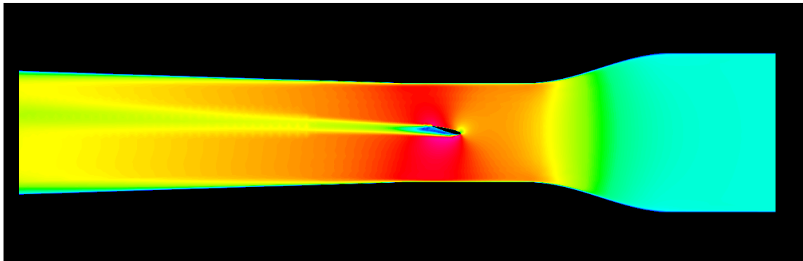
Figure 26 - C2 Wind Tunnel CFD Velocity Contours (15°)
