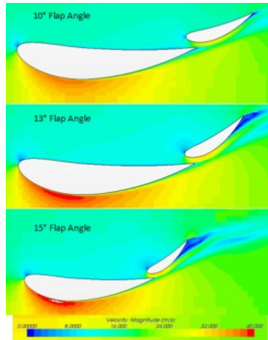
Figure 17 - Multi - Element Wing Element Configurations (Craig & Passmore, 2014)
