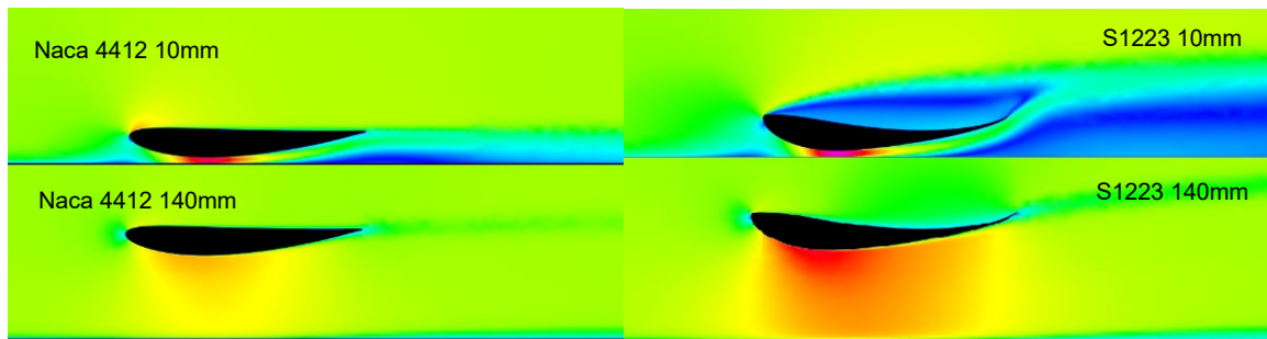
Figure 49 - Naca 4412 & S1223 Maximum & Minimum Heights (Velocity Contours)
