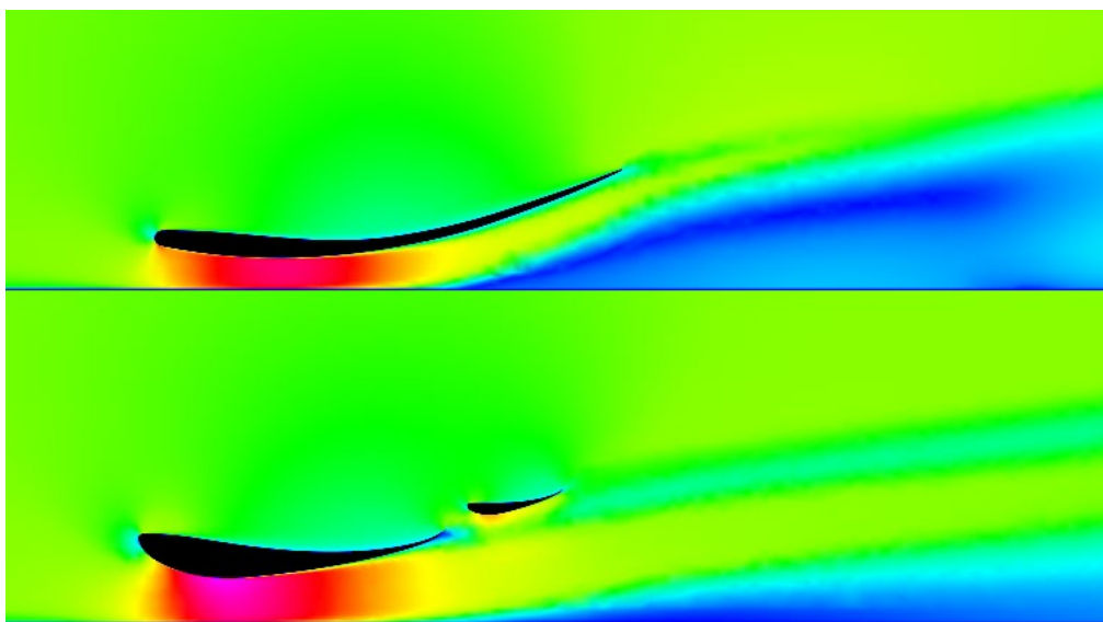
Figure 66 - Baseline Splitter vs New Concept (Velocity Contours)
