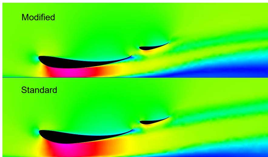
Figure 68 - Modified & Standard Main Plane Velocity Contours
