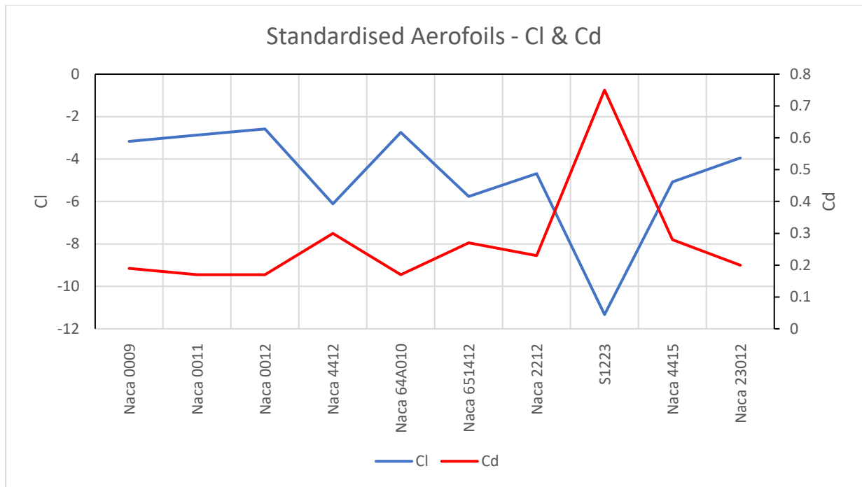
Graph 7 - Standardised Aerofoils - Cl & Cd
