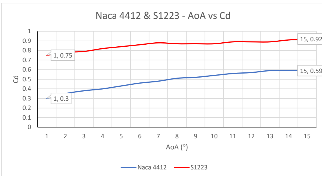
Graph 16 - Naca 4412 & S1223 - AoA vs Cd
