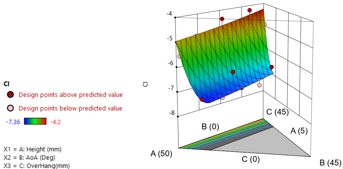
Graph 26 - Naca 4412 Secondary Element DOE Study (CI)
