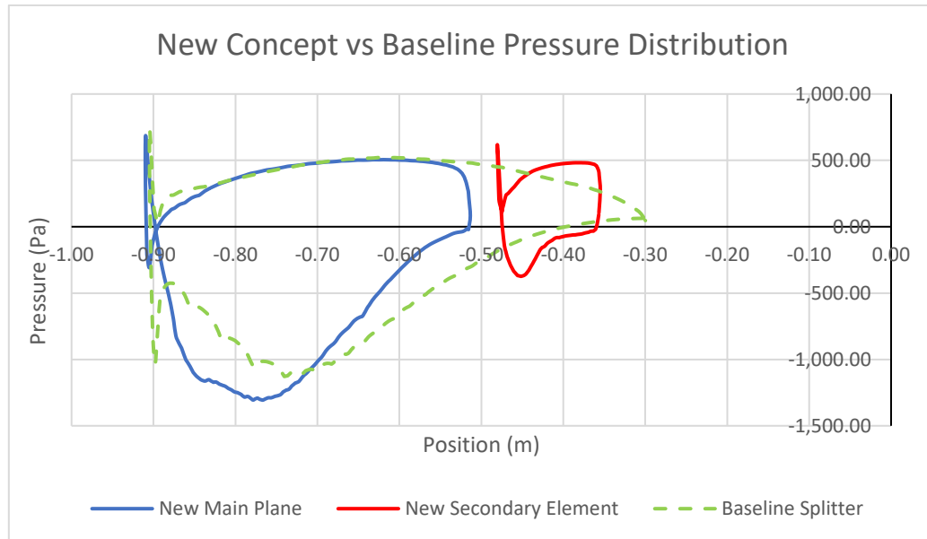
Graph 56 - New Concept vs Old Concept Pressure Distribution
