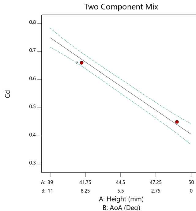
Graph 29 – Naca 4412 Overhang Influence (Cd) (0mm Overhang)
