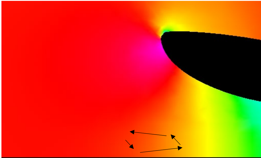
Figure 47 - Leading Edge Vortex Generation
