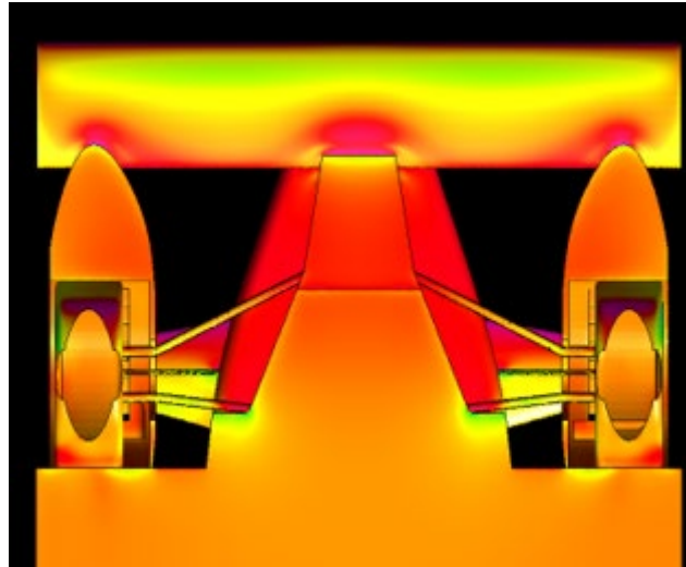
Figure 70 - Lower Surface Pressure Stagnation
