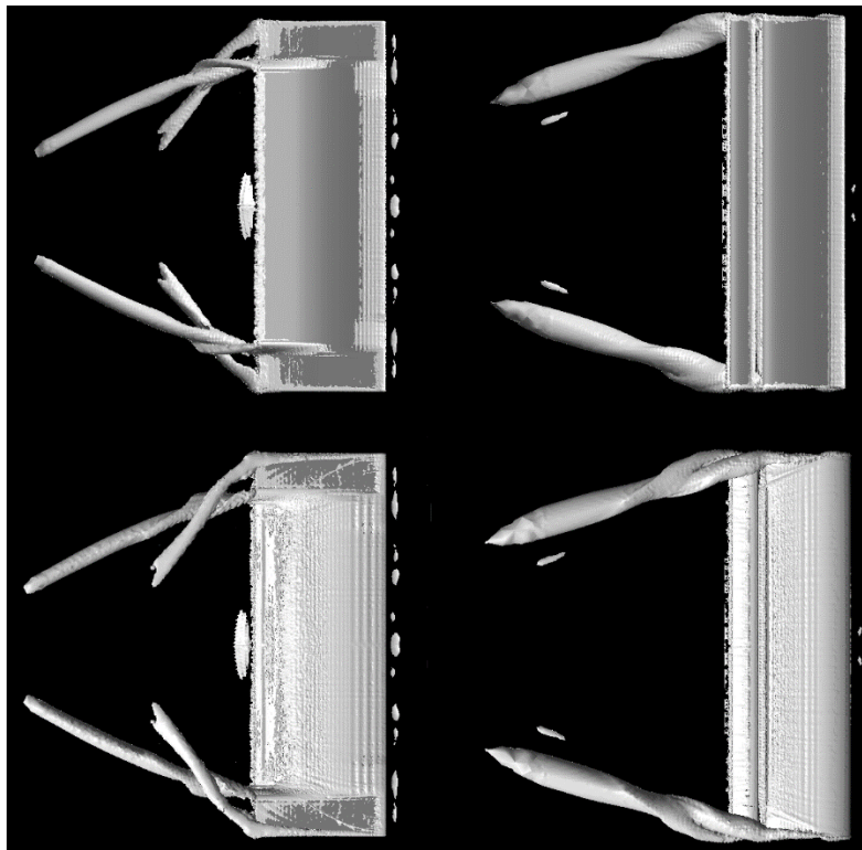
Figure 65 - Baseline Splitter vs New Concept Vortices
