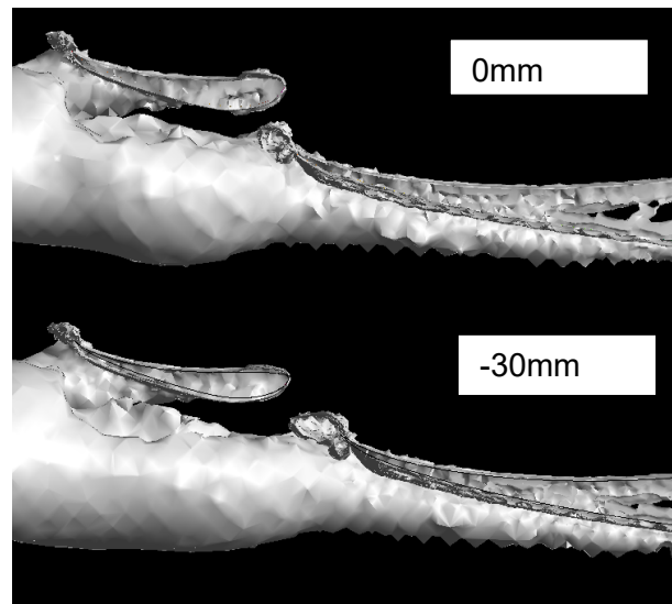
Figure 62 - Trailing Edge Vortex
