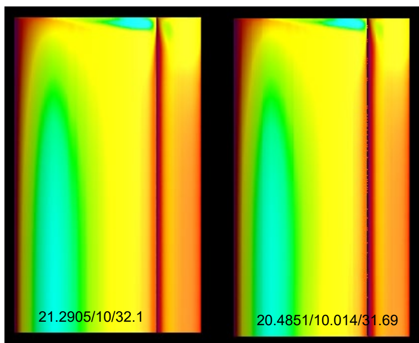
Figure 60 - S1223: Secondary Element DOE Optimisation (Lower Surface Pressure Contours)
