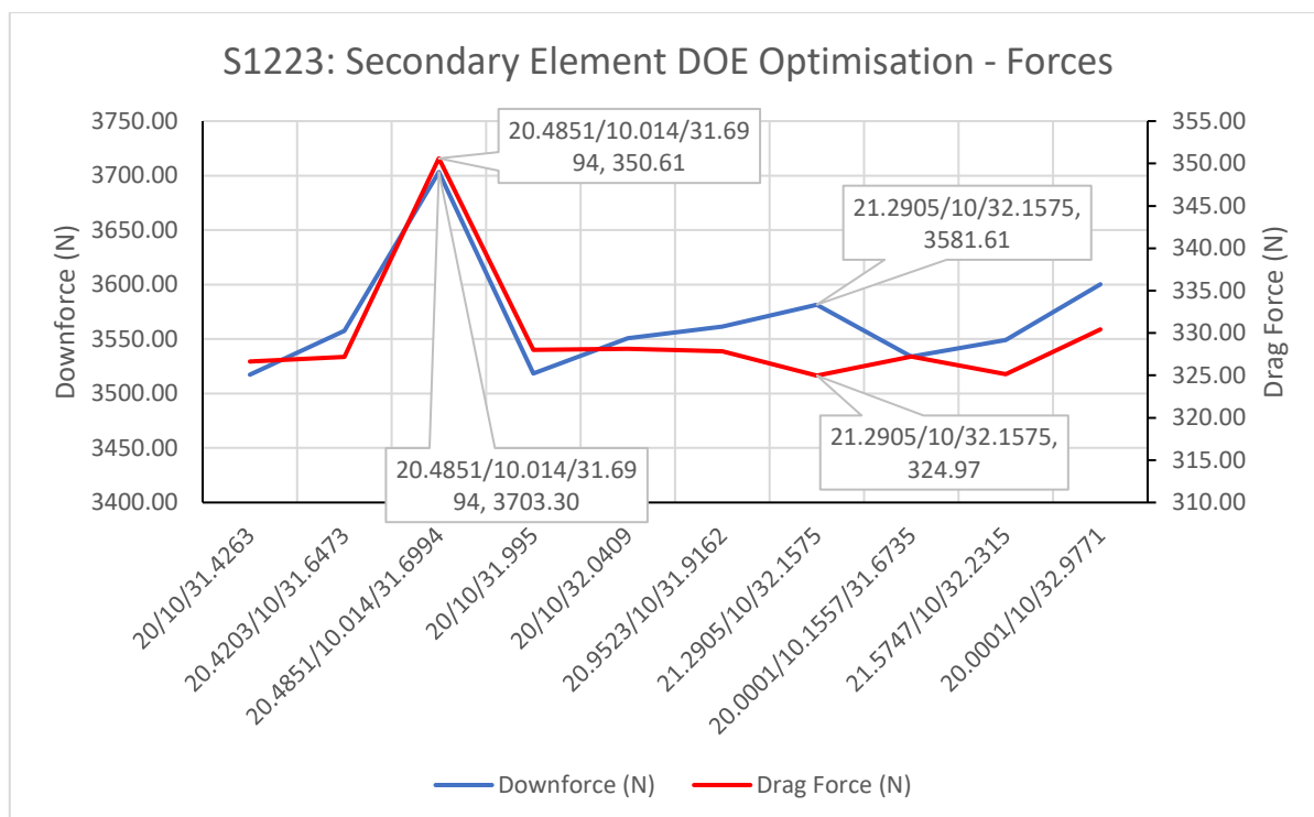
Graph 47 - S1223: Secondary Element DOE Optimisation (Forces)
