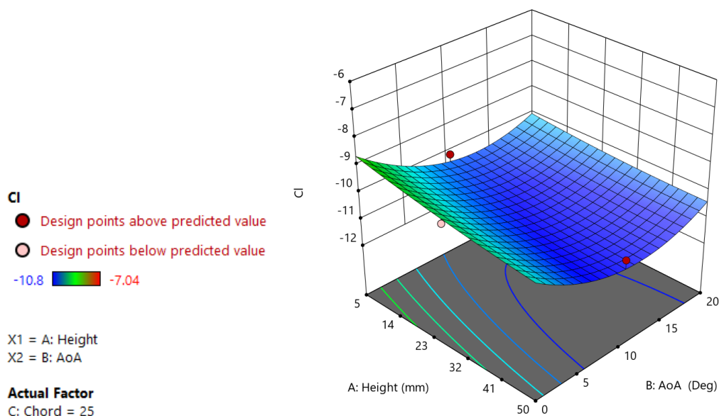
Graph 40 - S1223 Secondary Element DOE Study 2 (CI) (25% Chord)
