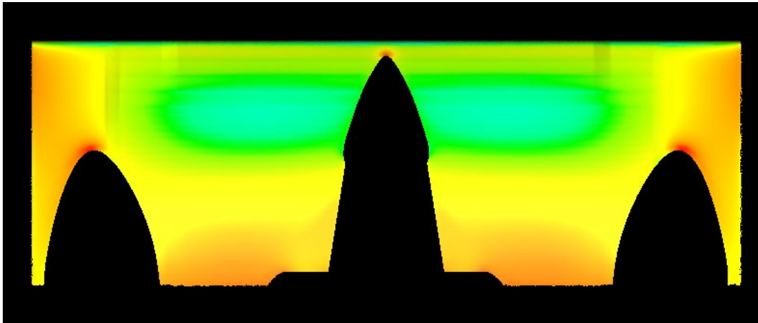
Figure 38 - JHTT02 Splitter Pressure Contours (Lower Surface)
