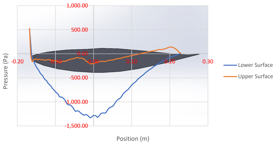
Naca 651412 Pressure Distribution
