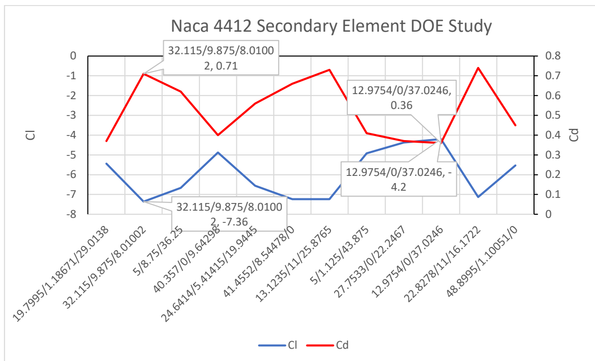
Graph 36 - Naca 4412 Secondary Element DOE Study (Cl & Cd)
