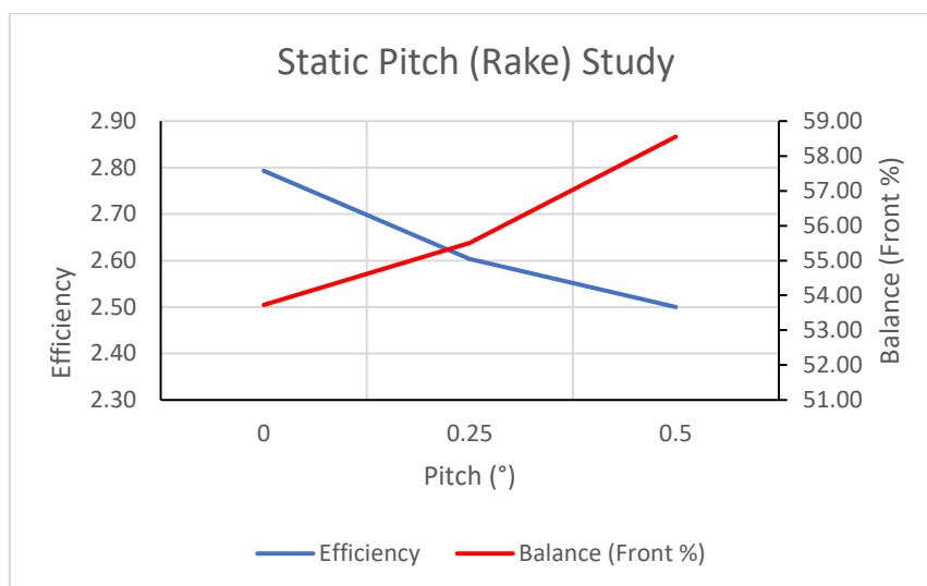
Graph 62 - Static Pitch Efficiency & Balance
