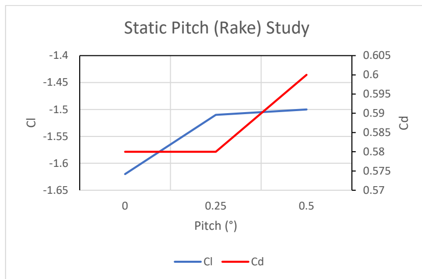
Graph 61 - Static Pitch Cl & Cd
