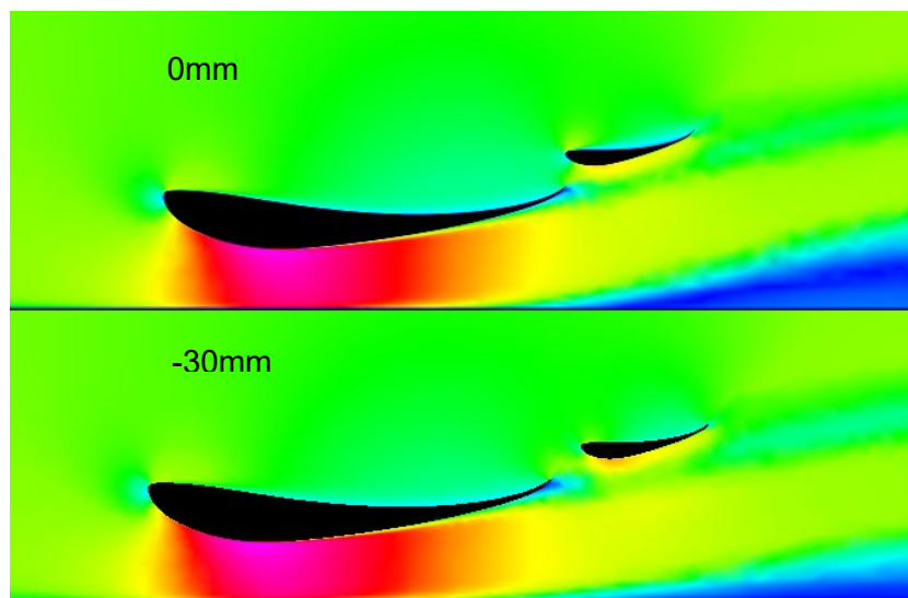
Figure 61 - Secondary Element Negative Overhang (0mm & 30mm) (Velocity Contours)
