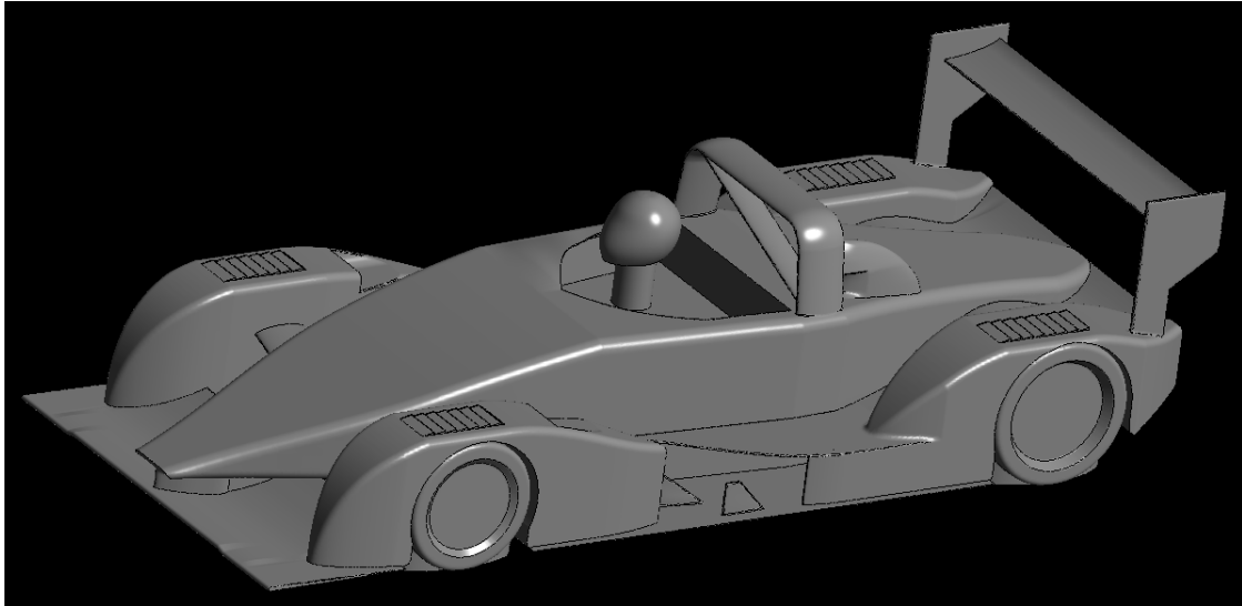
Figure 36 - Baseline Geometry (JHTT02)
