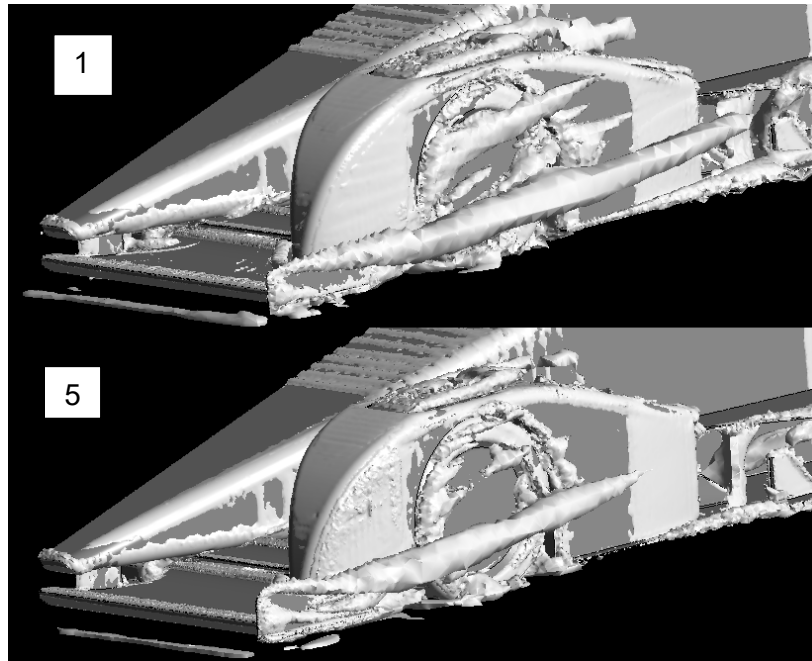
Figure 81 - End Plate Development Vortices
