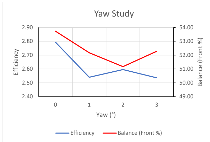
Graph 66 - Yaw Study Efficiency & Balance
