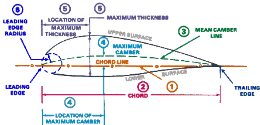
Figure 10 - Aerofoil Diagram (Birchall, 2011)
