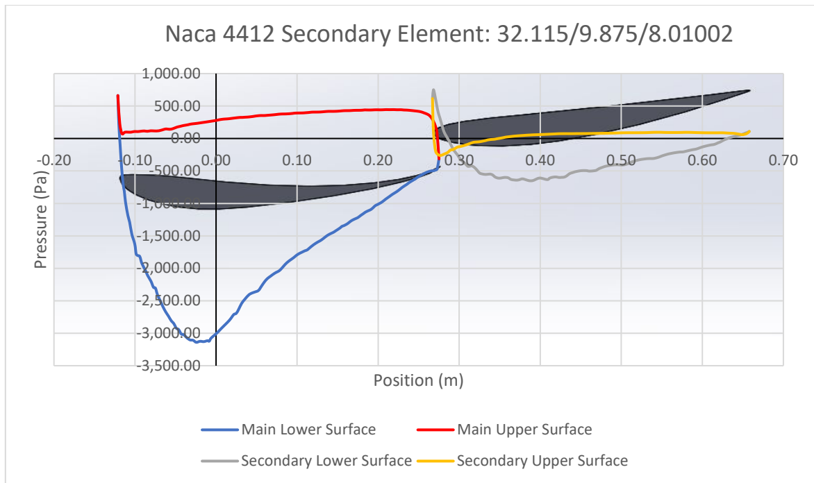
Graph 35 - Naca 4412 Secondary Element Pressure Distribution (32.115mm/9.875°/8.01002mm)
