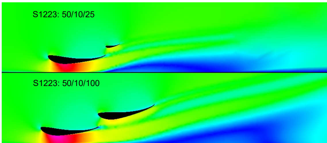
Figure 58 - S1223 Secondary Element Chord DOE Study Velocity Contours
