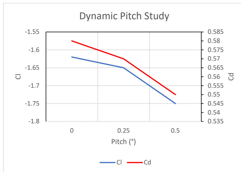
Graph 63 - Dynamic Pitch Cl & Cd
