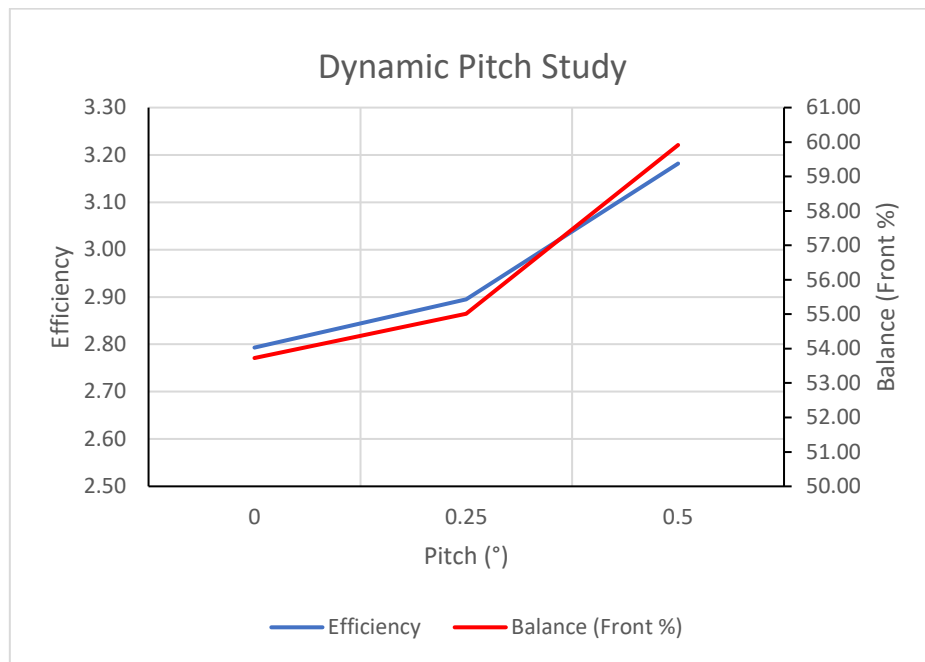
Graph 64 - Dynamic Pitch Efficiency & Balance
