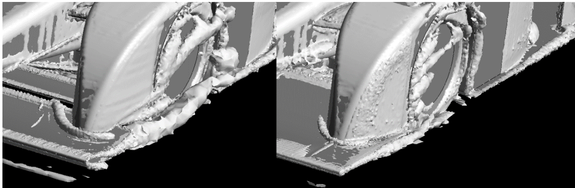
Figure 74 - New Concept & Baseline Edge Vortices
