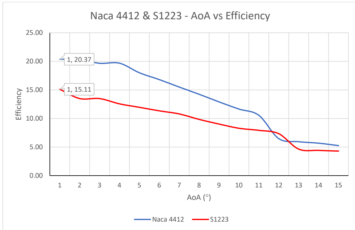
Graph 17 - Naca 4412 & S1223 - AoA vs Efficiency
