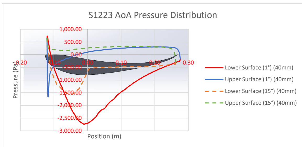
Graph 19 - S1223 Pressure Distribution (1° - 15°)
