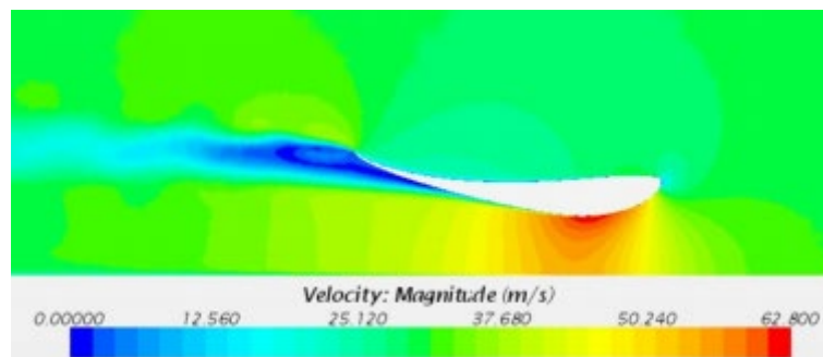
Figure 19 - Aerofoil in Ground Effect (S1223) (Mokhtar & Durrer, 2016)
