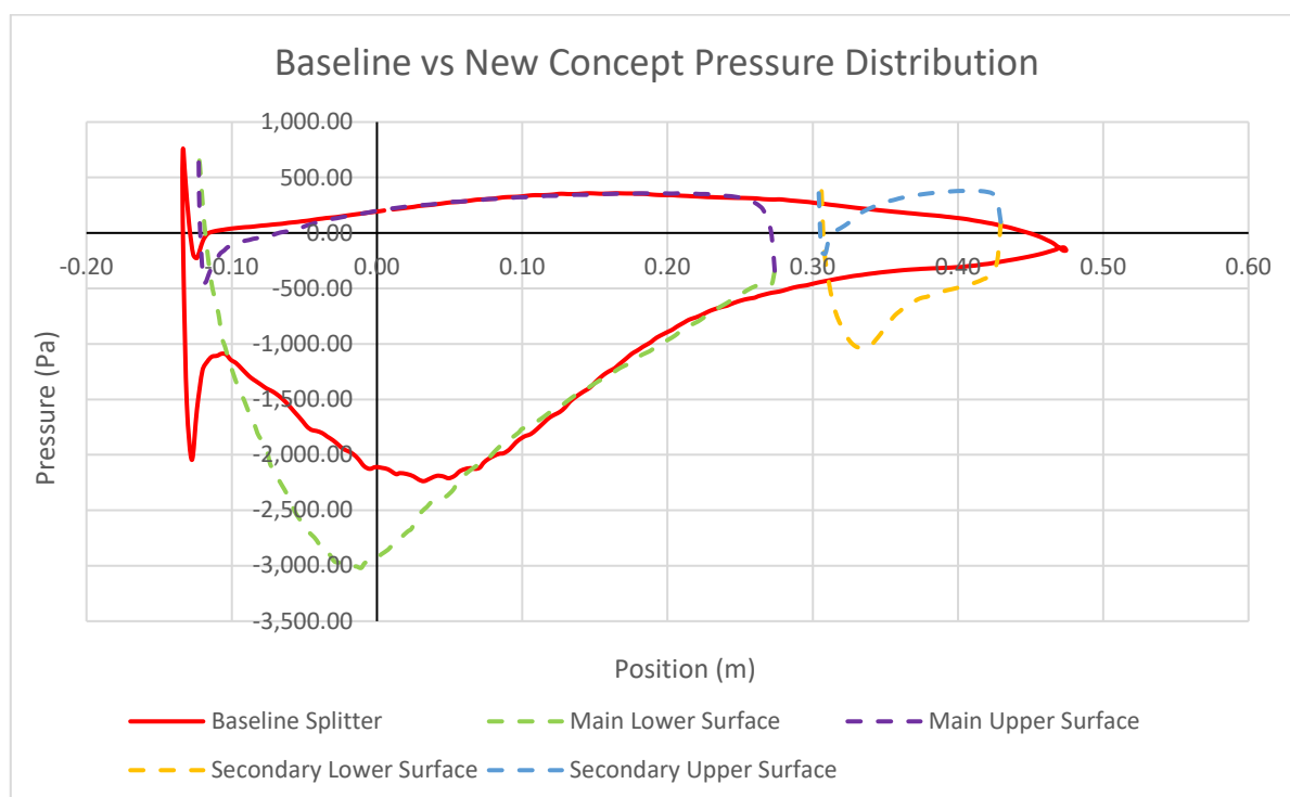
Graph 51 - Baseline vs New Concept Pressure Distribution
