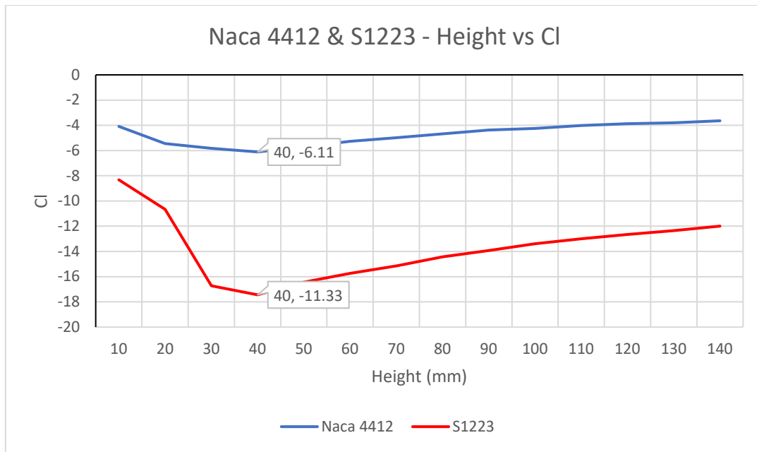
Graph 10 - Naca 4412 & S1223 - Height vs C_l
