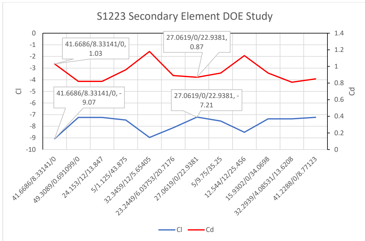
Graph 39 – S1223 Secondary Element DOE Study (CI & Cd)
