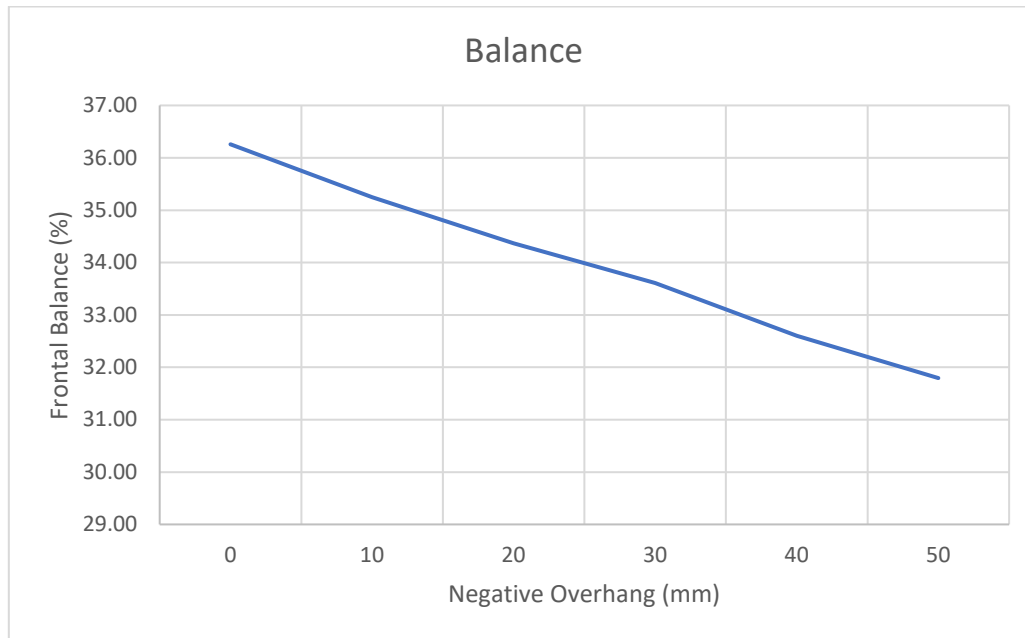
Graph 50 - Frontal Balance (%)
