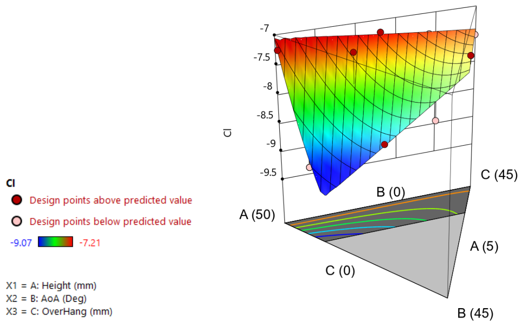
Graph 30 - S1223 Secondary Element DOE Study (Cl)
