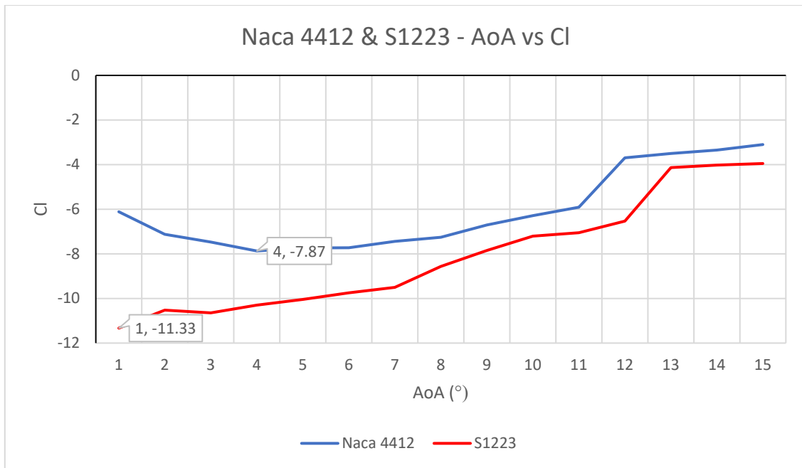
Graph 15 – Naca 4412 & S1223 – AoA vs Cl
