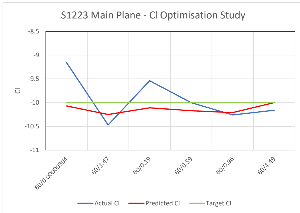
Graph 22 - S1223 Main Plane - Cl Optimisation Study
