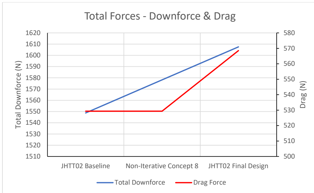
Graph 68 - Total Forces
