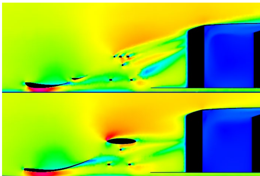
Figure 71 - New Concept vs Baseline (Velocity Contours)
