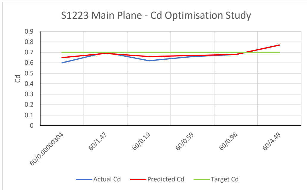
Graph 23 - S1223 Main Plane - Cd Optimisation Study
