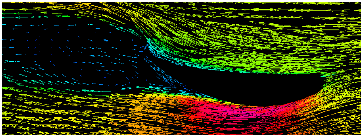
Figure 30 - Wing Lower Surface Recirculation
