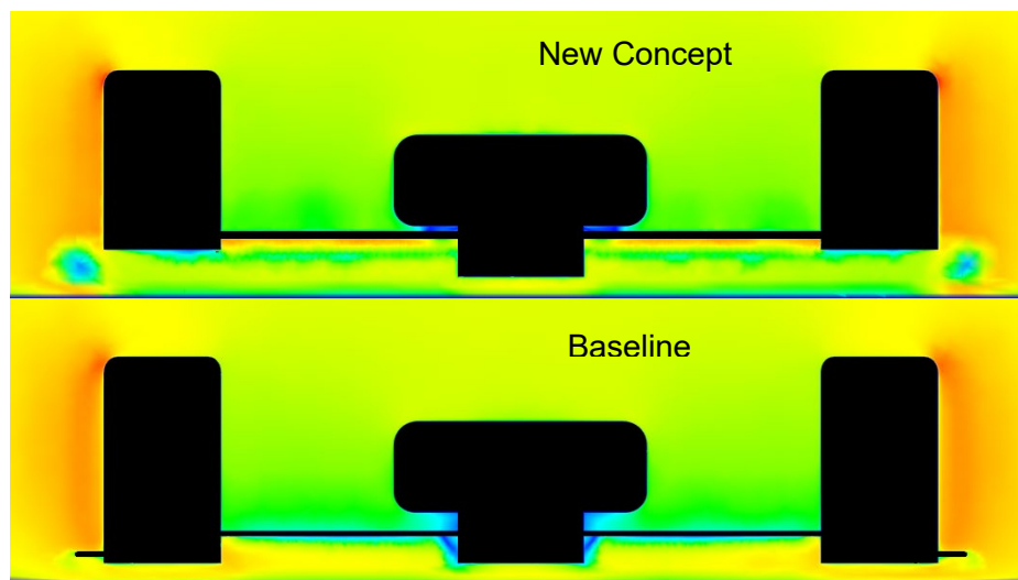
Figure 75 - Splitter Edge Vortex Velocity Contours
