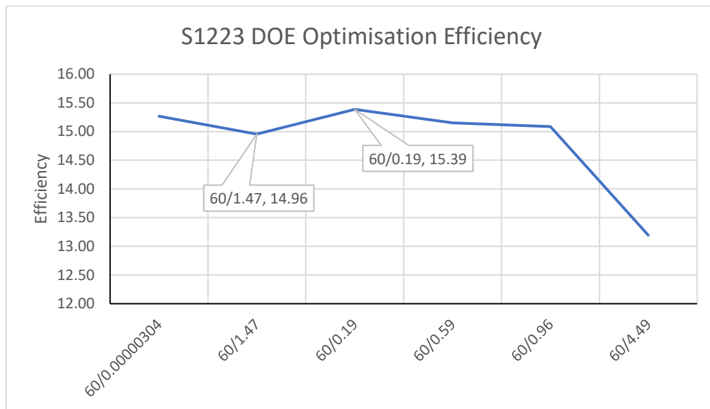
Graph 24 – S1223 Main Plane – DOE Optimisation Efficiency
