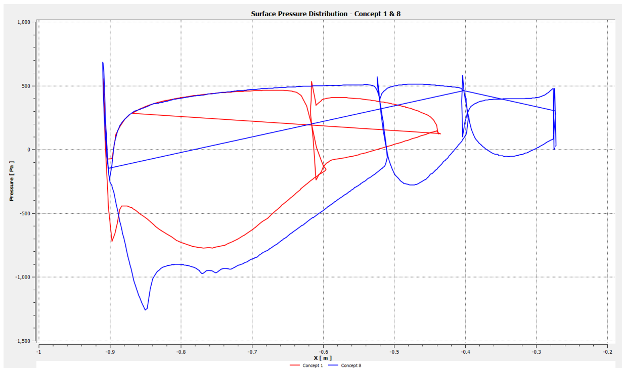
Graph 6 - Concepts 1 & 8 Surface Pressure Distribution
