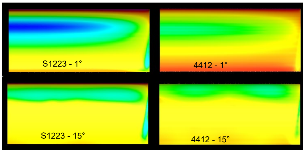
Figure 52 - Naca 4412 & S1223 Lower Surface Pressure Contours (1° - 15°)
