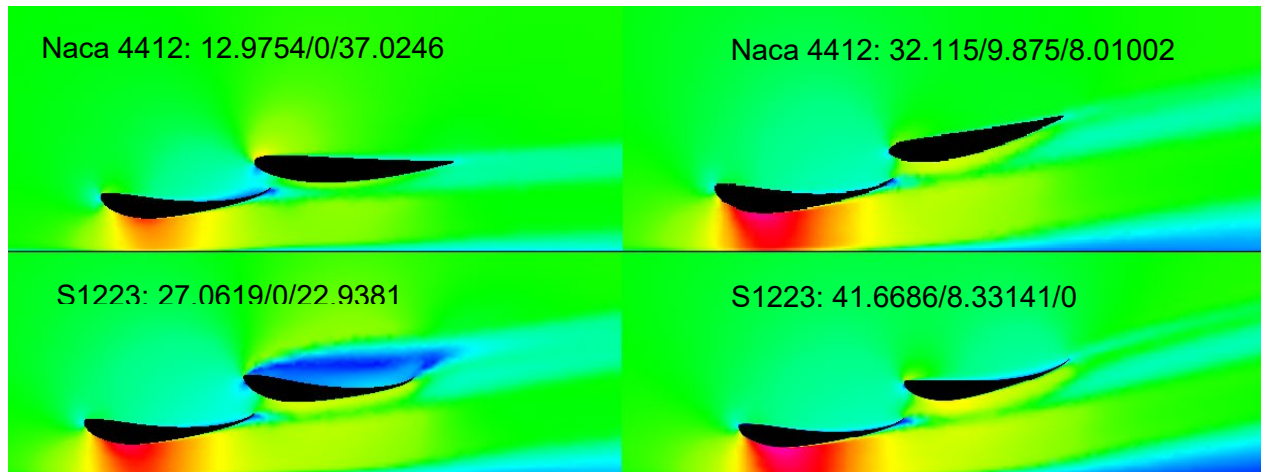
Figure 57 - Naca 4412 & S1223 Minimum & Maximum C_l Velocity Contours
