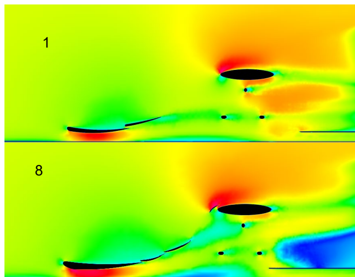
Figure 41 - Concept 1 & 8 Velocity Contours
