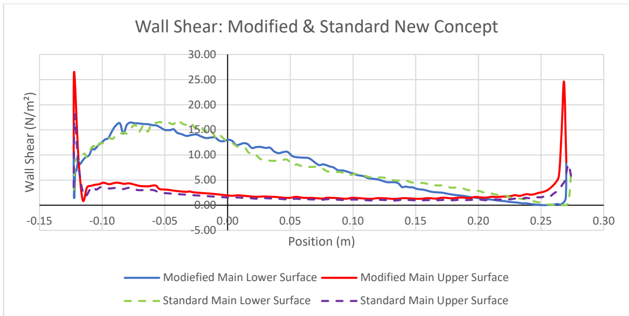
Graph 54 - Wall Shear: Modified & Standard New Concept
