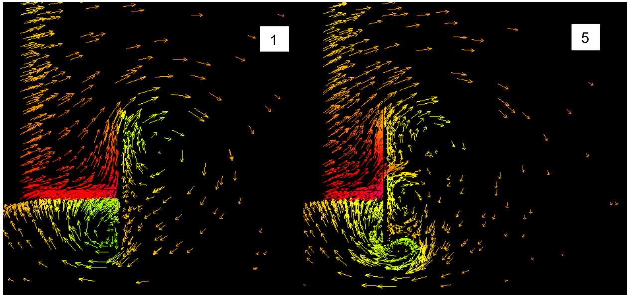
Figure 78 - End Plate Development 1 & 5 Pressure Vectors
