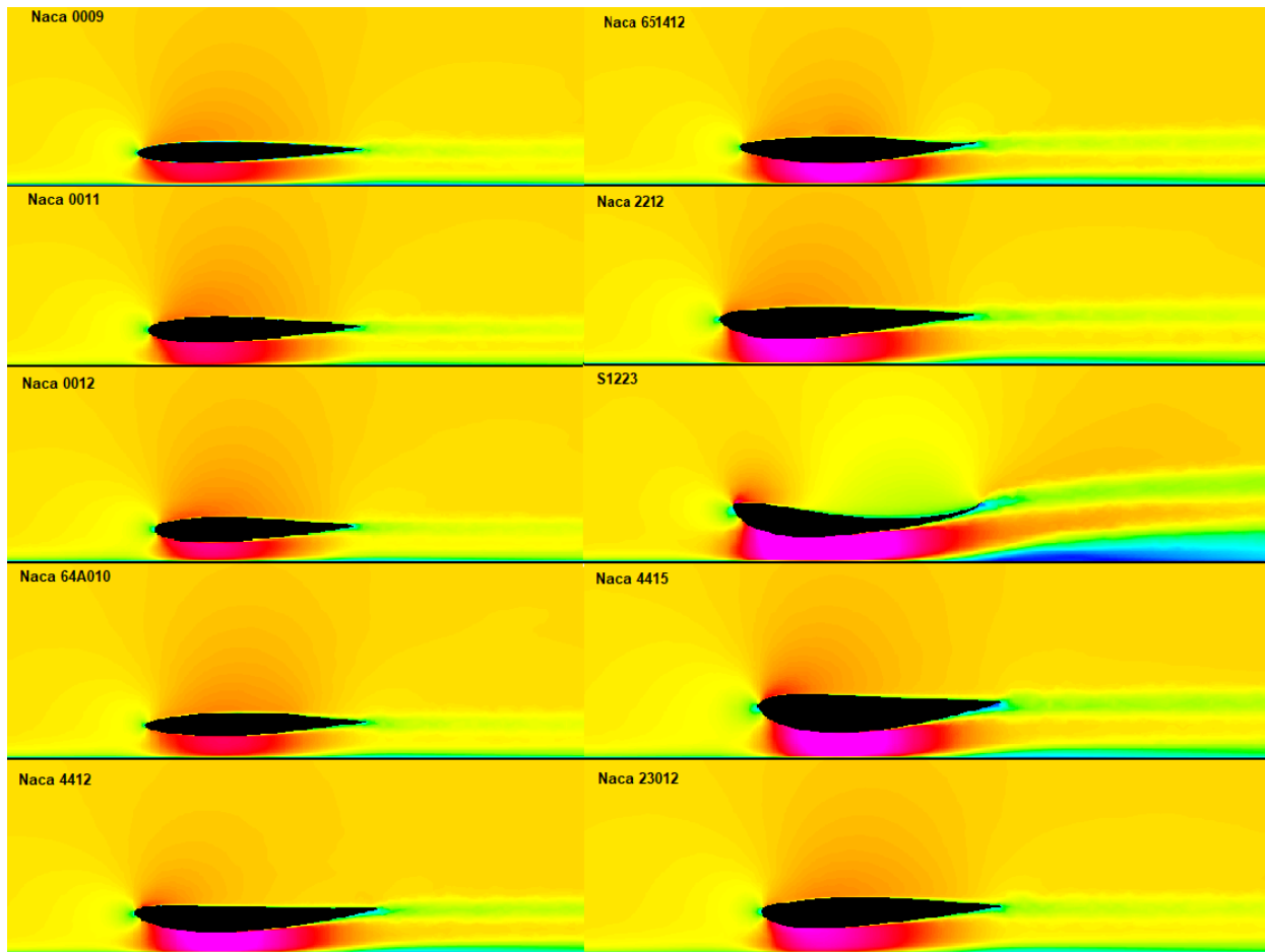
Figure 42 - Standardised Aerofoils (Velocity Contours)
