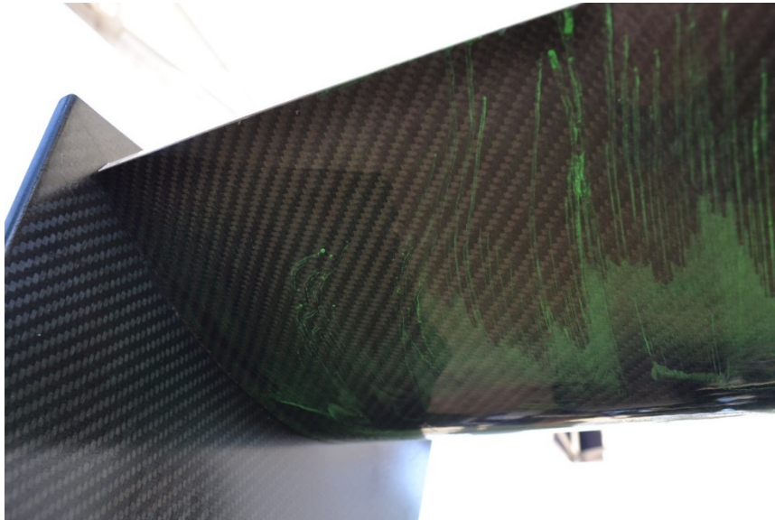
Figure 31 - MCR Sports 2000 Rear Wing Circuit Flow Visualisation Test
