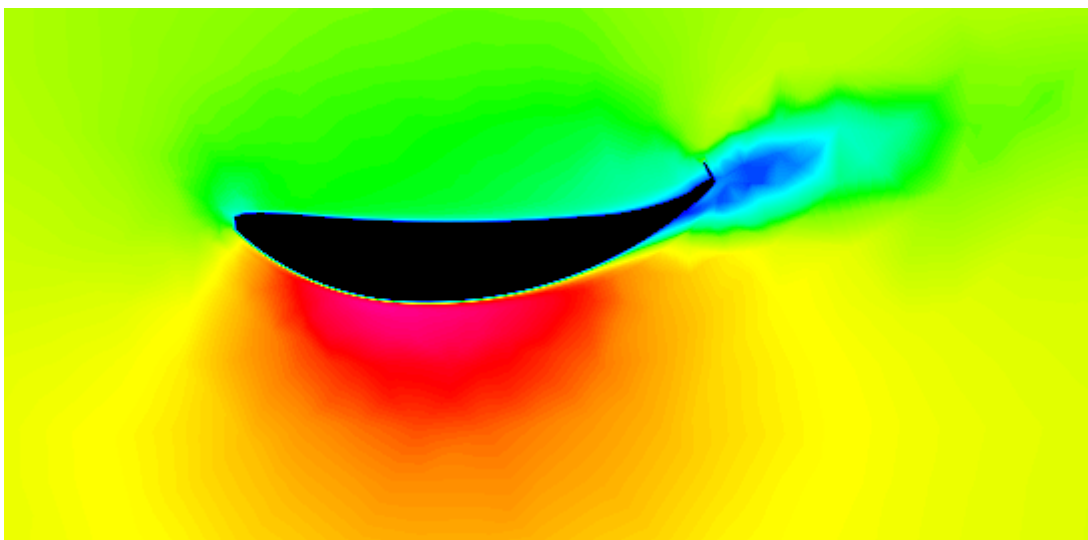
Figure 32 - MCR Sports 2000 Rear Wing Velocity Contours ( 5.1^\circ )
