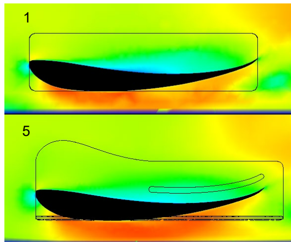
Figure 80 - Wing Edge Velocity Contours
