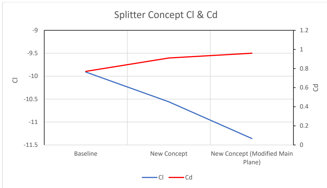
Graph 52 - Splitter Concepts CI & Cd
