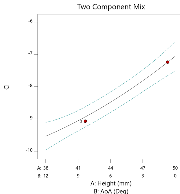
Graph 31 - S1223 Overhang Influence (Cl) (0mm Overhang)
