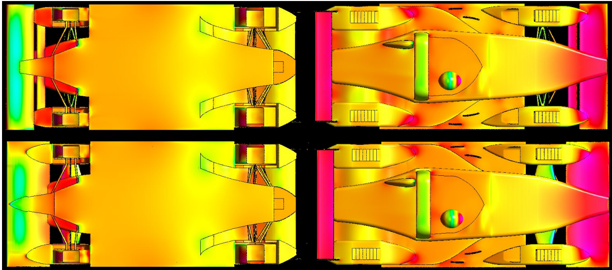
Figure 72 - New Concept vs Old Concept Pressure Contours
