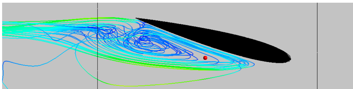
Figure 28 - Velocity Streamlines Showing Recirculation Naca 0012 (15°)
