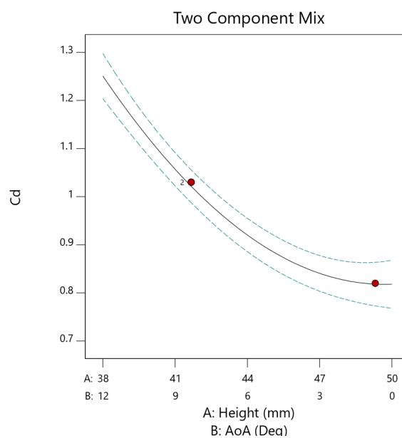
Graph 33 - S1223 Overhang Influence ( C_d ) (0mm Overhang)
