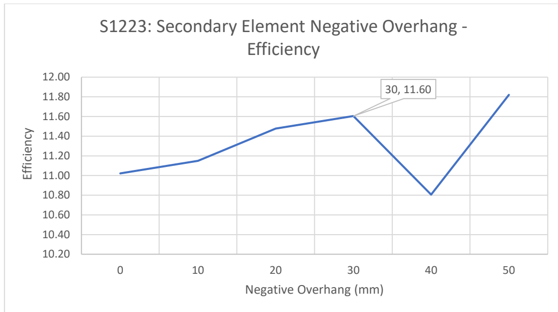
Graph 49 - S1223: Secondary Element Negative Overhang (Efficiency)
