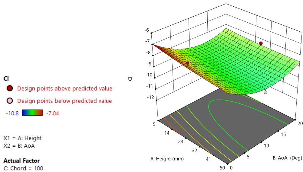
Graph 41 - S1223 Secondary Element DOE Study 2 (Cl) (100% Chord)
