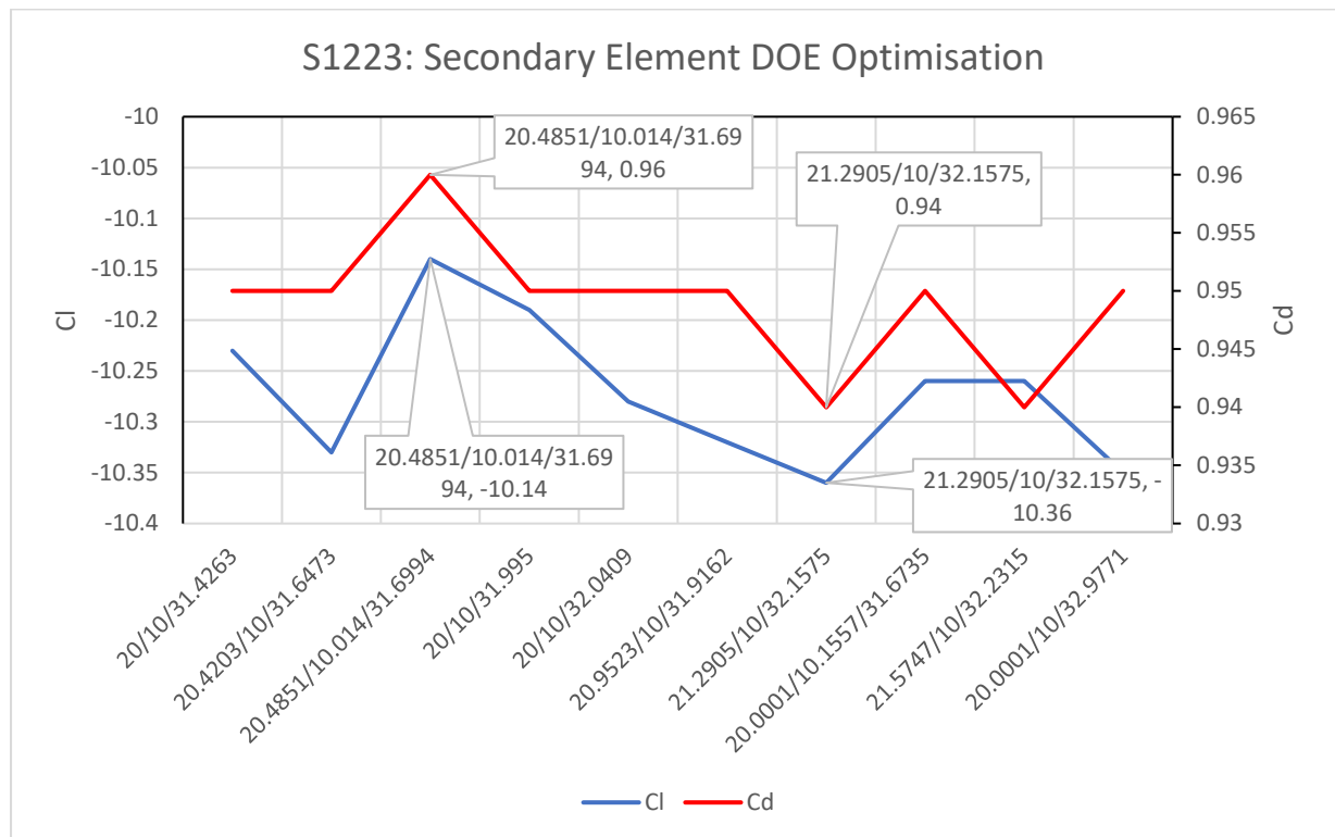
Graph 45 - S1223: Secondary Element DOE Optimisation (Cl & Cd)
