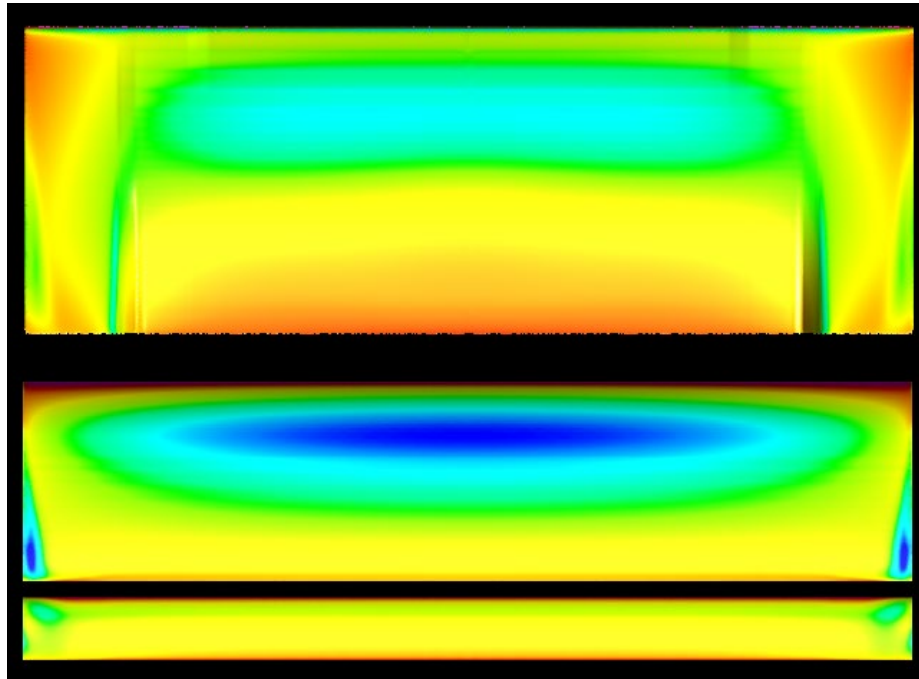
Figure 64 - Baseline Splitter vs New Concept (Lower Surface Pressure Contours)
