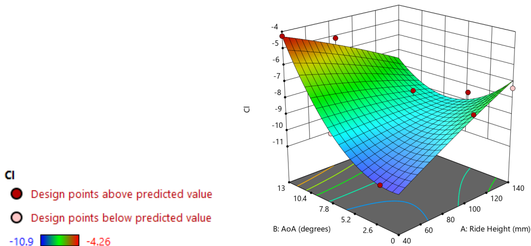
Graph 20 - S1223 Main Plane DOE Study (CI)
