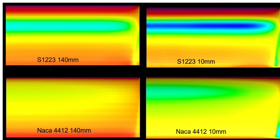
Figure 48 - Naca 4412 & S1223 Maximum & Minimum Heights (Pressure Contours)
