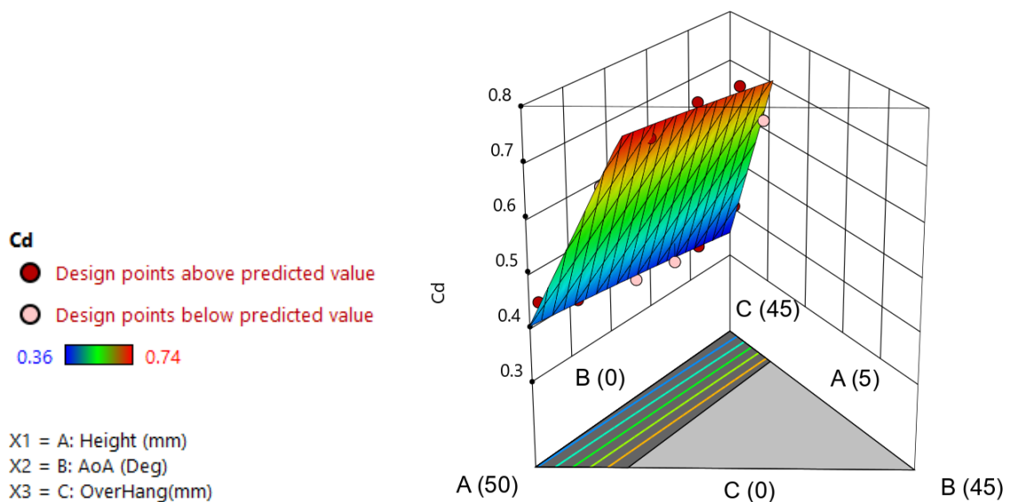
Graph 28 - Naca 4412 Secondary Element DOE Study ( C_d )
