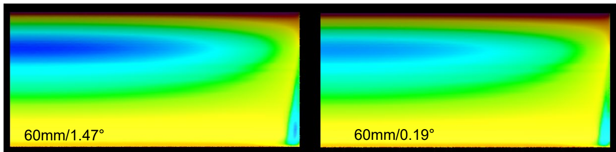
Figure 56 - S1223 Main Plane DOE Optimisation Lower Surface Pressure Contours
