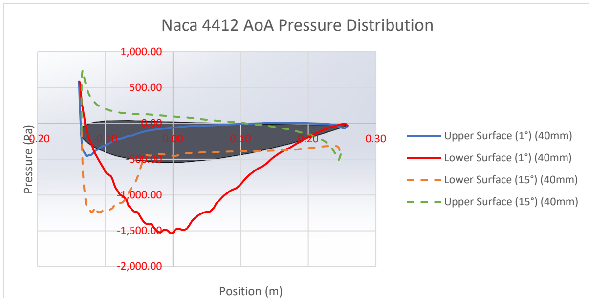
Graph 18 - Naca 4412 Pressure Distribution (1° - 15°)
