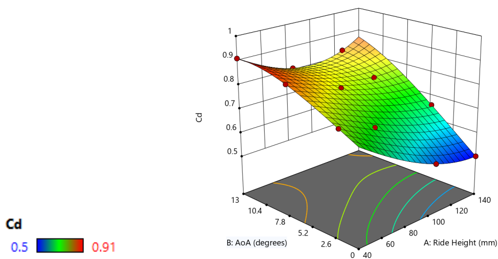
Graph 21 - S1223 Main Plane DOE Study (Cd)
