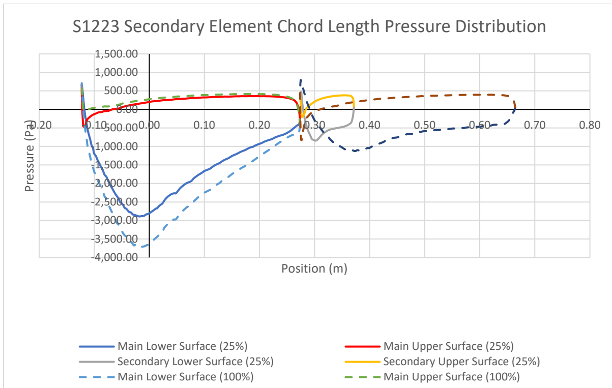
Graph 44 - S1223 Secondary Element Chord Length Pressure Distribution
