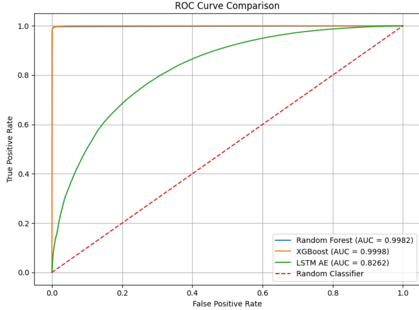
Figure 8: ROC Curve
