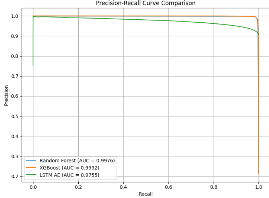
Figure 9: Precision-Recall Curve
