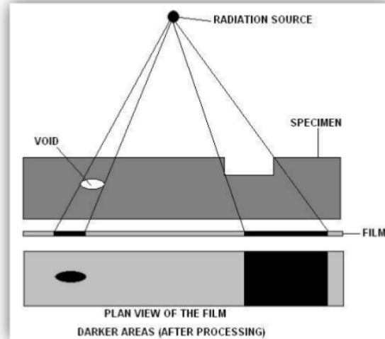
Figure 1 Radiography film-based technique (www.ndtdavari.com, 2019)
