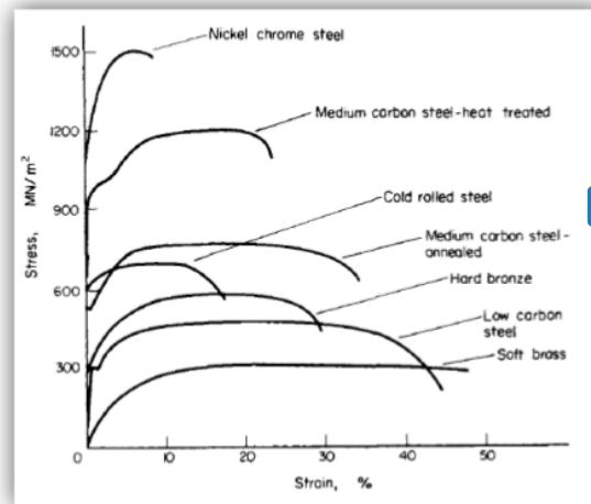
Figure 9 Stress Strain Graph (Hearn, E. J., 1997)
