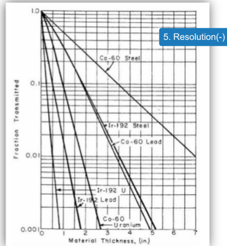
Figure 3 Radiographical material conductance chart (E. Mix, 2005)
