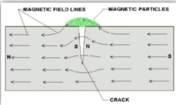
Figure 7 MPI diagram (nde-ed.org, 2019)
