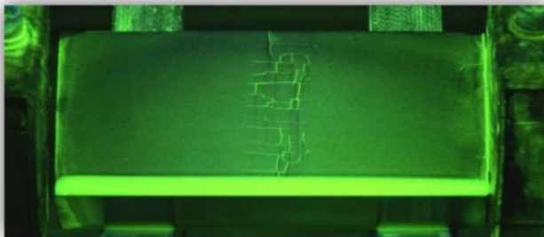
Figure 8 Test piece with fluorescent magnetic dye applied (Materialscience2000, 2014)
