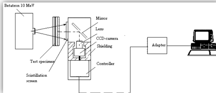
Figure 2 Radiography digital technique (ndt.net, 2014)
