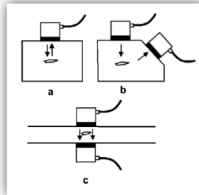
Figure 4 UT setup examples (Schmerr, 2016)
