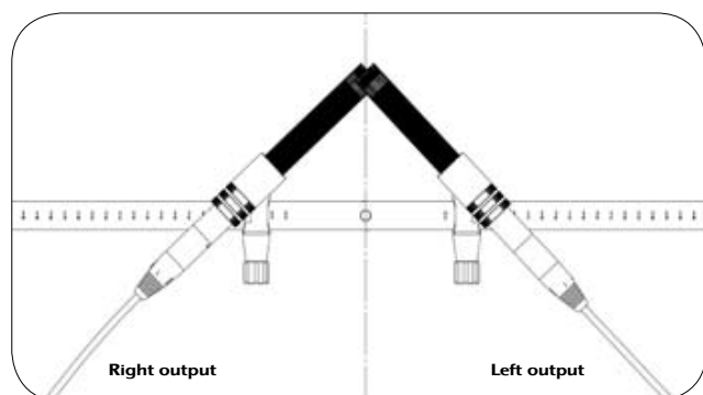
Fig. 12: XY setup
