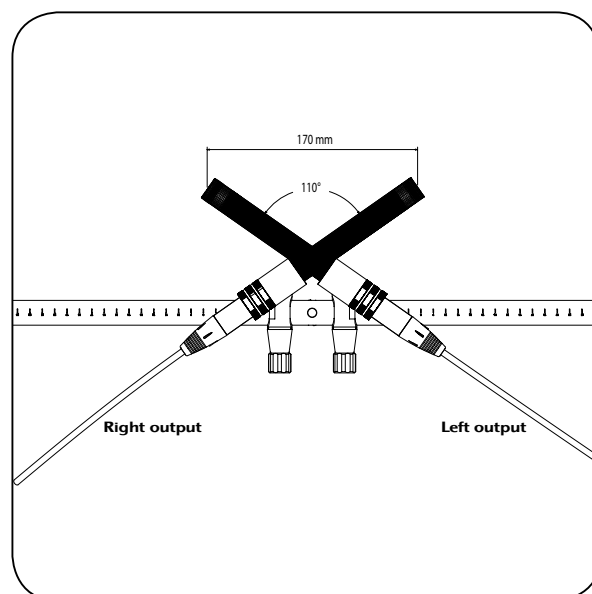
Fig 22: ORTF setup
