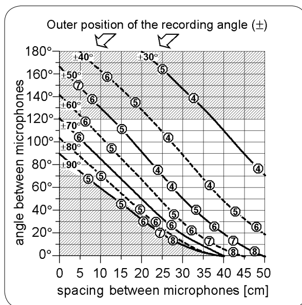
Fig. 20 Near coincident setup using first order cardioid microphones.
