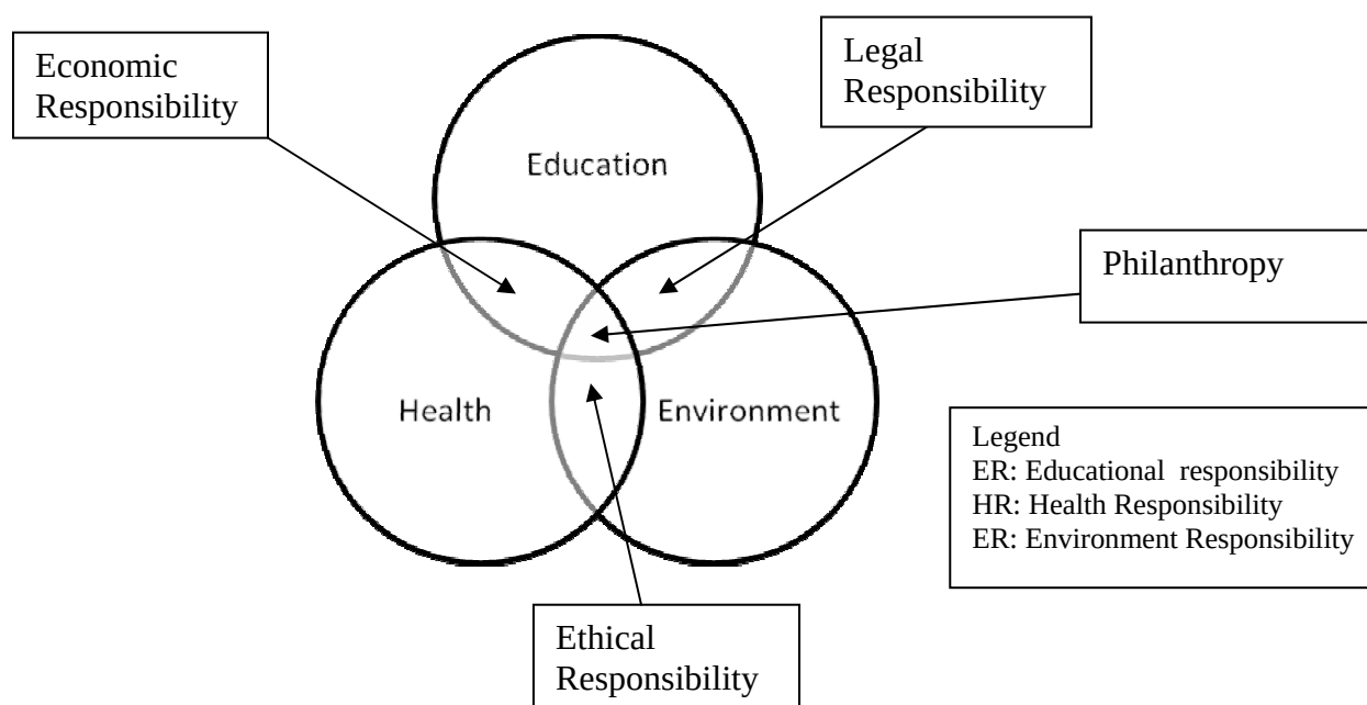
Figure 2: CSR model
