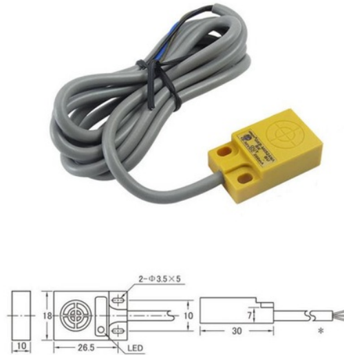
Figure 33 - GKB-M0524NA Inductive Proximity Sensor Dimensions (Hugong Automation, 2019)
