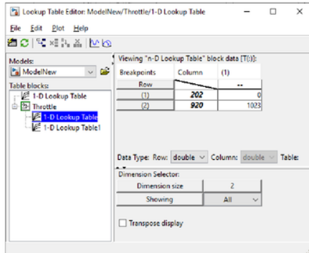
Figure 44 - Signal 1 Lookup Values
