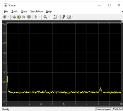
Figure 51 - Throttle Signal 1 Floating Without Pull-Down Resistor
