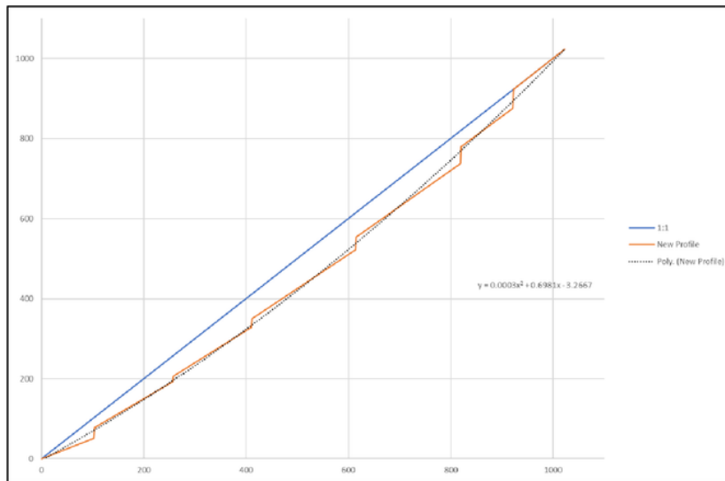
Figure 48 - Throttle Profile Calculator Graph
