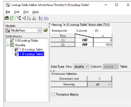
Figure 45 - Signal 2 Lookup Values
