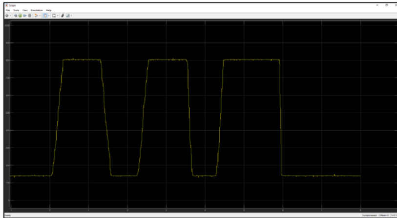
Figure 53 - 2010 Triumph Daytona 675 Throttle Position Signal
