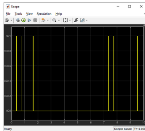
Figure 39 - Throttle Signal 1, 100% Opening
