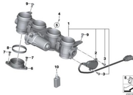
Figure 8 - 2017 BMW S1000RR Throttle Bodies Parts Diagram (Max BMW Motorcycles, 2019)
