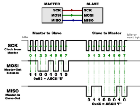
Figure 22 - SPI Master / Slave Interface (SparkFun, 2019)
