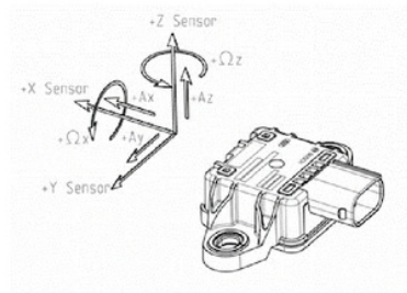
Figure 14 – IMU Sensor (Bosch, 2019)
