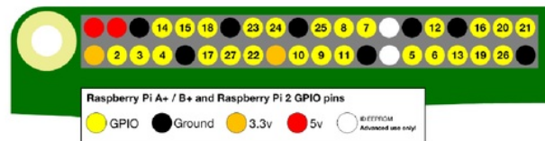
Figure 28 - Raspberry Pi 3 Model B+ GPIO Pin Map (Raspberry Pi Foundation, 2019)
