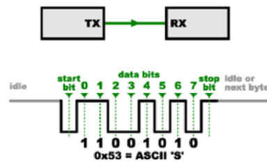
Figure 20 - Serial Asynchronous Data Transfer (SparkFun, 2019)
