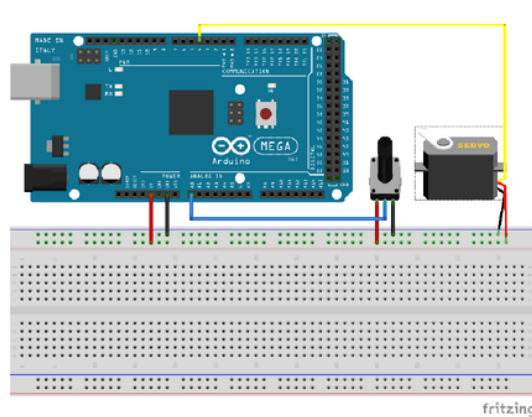
Figure 36 - Initial Throttle Wiring Diagram
