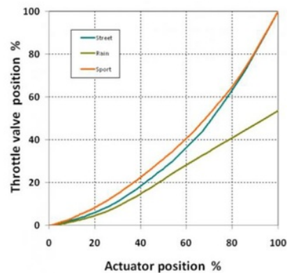
Figure 9 - 2014 KTM 1290 Super Duke R Throttle Maps (Motorcycle.com, 2013)
