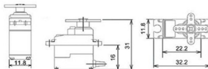
Figure 31 - Servo Motor SG-90 Dimensions (Components101, 2017)
