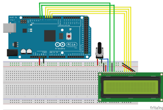
Figure 50 – LCD Wiring Diagram
