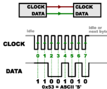
Figure 21 - SPI Synchronous Data Transfer (SparkFun, 2019)
