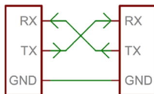
Figure 19 - Serial Connectivity (SparkFun, 2019)
