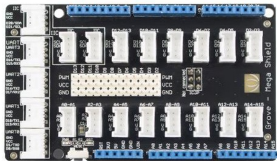
Figure 29 - Grove - Mega Shield V1.2 (Arduino, 2019)
