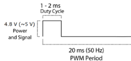
Figure 32 - Servo Motor SG-90 PWM (Components101, 2017)
