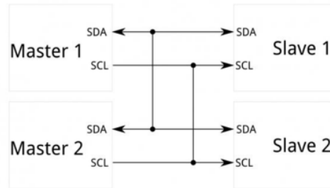
Figure 23 - I 2 C Master / Slave Interface (SparkFun, 2019)
