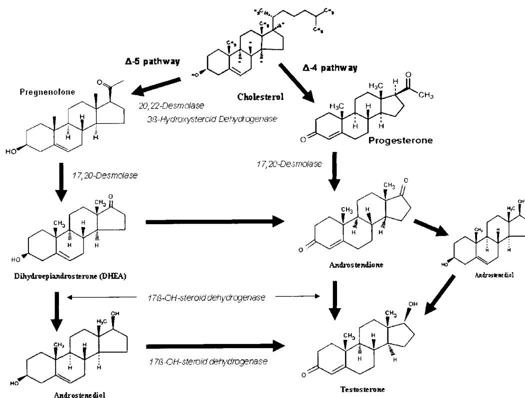
Figure 1. Testosterone synthesis.
