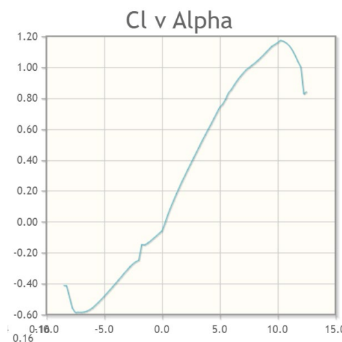
Figure 2: Coefficient of lift v Angle of Attack for the aerofoil used
