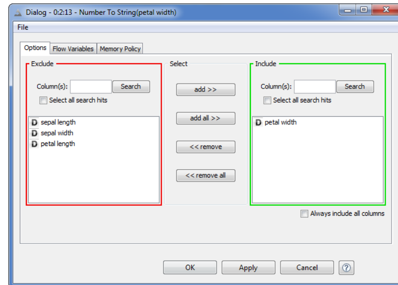
3.15. Configuration window of the “Number To String” node
