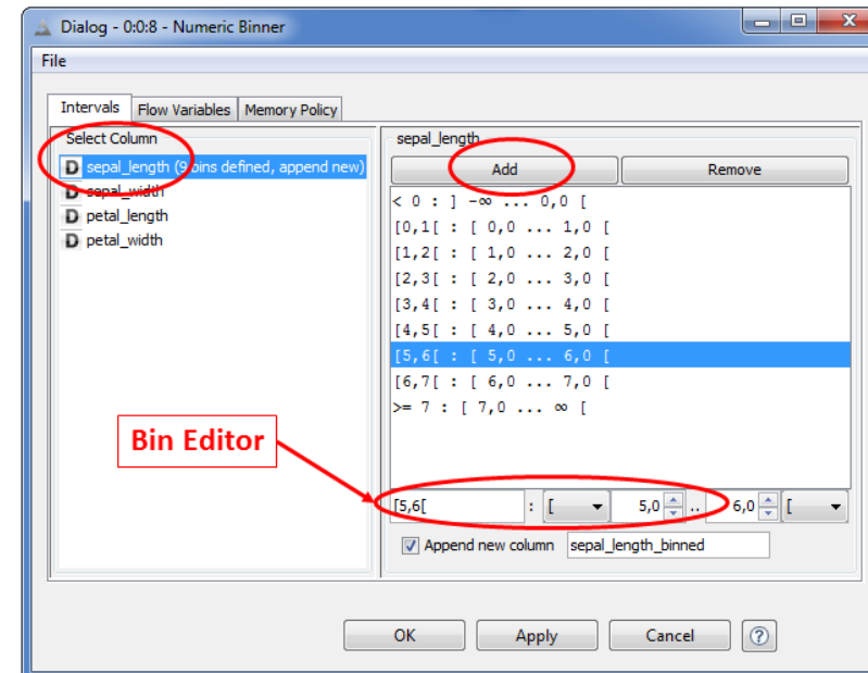
3.35. Configuration window for the „Numeric Binner“ node
