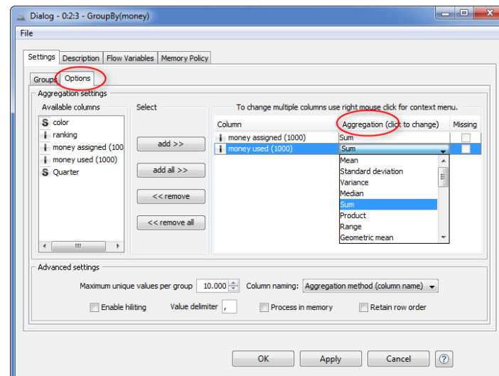
5.5. Configuration window for the “GroupBy” node: tab “Options”
