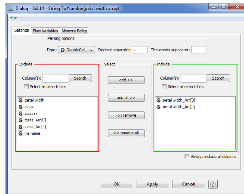
3.16. Configuration dialog of the “String To Number” node
