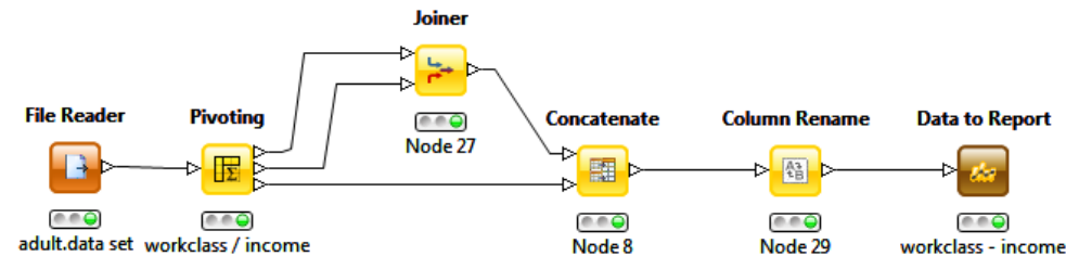
5.35. Exercise 2: The workflow
