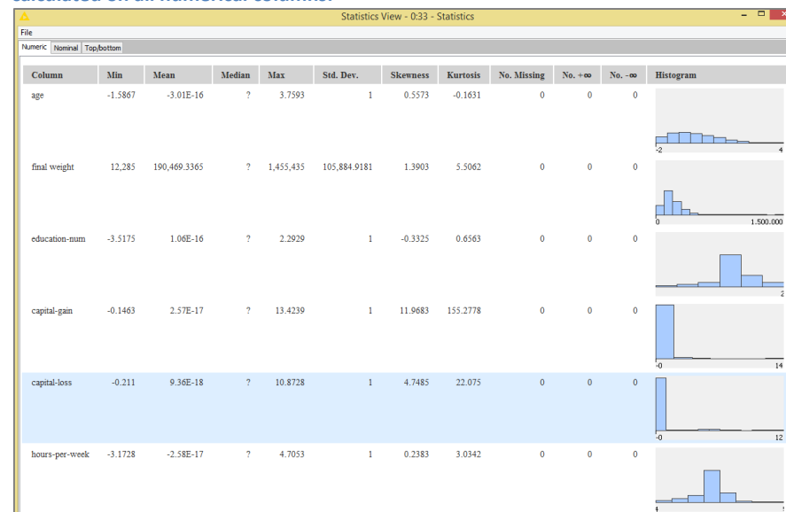
4.42. The “Numeric” tab of the “Statistics” node view displays statistical measures and histogram calculated on all numerical columns.
