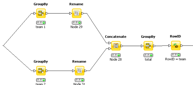
5.37. Meta-node "# scored goals"/"# taken goals"
