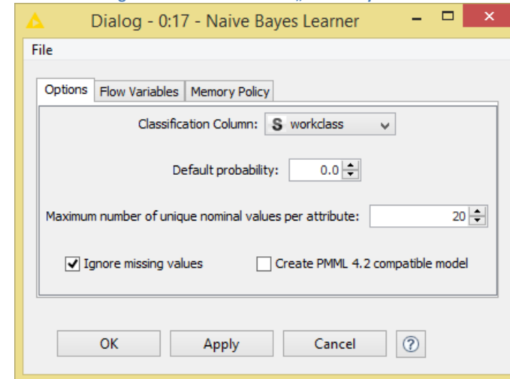
4.11. Configuration window for the „Naive Bayes Learner“ node
