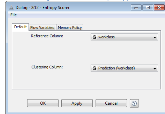
4.28. The configuration window of the „Entropy Scorer“ node
