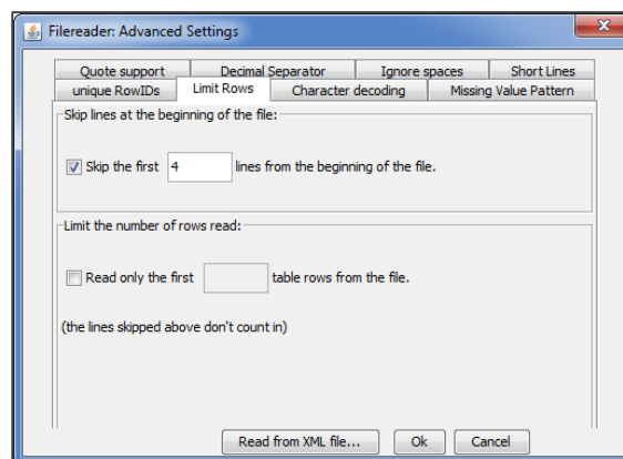
2.19. Advanced settings: Limit Rows
