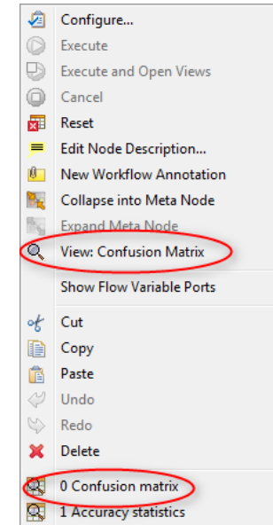
4.18. The context menu of the “Scorer” node
