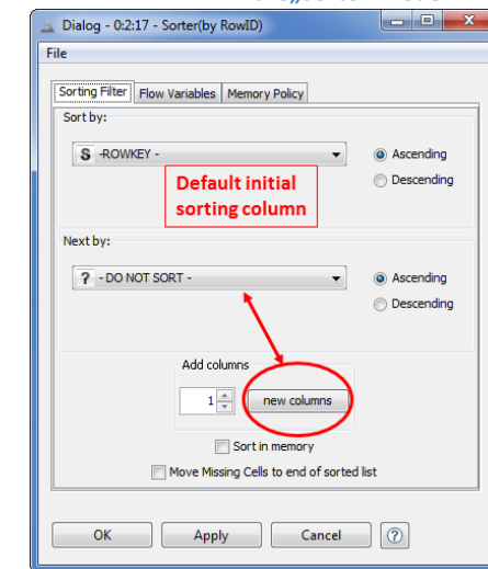
5.15. Configuration window for the „Sorter“ node
