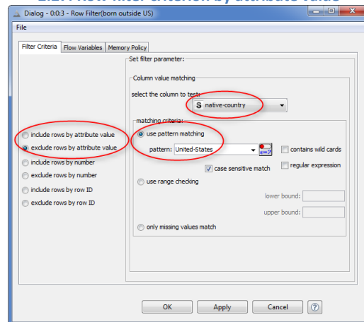
2.27. Row filter criterion by attribute value
