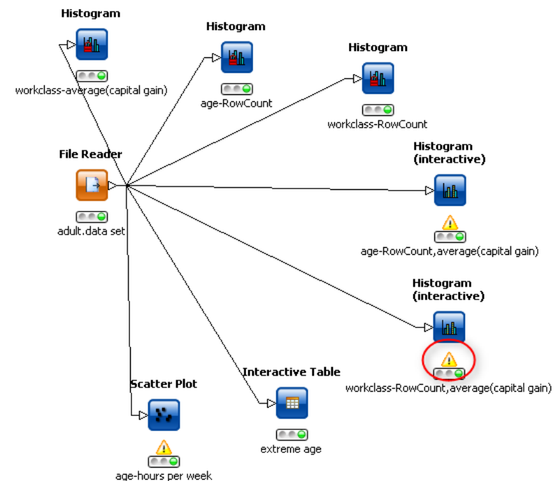
3.53. Exercise 3: Workflow
