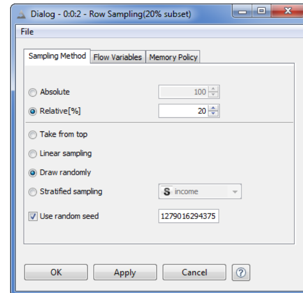
4.1. Configuration window for the “Row Sampling” node
