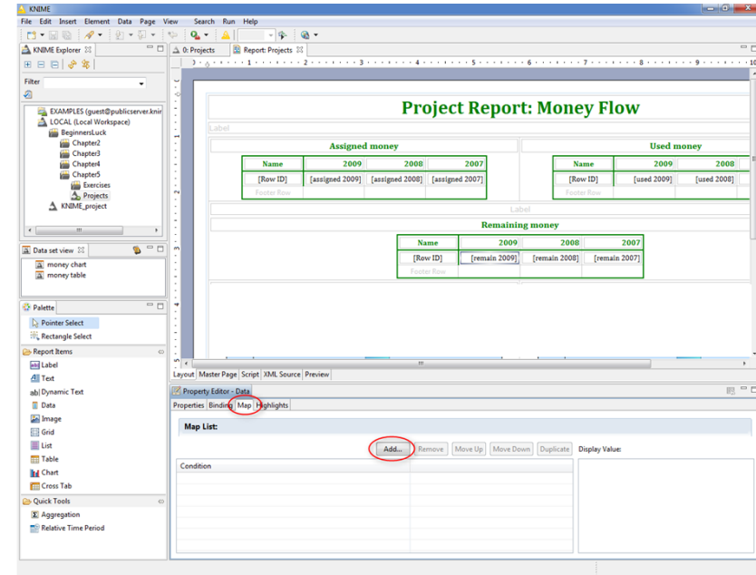
6.16. The Tab „Maps“ in the table Properties Editor defines text mapping for a table item
