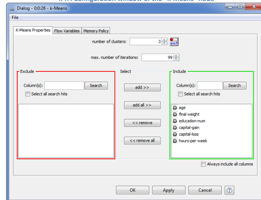
4.47. Configuration window of the “k-Means” node
