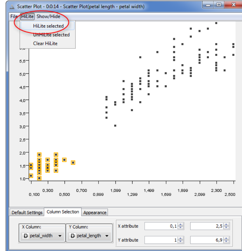
3.30. View of the „Scatter Plot“ node: “Column Selection” tab and “HiLite” menu
