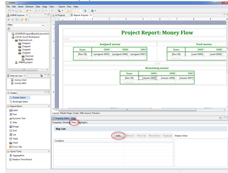
6.18. The „Highlights” tab in The Properties Editor defines conditional properties for a table item
