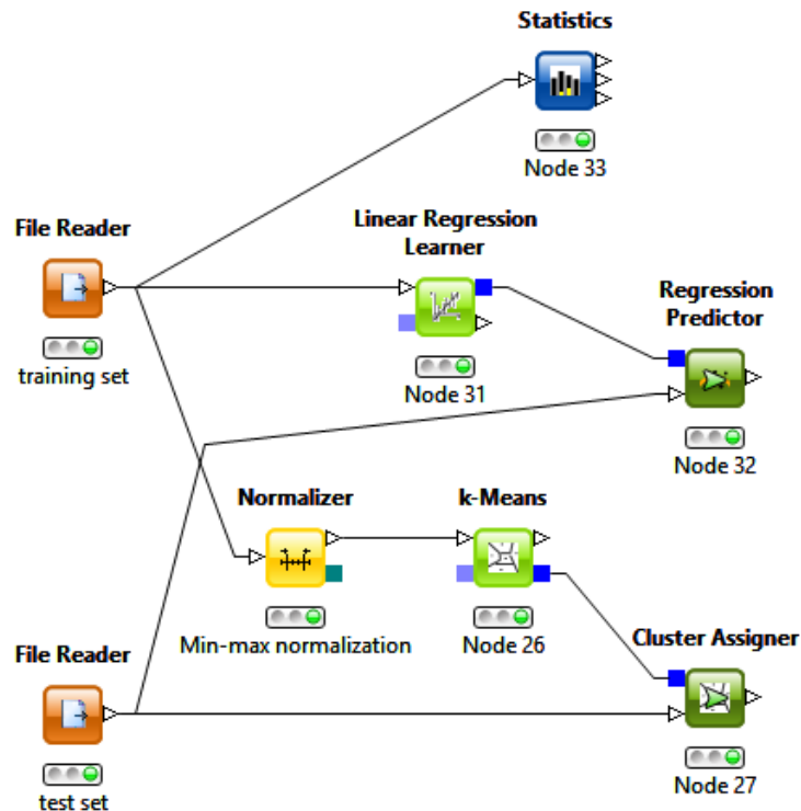
4.48. Workflow „Clustering and Regression“
