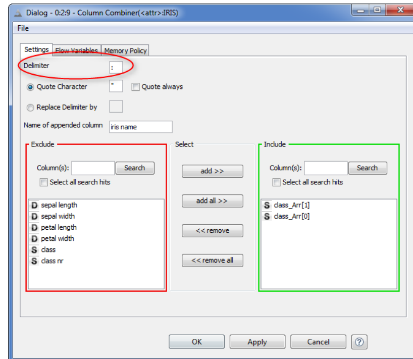
3.12. Configuration window for the „Column Combiner“ node
