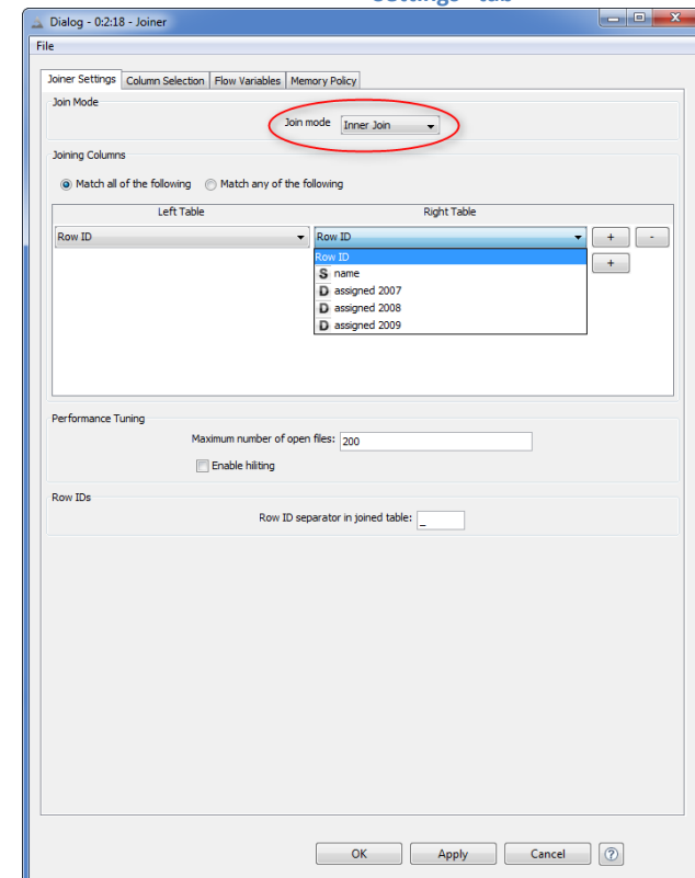
5.19. Configuration window for the „Joiner“ node: “Joiner Settings” tab
