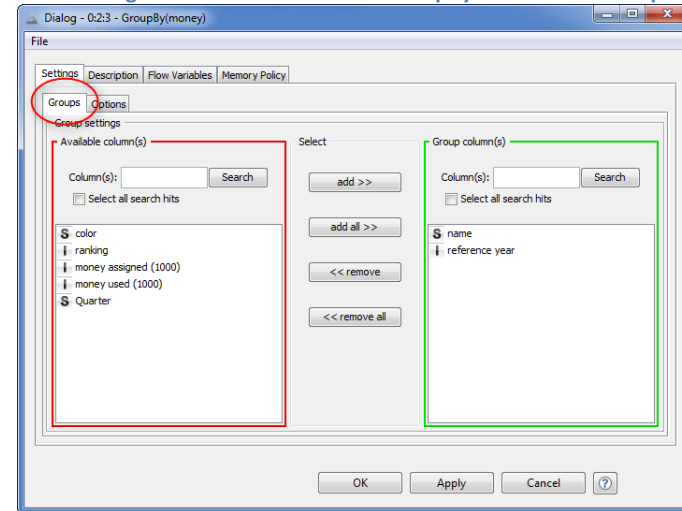
5.4. Configuration window for the “GroupBy” node: tab “Groups”
