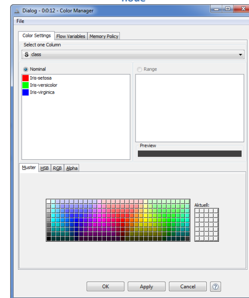
3.41. Configuration window of the „Color Manager” node
