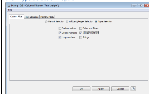
2.24. Configuration window of “Column Filter” node: the “Type Selection” option
