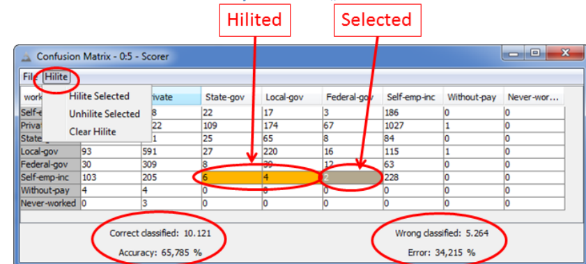
4.19. Hilite functionality of window „View: Confusion Matrix”
