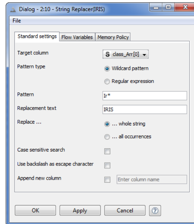
3.11. Configuration window for the „String Replacer“ node
