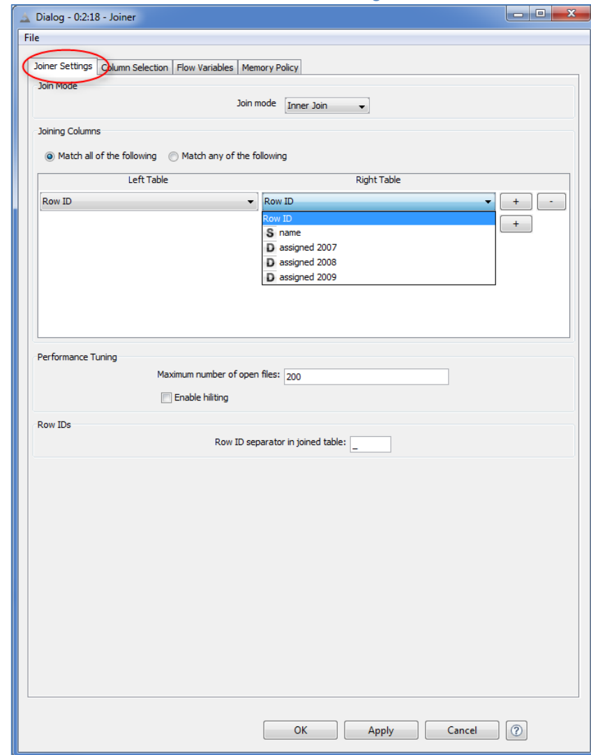
5.18. Configuration window for the „Joiner“ node, which includes two tabs to be filled in: “Joiner Settings” and “Column Selection”
