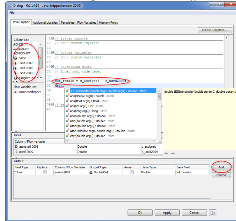
5.24. Configuration window for the “Java Snippet” node
