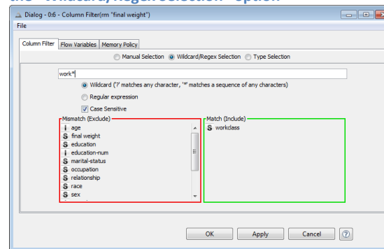
2.23. Configuration window of “Column Filter” node: the “Wildcard/Regex Selection” option
