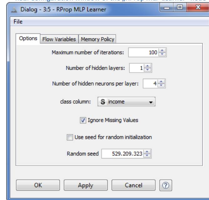
4.32. Configuration window of the „RProp MLP Learner“ node
