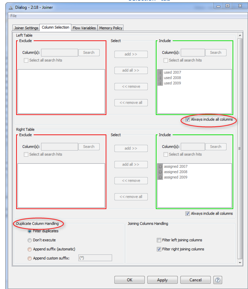
5.20. Configuration window for the „Joiner“ node: “Column Selection” tab
