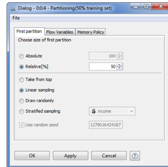
4.2. Configuration window of the "Partitioning" node
