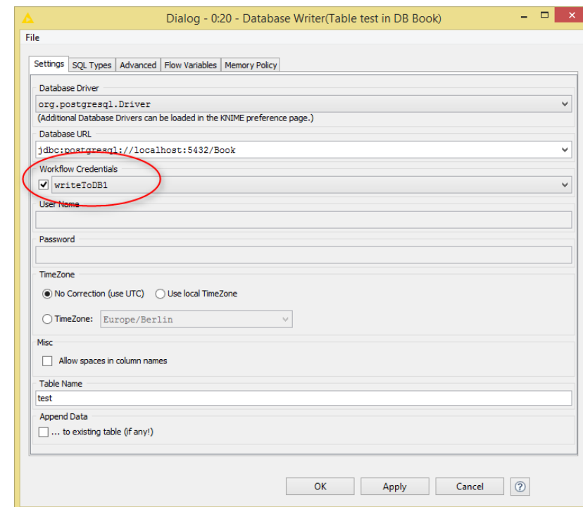
3.18. Configuration window of the „Database Writer“ node
