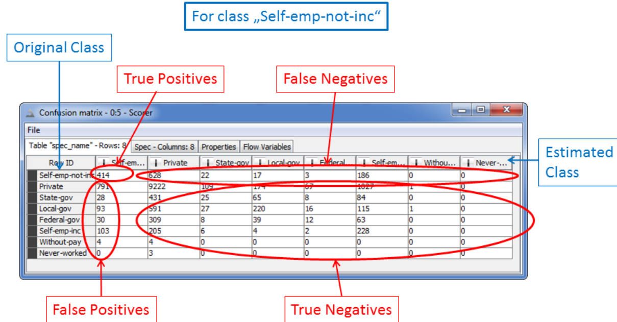
4.16. True Positives, False Negatives, True Negatives, and False Positives in the Confusion Matrix for the class “Self-emp-not-inc”.
