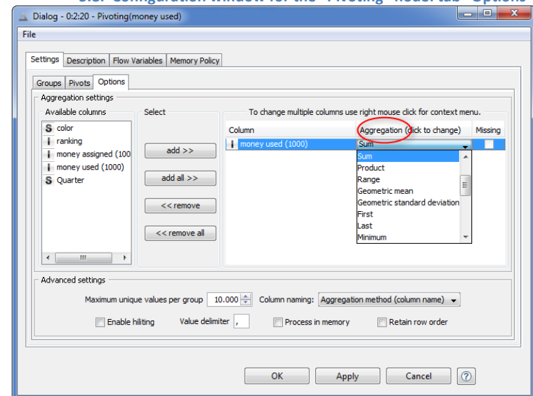
5.8. Configuration window for the "Pivoting" node: tab "Options"
