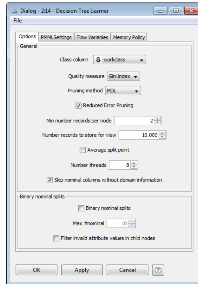
4.22. Configuration window for the „Decision Tree Learner“ node
