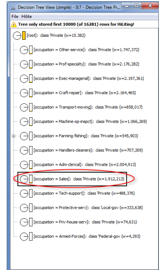
4.27. „Decision Tree View (simple)“ window
