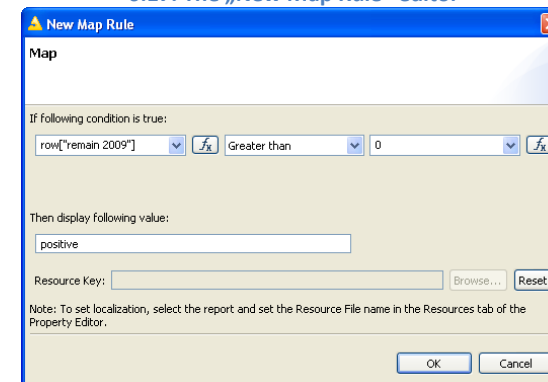
6.17. The „New Map Rule“ editor
