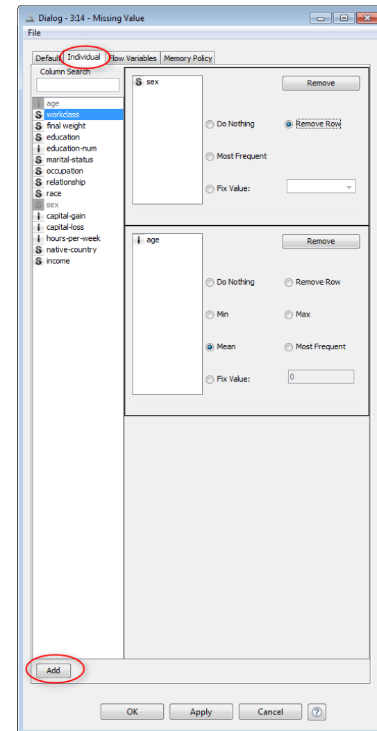
4.7. Configuration window for „Missing Value“ node: Tab “Individual”
