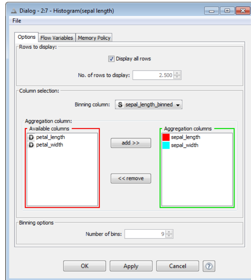
3.36. Configuration window of the „Histogram“ node
