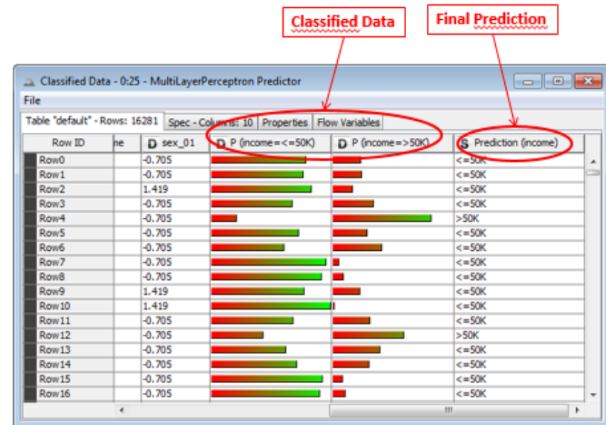
4.34. Output Data Table of the „Multilayer Perceptron Predictor“ node
