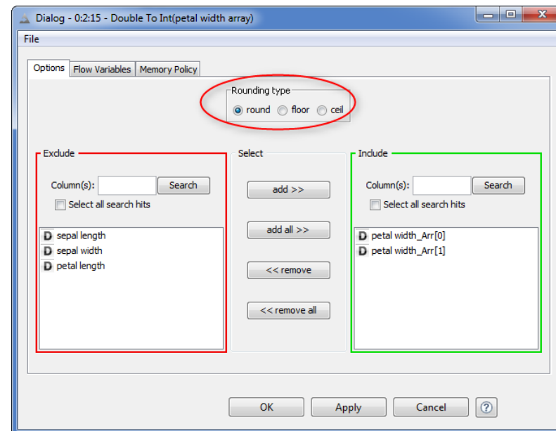
3.17. Configuration window of the “Double To Int” node
