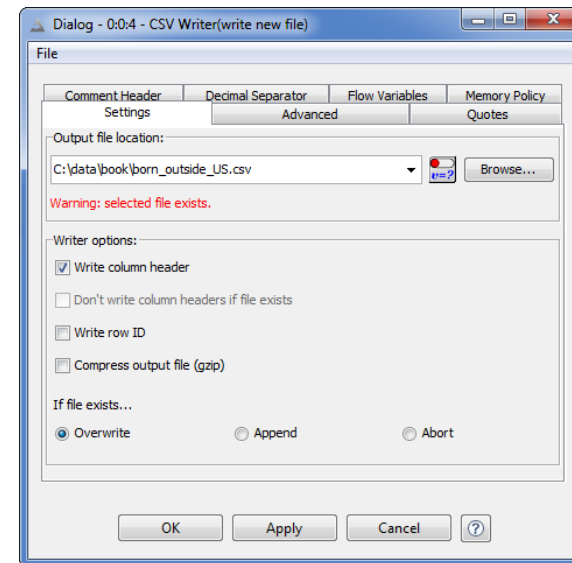
2.32. Configuring a “CSV Writer” node
