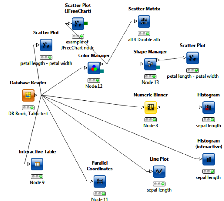
3.48. The final version of the "my_first_data_exploration" workflow
