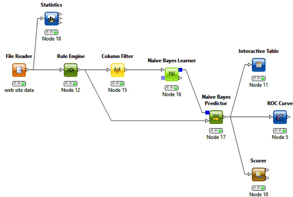
4.54. Exercise 3: workflow
