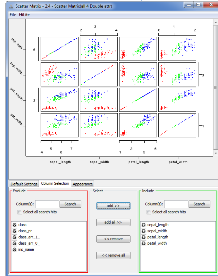
3.42. View of the “Scatter Matrix” plot with customized colors
