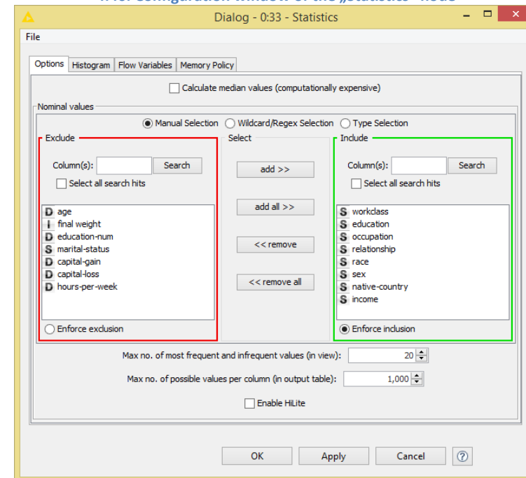
4.40. Configuration window of the „Statistics“ node
