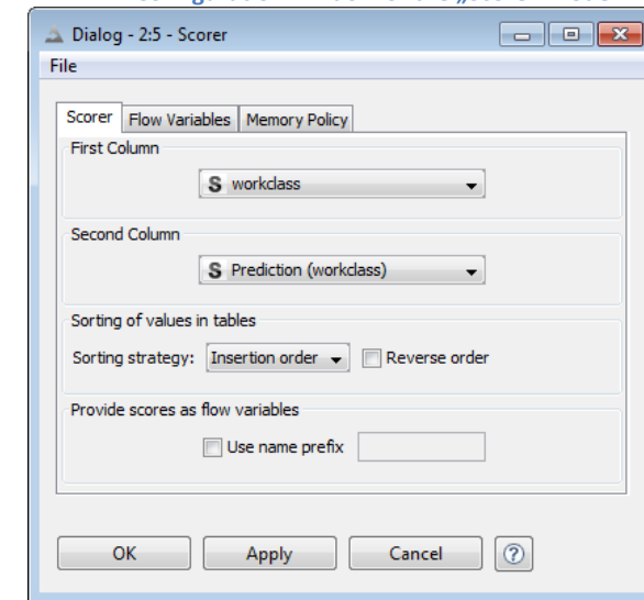
4.14. Configuration window of the „Scorer“ node
