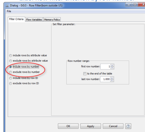
2.28. Row filter criterion by row number
