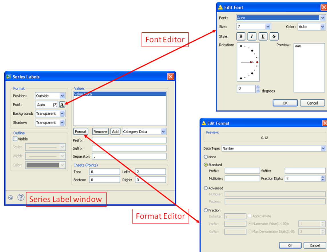
6.31. The „Series Labels“ window. The „A“ button opens the “Font Editor”. The “Format” button opens the “Format Editor”
