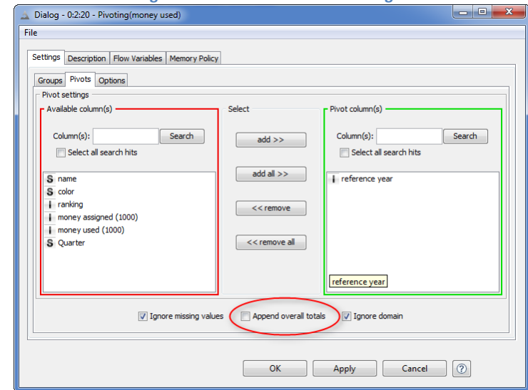
5.7. Configuration window for the "Pivoting" node: tab "Pivots"
