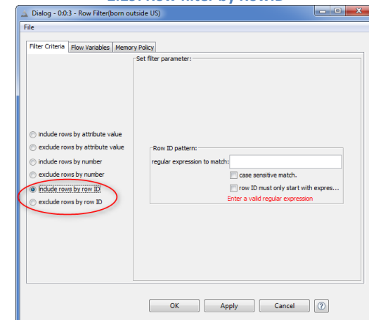
2.29. Row filter by RowID
