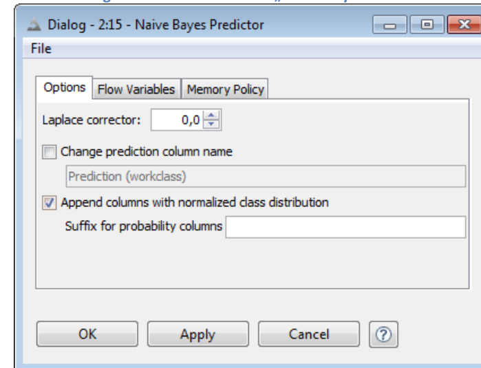
4.12. Configuration window for the „Naive Bayes Predictor“ node
