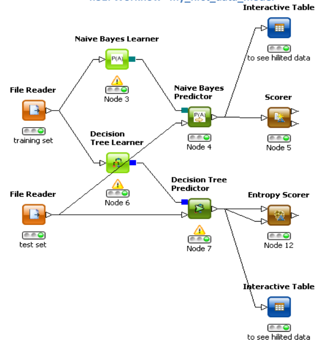
4.31. Workflow "my_first_data_model"
