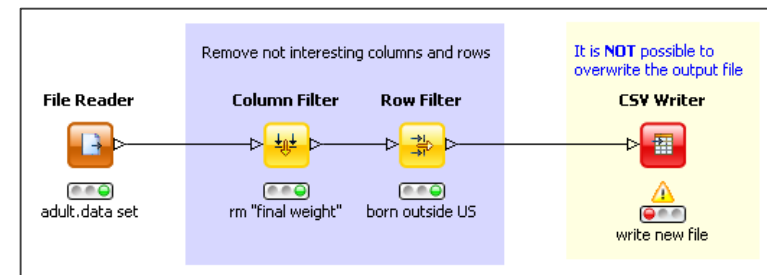
2.33. Workflow “my_first_workflow”
