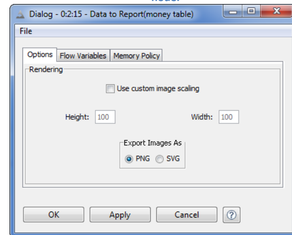
5.27. Configuration window of the “Data To Report” node.
