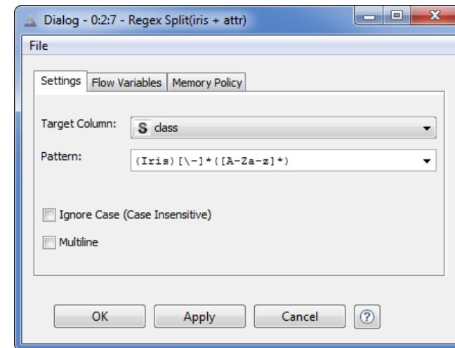
3.8. Configuration dialog for the "RegEx Split" node
