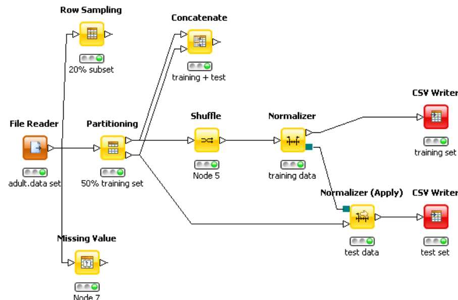
4.9. The “data_preparation” workflow
