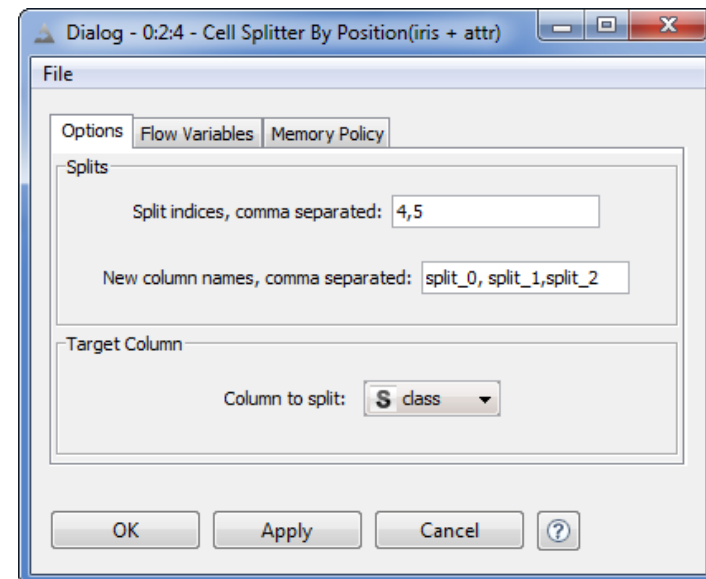
3.6. Configuration dialog for the "Cell Splitter by Position" node
