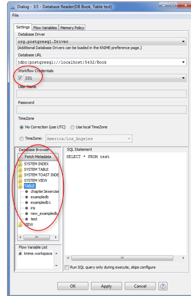
3.26. Configuration window of the „Database Reader“ node
