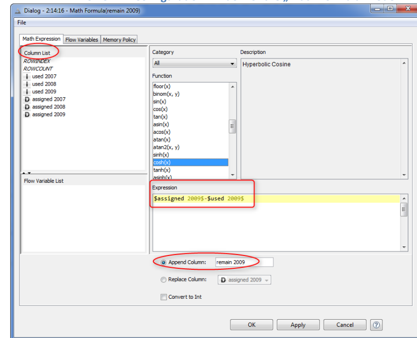
5.25. Configuration window of the „Math Formula“ node
