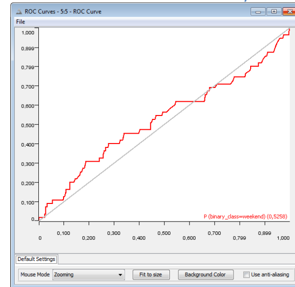
4.55. Exercise 3: ROC Curve on the results of the Bayesian classifier
