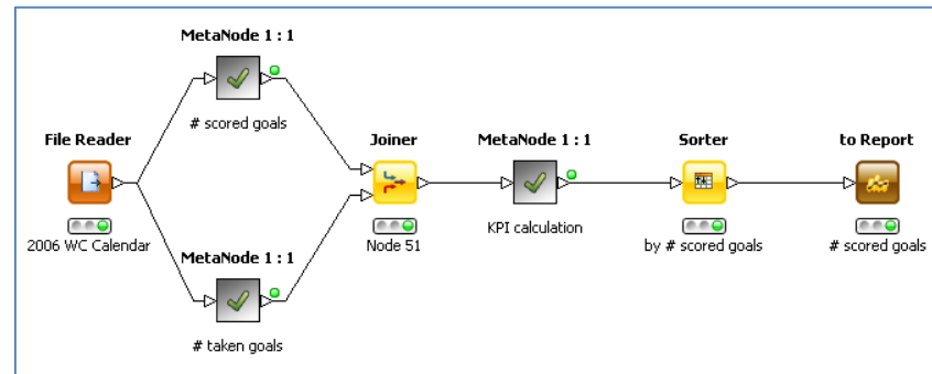
5.37. Meta-node "# scored goals"/"# taken goals"
