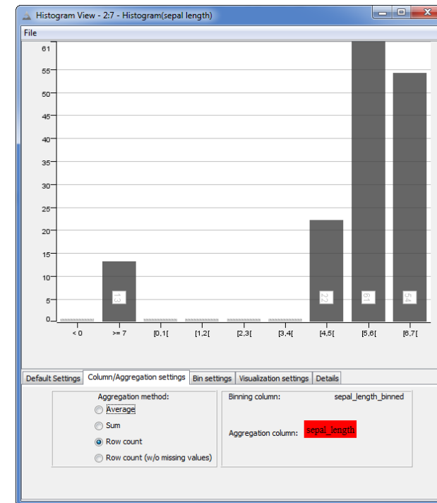
3.37. View window of the „Histogram“ node. The figure represents a histogram built on the prepared “sepal_length_binned” column
