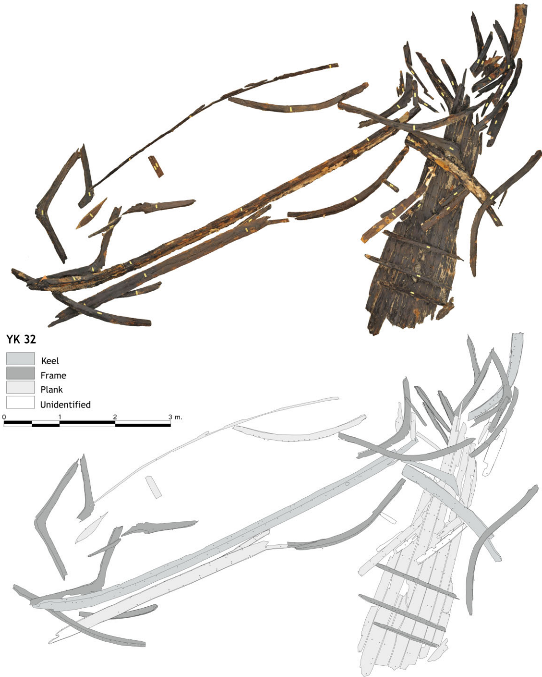
Figure 21. YK 32 wreck, drawing and photo-mosaic. (IU Yenikapı Shipwrecks Project Archive)
