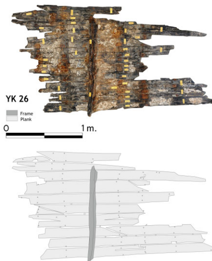
Figure 14. YK 26 wreck, drawing and photo-mosaic. (IU Yenikapı Shipwrecks Project Archive)
