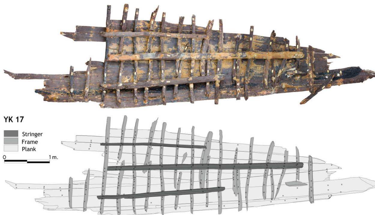
Figure 23. YK 17 wreck, drawing and photo-mosaic. (IU Yenikapı Shipwrecks Project Archive)
