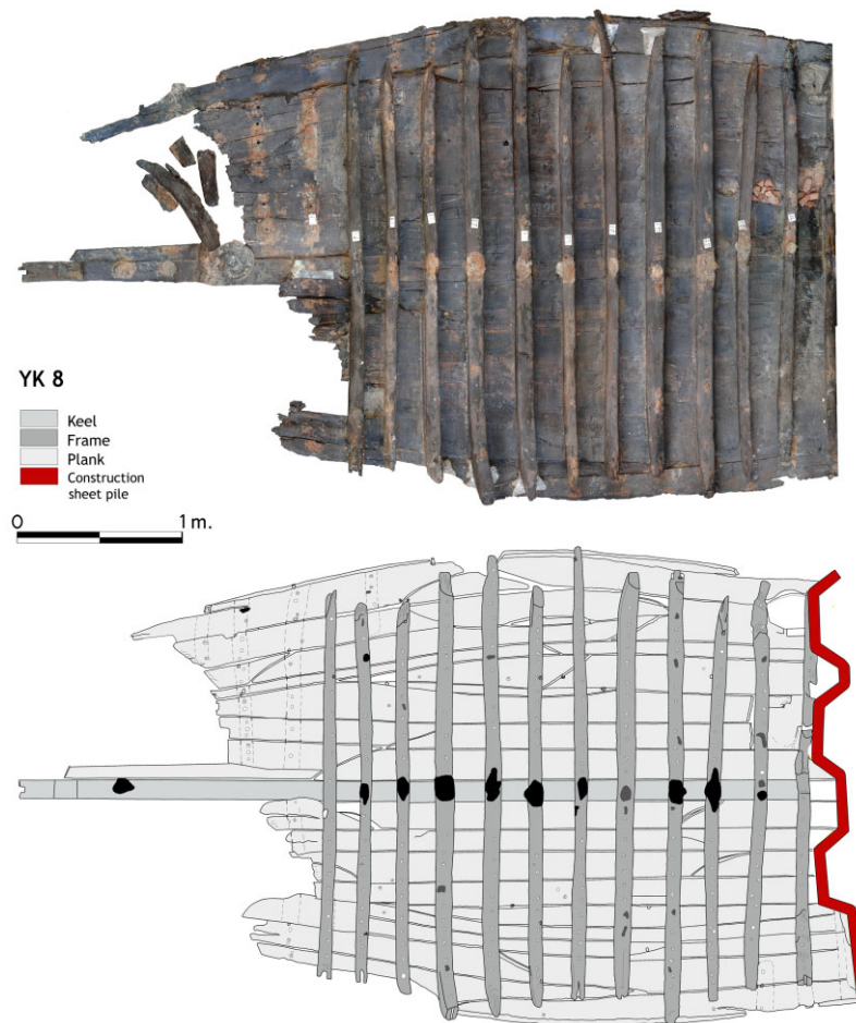
Figure 8. YK 8 wreck, drawing and photo-mosaic. (IU Yenikapı Shipwrecks Project Archive)
