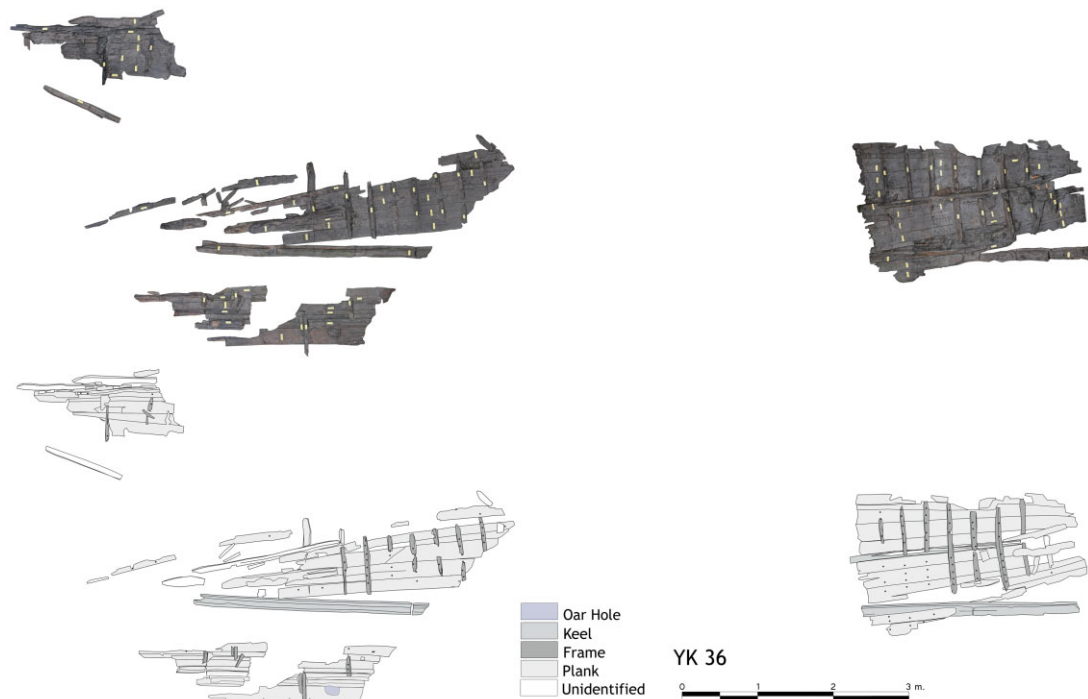
Figure 30. YK 36 wreck, drawing and photo-mosaic. (IU Yenikapı Shipwrecks Project Archive)
