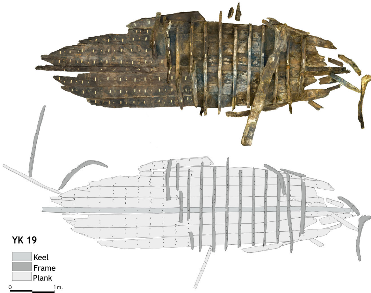
Figure 12. YK 19 wreck, drawing and photo-mosaic. (IU Yenikapı Shipwrecks Project Archive)
