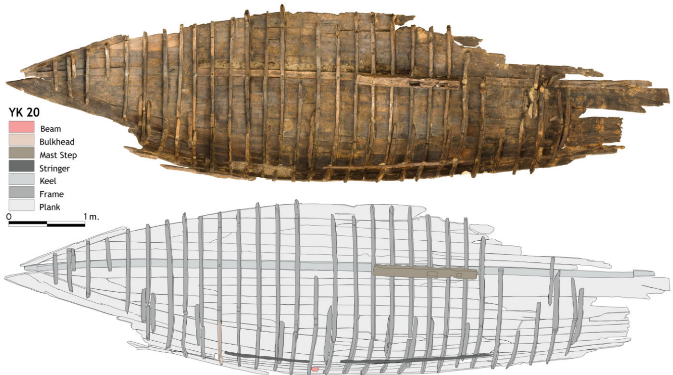
Figure 13. YK 20 wreck, drawing and photo-mosaic. (IU Yenikapı Shipwrecks Project Archive)
