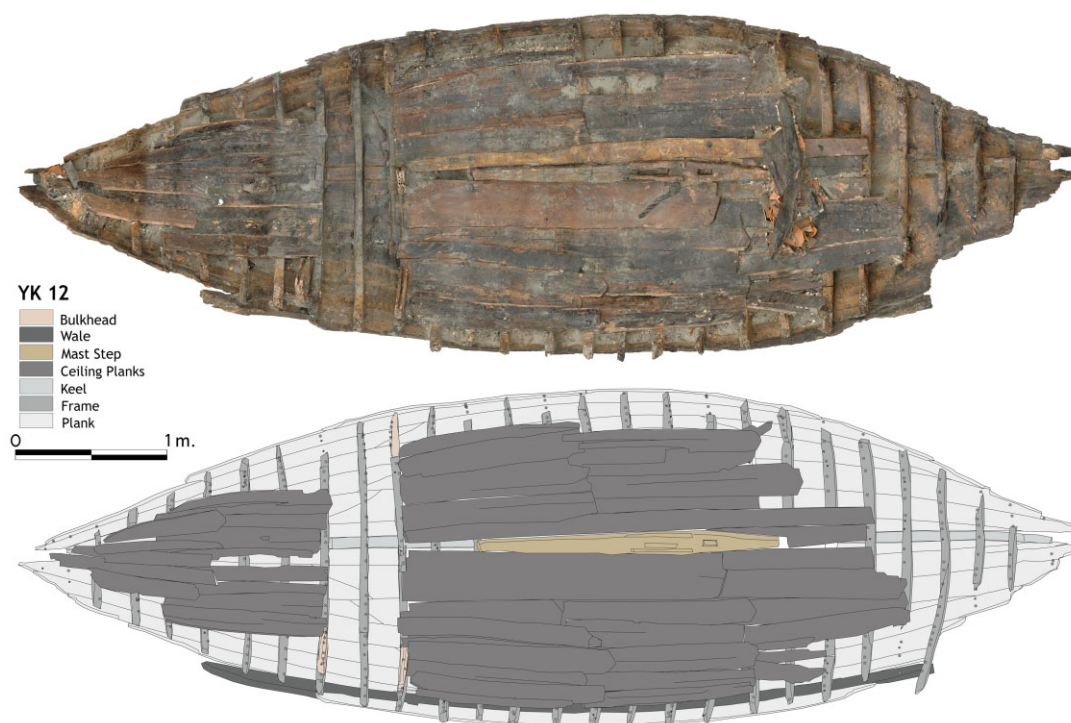
Figure 10. YK 12 wreck, drawing and photo-mosaic. (IU Yenikapı Shipwrecks Project Archive)
