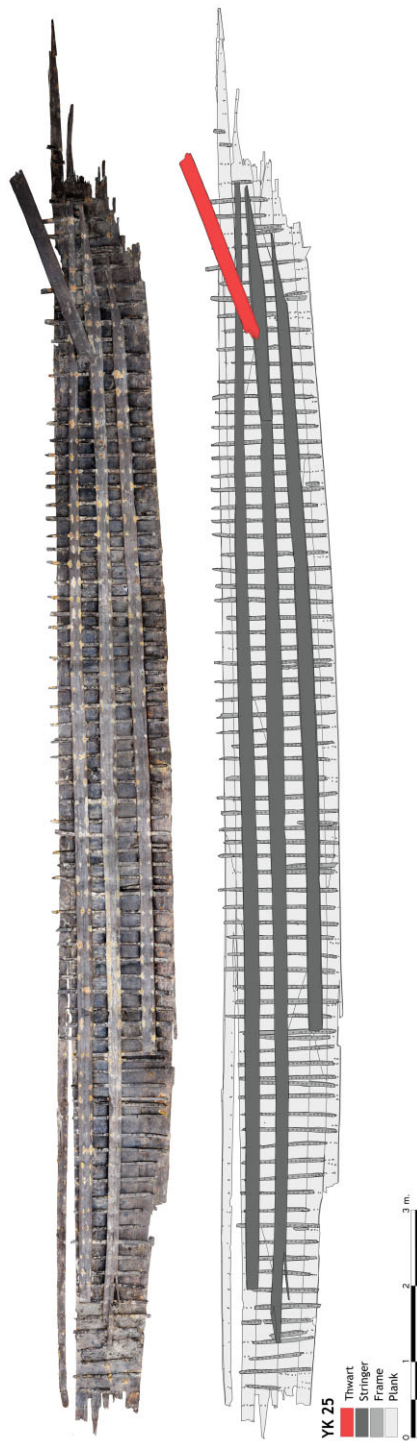
Figure 29. YK 25 wreck, drawing and photo-mosaic. (IU Yenikapı Shipwrecks Project Archive)
