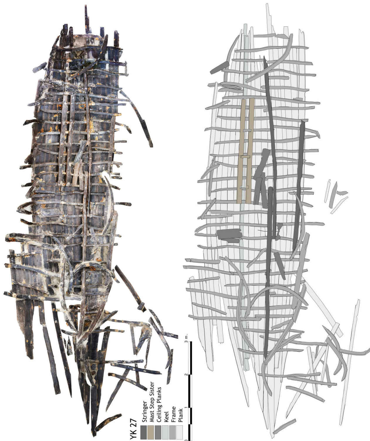
Figure 25. YK 27 wreck, drawing and photo-mosaic. (IU Yenikapı Shipwrecks Project Archive)
