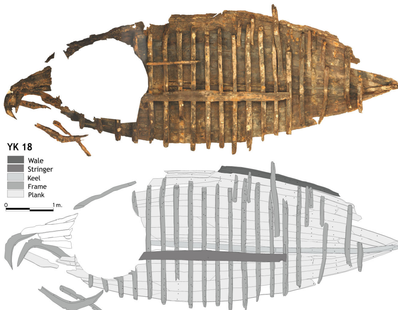
Figure 11. YK 18 wreck, drawing and photo-mosaic. (IU Yenikapı Shipwrecks Project Archive)
