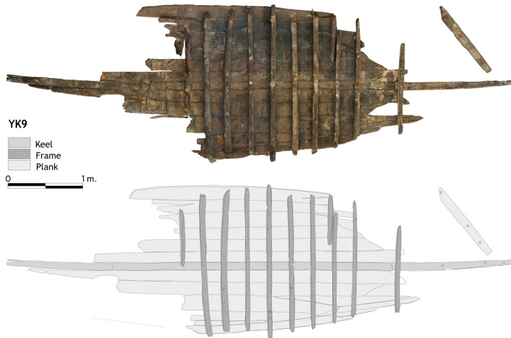
Figure 9. YK 9 wreck, drawing and photo-mosaic. (IU Yenikapı Shipwrecks Project Archive)
