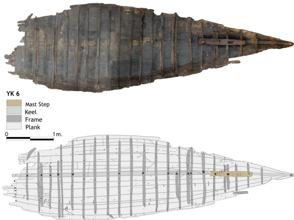
Figure 6. YK 6 wreck, drawing and photo-mosaic. (IU Yenikapı Shipwrecks Project Archive)
