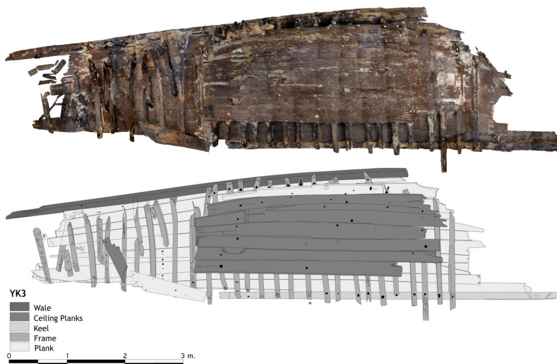
Figure 15. YK 3 wreck, drawing and photo-mosaic. (IU Yenikapı Shipwrecks Project Archive)
