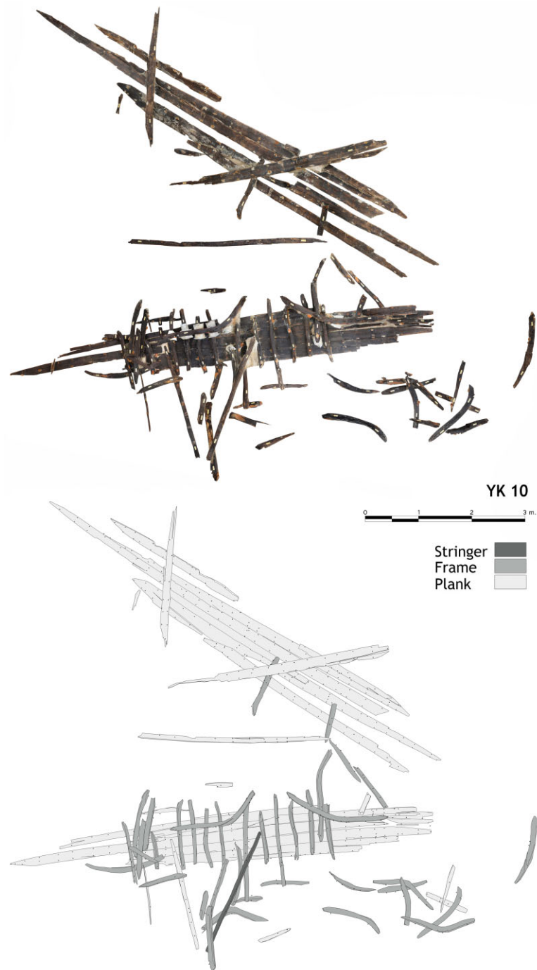
Figure 16. YK 10 wreck, drawing and photo-mosaic. (IU Yenikapı Shipwrecks Project Archive)
