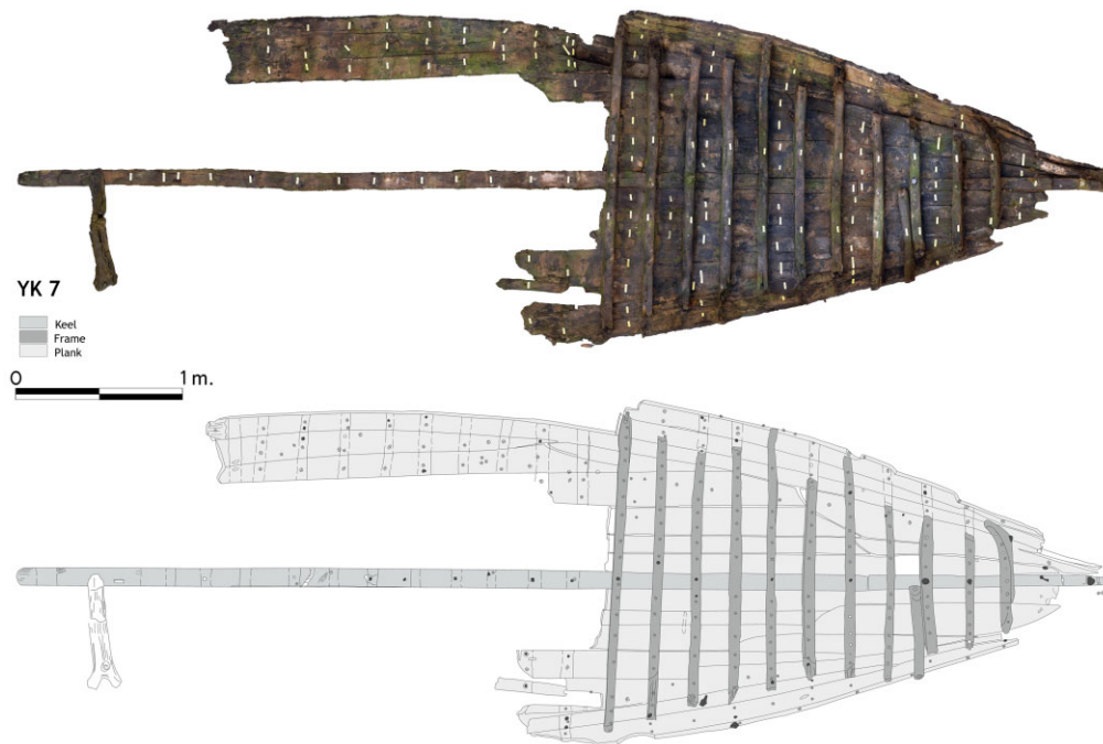
Figure 7. YK 7 wreck, drawing and photo-mosaic. (IU Yenikapı Shipwrecks Project Archive)
