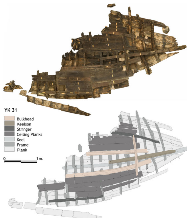
Figure 20. YK 31 wreck, drawing and photo-mosaic. (IU Yenikapı Shipwrecks Project Archive)
