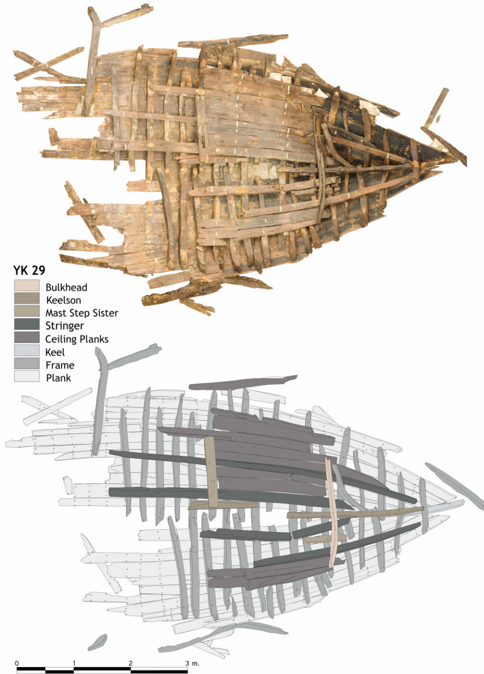
Figure 19. YK 29 wreck, drawing and photo-mosaic. (IU Yenikapı Shipwrecks Project Archive)
