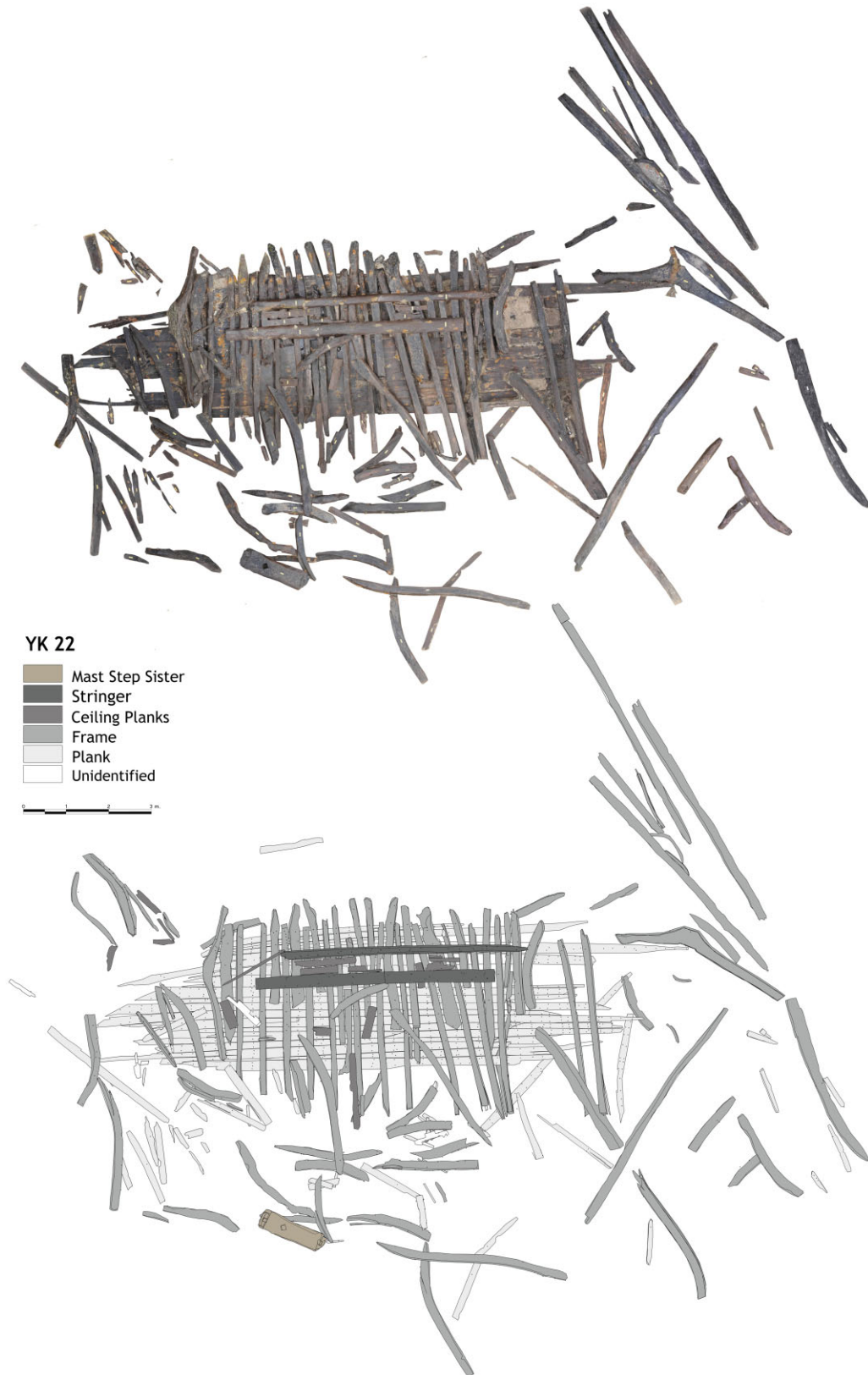
Figure 24. YK 22 wreck, drawing and photo-mosaic. (IU Yenikapı Shipwrecks Project Archive)
