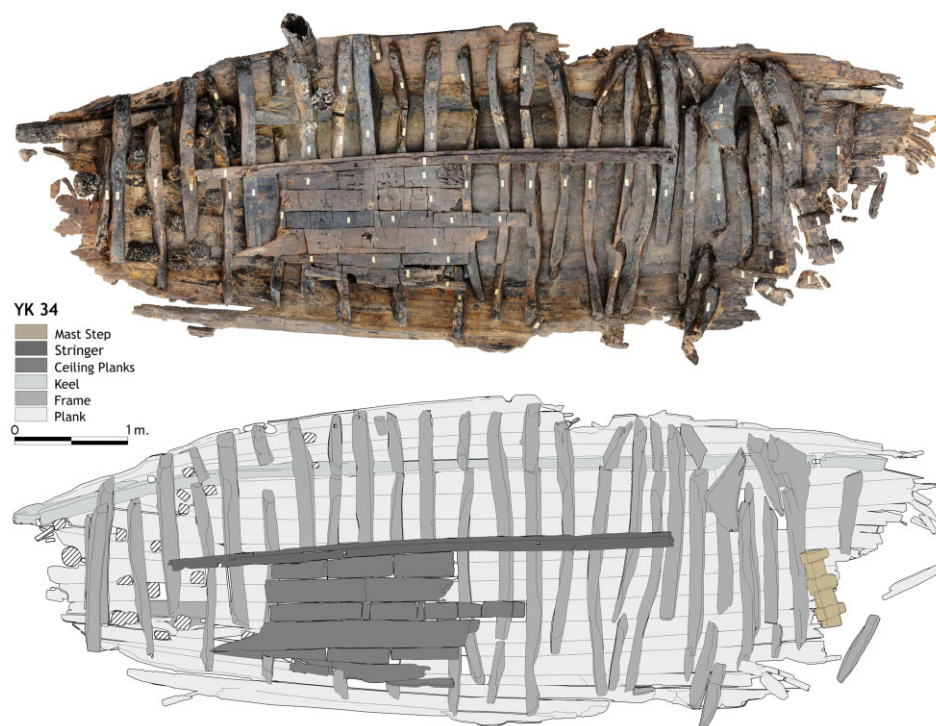
Figure 22. YK 34 wreck, drawing and photo-mosaic. (IU Yenikapı Shipwrecks Project Archive)
