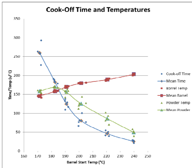
Figure 5. Cook-off temperatures and time (plotted on the same axes).
