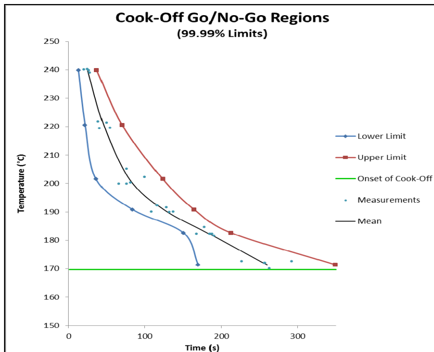
Figure 8. Time/Temperature relationships where cook-off is likely.
