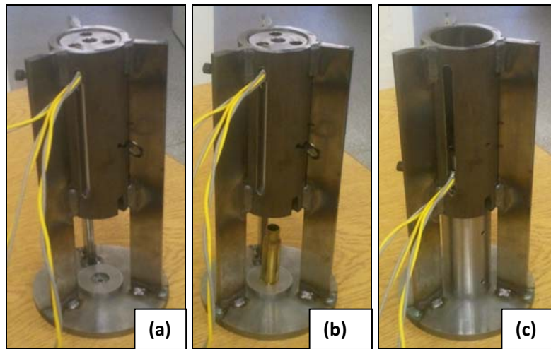
Figure 2. Test apparatus (a) unloaded, (b) loaded and (c) activated.
