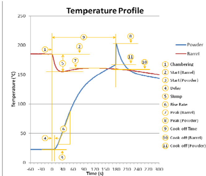
Figure 4. Characteristic curve key features.
