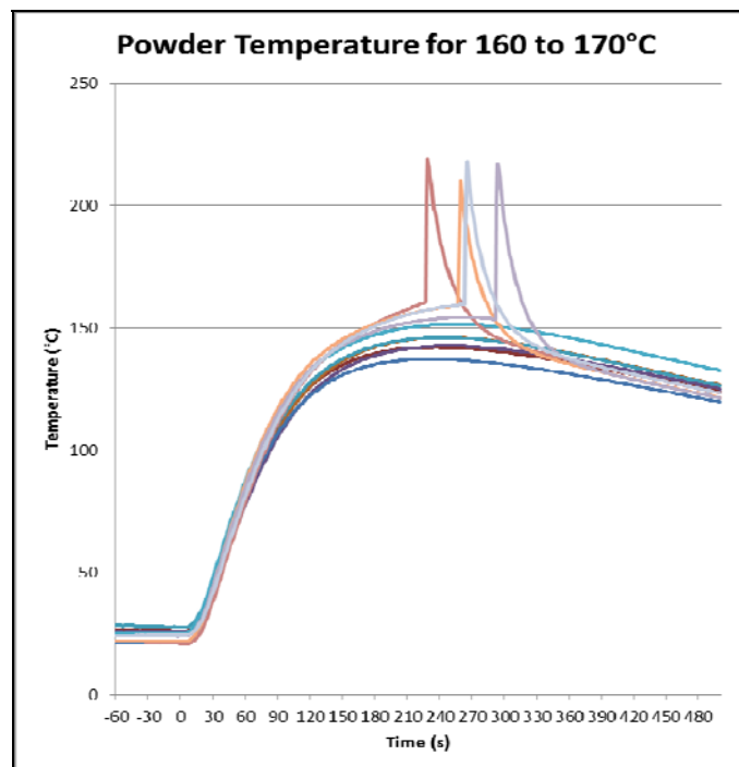
Figure 7. Bulls Eye Propellant Temperature plot (160 to 170°C range).
