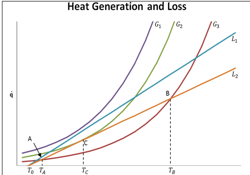
Figure 1: Heat generation (G) and loss (L)
