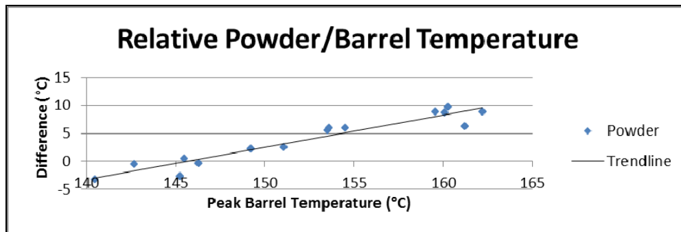
Figure 6. Relative powder to barrel temperatures.
