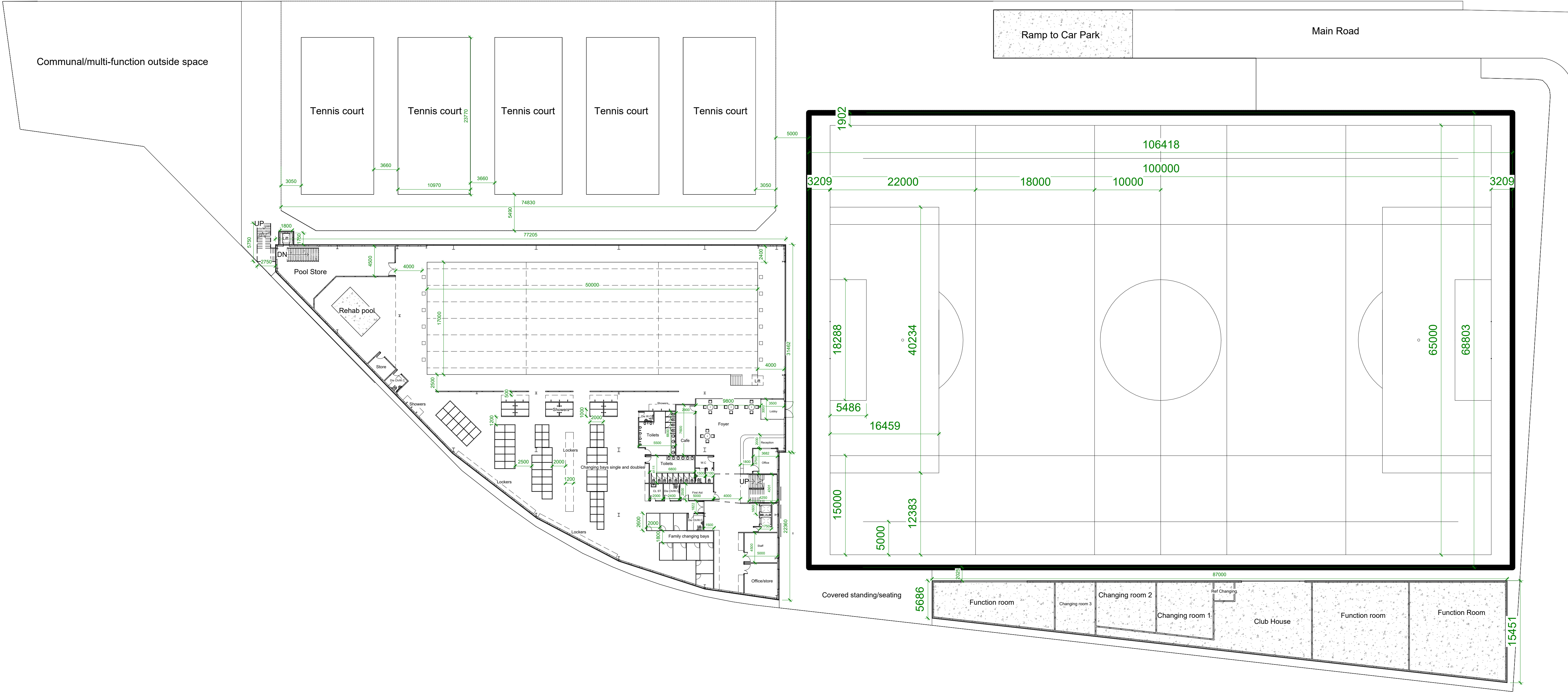
Ground Floor Whole Site 1 : 300
