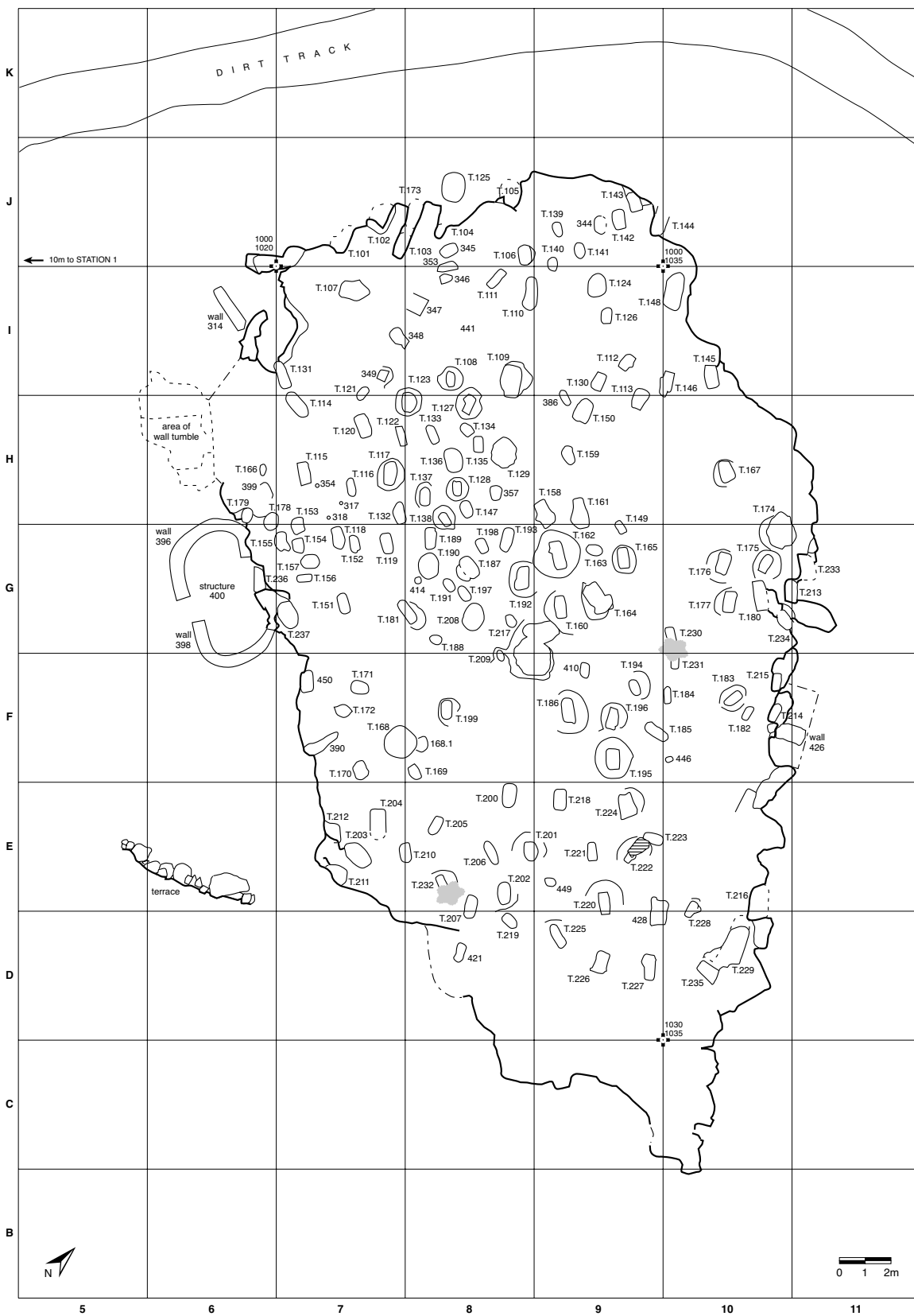
Figure 4: Plan of Souskiou-Laona at the end of the 2004 season
