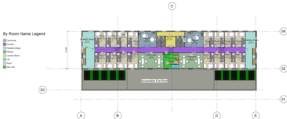
2 02 - First Floor 1 : 200
