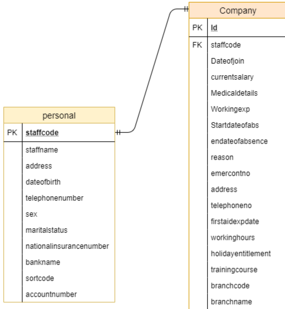
Figure: Entity-Relationship diagram
