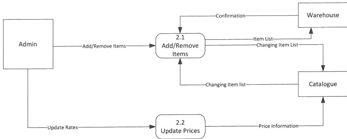
Level 1 DFD – Admin Catalogue Updates
