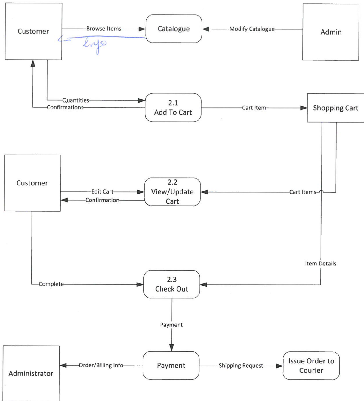
Level 1 DFD – Shopping Cart
