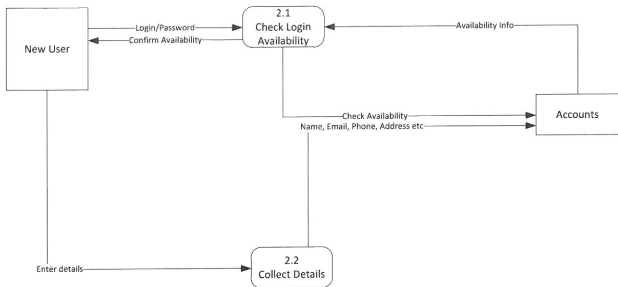
Level 1 DFD - Registration
